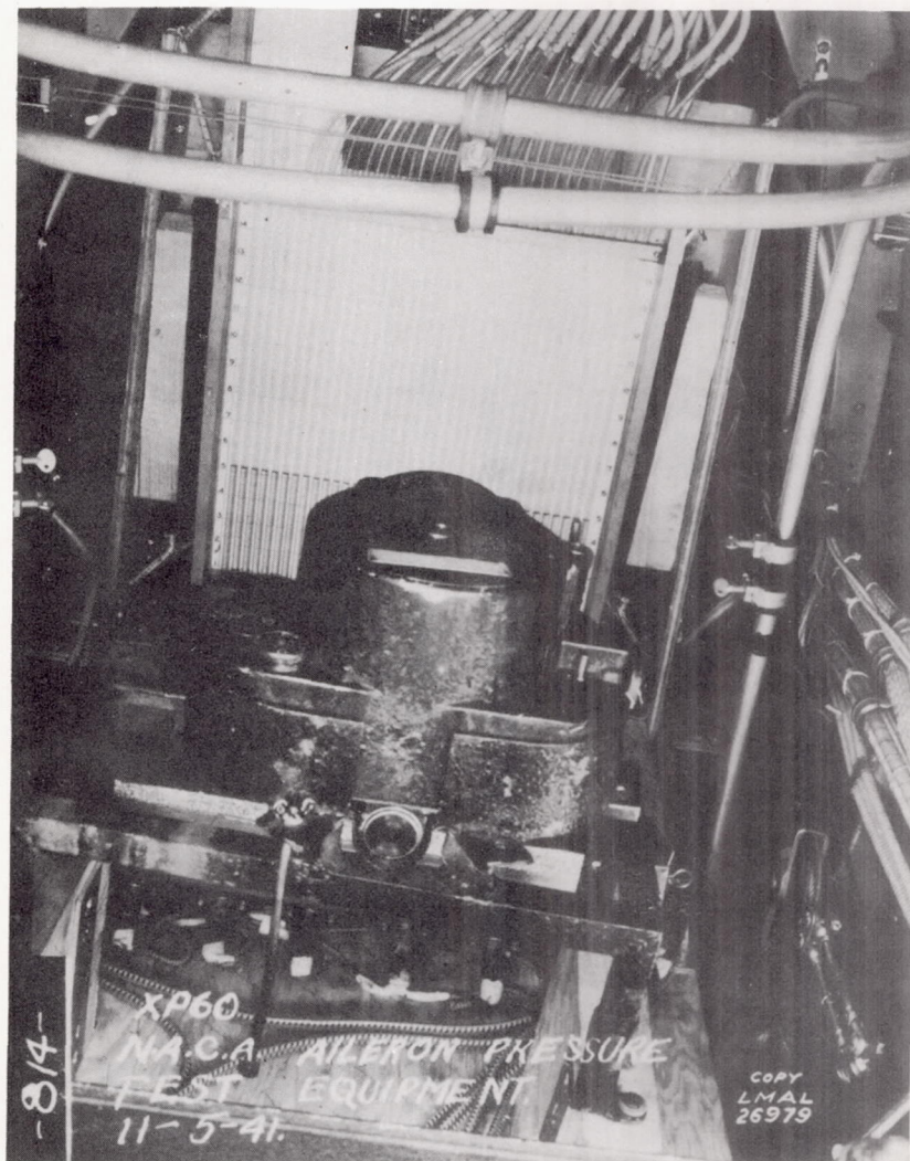
Figure 2.- Liquid manometer and recording camera mounted in fuselage.
