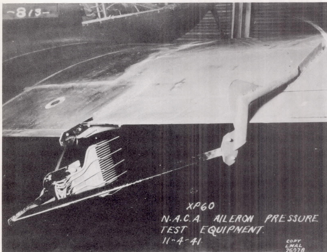
Figure 1.- Survey rake mounted behind wing.
