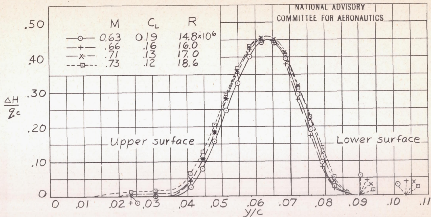
Figure 7.- Wake profiles for smooth surfaces with transition fixed at 5 percent of the chord. ( y/c=0.0235 corresponds to top tube in wake-survey rake and y/c=0.1035 to bottom tube.)
