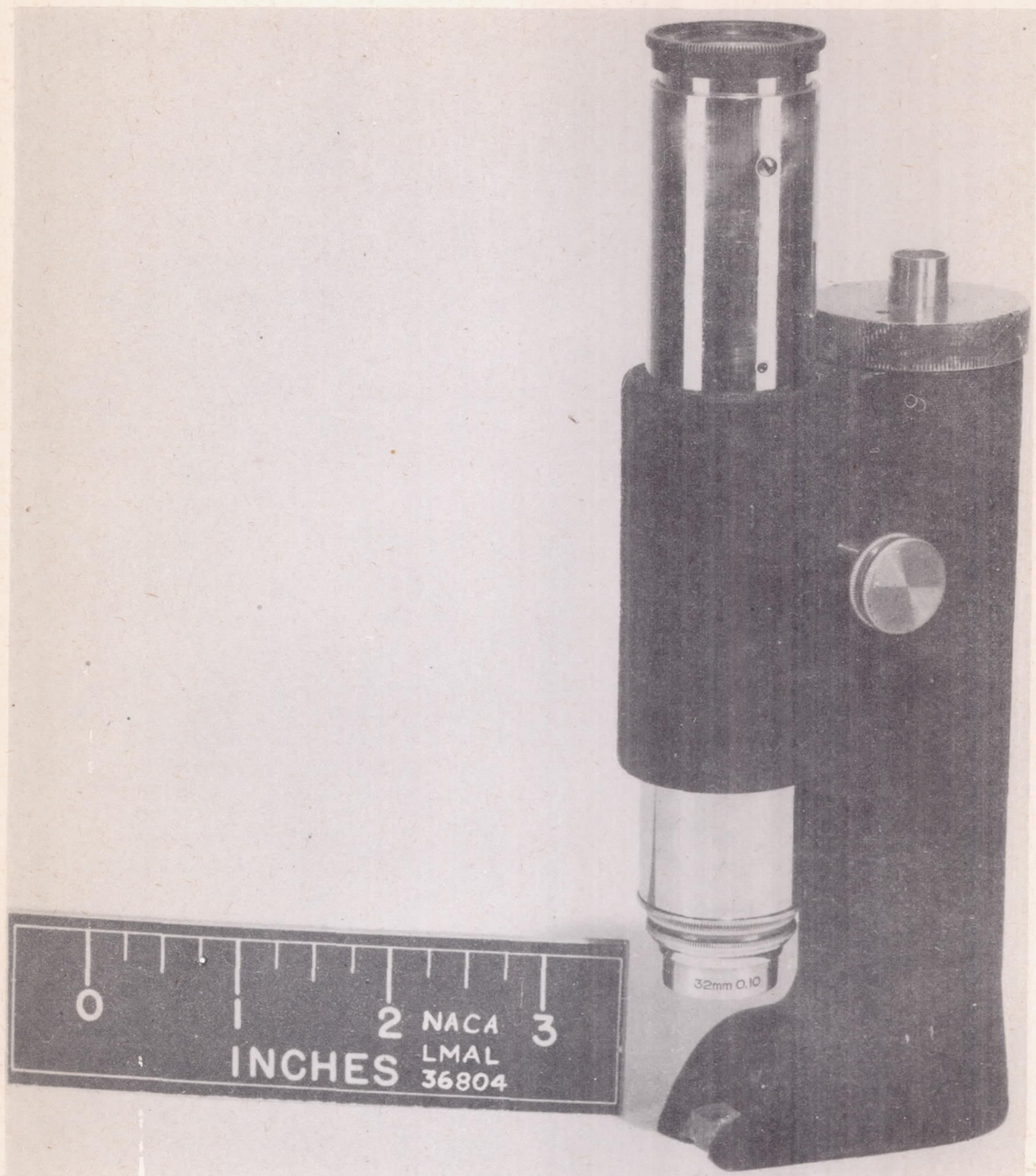
Figure 3.- Microscope with prism attached to base used in measuring surface roughness.
