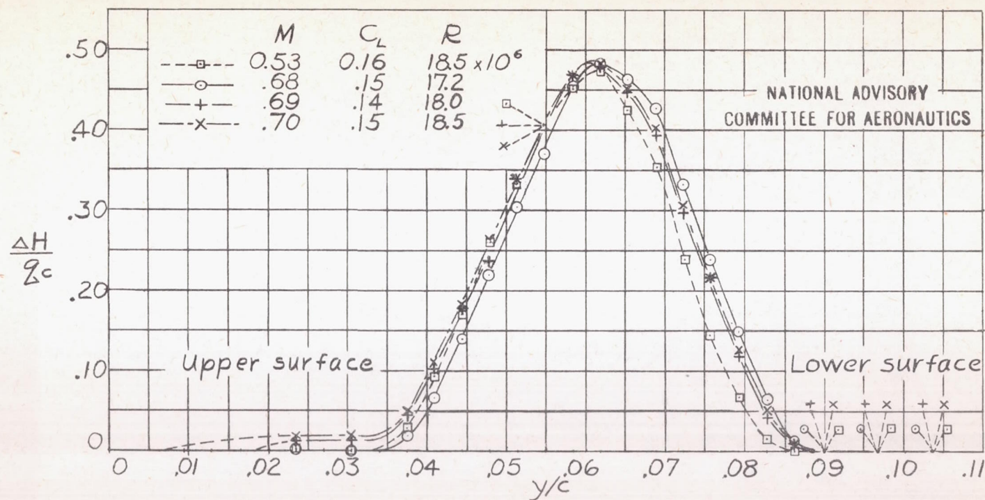
Figure 6.- Wake profiles for roughened surfaces with transition fixed at 5 percent of the chord. ( y/c=0.0235 corresponds to top tube of wake-survey rake and y/c=0.1035 to bottom tube.)
