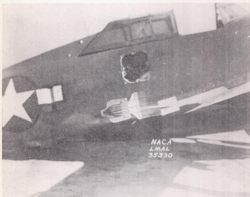
Figure 4.- Wake-survey rake installed on P-47D airplane.
