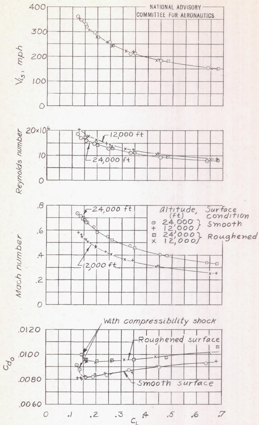
Figure 5:- Profile-drag coefficients for smooth and roughened surfaces with transition fixed at 5 percent chord. Mach number, Reynolds number, and indicated airspeed are plotted above the profile-drag curves.
