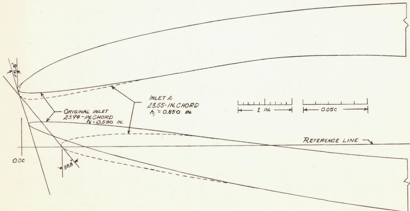
Figure 5.- Profiles of the original and modified inlets.
