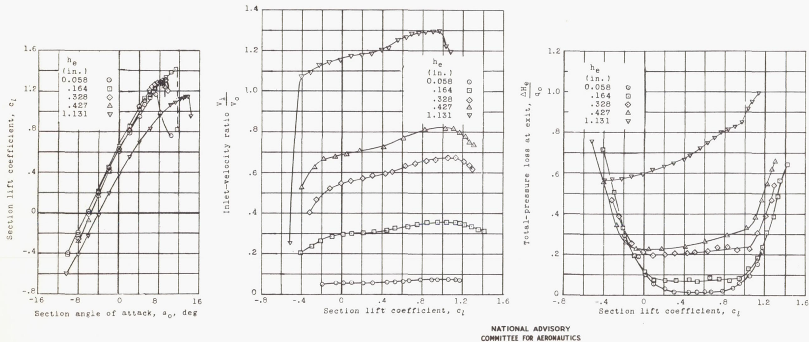
Figure 13.- Aerodynamic characteristics of the wing inlet section with inlet 5, modified exit, and baffle plate in duct; tests, LTT 399 and TDT 763.
