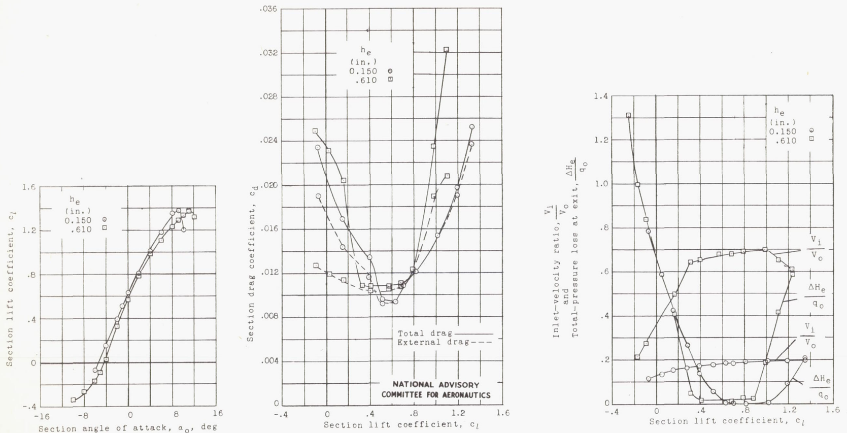
(a) Lift, drag, and flow characteristics.
