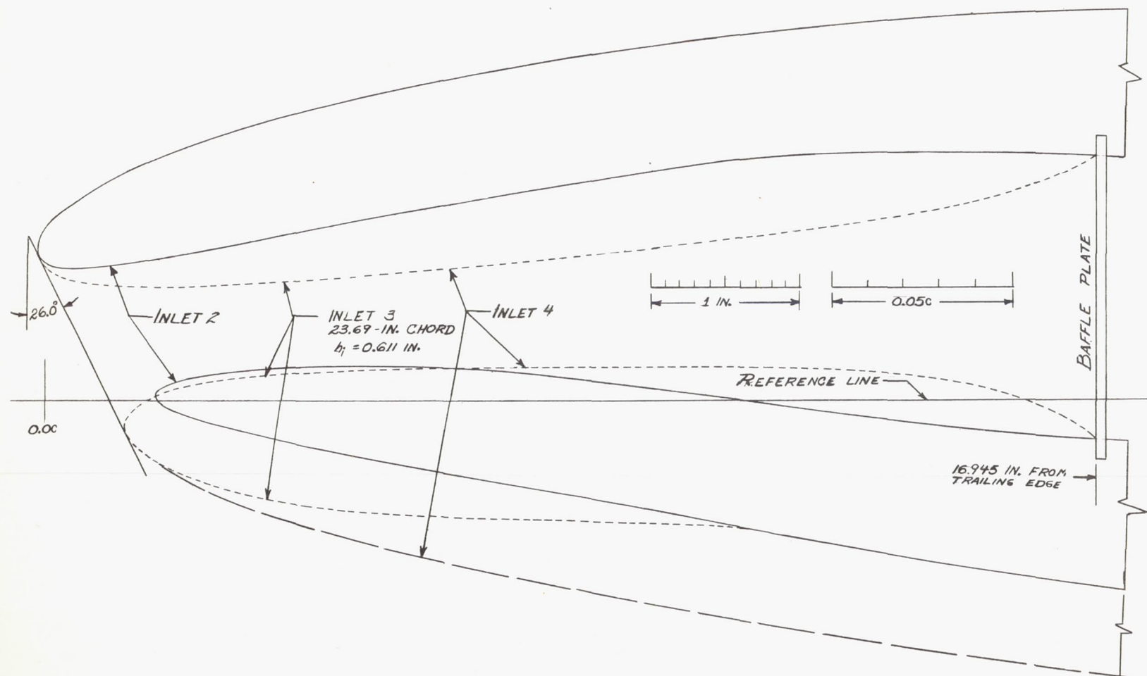
(a) Profiles of inlets 2, 3, and 4.
