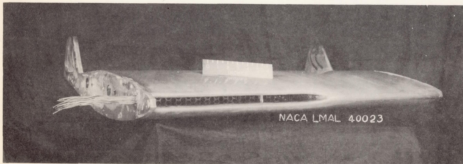
(b) Three-quarter view of model inverted showing fairing between ducted and plain airfoil sections.
