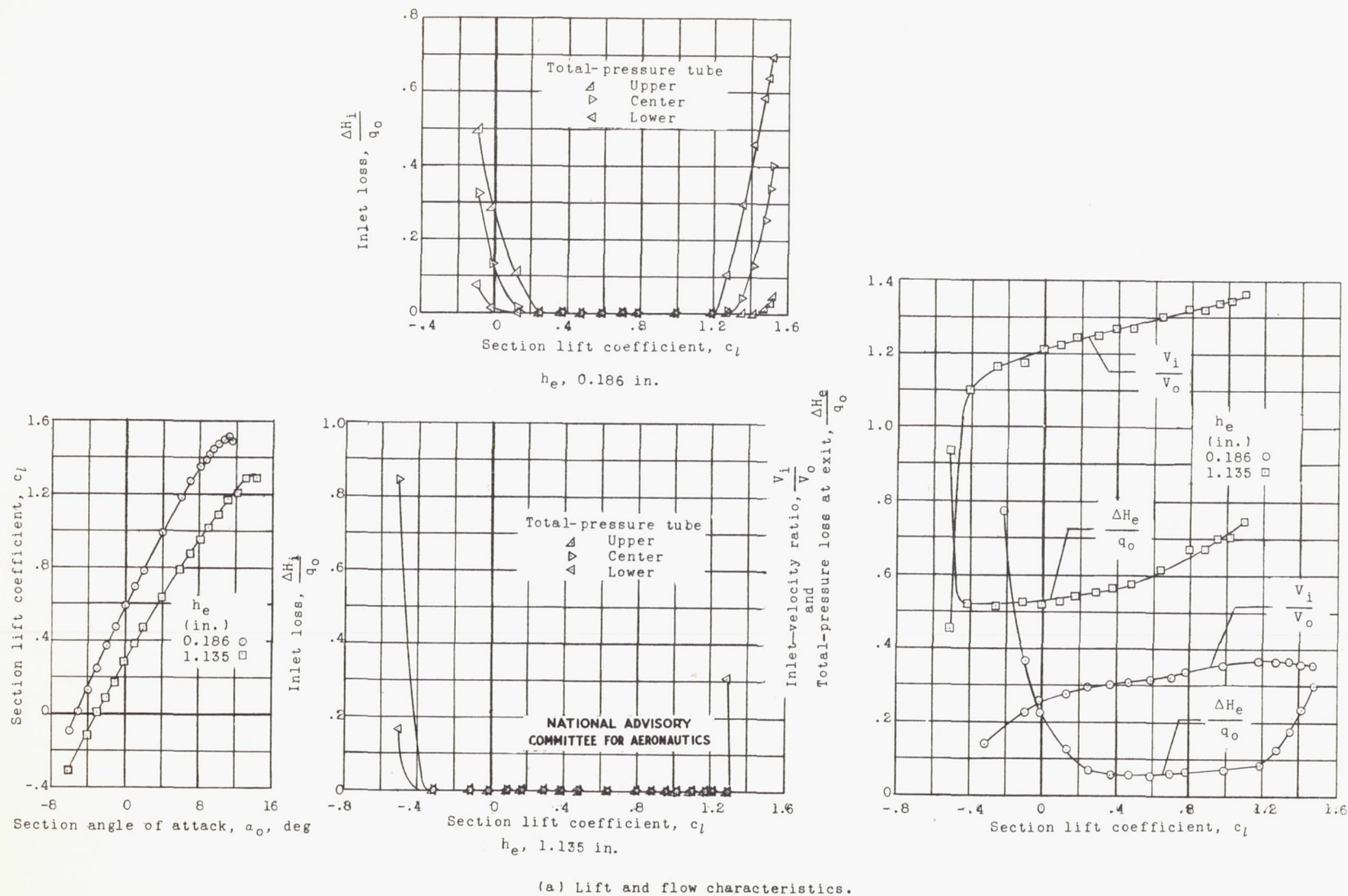
Figure 10.- Aerodynamic characteristics of the wing-inlet section with inlet 3, modified exit, and baffle plate in duct; R, 2.4 \times 10^6 ; test, LTT 380.
