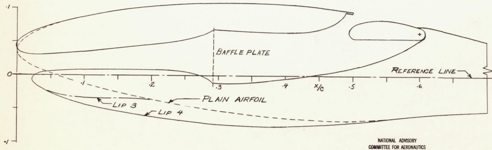
(b) Sketch showing blister required to fair lip 4 into plain airfoil section.
