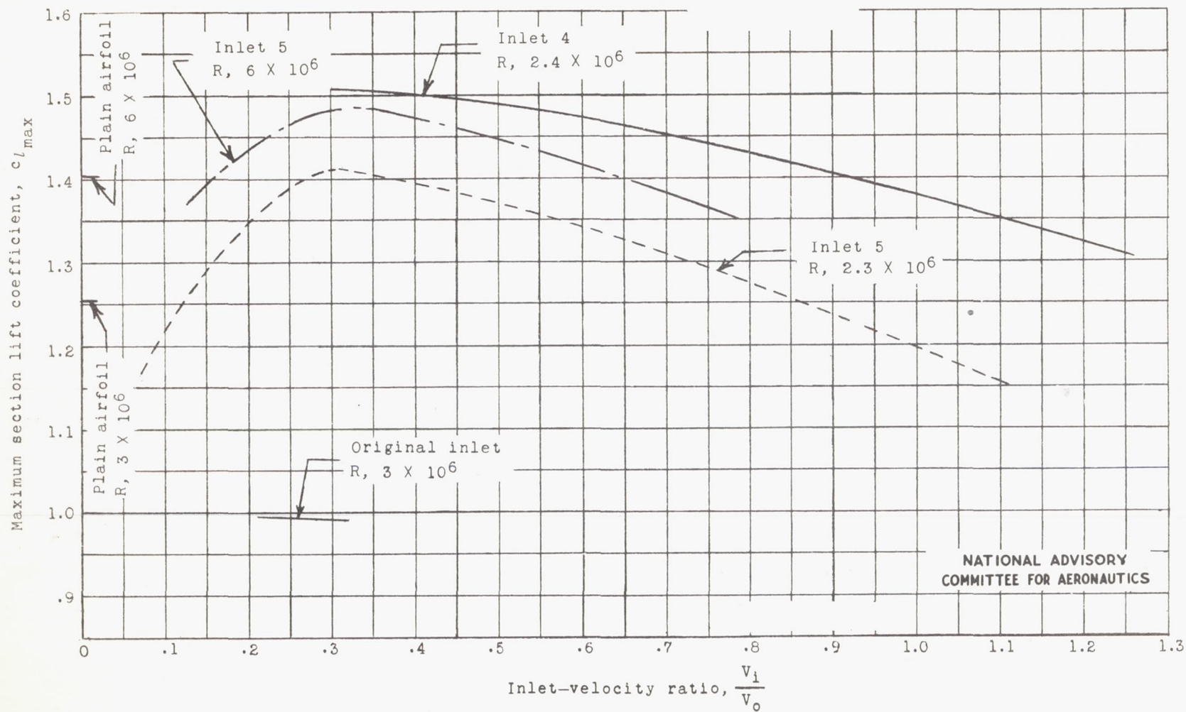
(a) Maximum lift characteristics.
