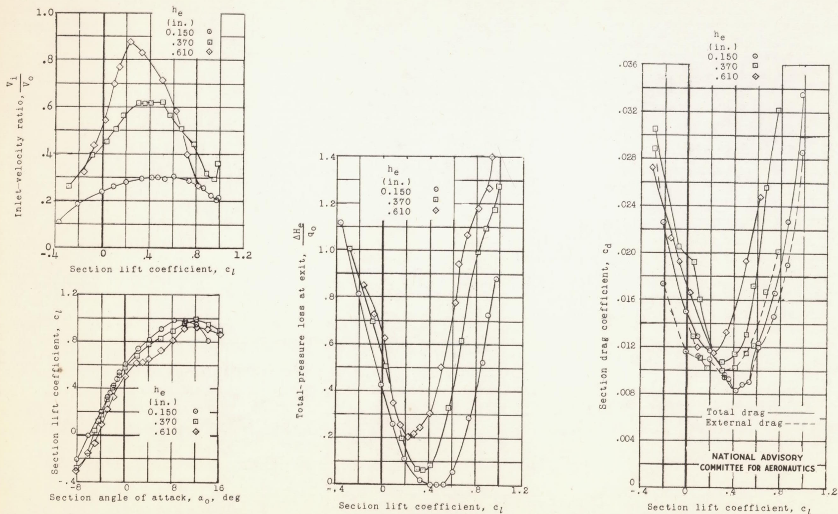
(a) Lift, drag, and flow characteristics; R, 3 \times 10^6 .
