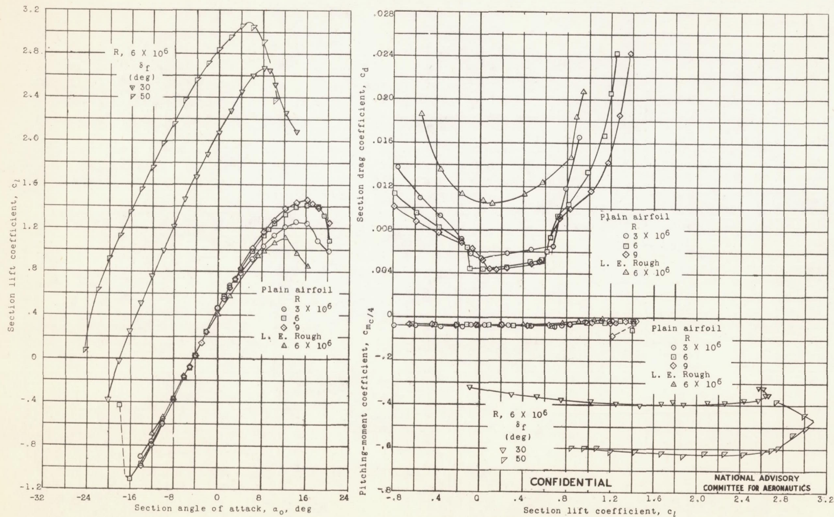
(a) Lift, drag, and pitching-moment characteristics.
