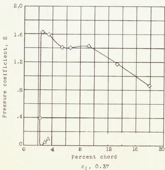
(b) Pressure distributions, lower surface; h_e , 0.186 inches.
