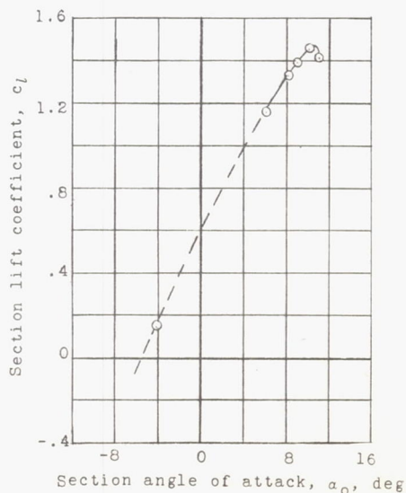
Figure 11.- Pressure distributions on the lower surface and lift characteristics of the wing inlet section with inlet 4, modified exit, and baffle plate in duct; h_e, 0.188 inches; R, 2.0 \times 10^6 ; test, LTT 380.
