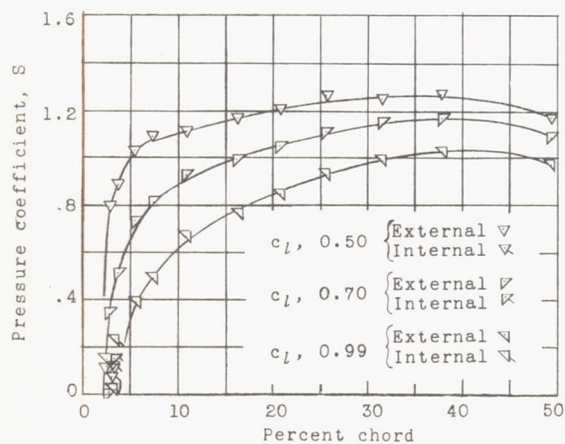
Figure 11.- Pressure distributions on the lower surface and lift characteristics of the wing inlet section with inlet 4, modified exit, and baffle plate in duct; h_e, 0.188 inches; R, 2.0 \times 10^6 ; test, LTT 380.
