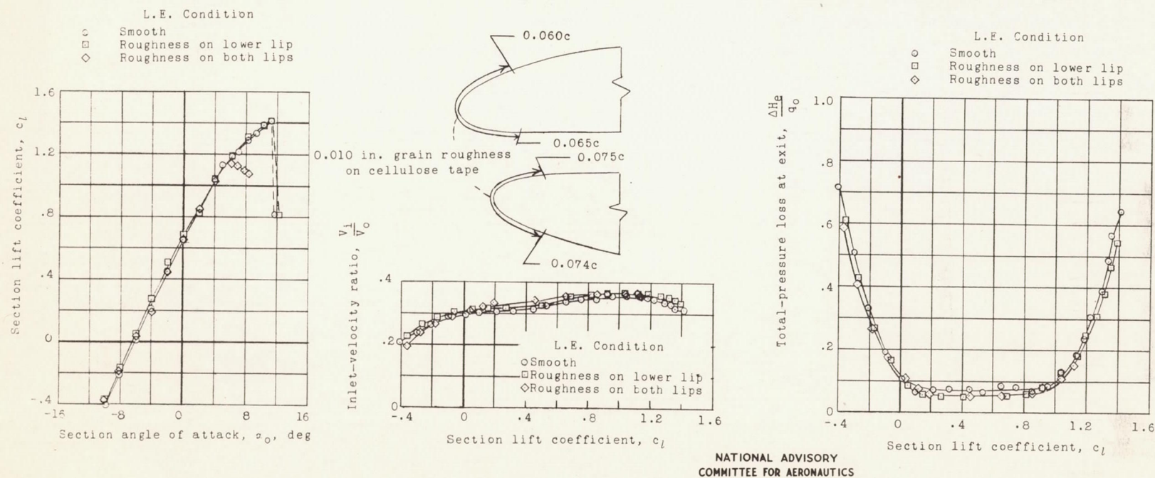
(f) Lift and flow characteristics with and without leading-edge roughness; h_e , 0.164 inches; R , 2.3 \times 10^6 .
