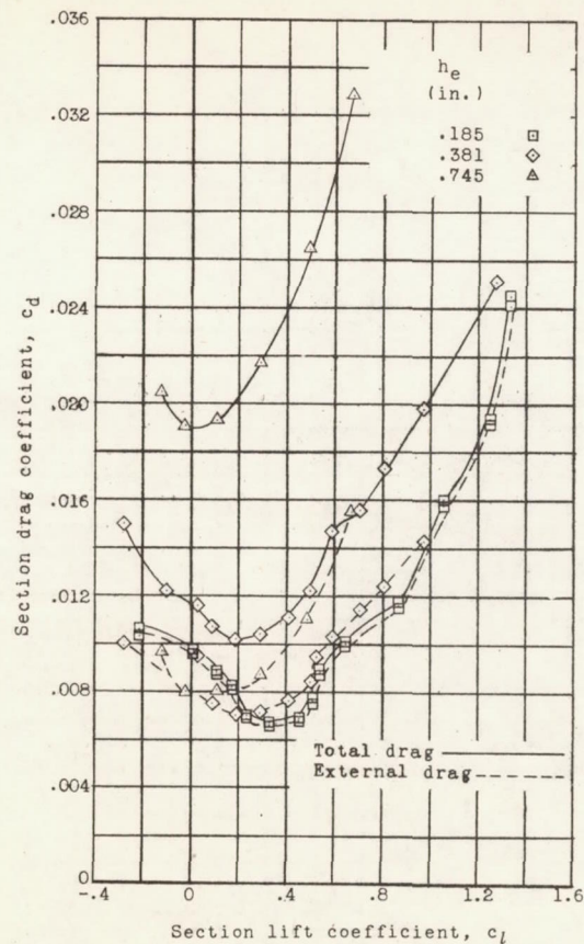
(e) Lift, drag, and flow characteristics; R, 6 \times 10^6 .
