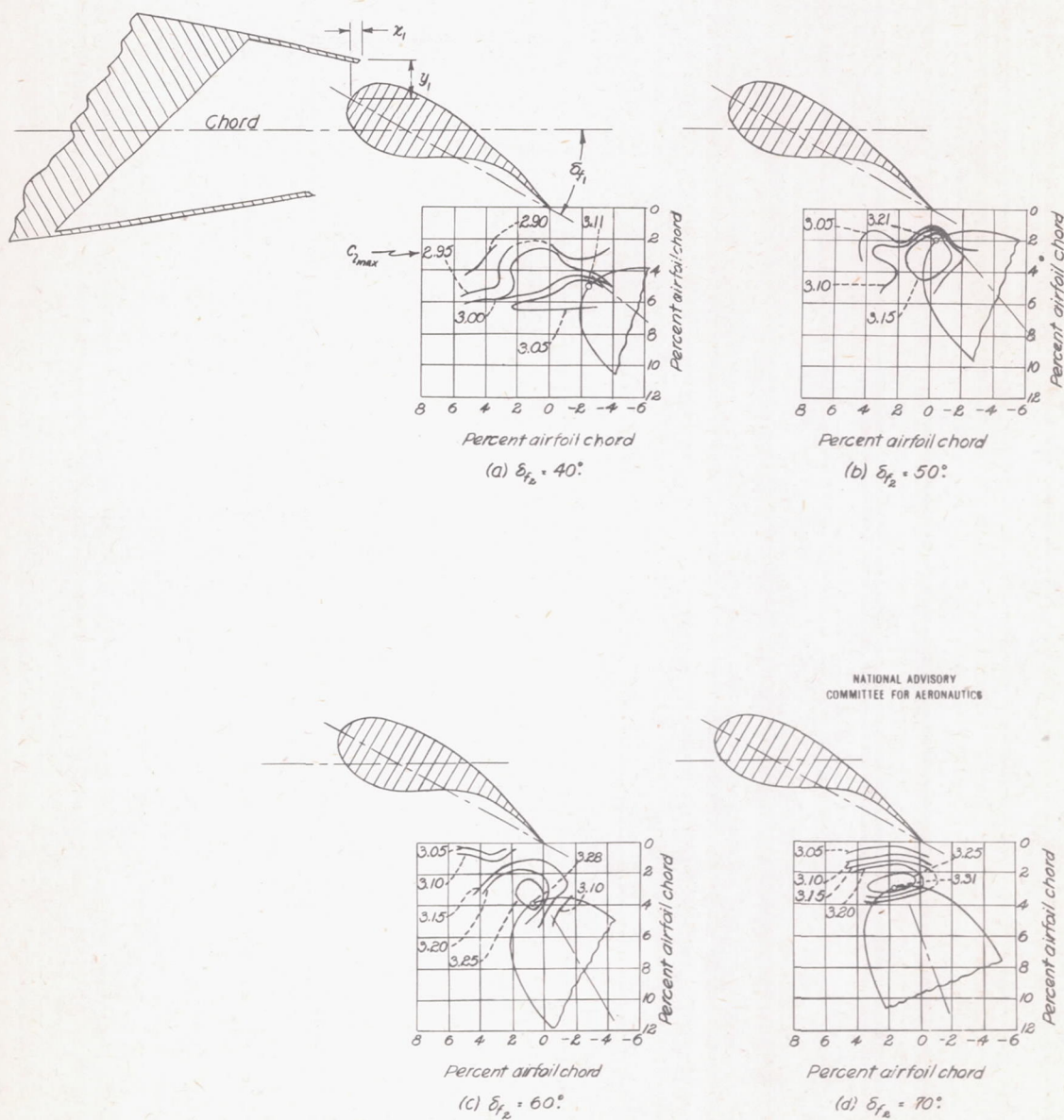
Figure 5.-Contours of rear-flap position for c_{l,max} . Position 3; \delta_{f_1} = 30^\circ ; x_1 = 0.70 ; y_1 = 2.45 . (Values of x_1, y_1 are given in percent airfoil chord.)
