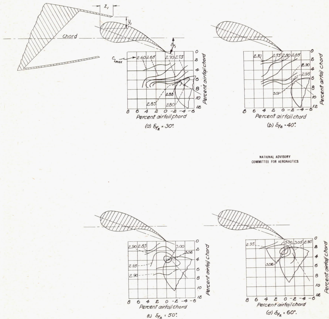
Figure 4.-Contours of rear-flap position for C_{lmax} . Position 2; \delta_{f1} = 20^\circ ; x_1 = 2.70 ; y_1 = 2.45 . (Values of x_1, y_1 are given in percent airfoil chord.)
