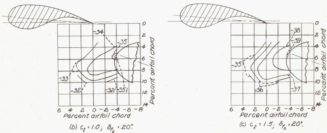
Figure 9.- Contours of rear-flap position for C_{m(a,c)_0} . Position 1; \delta_{f_1} = 5^\circ ; x_1 = 5.70 ; y_1 = 3.45 . (Values of x_1, y_1 are given in percent airfoil chord.)
