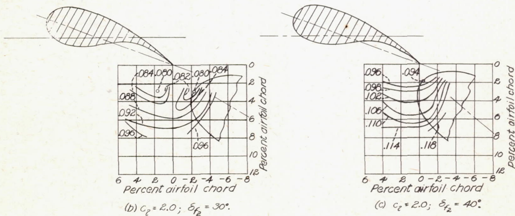
Figure 7.- Contours of rear flap position for c_{L0} . Position 2; \delta_{f_1} = 20^\circ ; x_1 = 2.70 ; y_1 = 2.45 . (Values of x_1, y_1 are given in percent airfoil chord.)
