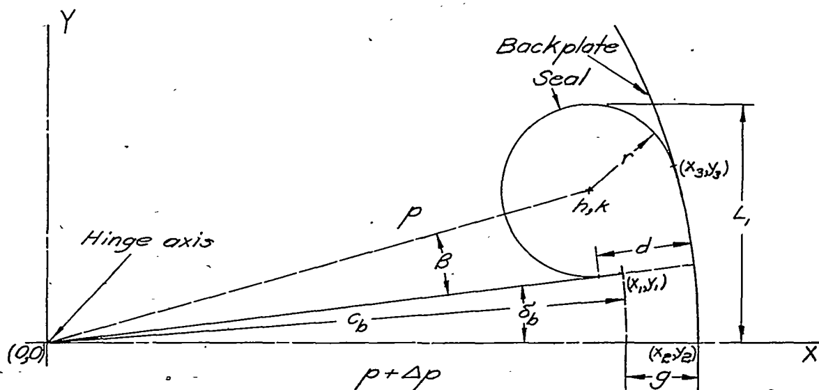
(b) Seal lying against the overhang. NATIONAL ADVISORY COMMITTEE FOR AERONAUTICS Figure 5. - Internal balance with seal and circular-arc backplate; center at (0,0).
