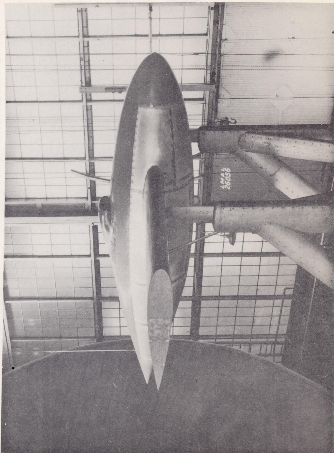
Figure 1.- Model with scoop B-1-c mounted in tunnel.
