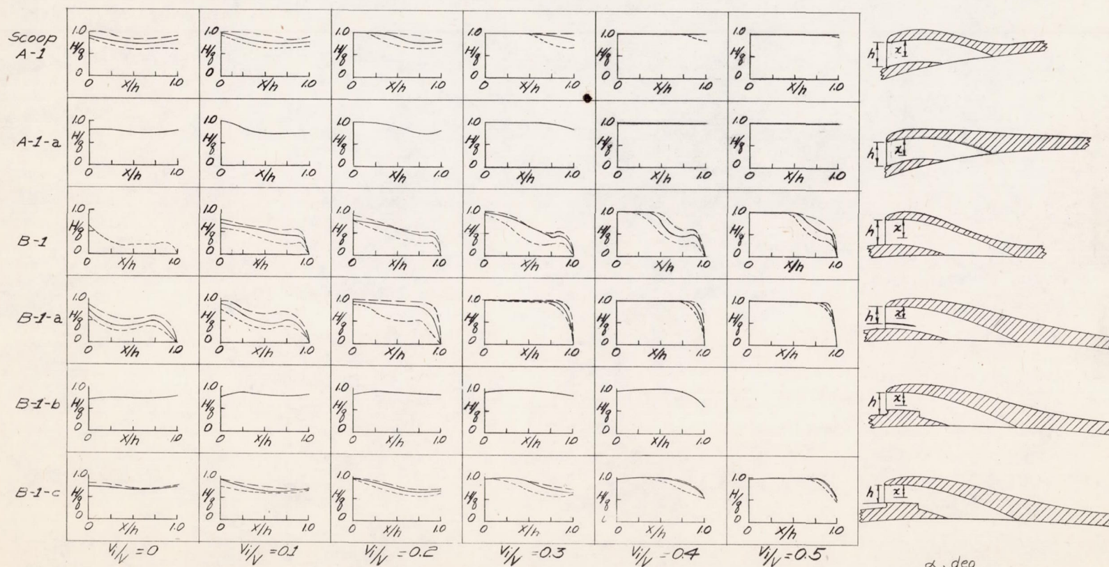
Figure 11.— Comparison of total pressures available in scoop entrances. (Measure with 60 th scale)
