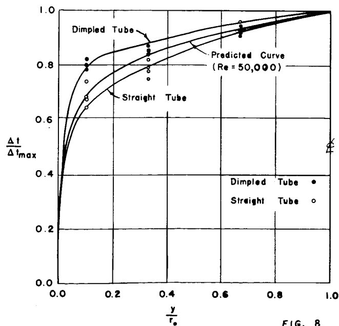
TEMPERATURE DISTRIBUTIONS AT OUTLET OF STRAIGHT AND DIMPLED TUBES WITHOUT MIXING CHAMBERS
