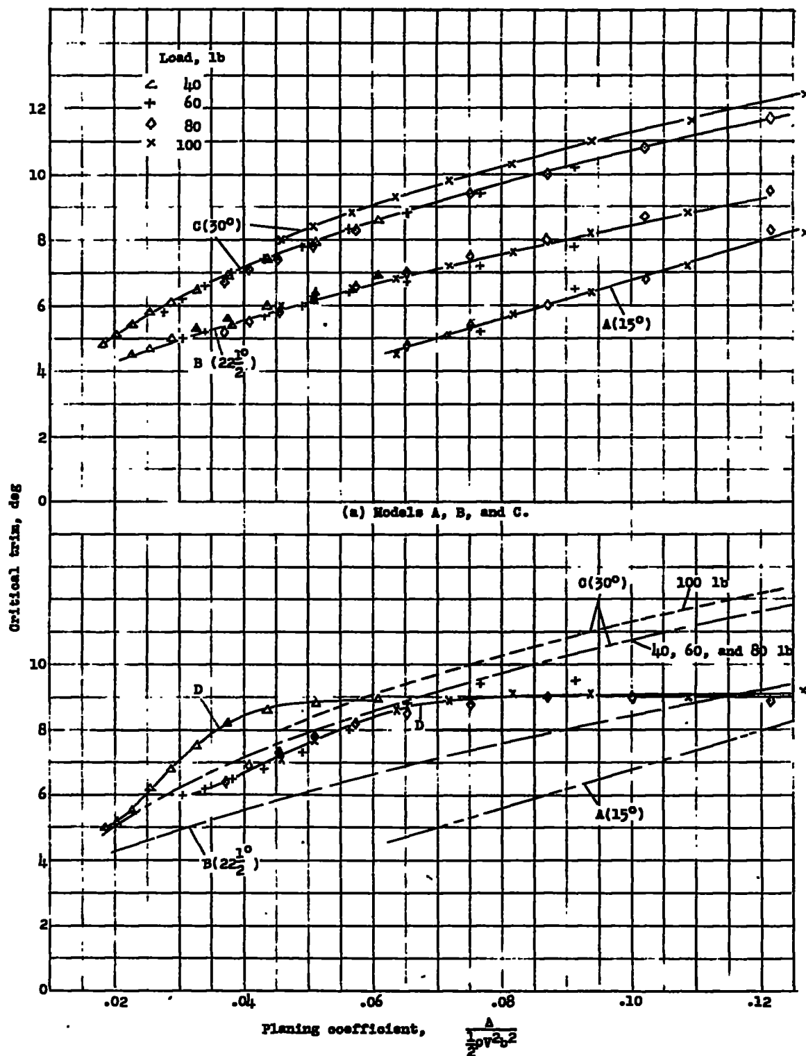
Figure 6.- Variation of critical trim with planing coefficient. Plotted points are from faired curves of figure 3.
