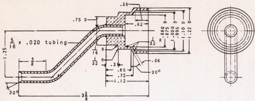
(b) Fuel-transfer tube.
