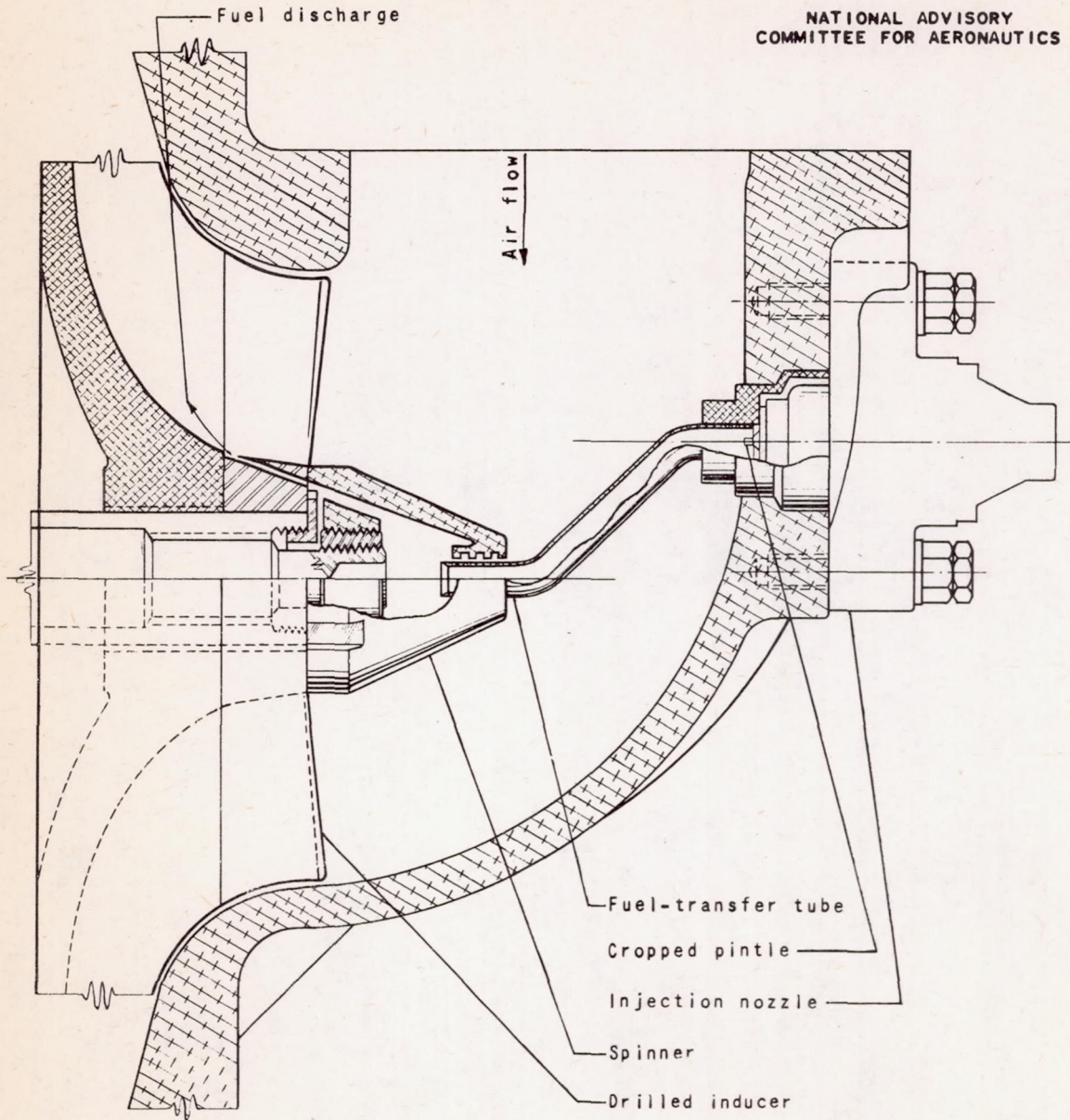
(a) Cross-sectional view of installation.
