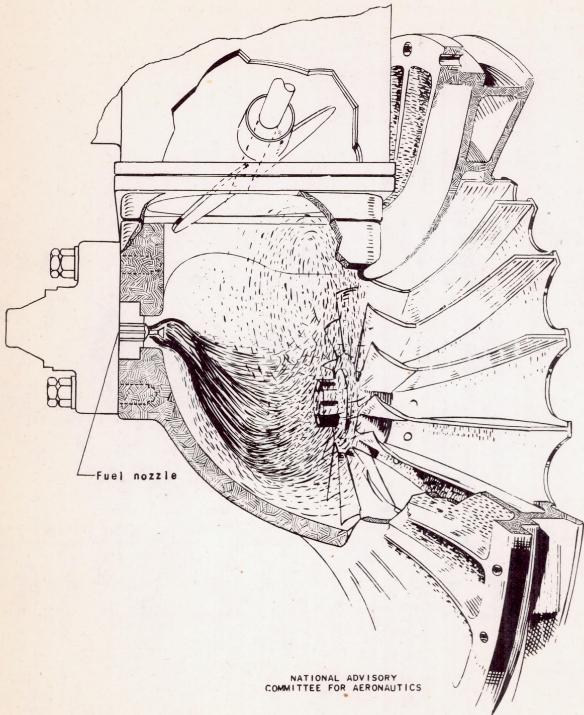
(b) Air flow, 5775 pounds per hour; fuel-air ratio, 0.080. Figure 5. - Continued. Fuel-spray pattern of Standard injection nozzle in the supercharger inlet elbow of an aircraft engine.
