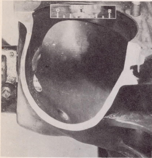
(a) Conventional nozzle lowered to center line of impeller.
