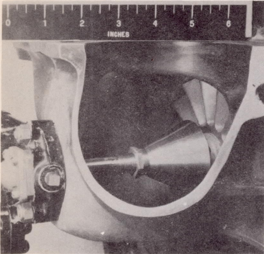
(i) Extended nozzle lowered to center line of impeller using a 360° hood.
