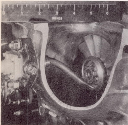
(k) A 15-hole cup-shaped spinner placed behind the impeller retaining nut.
