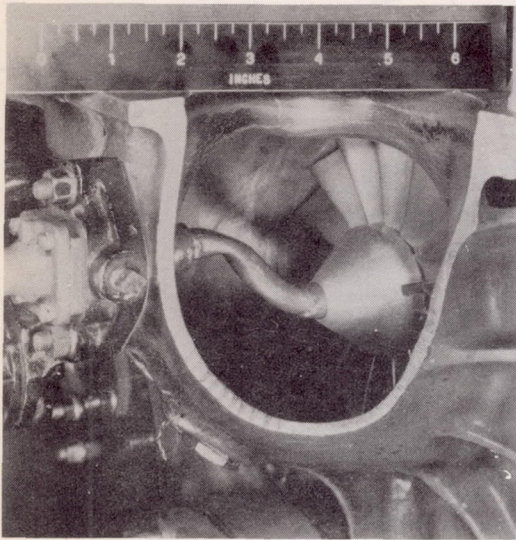
(m) Cone-shaped spinner containing a large inner cavity and fitted upon a revised and threaded impeller nut.
