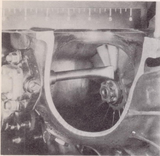
(e) A straight tube extending from the conventional nozzle, flattened on the exit end, and bent approximately 45^\circ .
