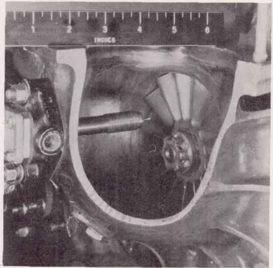
(b) Long nozzle extended toward the impeller from the regular position.
