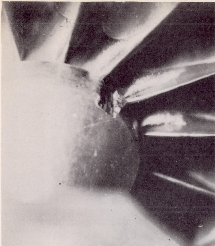
Fuel outlets in retarded position
