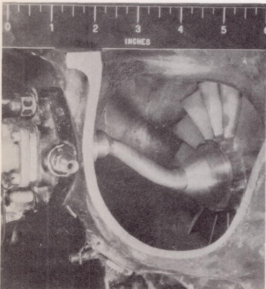
(o) Impeller-inducer injection using a spinner nut.
