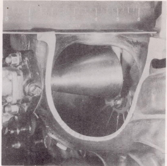
(f) The conventional type nozzle with a new pintle stem incorporating a smaller included angle on the pintle head and using a 360^\circ protective hood.
