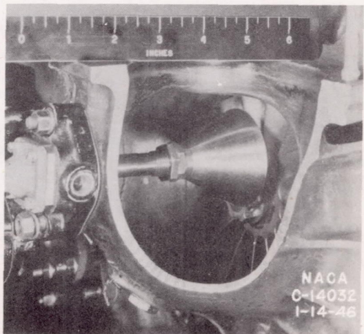
(h) Long nozzle extended to the impeller from the regular position using a 360^\circ hood.
