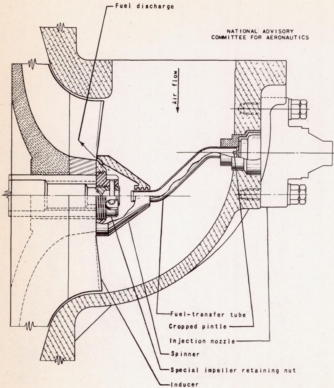
(a) Cross-sectional view of installation.
