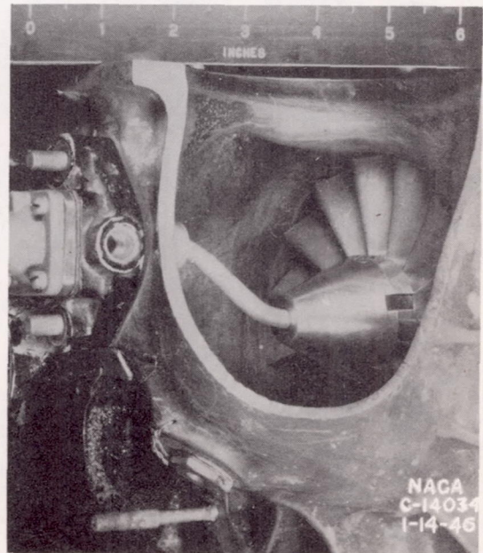
(p) A revision of figure 2(o) incorporating internal threads at the entrance of the spinner.
