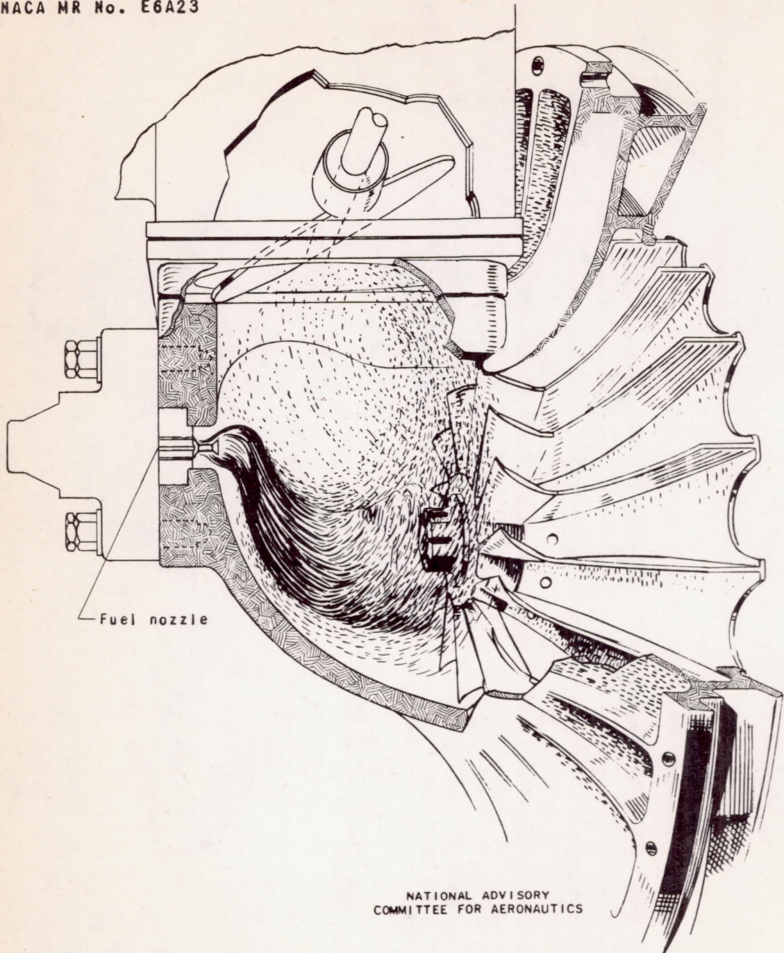
(a) Air flow, 4600 pounds per hour; fuel-air ratio, 0.080. Figure 5. - Fuel-spray pattern of Standard injection nozzle in the supercharger inlet elbow of an aircraft engine.
