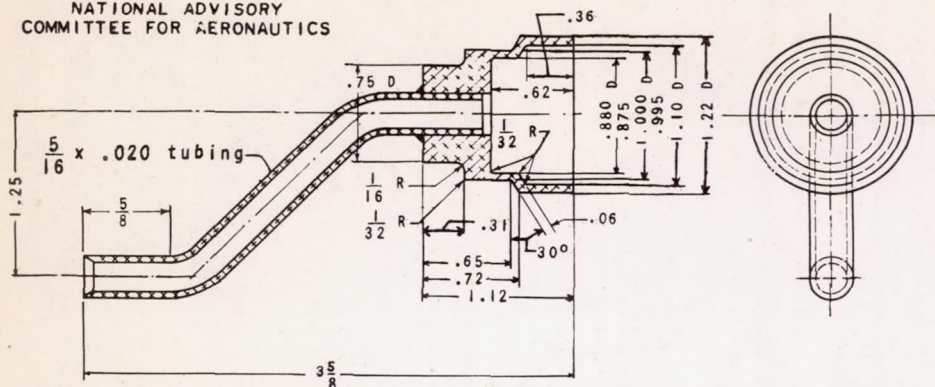
(b) Fuel-transfer tube.
