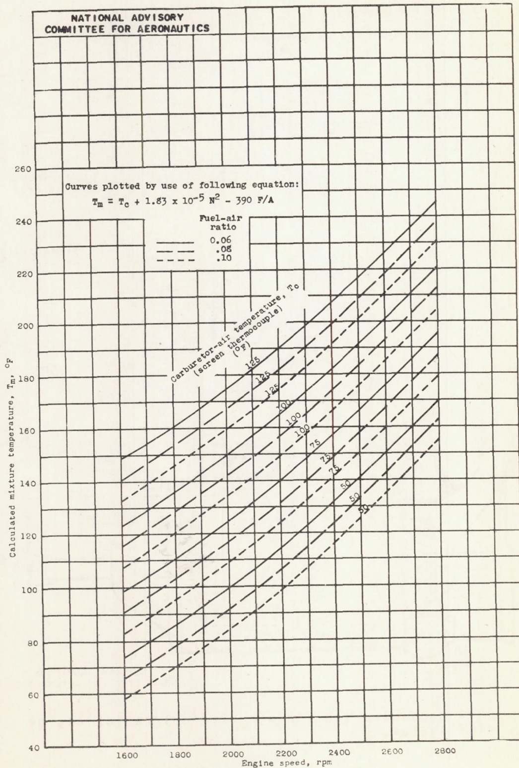
Figure 4. - Calculated relation between engine speed, carburetor-air temperature, fuel-air ratio, and mixture temperature. Impeller diameter, 11.3 inches.
