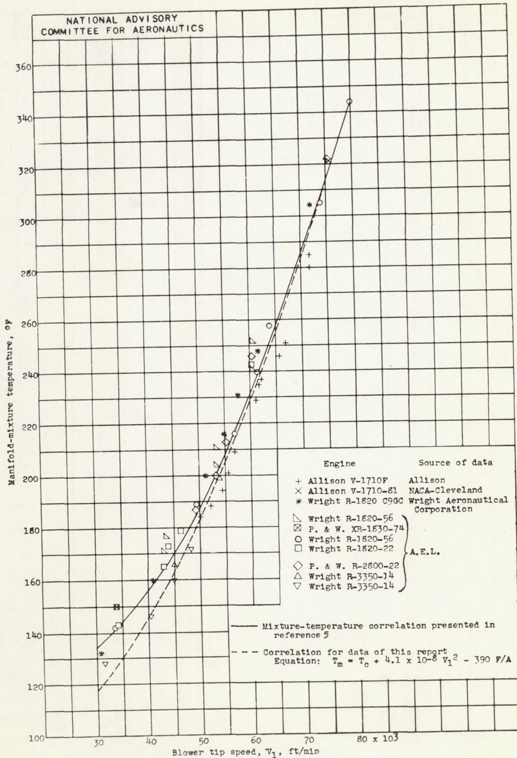
Figure 7. - Correlation of mixture-temperature data from outside sources. Carburetor-air temperature, 100^\circ \text{F} ; fuel-air ratio, 0.05. Plot obtained from plate 4 of reference 5.
