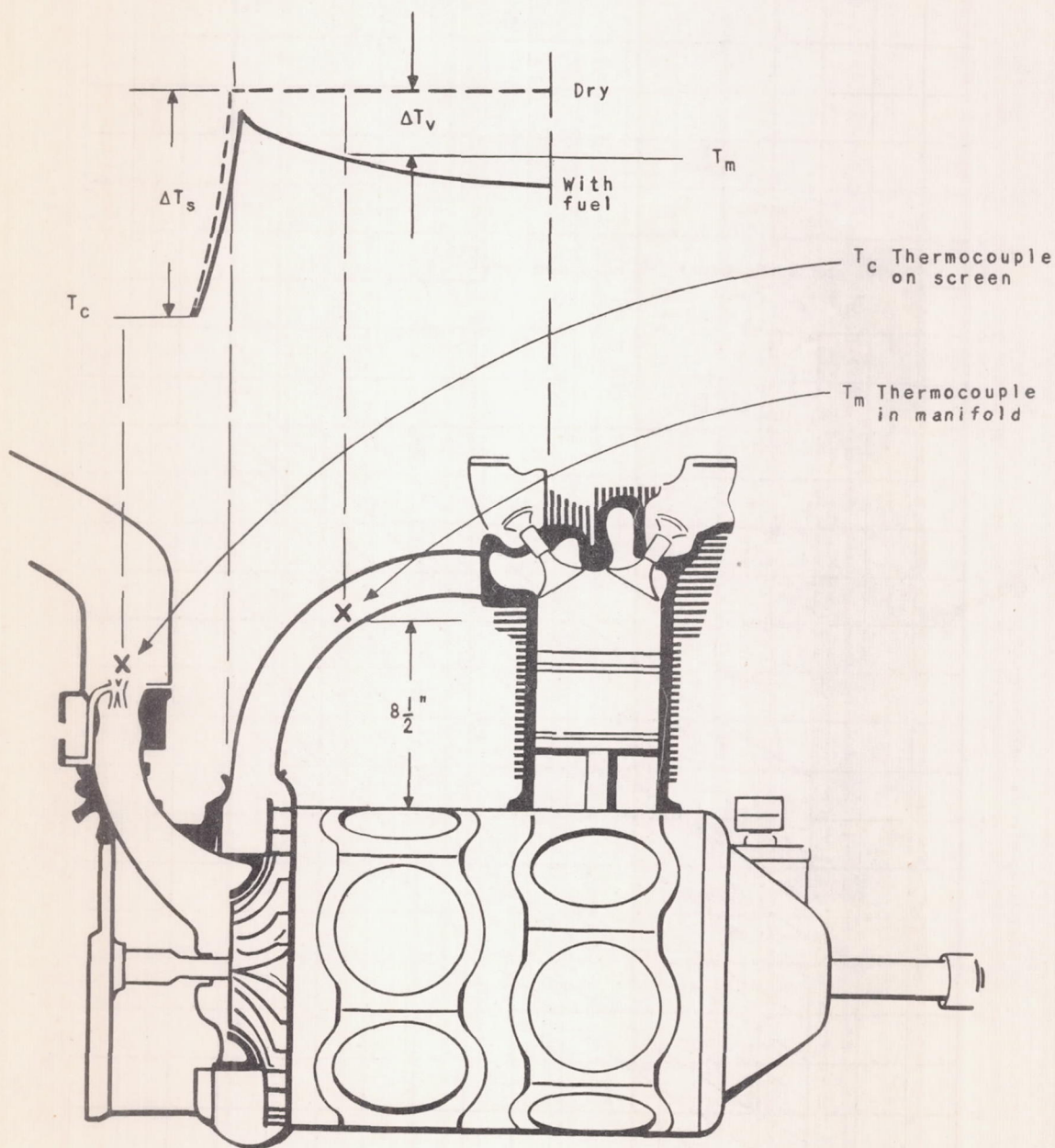
Figure 3. - Schematic section of a typical radial-engine induction system.
