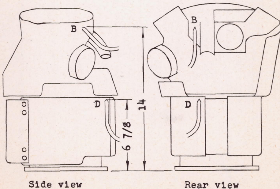
Rear-row cylinder
