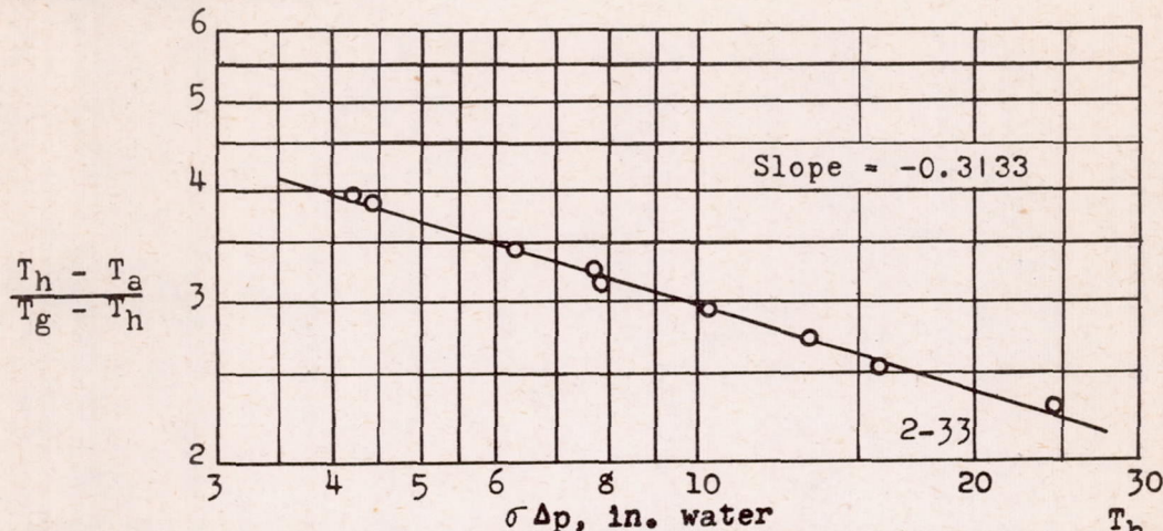
Figure 5. - Variation of cooling-temperature differential \frac{T_h - T_a}{T_g - T_h}
