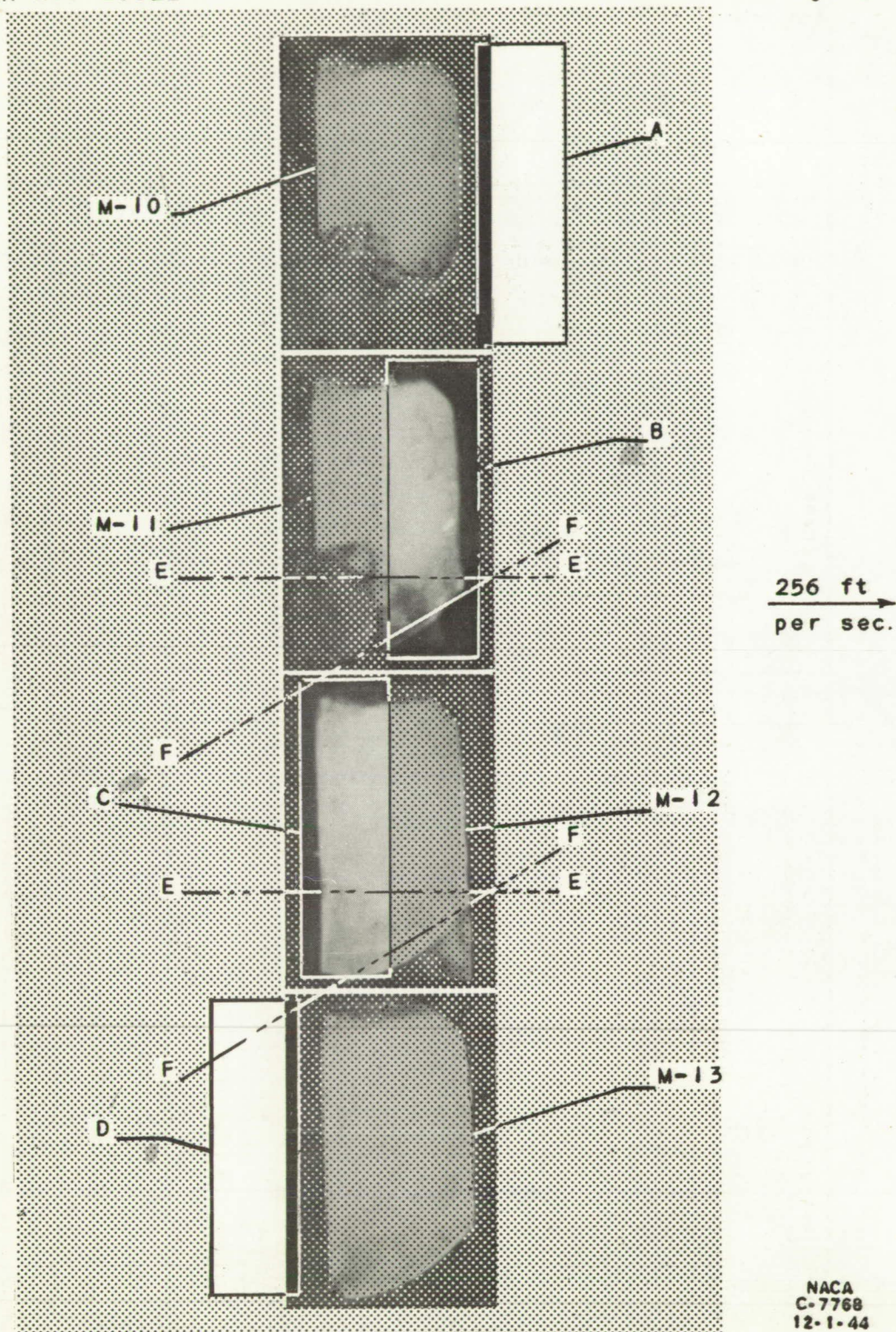
Figure 3. - Equivalent manner of exposure of frames in high-speed photographs. A, B, C, D, rectangular slots in an opaque screen; M-10, M-11, M-12, M-13, successive frames from knocking portion of figure 2.
