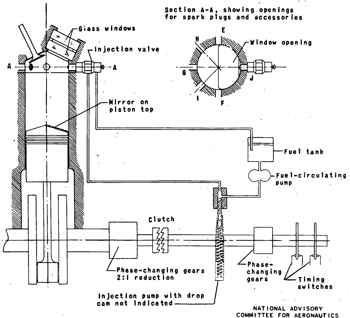
Figure 1. - Diagrammatic sketch of NACA combustion apparatus.
