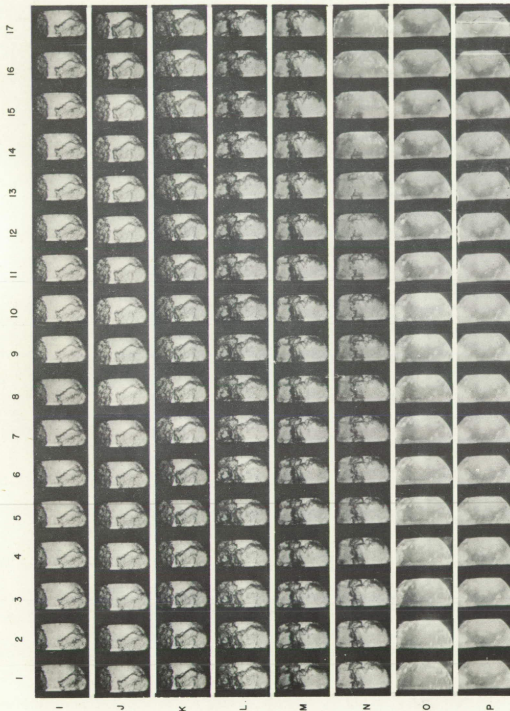
Figure 6. - (Fig. 8 of reference 16.) High-speed motion pictures of knocking combustion cycle in an engine cylinder showing detonation apparently not preceded by auto-ignition with shell-burst effect of bright luminous spots. Fuel, 50 percent S-1 and 50 percent M-2; spark plug at top, hot spot at bottom. (See fig. 7 for enlargement of knocking portion.)
