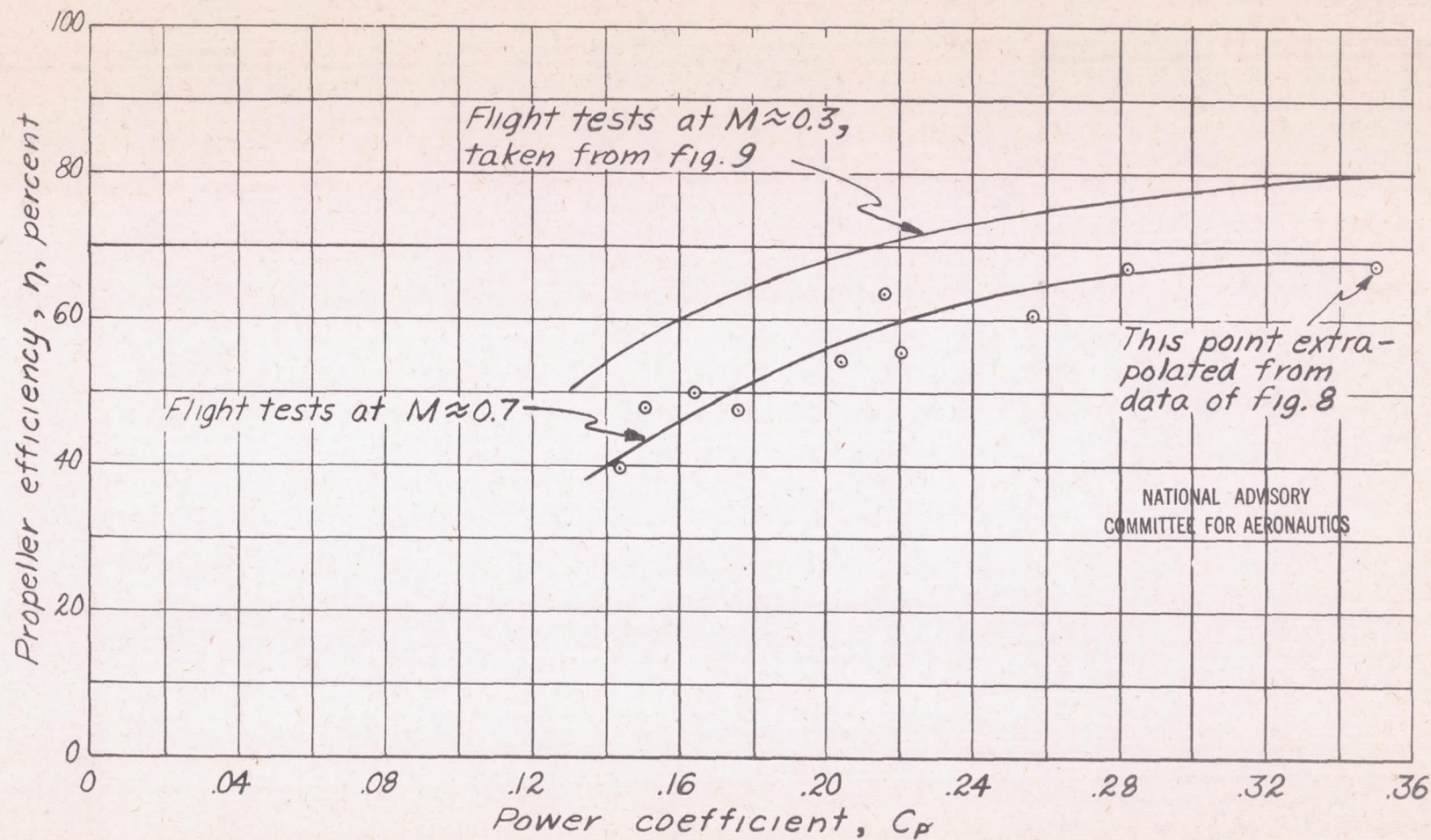
Figure 13.- Effect of blade loading on propeller efficiency at high speed. J \approx 2.70 .
