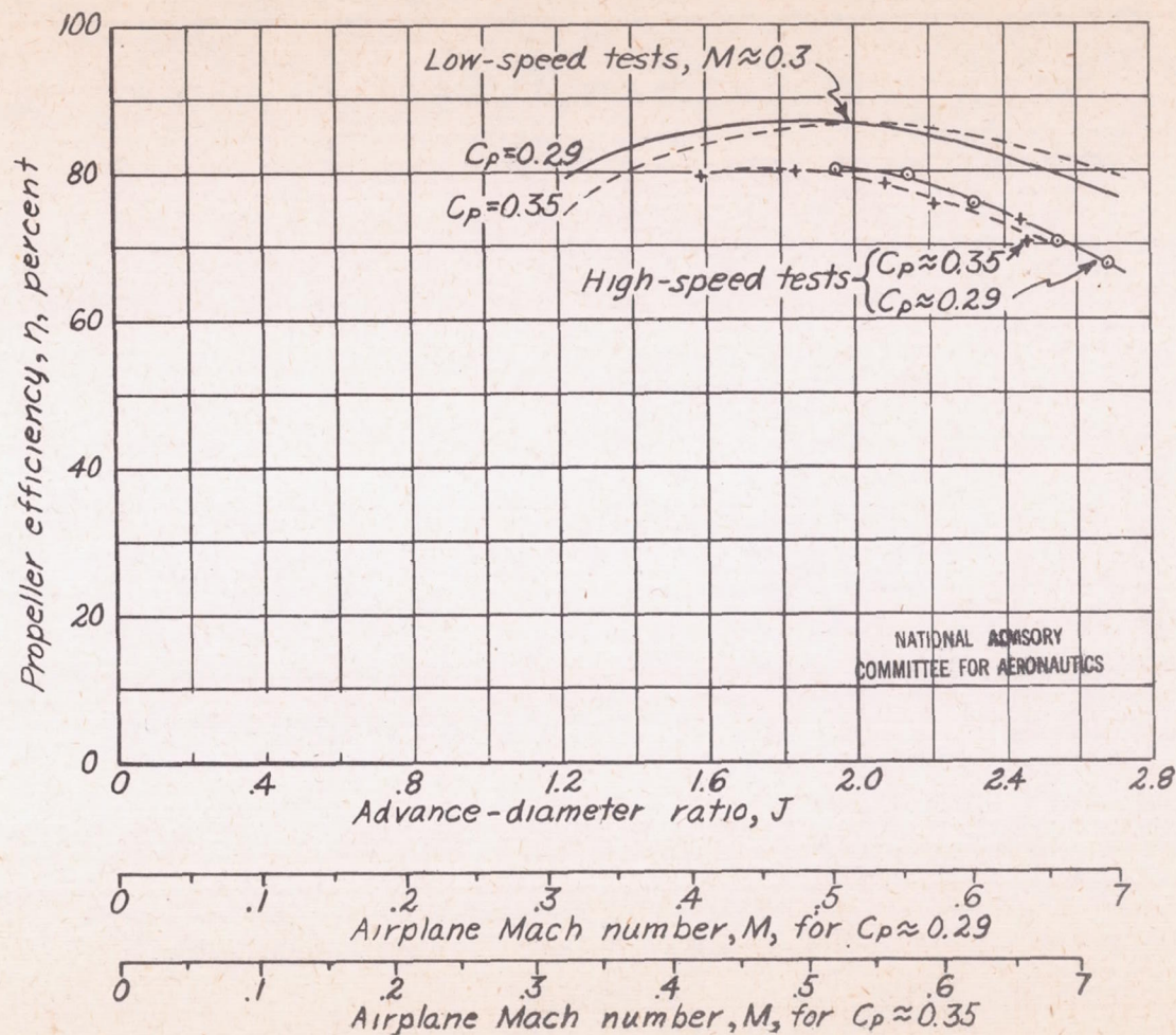
Figure 8.- Effect of compressibility on propeller efficiency for constant power coefficient. C_p \approx 0.29 and C_p \approx 0.35 .
