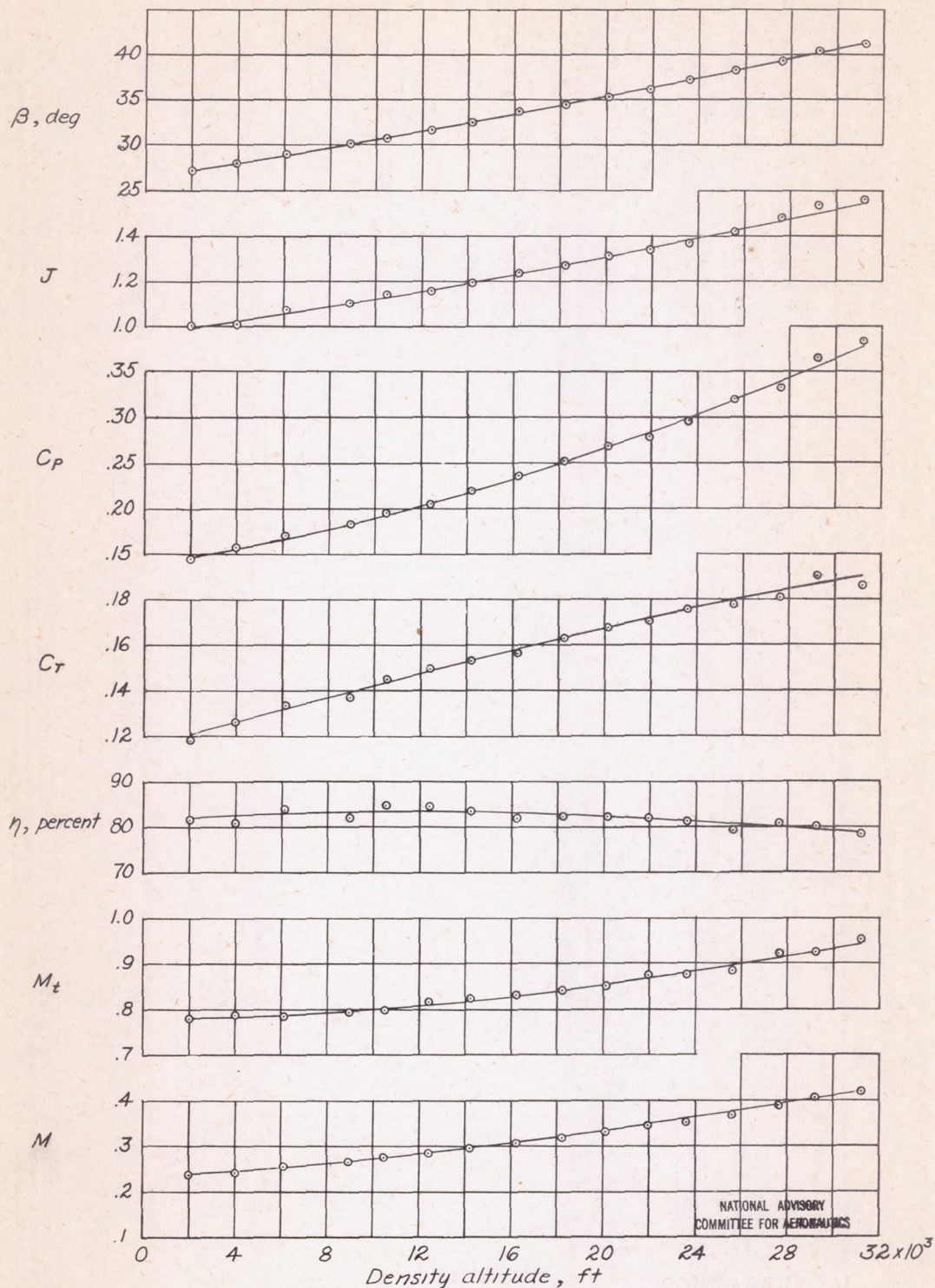
Figure 6.- Normal-power climb at an indicated airspeed of 165 miles per hour. Curtiss No. 714-1C2-12 four-blade propeller on Republic P-47C airplane.
