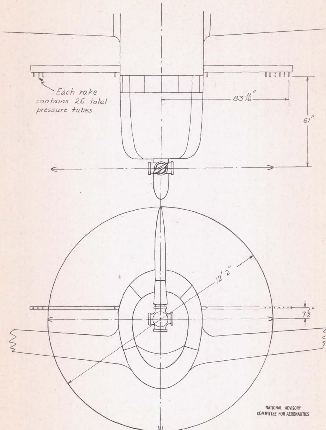
Figure 2.- Location of propeller and survey rakes on a Republic P-47C airplane.
