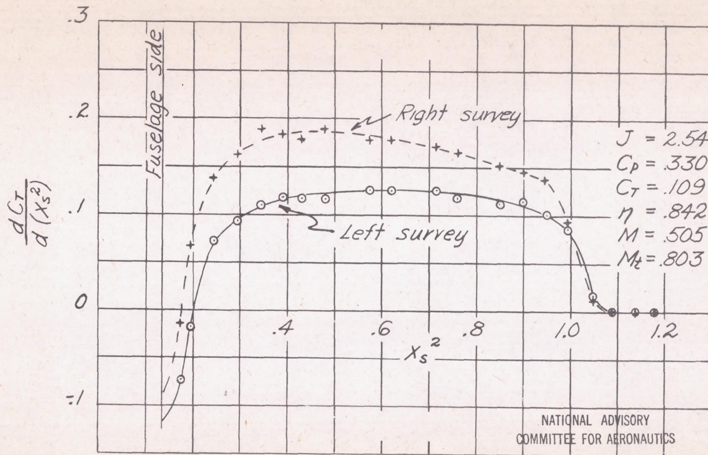
Figure 12.- Thrust-grading curve for run 12-1.
