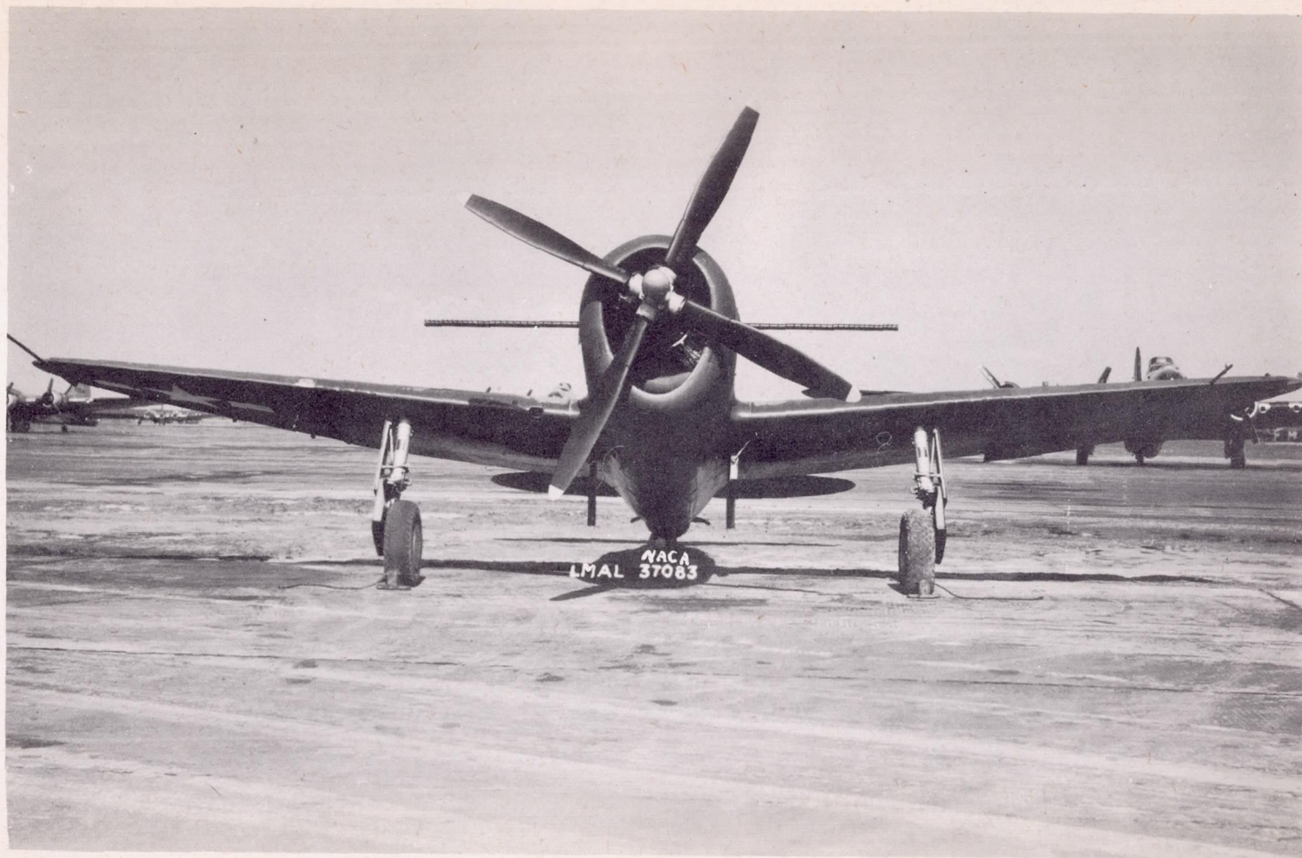
Figure 3.- Republic P-47C airplane equipped with a Curtiss No. 714-1C2-12 four-blade propeller and survey rakes.
