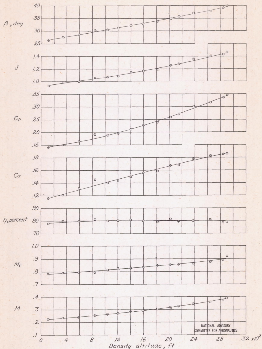
Figure 5.- Normal-power climb at an indicated airspeed of 160 miles per hour. Curtiss No. 714-1C2-12 four-blade propeller on Republic P-47C airplane.
