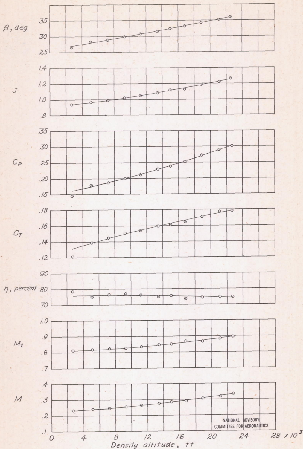
Figure 4.- Military-power climb at an indicated airspeed of 165 miles per hour. Curtiss No. 714-1C2-12 four-blade propeller on Republic P-47C airplane.
