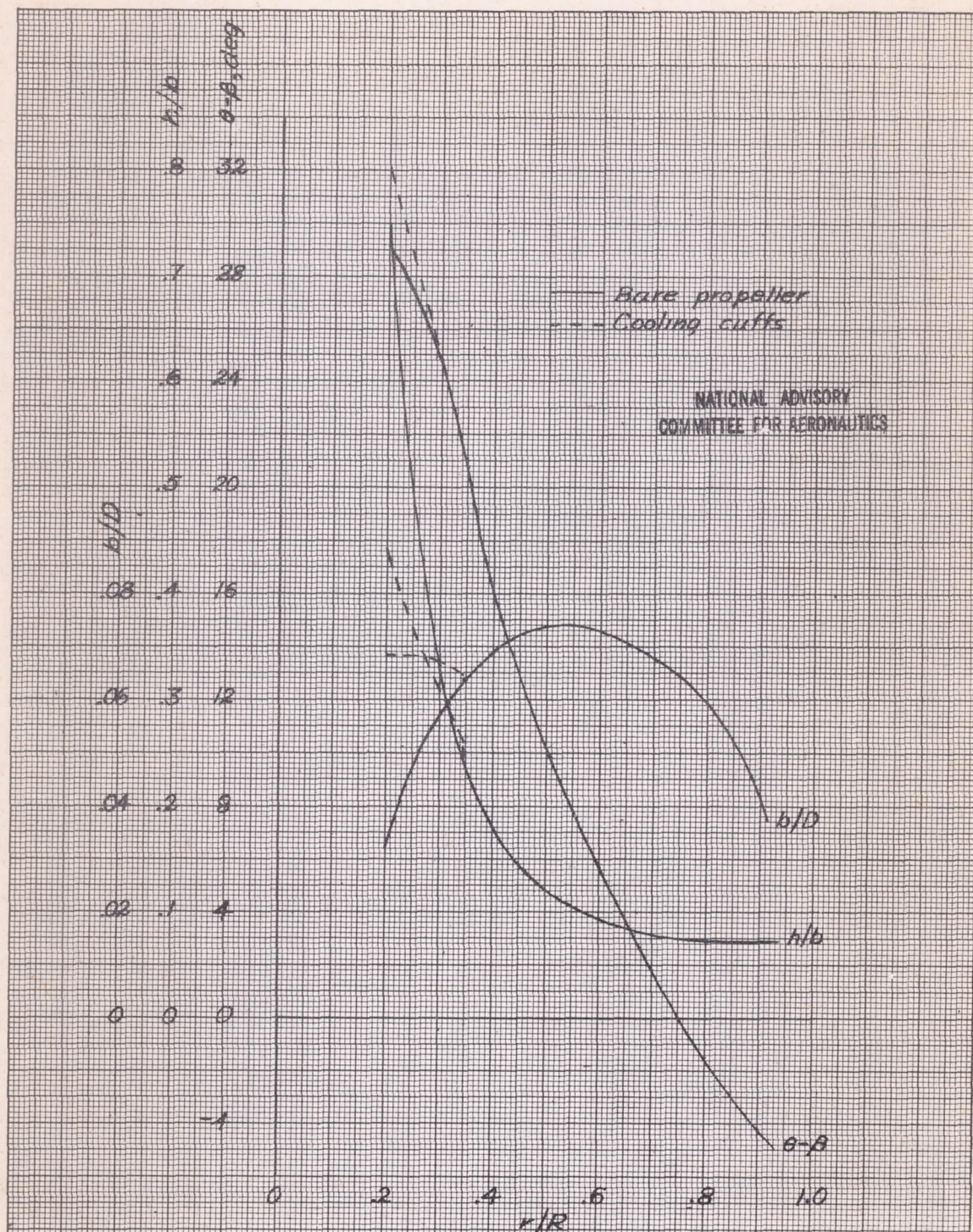
Figure 1.- Blade-form curves for Curtiss No. 714-1C2-12 four-blade propeller.
