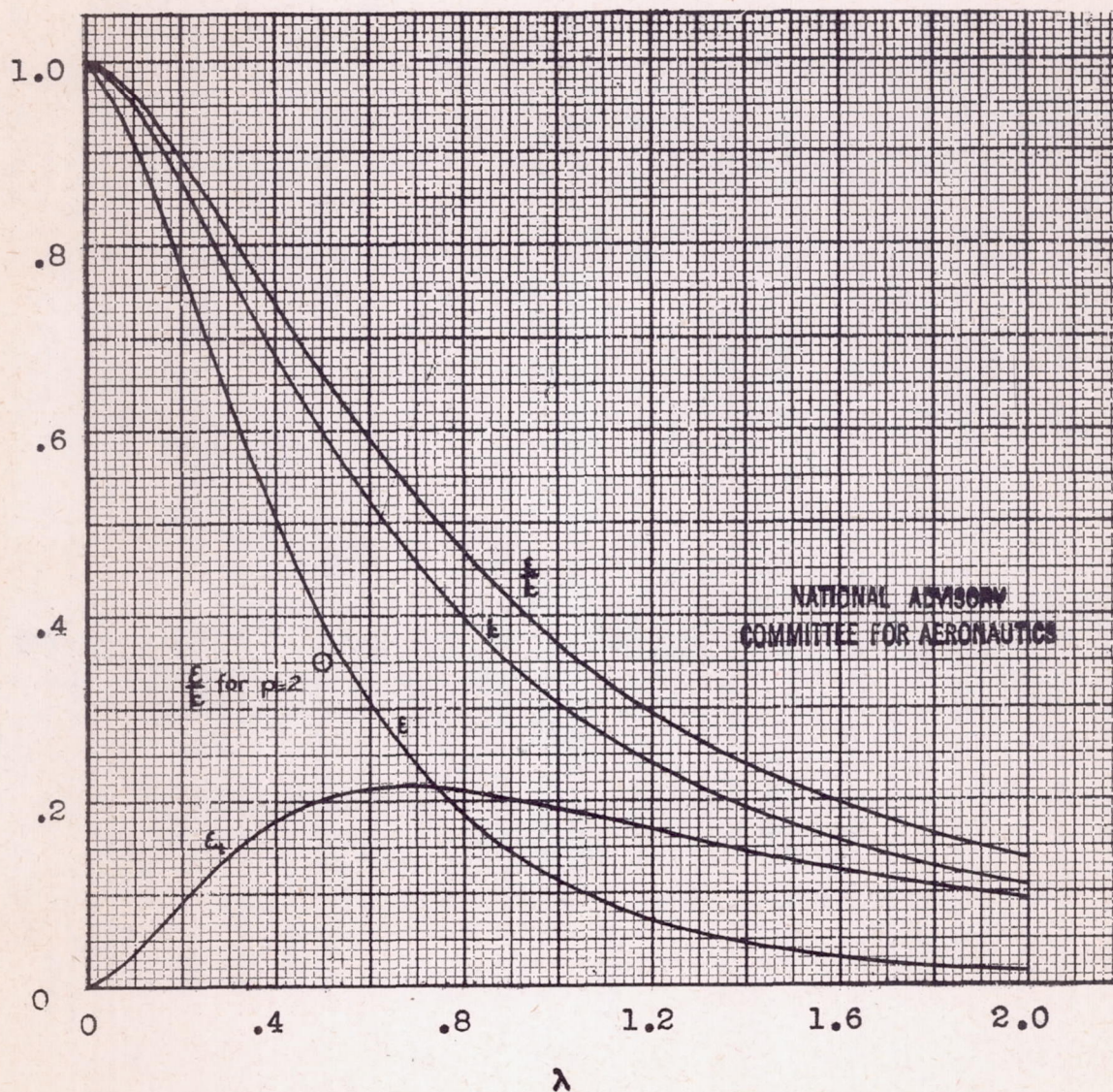
Figure 4.- Loss functions for an infinite number of blades.
