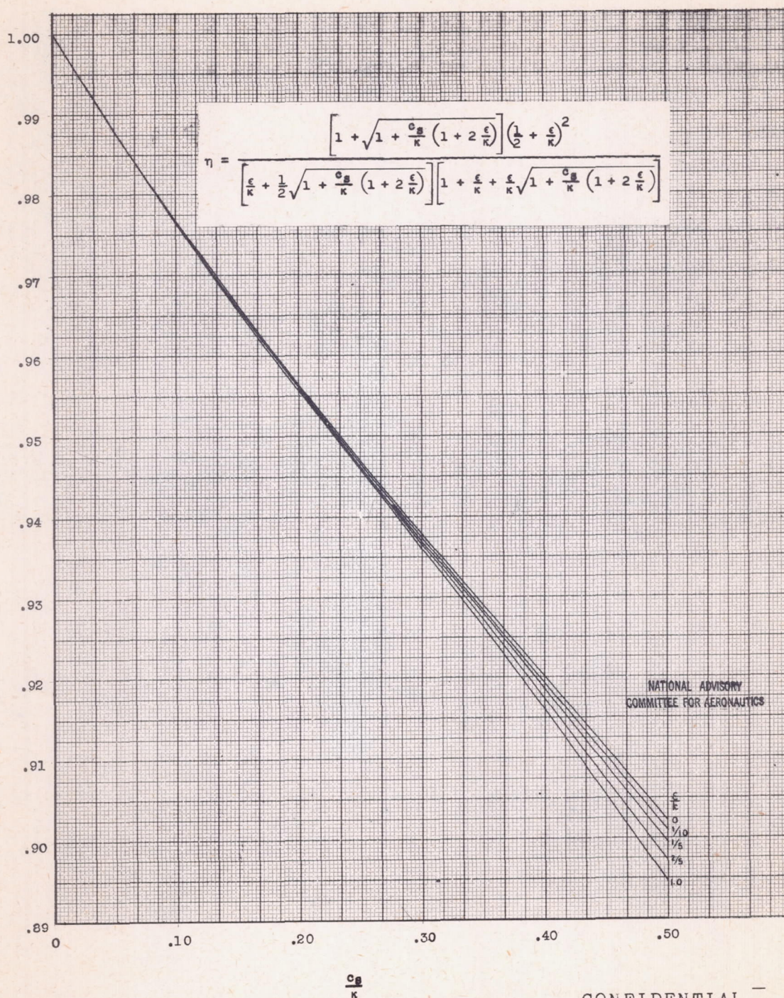
Figure 2.- Propeller efficiency.
