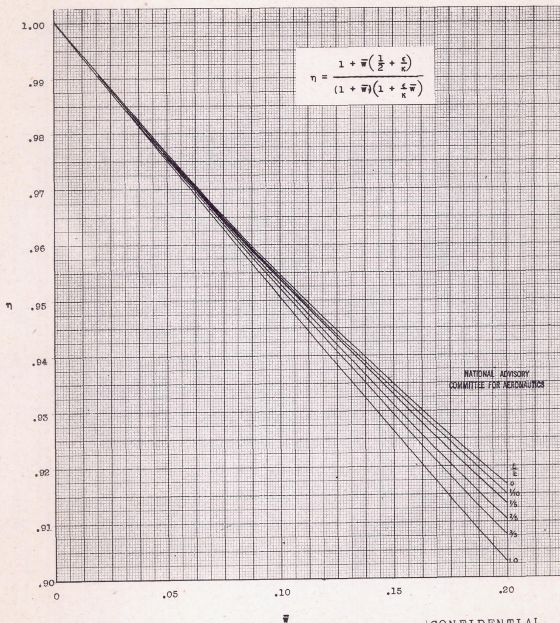
Figure 1.- Propeller efficiency.
