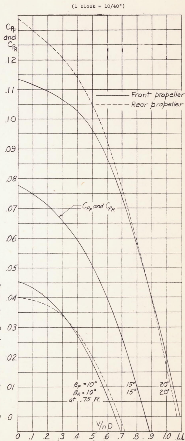
Figure 14.- Individual power-coefficient curves for eight-blade dual-rotating propeller.
