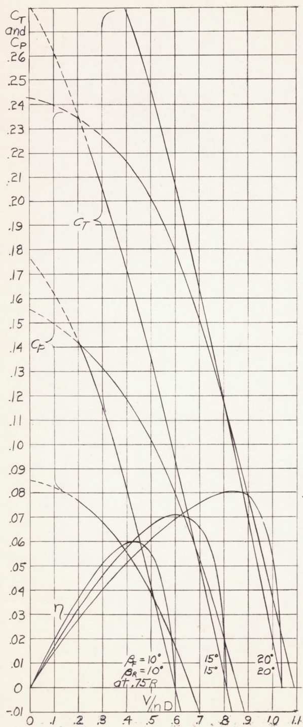
Figure 13.- Propeller characteristics at low blade angles. Eight-blade dual-rotating propeller.
