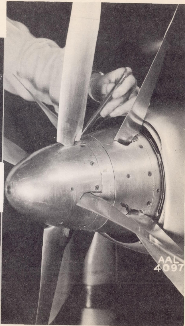
Figure 4.- Details of dual spinner.
