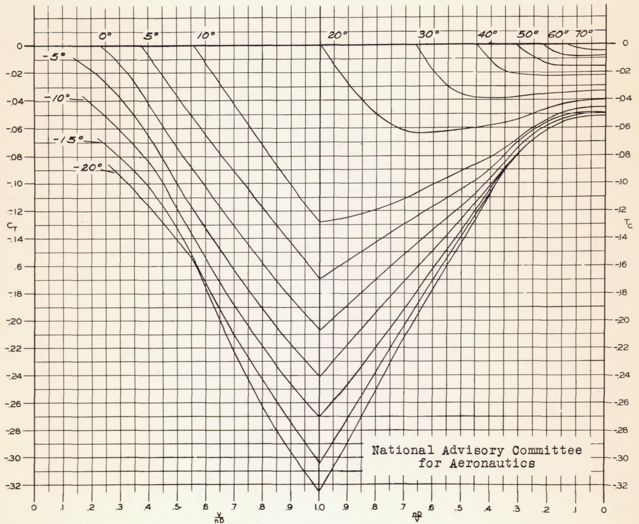
Figure 11.- Negative thrust coefficients at constant blade angles for the four-blade, single propeller.
