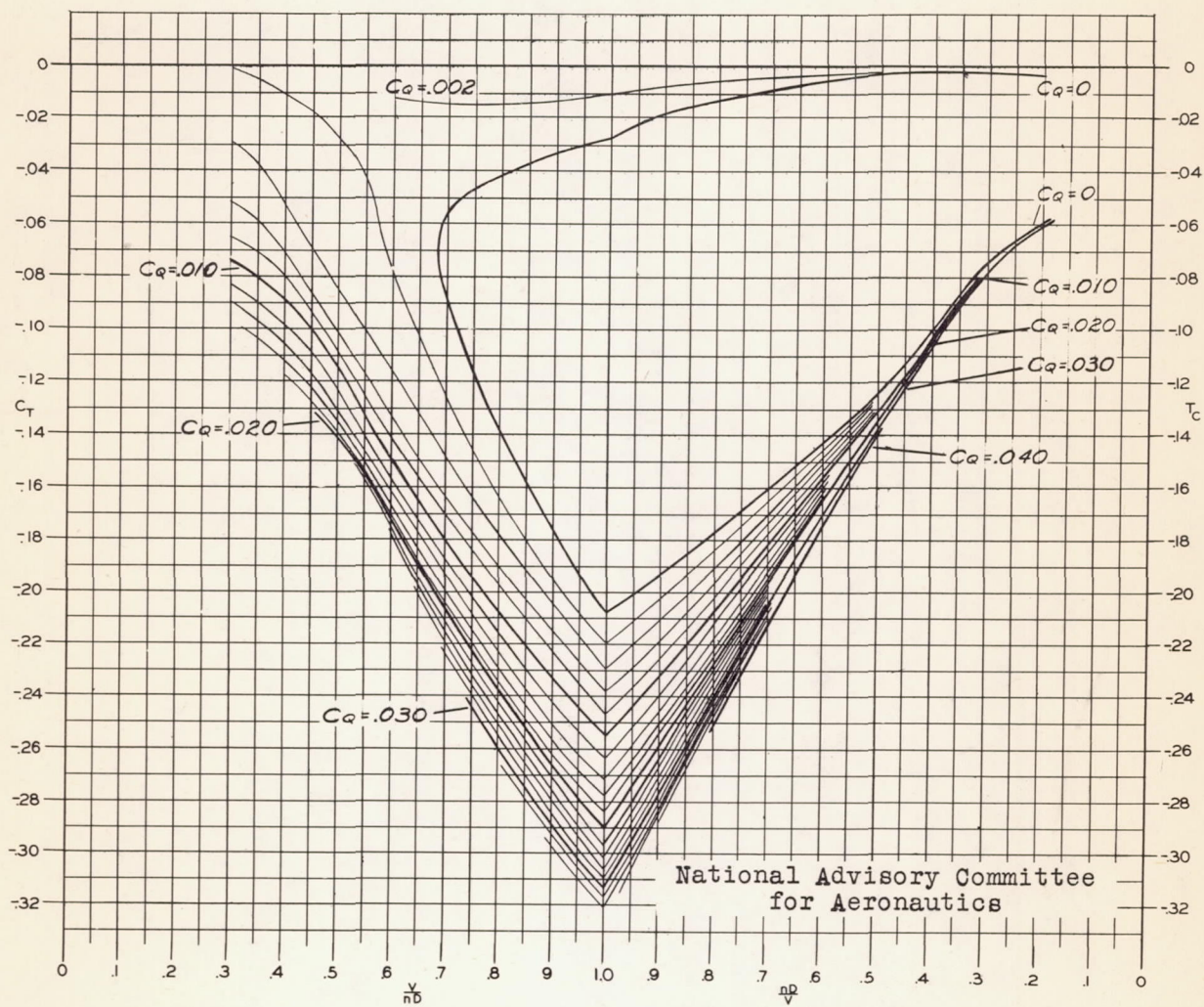
Figure 7.- Negative thrust coefficients at constant torque coefficients for the four-blade, single propeller.
