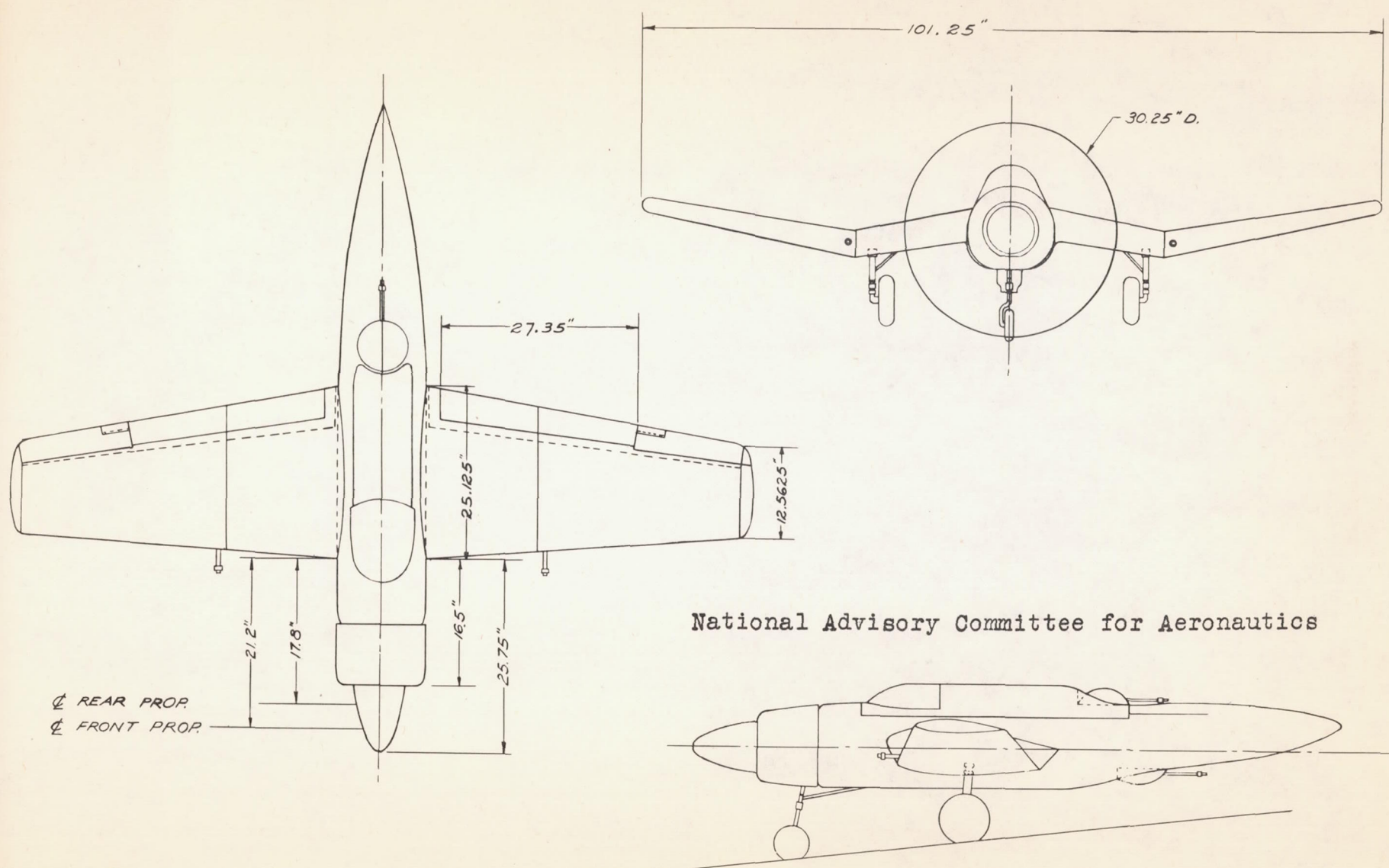
Figure 5.- Three view sketch of the model.
