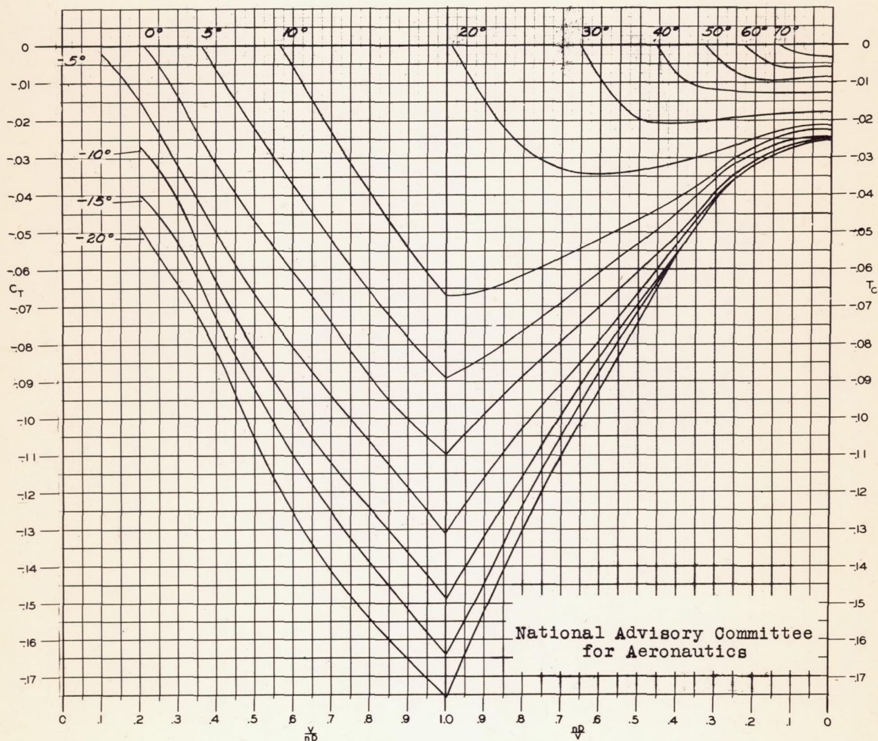
Figure 10.- Negative thrust coefficients at constant blade angles for the two-blade, single propeller.
