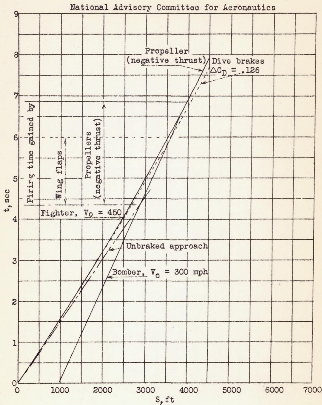
Figure 19.- The variation of time with distance for a fighter overtaking a bomber.
