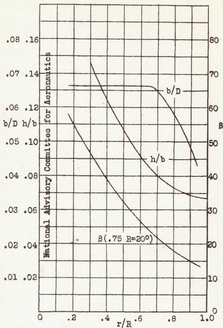
Figure 1.- Blade-form curves for the Hamilton Standard conventional propellers, 6457A-6. D, diameter; R, radius to tip; r, station radius; b, section chord; h, section thickness; \beta , blade angle.
