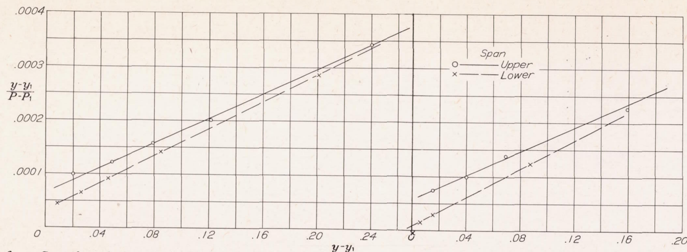
Figure 8.- Graph of load-deflection data. Initial deflection at center support, 0.749 inch.
