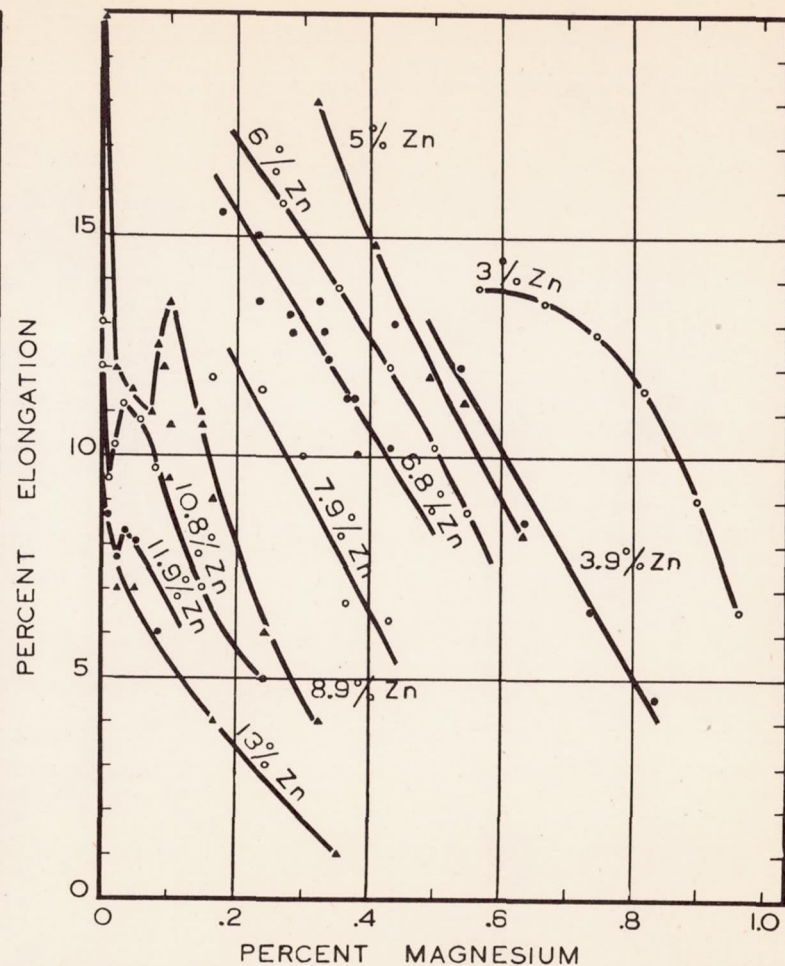
Figure 1b.- The effect of magnesium content on the percent elongation in 2 inches of gage length of alloys containing approximately 0.4% copper, 0.15% iron, 0.08% silicon, 0.25% chromium, and various amounts of zinc. All alloys as cast and aged 30 days at 85°F.
