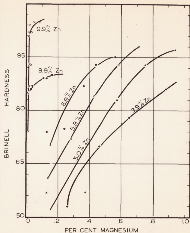
Figure 3d.- The effect of magnesium content on the Brinell hardness of alloys containing approximately 1.75% copper, 0.15% iron, 0.08% silicon, 0.25% chromium, and various amounts of zinc. All alloys cast and aged 30 days at 85°F.
