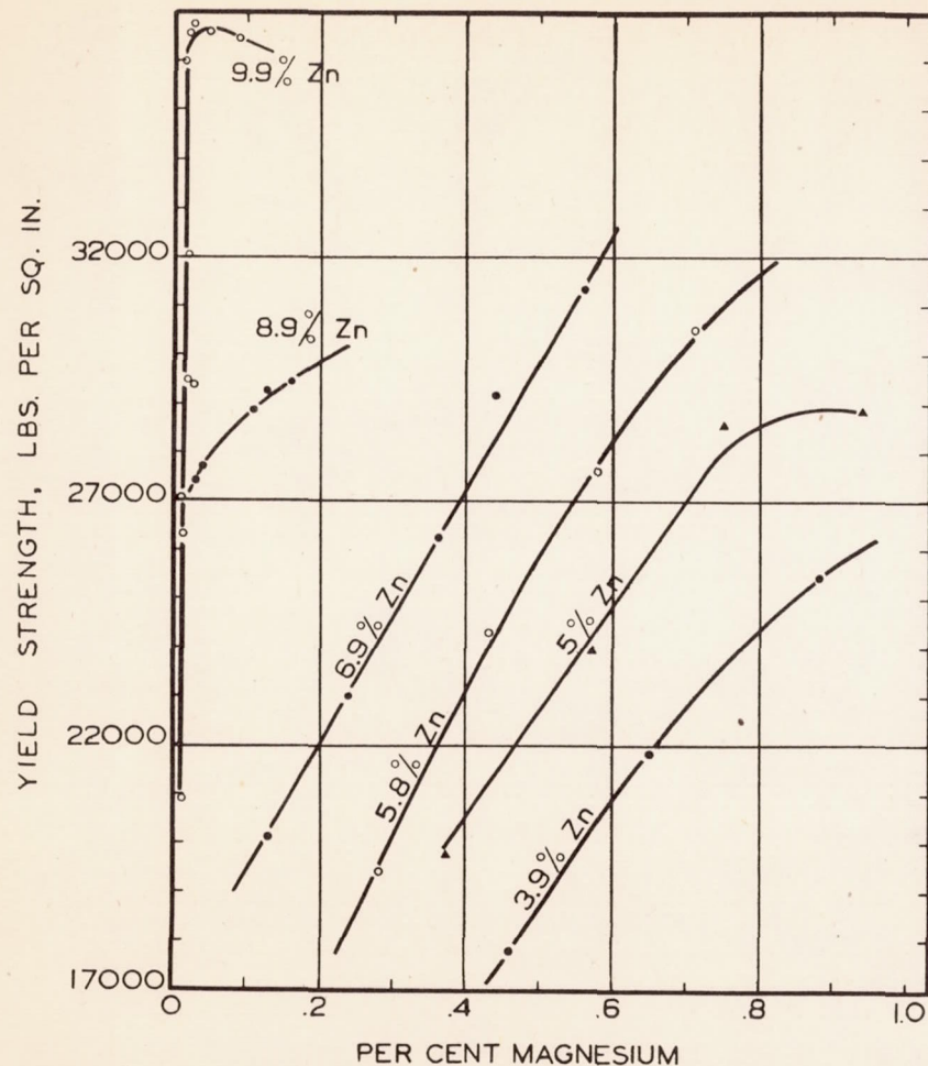
Figure 3c.- The effect of magnesium content on the yield strength of alloys containing approximately 1.75% copper, 0.15% iron, 0.08% silicon, 0.25% chromium, and various amounts of zinc. All alloys as cast and aged 30 days at 85°F.
