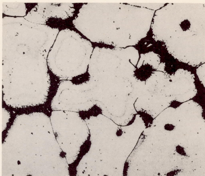
FIG. 8a Photomicrograph at X100 of an alloy containing 1.05% Cu, 0.15% Fe, 0.13% Si, 7.02% Zn, 0.14% Ti, 0.29% Mg and 0.30% Cr. Keller's etch.
