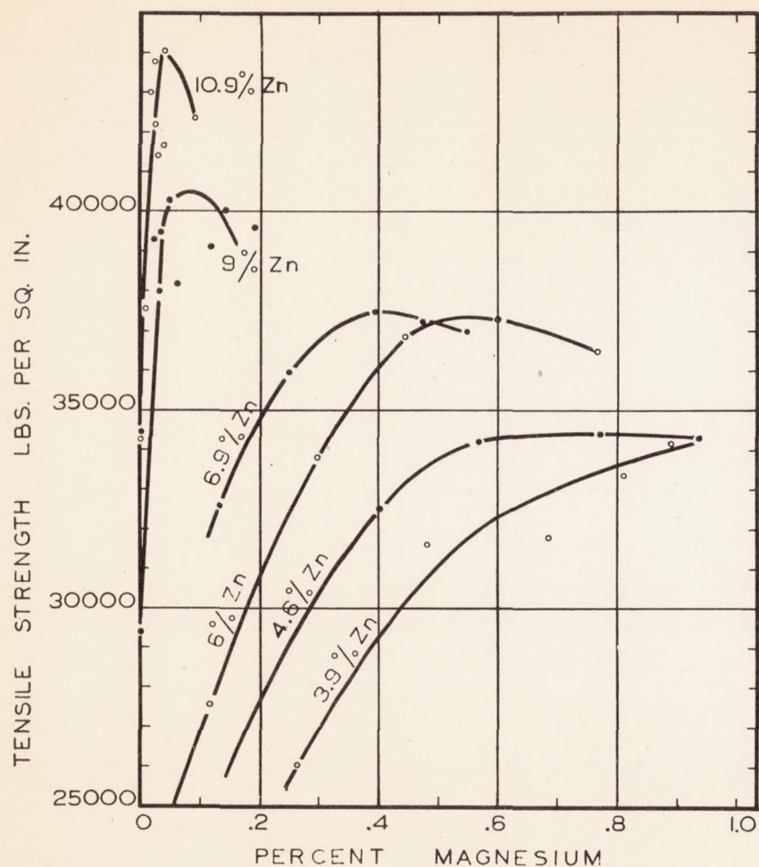
Figure 2a.- The effect of magnesium content on the tensile strength of alloys containing approximately 1.0% copper, 0.15% iron, 0.08% silicon, 0.25% chromium, and various amounts of zinc. All alloys as cast and aged 30 days at 85°F.
