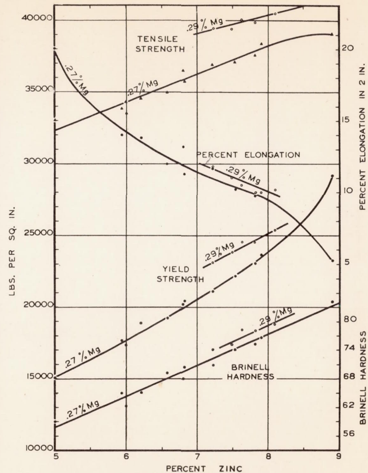
Figure 5.- The effect of zinc content on the tensile properties and hardness of cast test bars of aluminum alloys containing approximately 0.35% copper, 0.18% iron, 0.08% silicon, 0.13% titanium, 0.28% chromium, and 0.27% and 0.29% magnesium. All alloys aged 30 days at 85°F.
