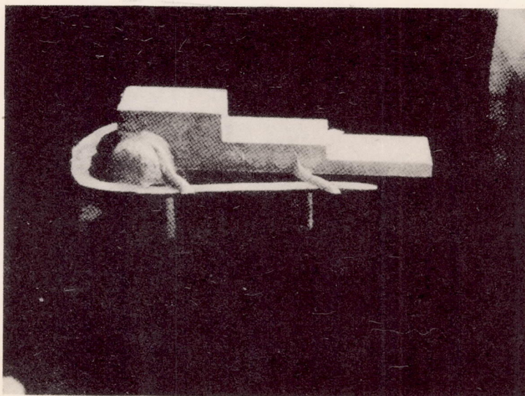
FIG. 10. The Step Casting with Gate and Risers Attached.
