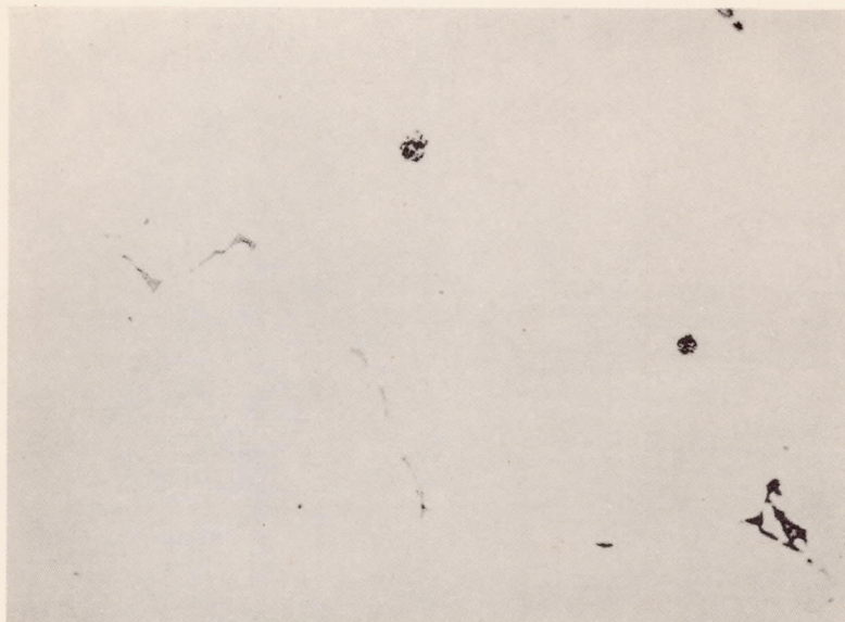
FIG. 8c Photomicrograph at X500 showing the elongated irregular gray constituent \alpha Al-Fe-Si. The rounded light gray constituent is CuAl 2 rosettes. Unetched. Composition similar to that illustrated by Fig. 8b.
