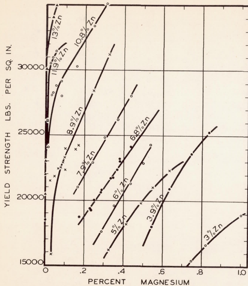
Figure 1c.- The effect of magnesium content on the yield strength of alloys containing approximately 0.4% copper, 0.15% iron, 0.08% silicon, 0.25% chromium, and various amounts of zinc. All alloys as cast and aged 30 days at 85°F.
