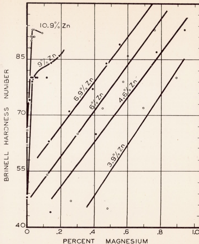
Figure 2d.- The effect of magnesium content on the Brinell hardness of alloys containing approximately 1.0% copper, 0.15% iron, 0.08% silicon, 0.25% chromium, and various amounts of zinc. All alloys as cast and aged 30 days at 85°F.
