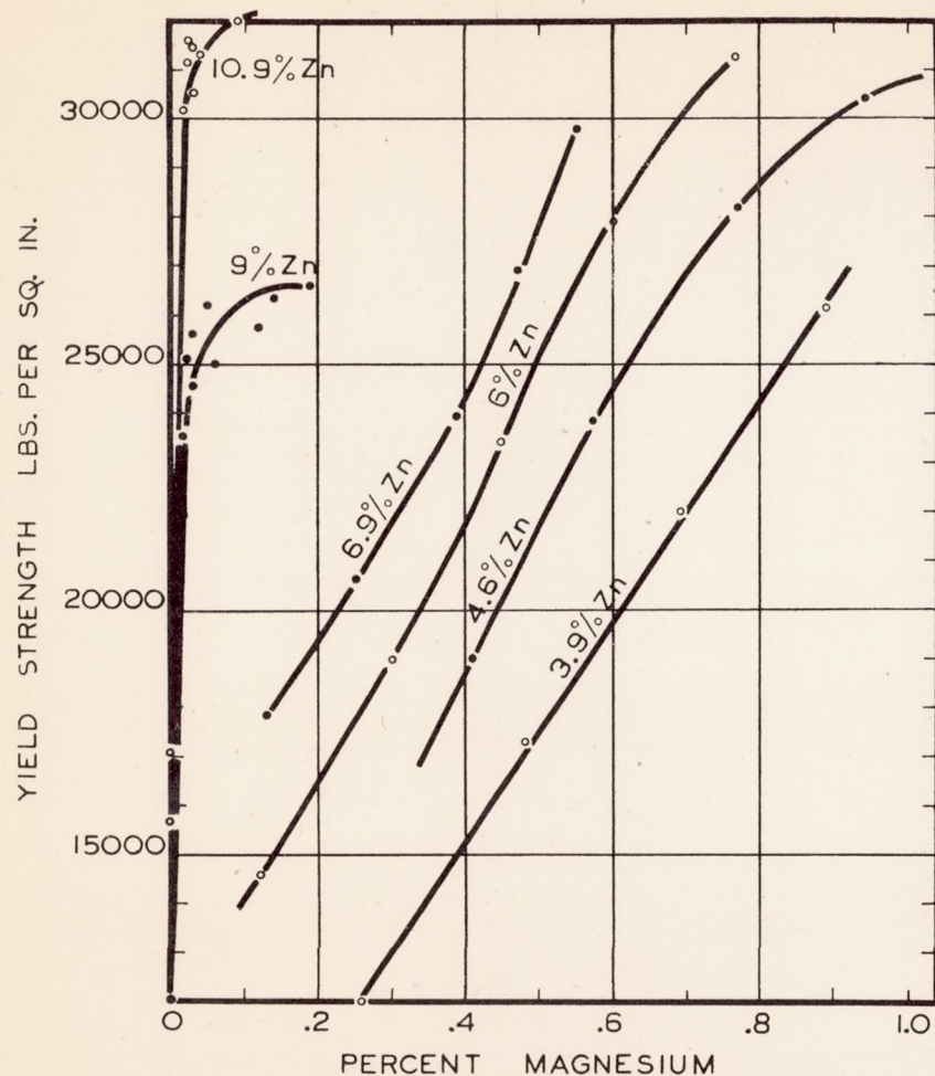
Figure 2c.- The effect of magnesium content on the yield strength of alloys containing approximately 1.0% copper, 0.15% iron, 0.08% silicon, 0.25% chromium, and various amounts of zinc. All alloys as cast and aged 30 days at 85°F.
