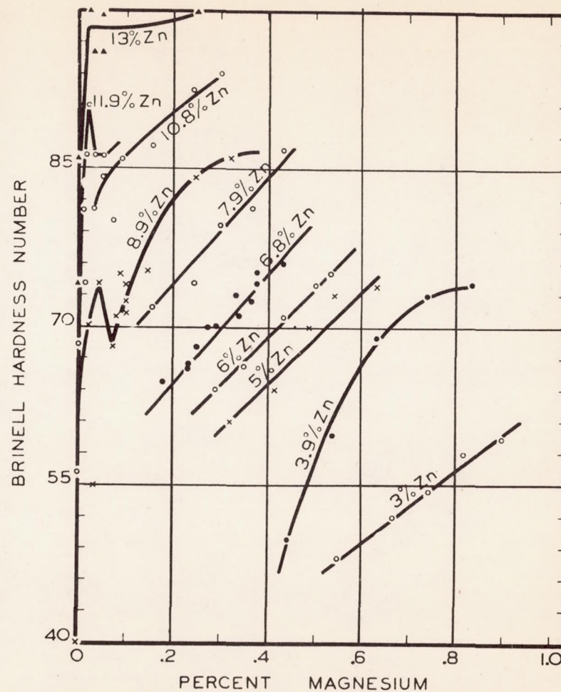
Figure 1d.- The effect of magnesium content on the Brinell hardness of alloys containing approximately 0.4% copper, 0.15% iron, 0.08% silicon, 0.25% chromium, and various amounts of zinc. All alloys as cast and aged 30 days at 85°F.
