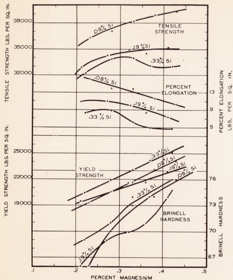
Figure 6.- The effect of magnesium content on the tensile properties and hardness of cast test bars of aluminum alloys containing approximately 0.38% copper, 0.15% iron, 6.6% zinc, 0.13% titanium, 0.22% chromium, and 0.08, 0.19, and 0.33% silicon. All alloys aged 30 days at 85°F.
