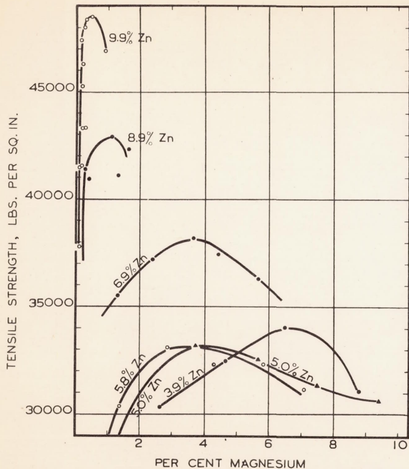
Figure 3a.- The effect of magnesium content on the tensile strength of alloys containing approximately 1.75% copper, 0.15% iron, 0.08% silicon, 0.25% chromium, and various amounts of zinc. All alloys as cast and aged 30 days at 85°F.
