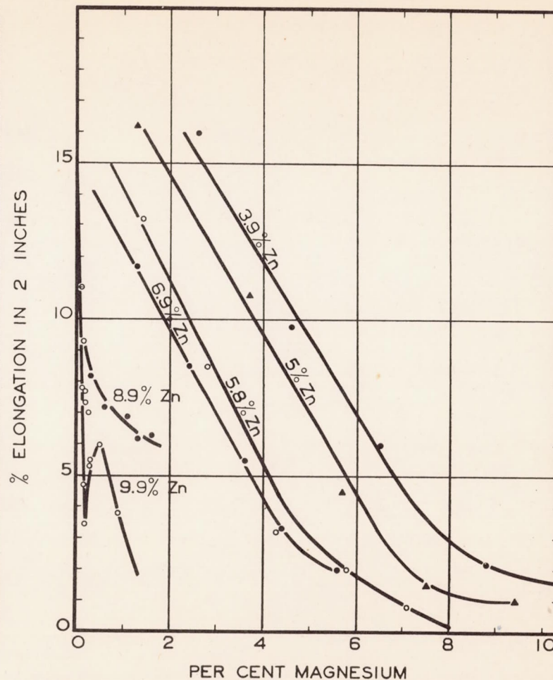
Figure 3b.- The effect of magnesium content on the percent elongation in 2 inches of gage length of alloys containing approximately 1.75% copper, 0.15% iron, 0.08% silicon, 0.25% chromium, and various amounts of zinc. All alloys as cast and aged 30 days at 85°F.
