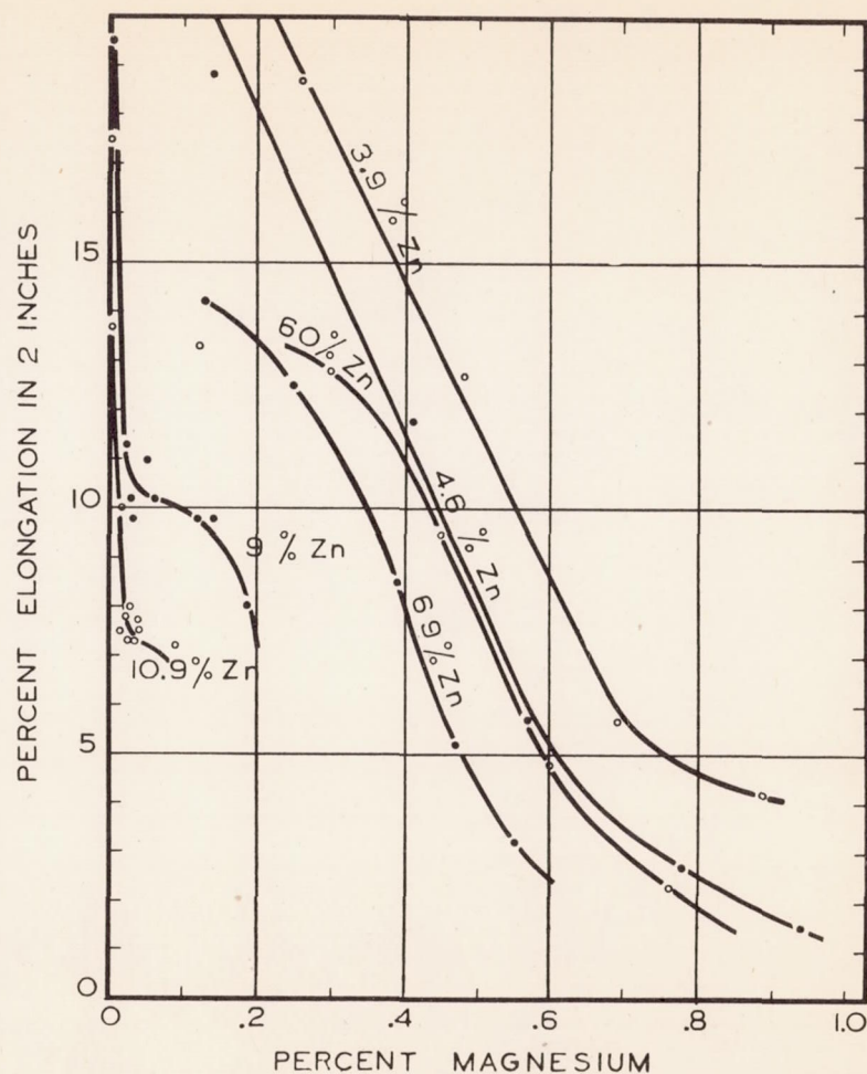
Figure 2b.- The effect of magnesium content on the percent elongation in 2 inches of gage length of alloys containing approximately 1.0% copper, 0.15% iron, 0.08% silicon, 0.25% chromium, and various amounts of zinc. All alloys as cast and aged 30 days at 85°F.
