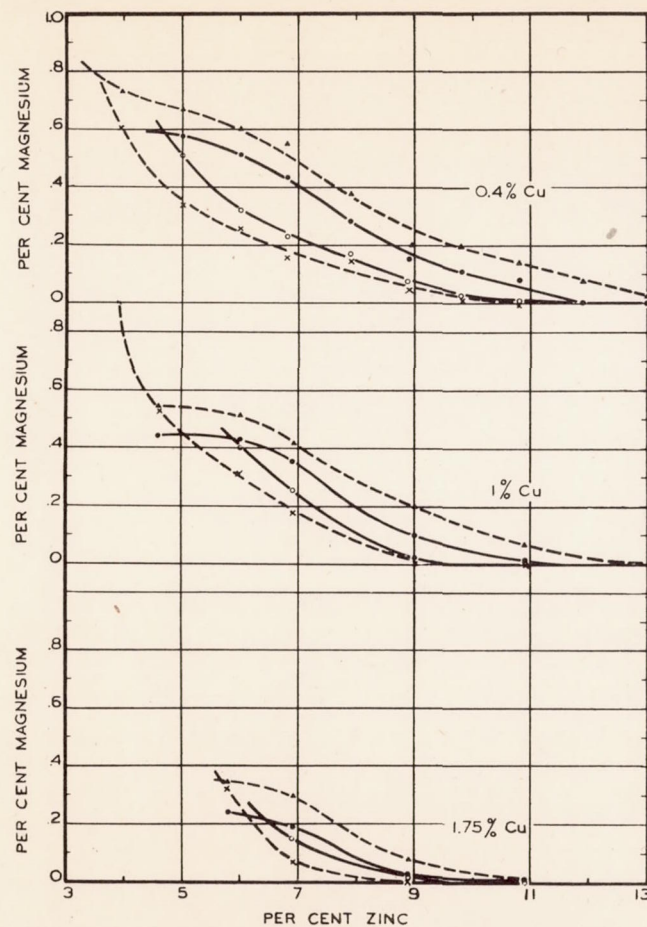
Figure 4.- The inside area represents the range in magnesium and zinc contents of cast test bars which will generally attain, after aging 30 days at 85°F, a minimum tensile strength and elongation of 36,000 pounds per square inch. and 10 percent respectively. The composition represented by the outside dashed lines will generally produce a minimum of 34,000 pounds per square inch and 7 percent elongation. These data are for aluminum alloys containing 0.15% iron, 0.08% silicon, 0.15% titanium, and 0.25% chromium and the copper, magnesium and zinc contents indicated on the chart.
