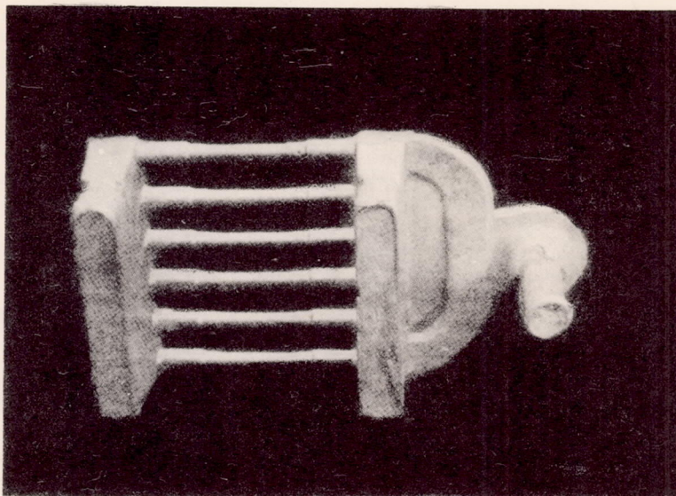
FIG. 9 The Six Bar Casting with Gate and Risers Attached.
