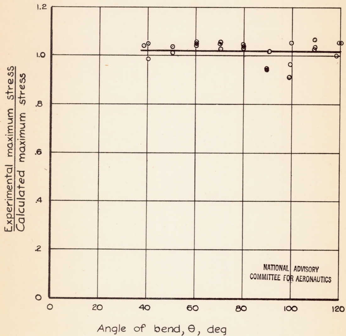
Figure 6. — Ratio of experimental to calculated maximum stress for angles of bend.
