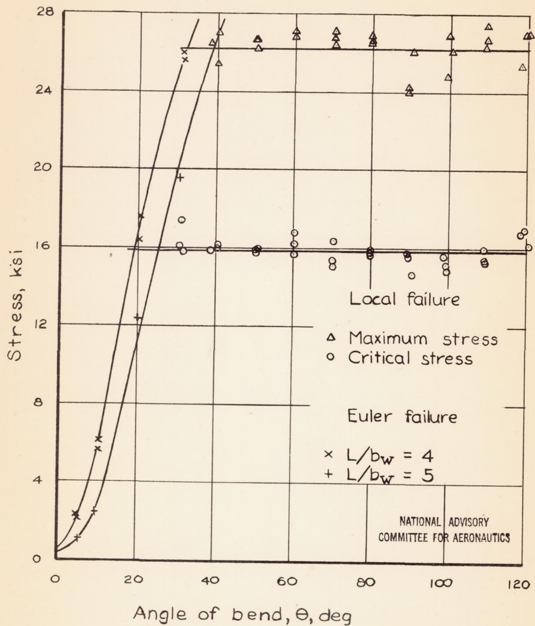
Figure 4.— Effect of angle of bend on the critical and maximum stress of 24 S-T aluminum-alloy columns of Z-section.
