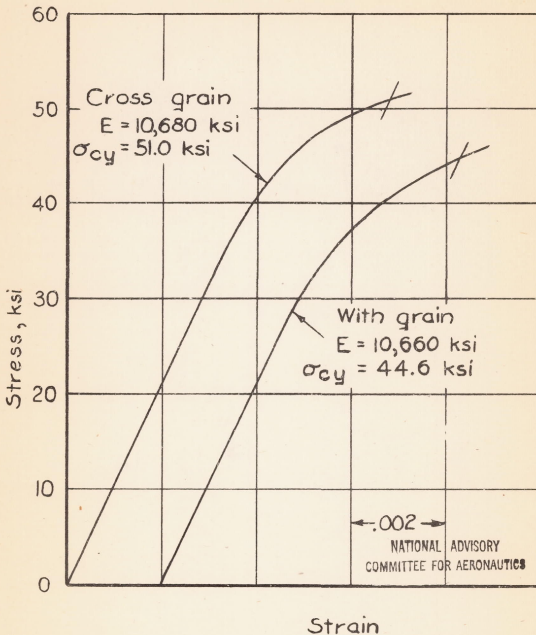
Figure 1.- Compressive stress-strain curves for 24 S-T aluminum alloy.
