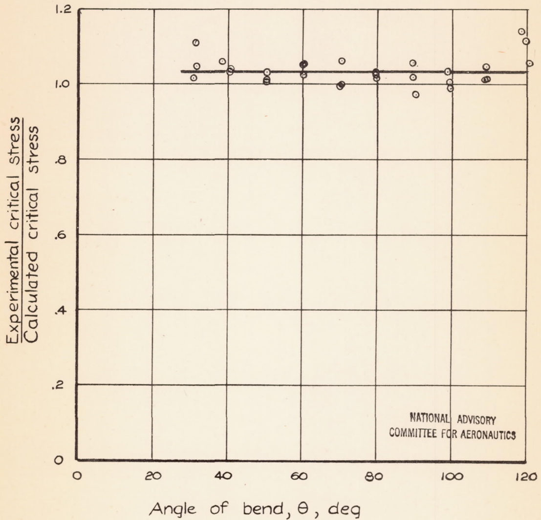
Figure 5. - Ratio of experimental to calculated critical stress for angles of bend.
