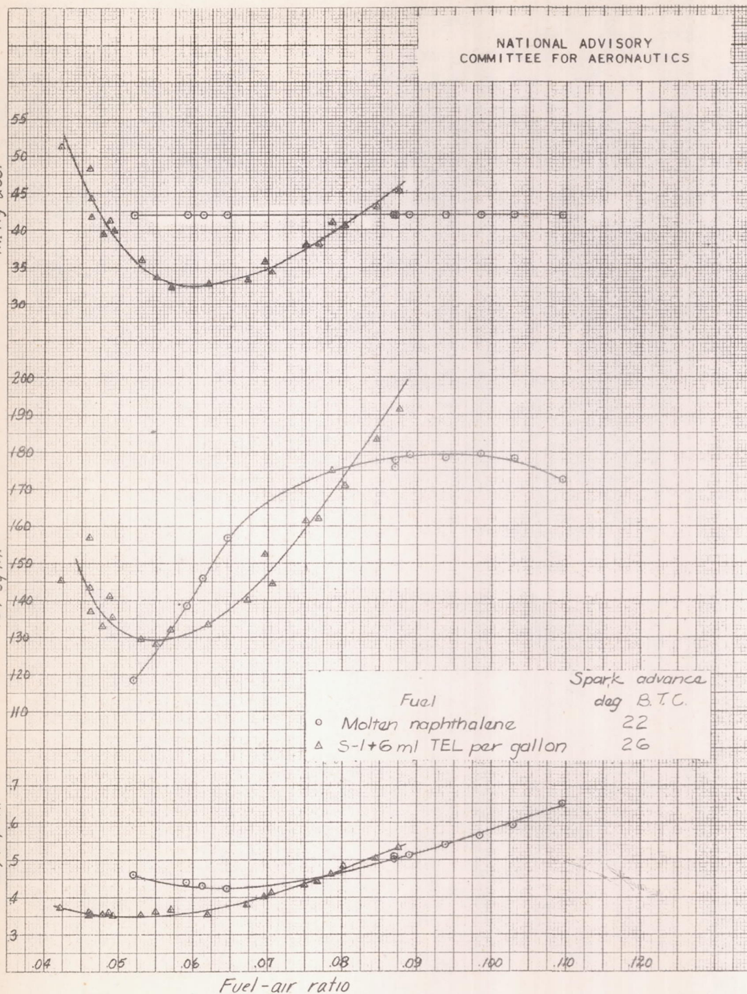
Figure 7. - Comparison of performance of CFR engine using molten naphthalene and S-1 plus 6 ml TEL per gallon as fuels. Inlet-air temperature, 300° F; compression ratio, 8; engine speed, 2000 rpm; maximum safe inlet-air pressure during naphthalene tests, 42.0 inches mercury absolute.
