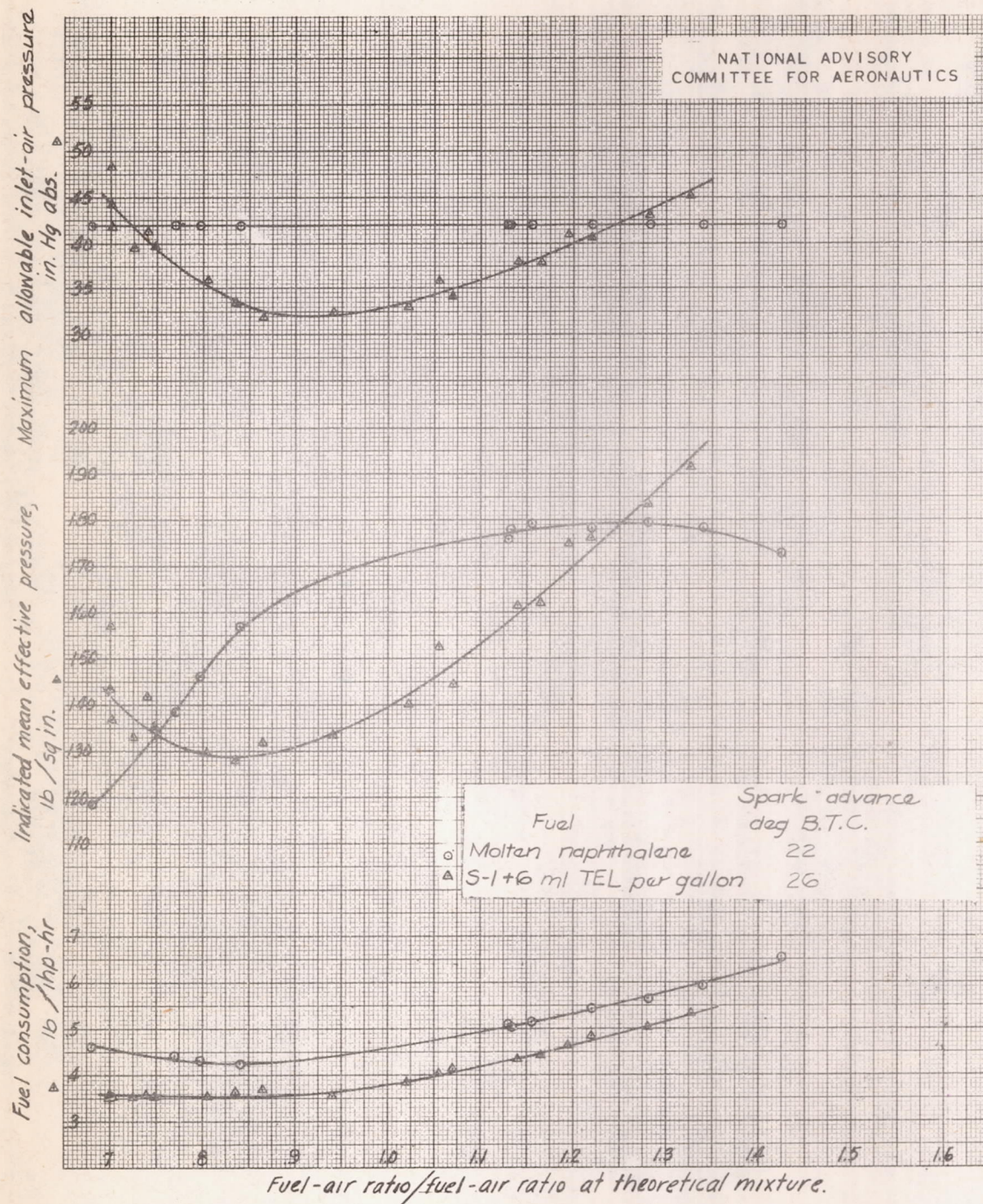
Figure 14. - Comparison of performance of CFR engine using molten naphthalene and S-1 plus 6 ml TEL per gallon as fuels. Inlet-air temperature, 200° F; compression ratio, 8; engine speed, 2000 rpm; maximum safe inlet-air pressure during naphthalene tests, 42.0 inches mercury absolute.
