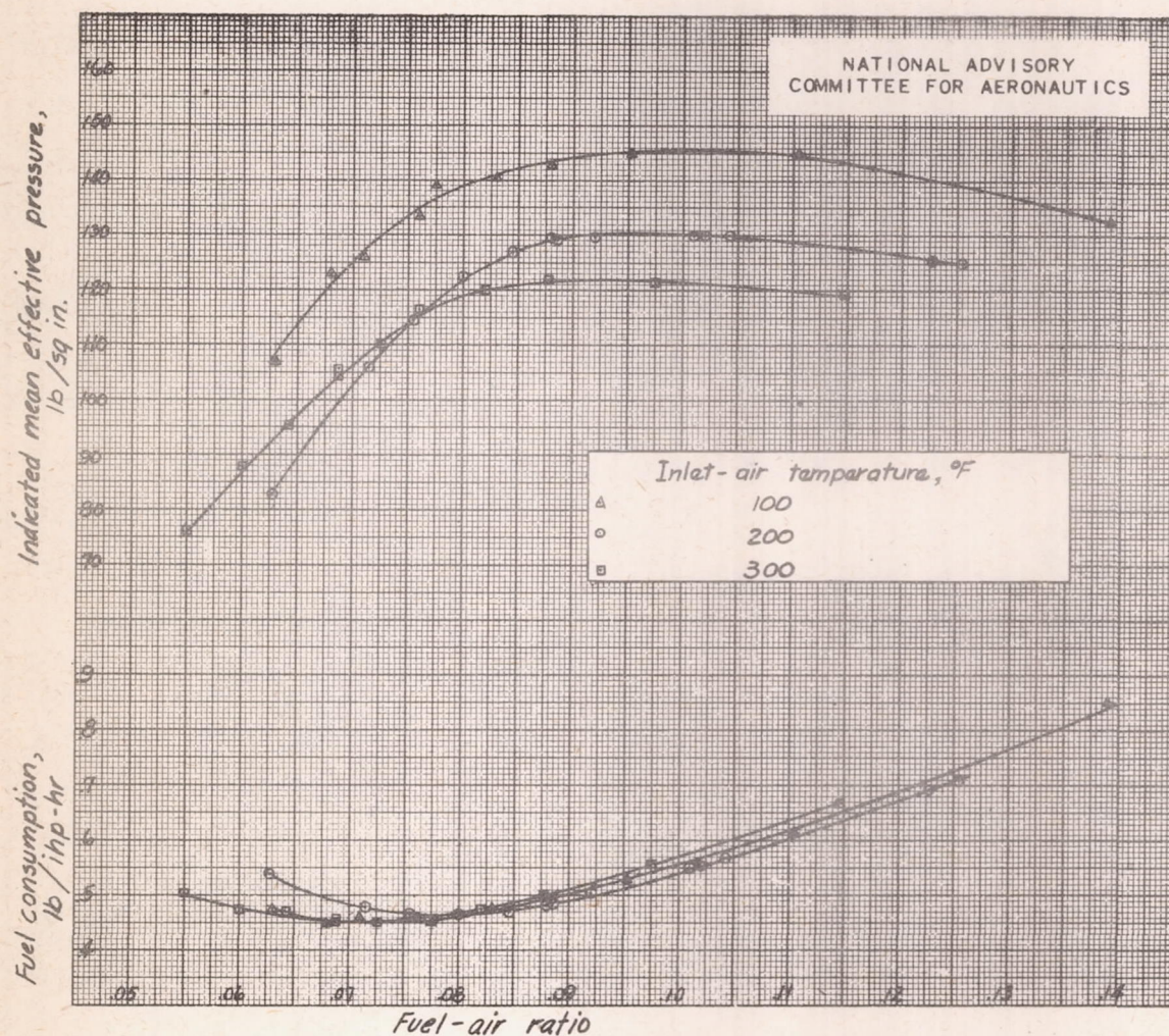
Figure 10. - Effect of inlet-air temperature on performance of CFR engine using molten naphthalene as fuel. Inlet-air pressure, 30.1 inches mercury absolute; compression ratio, 8; engine speed, 2000 rpm; spark advance, 22° B.T.C.
