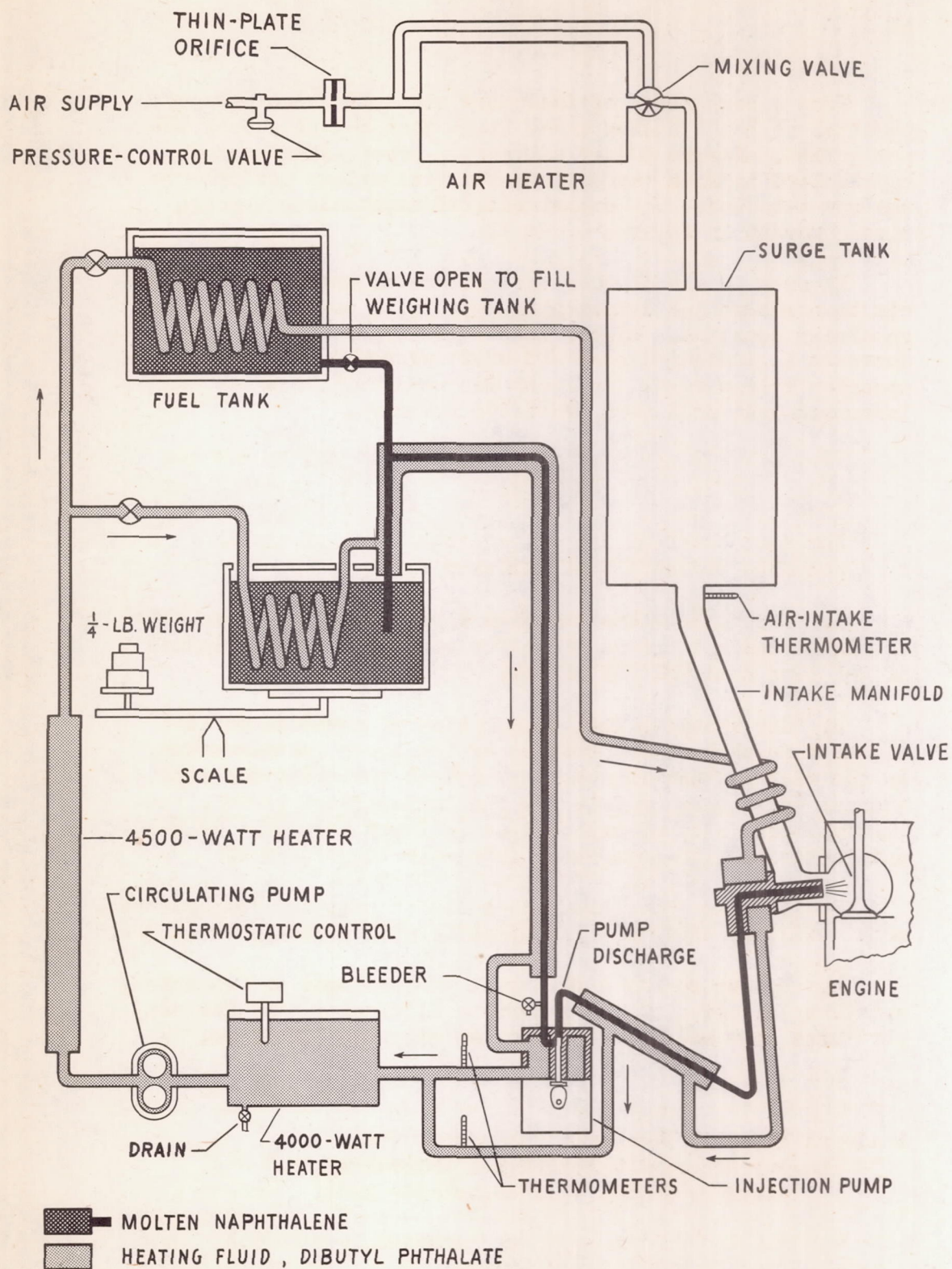
FIG. 1 DIAGRAMMATIC LAYOUT OF NAPHTHALENE SYSTEM
