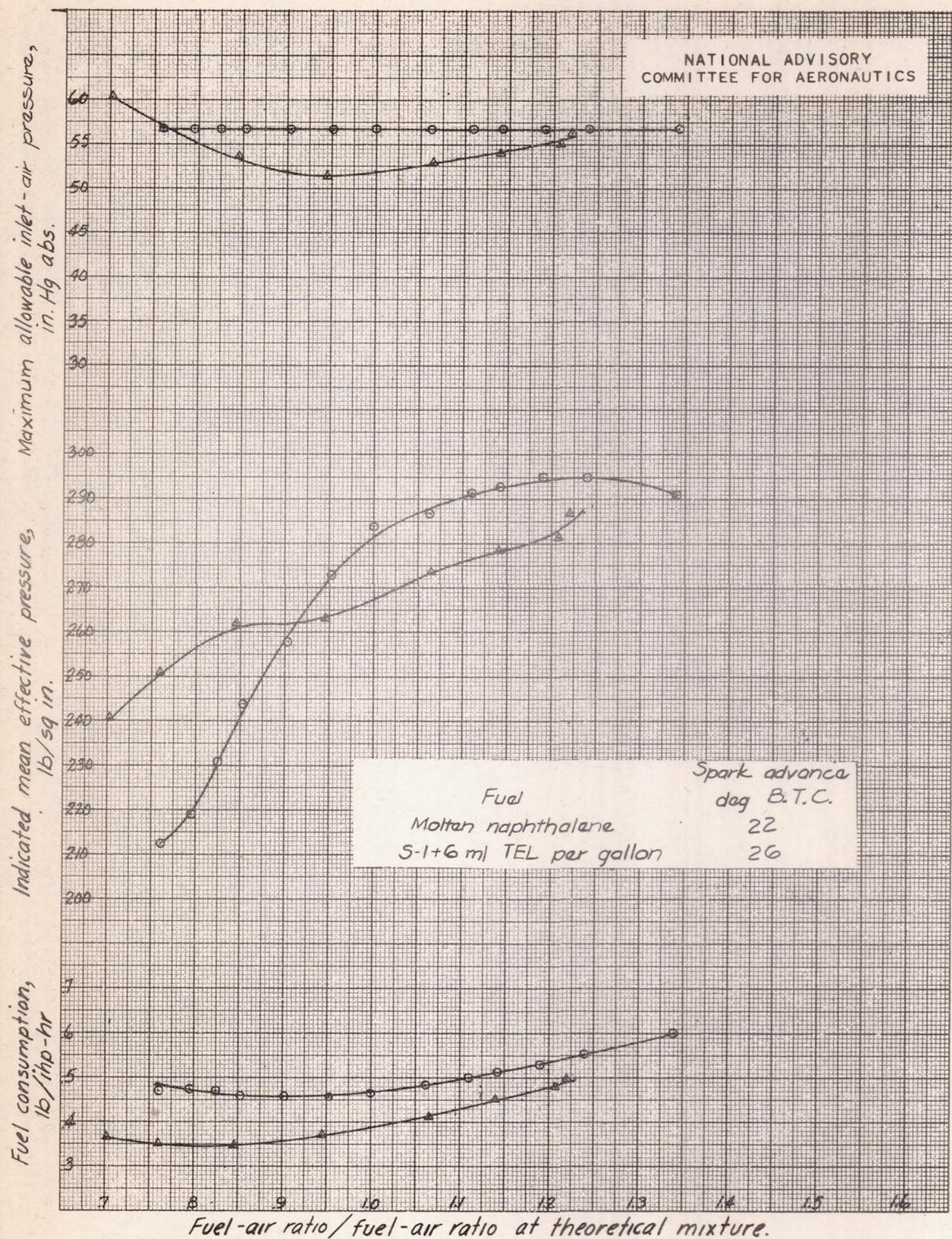
Figure 12. - Comparison of performance of CFR engine using molten naphthalene and S-1 plus 6 ml TEL per gallon as fuels. Inlet-air temperature, 100° F; compression ratio, 8; engine speed, 2000 rpm; maximum inlet-air pressure available during naphthalene tests, 56.75 inches mercury absolute.
