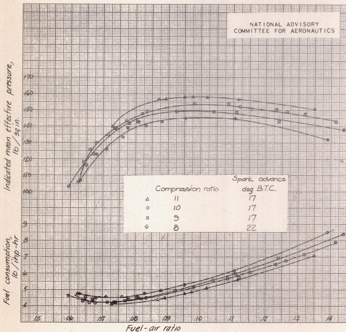
Figure 11. - Effect of compression ratio on performance of CFR engine using molten naphthalene as fuel. Inlet-air pressure, 30.1 inches mercury absolute; inlet-air temperature, 100° F; engine speed, 2000 rpm.
