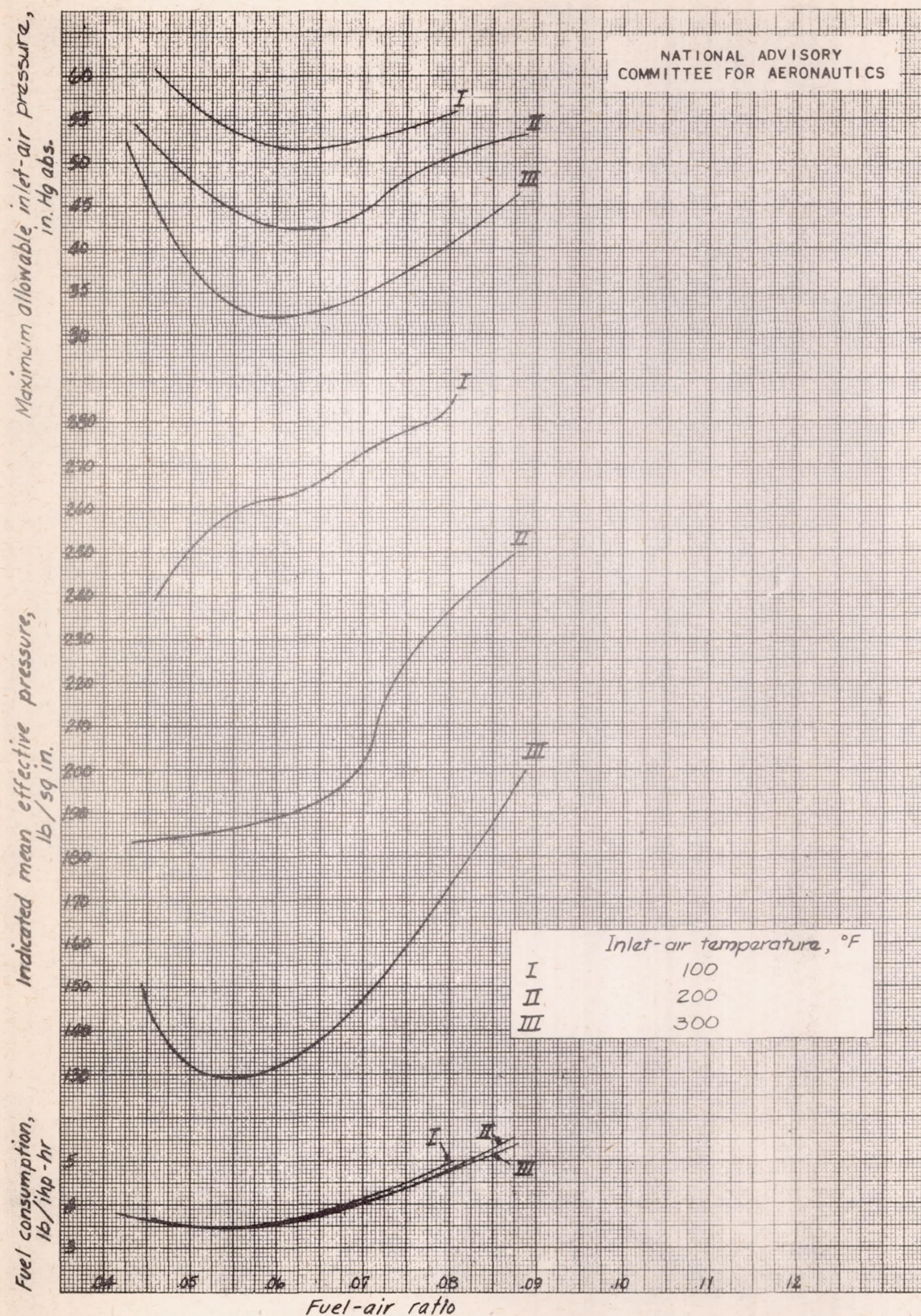
Figure 9. - Effect of inlet-air temperature on knock-limited performance of CFR engine using S-1 plus 6 ml TEL per gallon as fuel. Compression ratio, 8; engine speed, 2000 rpm; spark advance, 26° B.T.C.
