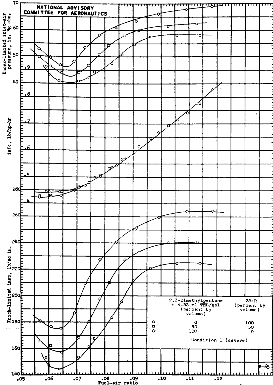
(a) Inlet-air temperature, 225° F; coolant temperature, 375° F; spark advance, 45° B.T.O. Figure 1. - Knock-limited performance of blends of 2,3-dimethylpentane and 28-R fuel, in CFR engine at compression ratio of 6.0. Engine speed, 1800 rpm; oil temperature, 165° F.
