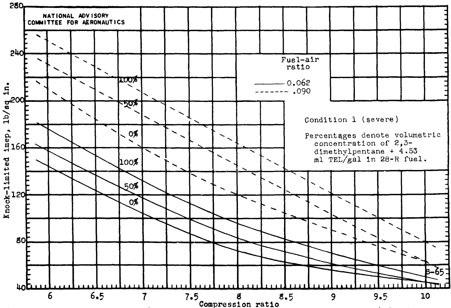
(a) Inlet-air temperature, 225° F; coolant temperature, 375° F; spark advance, 45° B.T.C. Figure 4. - Effect of compression ratio on knock-limited performance of 0, 50, and 100 percent 2,3-dimethylpentane in 28-R fuel at fuel-air ratios of 0.062 and 0.090. Engine speed, 1800 rpm; oil temperature, 165° F.
