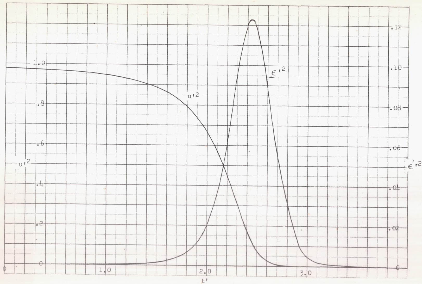
Figure 6.- Flow about a source-shaped impact tube. u'^2 obtained from equation (24) and \epsilon'^2 obtained from equation (22) for K = 3 by integration by Simpson's rule.
