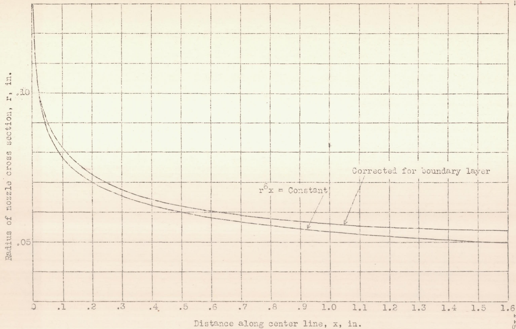
Figure 10.- Shape of nozzle, radius against distance along center line.
