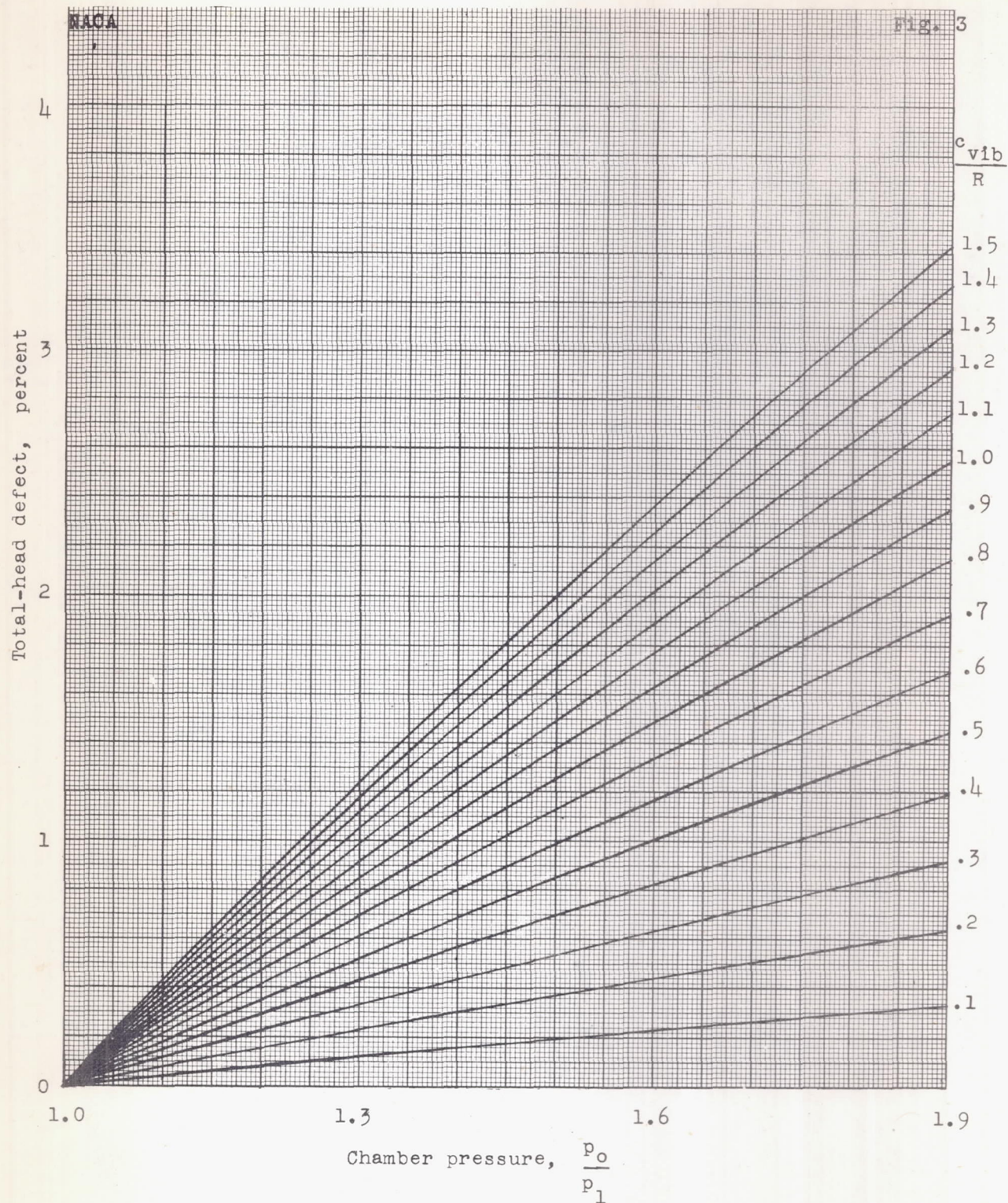
Figure 3.- Theoretical total-head defect in percent of dynamic pressure \frac{P_0}{P_1} - 1 for an instantaneous compression. (Linear molecules, c_p' = 3.5R ).
