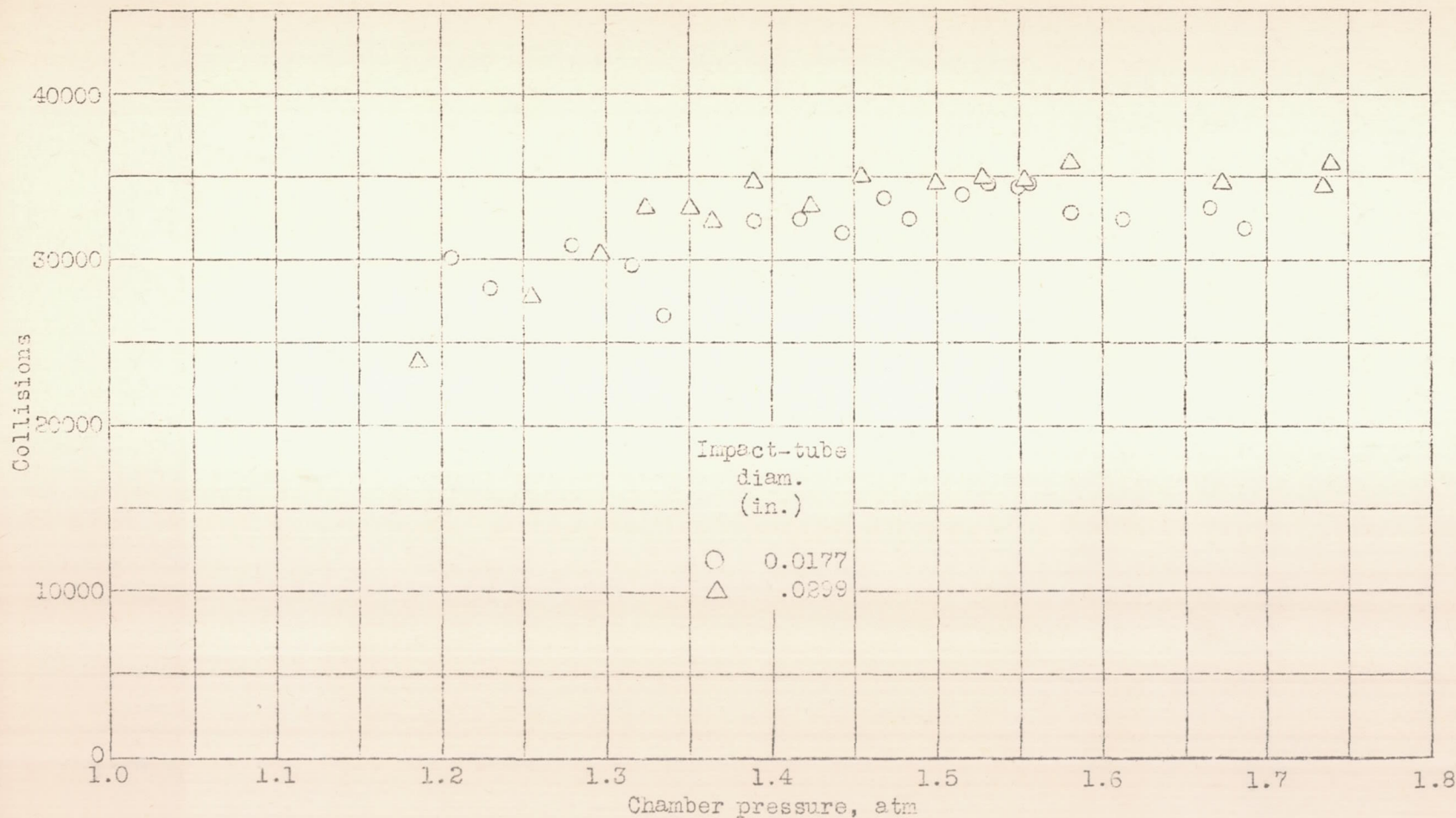
Figure 11.- Measurement of relaxation time of vibrational heat capacity in \text{CO}_2 . Temperature near 105^\circ \text{F} . Collisions = Relaxation time \times Collisions per molecule per second.
