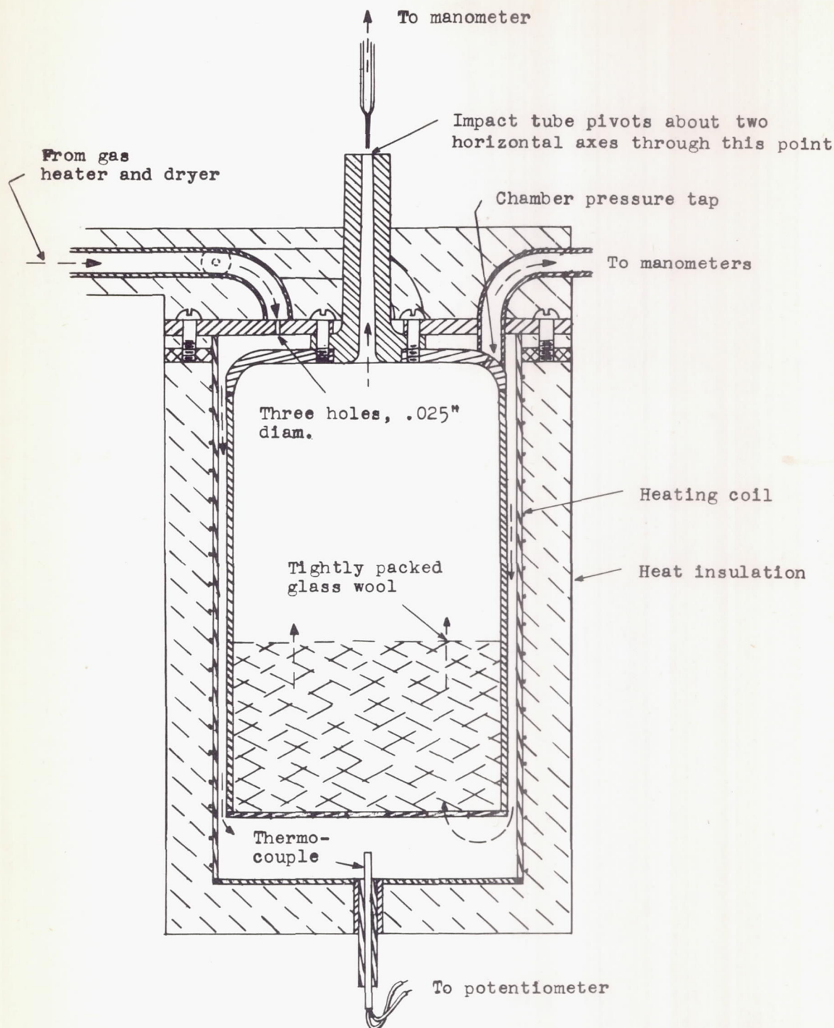
Figure 9.- Longitudinal section through chamber.
