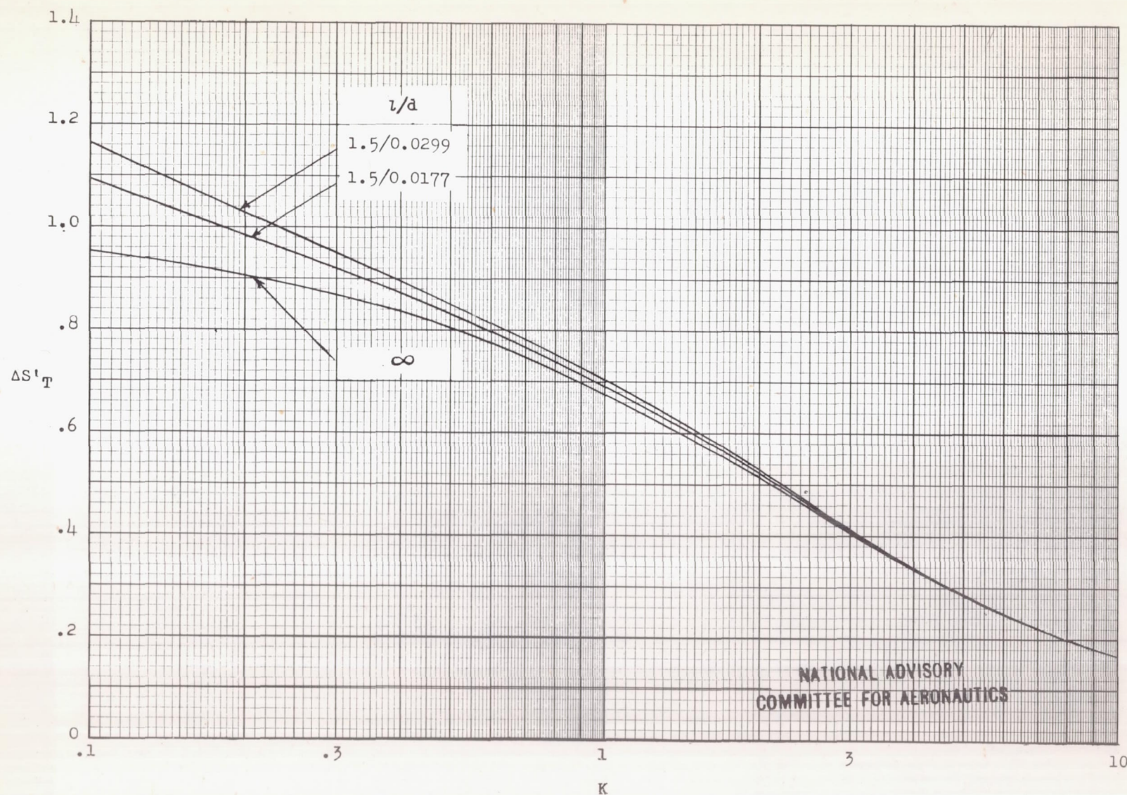
Figure 8.- Total entropy increase in nozzle and impact tube. \Delta S'_T = \Delta S'_{\text{tube}} + \Delta S'_N ; K = d/U\tau .
