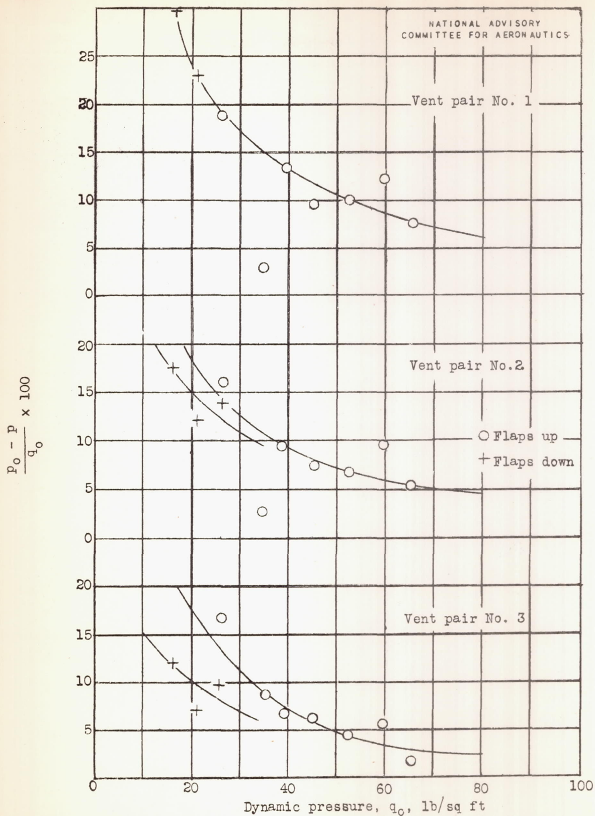
Figure 7.- Departure of the static pressure, measured with the fuselage static pressure "mice" from the ambient static pressure for various flap deflections on the Lockheed 12A airplane.
