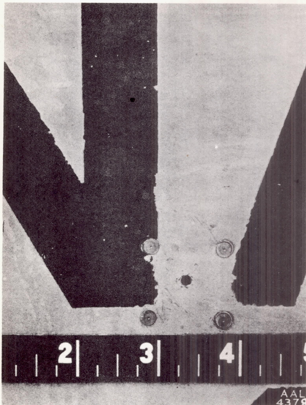
Figure 3.- The final fuselage static-pressure vent on the Lockheed 12A airplane.
