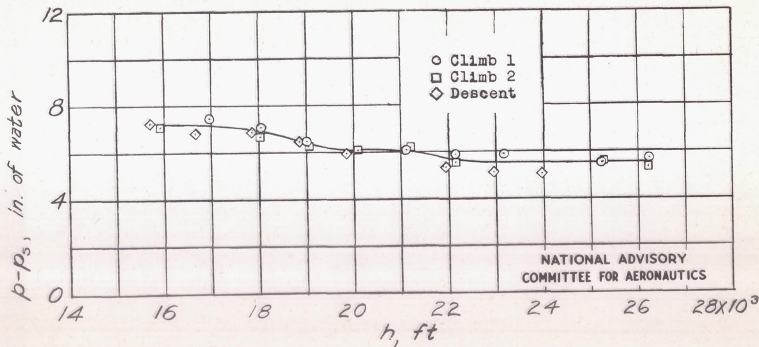
Figure 3.- Variation with altitude of the difference between atmospheric pressure and standard atmospheric pressure as determined from surveys.
