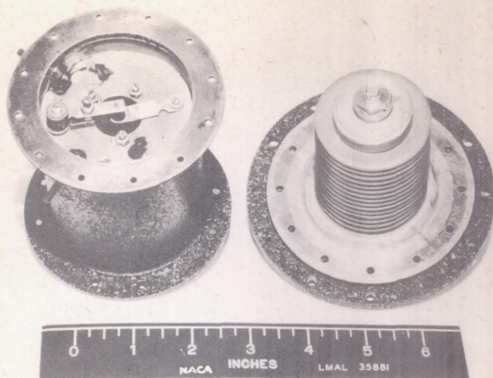
Figure 6.- Contact and terminals of NACA Mach number warning device assembled in case; outer bellows and fastening screw mounted.
