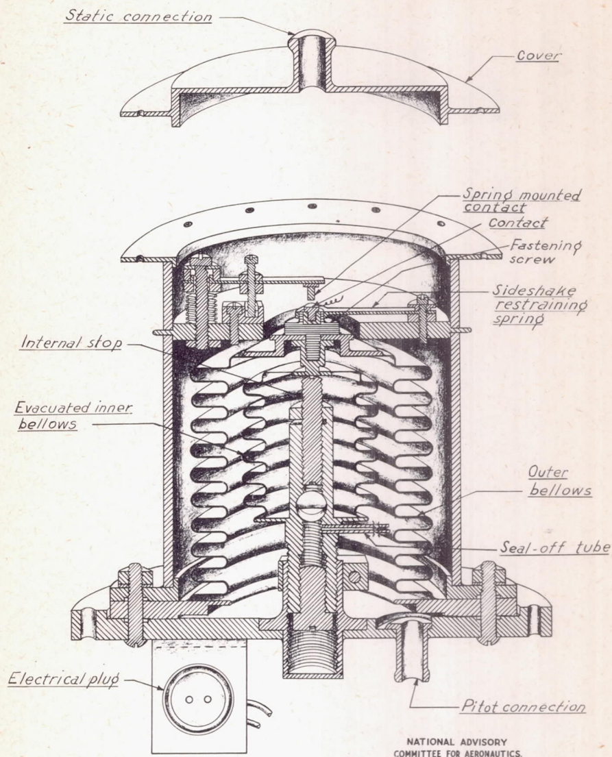
Figure 1.-Cross-sectional view of NACA Mach number warning device.
