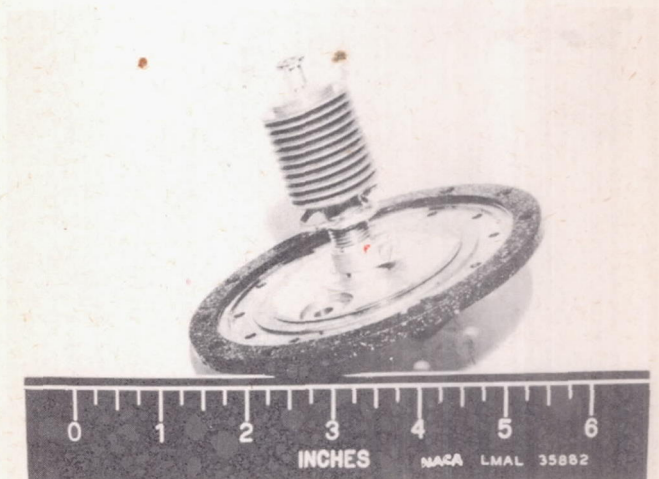
Figure 5.- Evacuated inner bellows of NACA Mach number warning device mounted on base.
