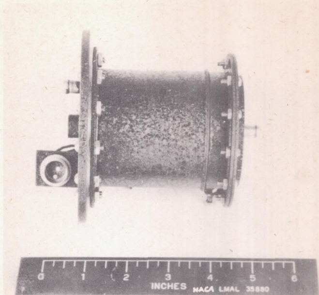
Figure 4.- NACA Mach number warning device.
