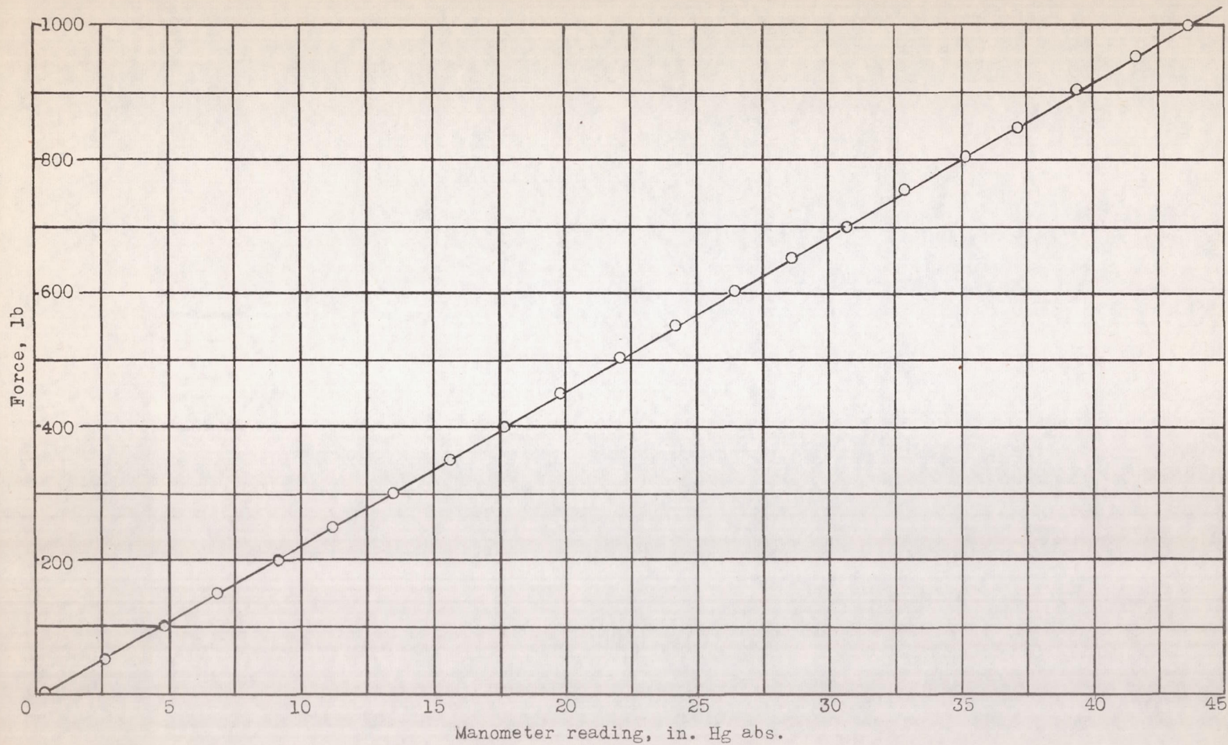
Figure 8.- Calibration of torque indicator for 1500-horsepower dynamometer.
