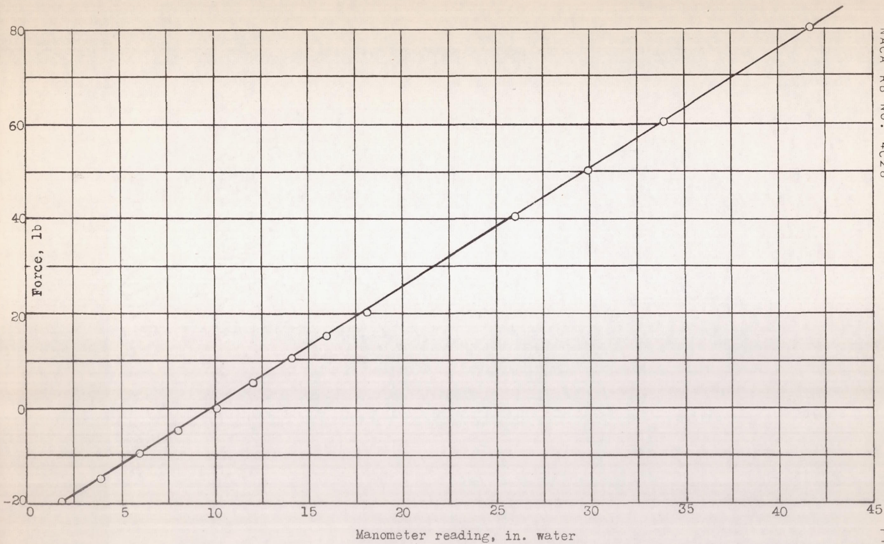
Figure 9.- Calibration of torque indicator for 300-horsepower dynamometer.
