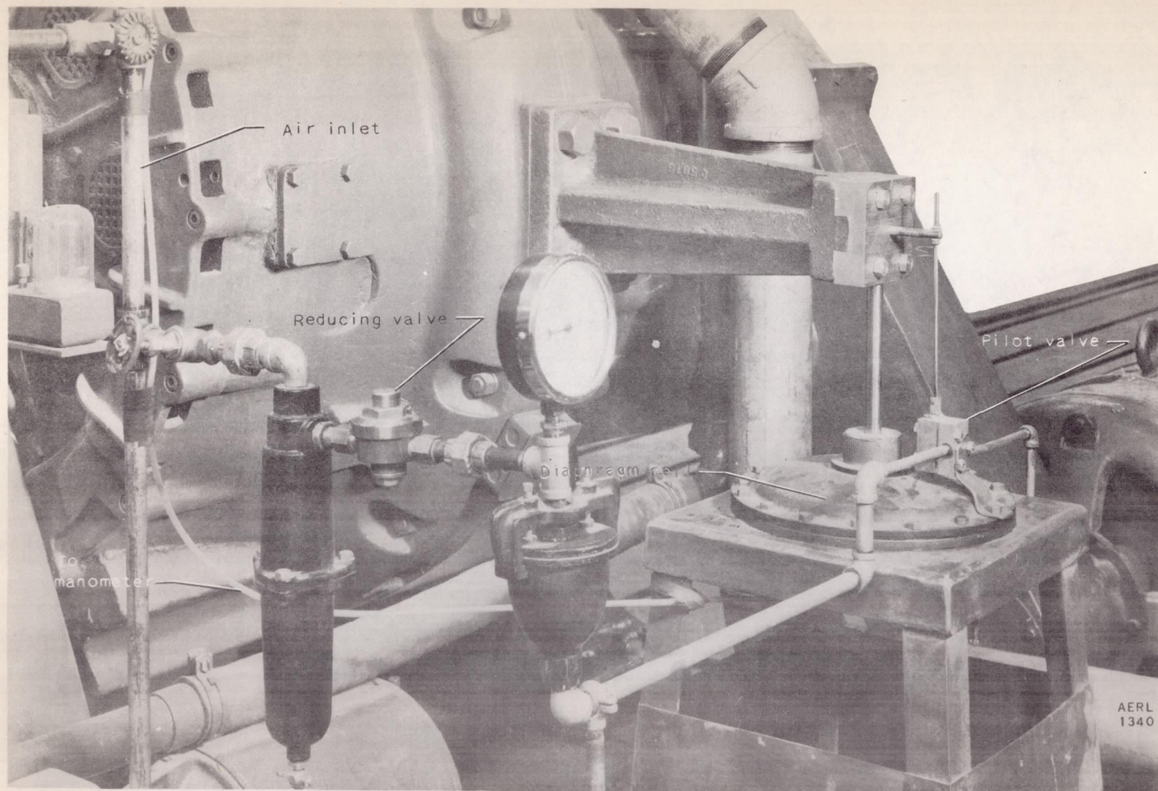
Figure 3.- Installation of torque indicator for 1500-horsepower dynamometer.
