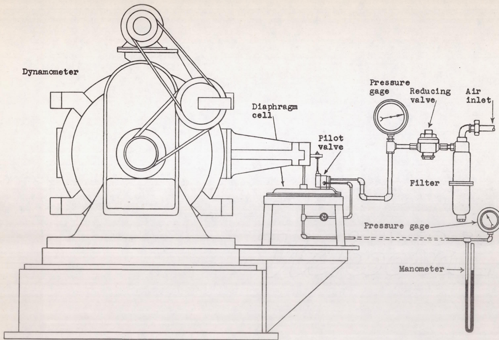
Figure 1.- Schematic diagram of dynamometer-torque indicator.
