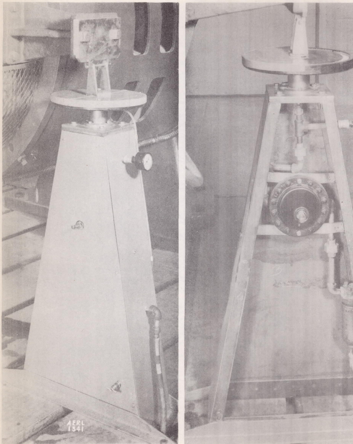
Figure 4.- Installation of torque indicator for 1000-horsepower dynamometer.
