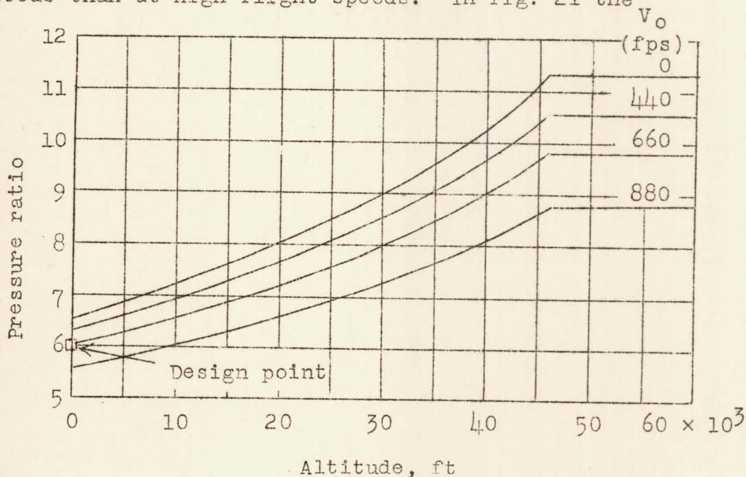
Figure 21.- Effect of altitude on pressure ratio over an axial compressor. Constant rotational speed and air volume.
