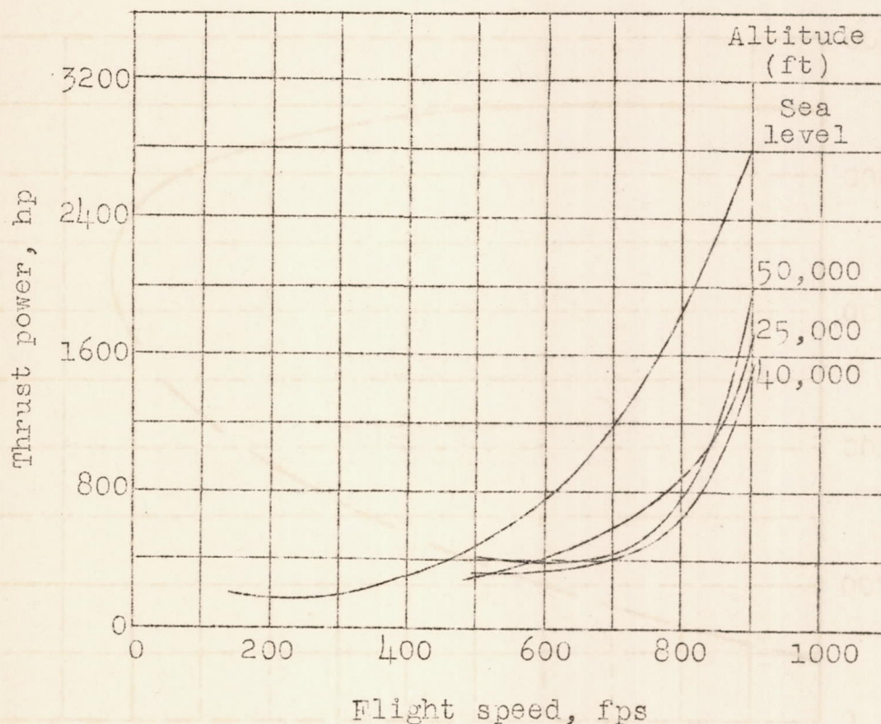
Figure 18.- Power required by airplane for level flight.
