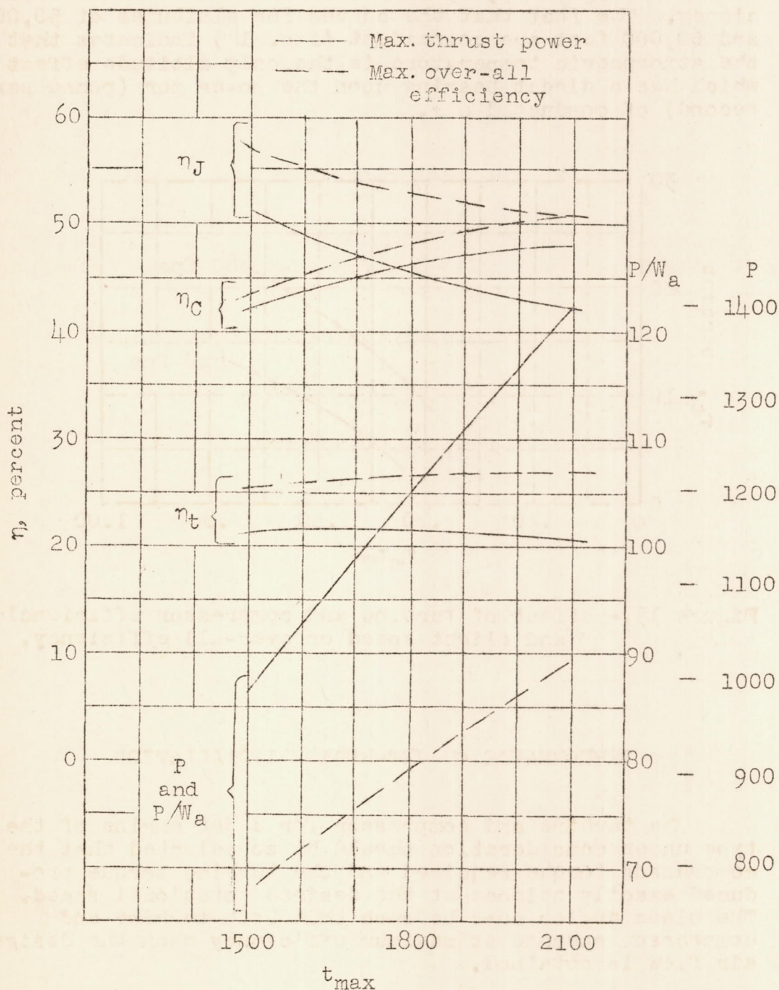
Figure 12.- Effect of temperature on power and efficiencies. Altitude, 40,000 feet; V_0 = 880 feet per second; \eta_C = \eta_T = 85 percent.
