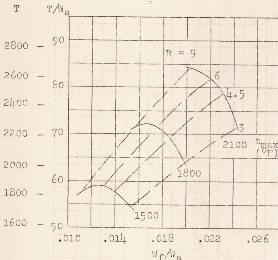
Figure 8.- Effects of fuel-air ratio, pressure ratio, and maximum temperature on thrust. At sea level; V_0 = 0 ; \eta_c = \eta_T = 85 percent.
