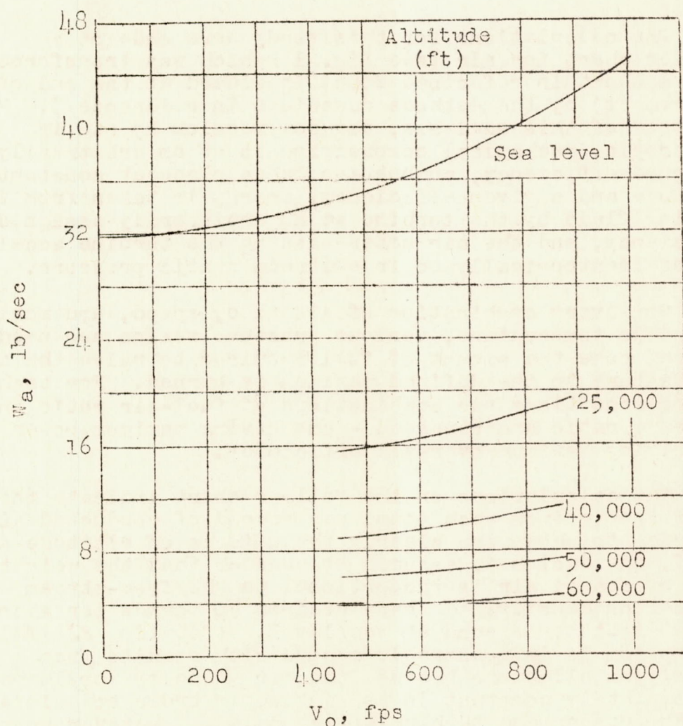
Figure 2.- Weight flow of charge air.
