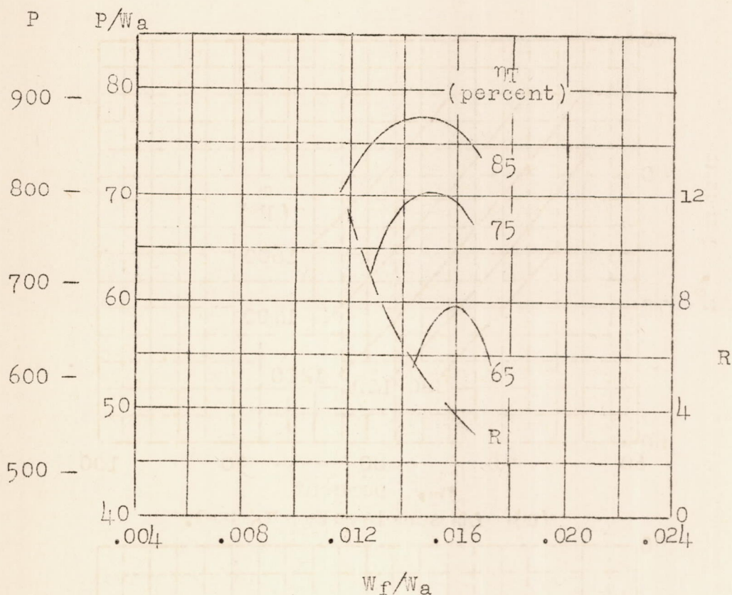
Figure 6.- Effect of fuel-air ratio on thrust power and pressure ratio. Altitude, 40,000 feet; V_0 = 880 feet per second; t_{max} = 1500^\circ \text{F} ; \eta_c = 75 percent.
