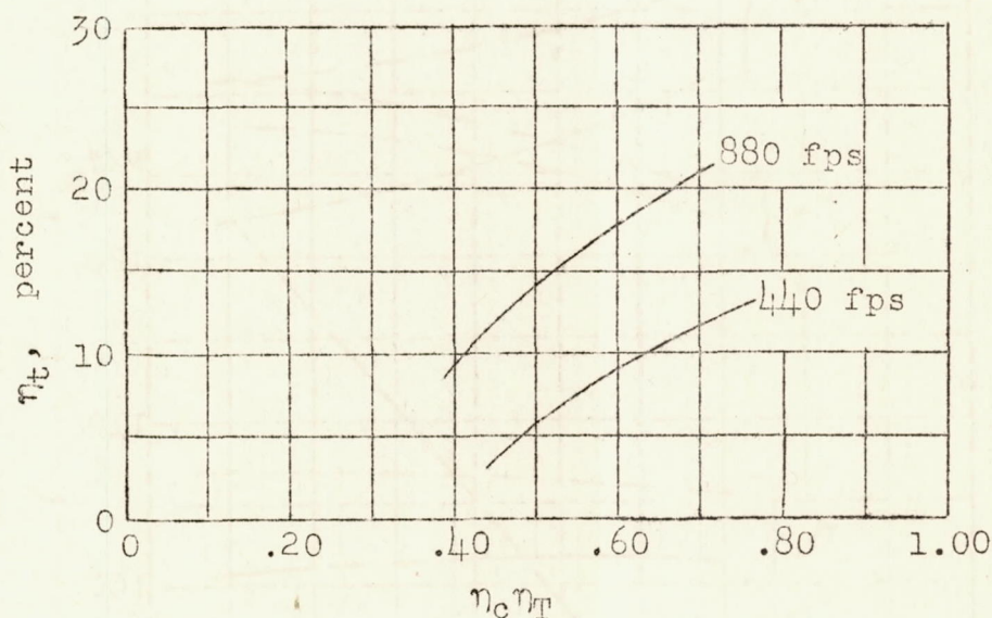
Figure 13.- Effect of turbine and compressor efficiencies and flight speed on over-all efficiency.
