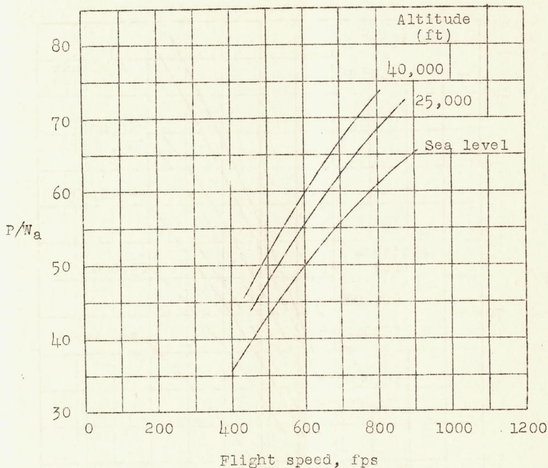
Figure 15.- Engine performance when design is for maximum over-all efficiency. t_{\max} = 1800^{\circ} \text{ F} ; \eta_c = \eta_T = 85 percent.
