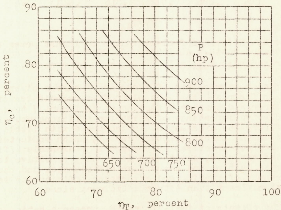
(b) Altitude, 40,000 feet; V_0 = 880 feet per second.
