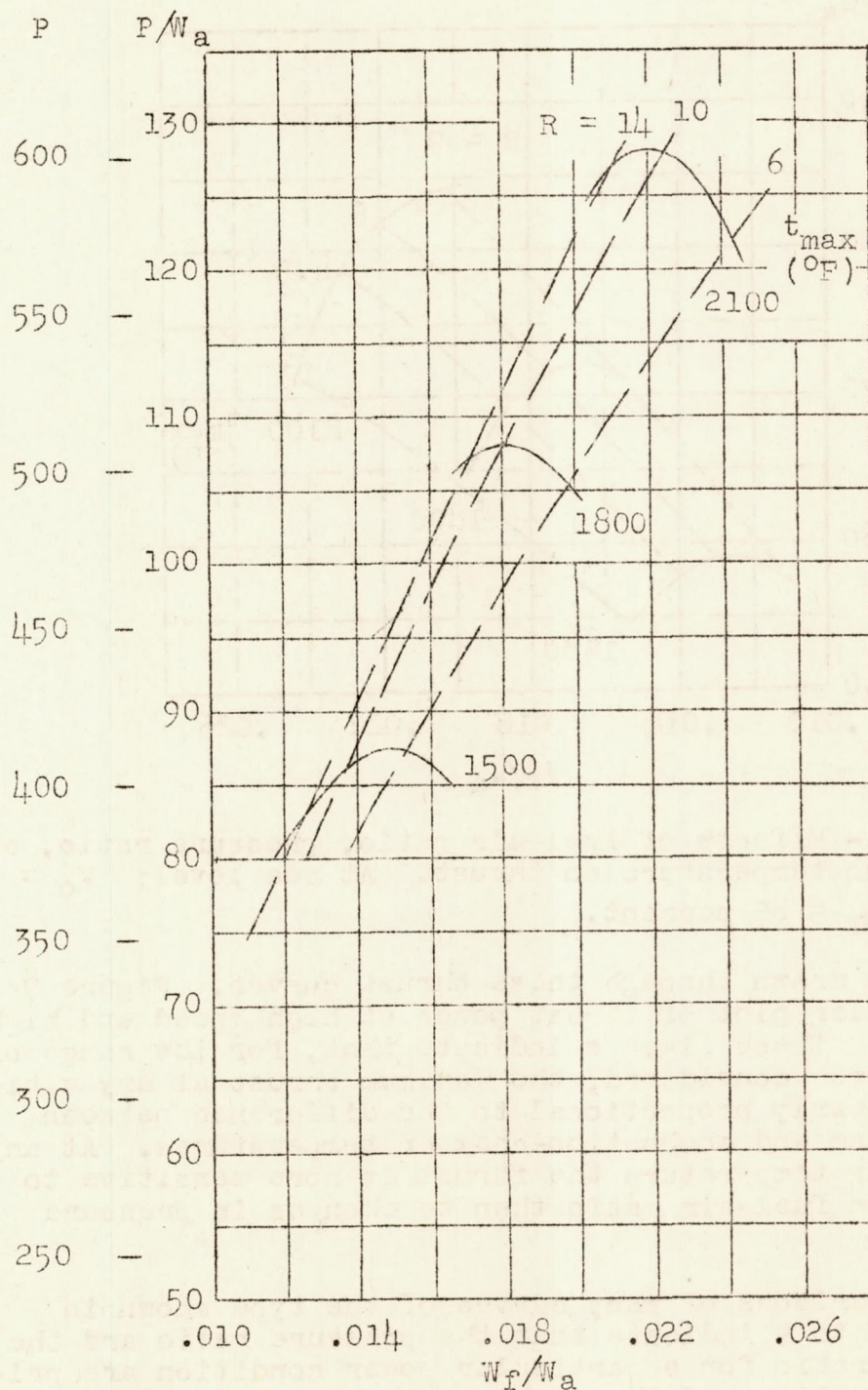
Figure 9.- Effects of fuel-air ratio, pressure ratio, and maximum temperature on thrust power. Altitude, 60,000 feet; V_o = 880 feet per second; \eta_c = \eta_T = 85 percent.
