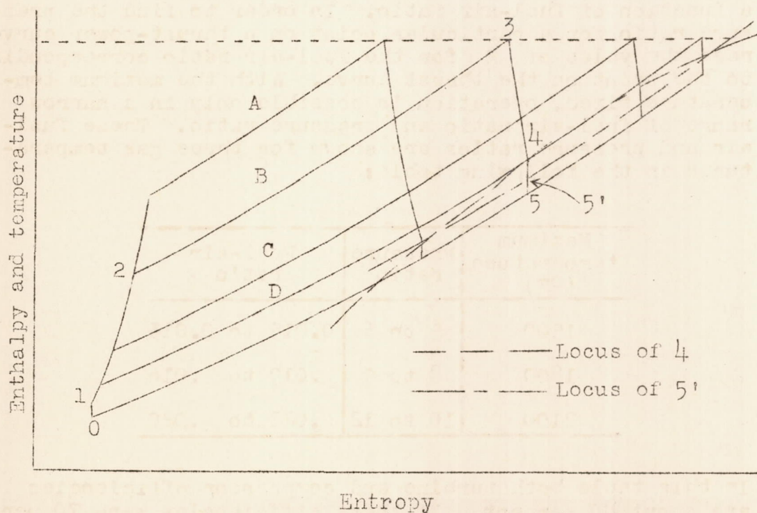
Figure 3.- Jet-engine cycles.
