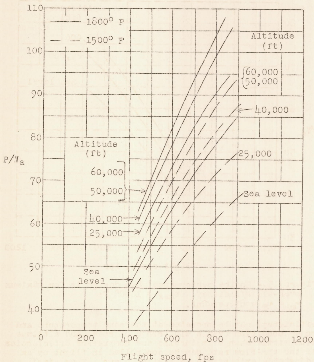
Figure 14.- Engine performance when design is for maximum power. \eta_c = \eta_T = 85 percent.
