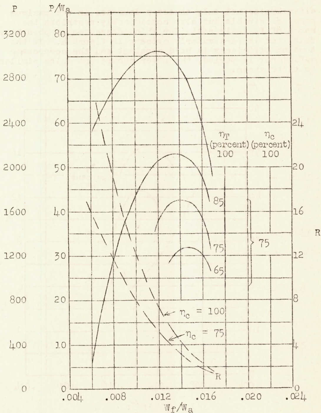
Figure 5.- Effect of fuel-air ratio on thrust power and pressure ratio. At sea level; V_o = 800 feet per second; t_{max} = 15000^\circ \text{ F.}
