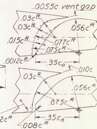
(b) Sealed-internal-balance aileron on the NACA 66,2-216 airfoil.
