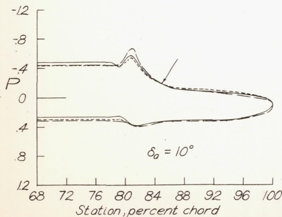
Figure 10. —Pressure distribution of 0.20c aileron having a sealed internal balance of 0.60c a on the NACA 66,2-216 airfoil, showing the effect of vent gap. M = 0.36 .
