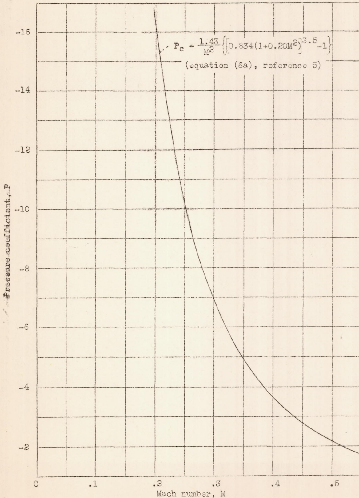
Figure 8.- Theoretical variation of critical-pressure coefficient with Mach number.
