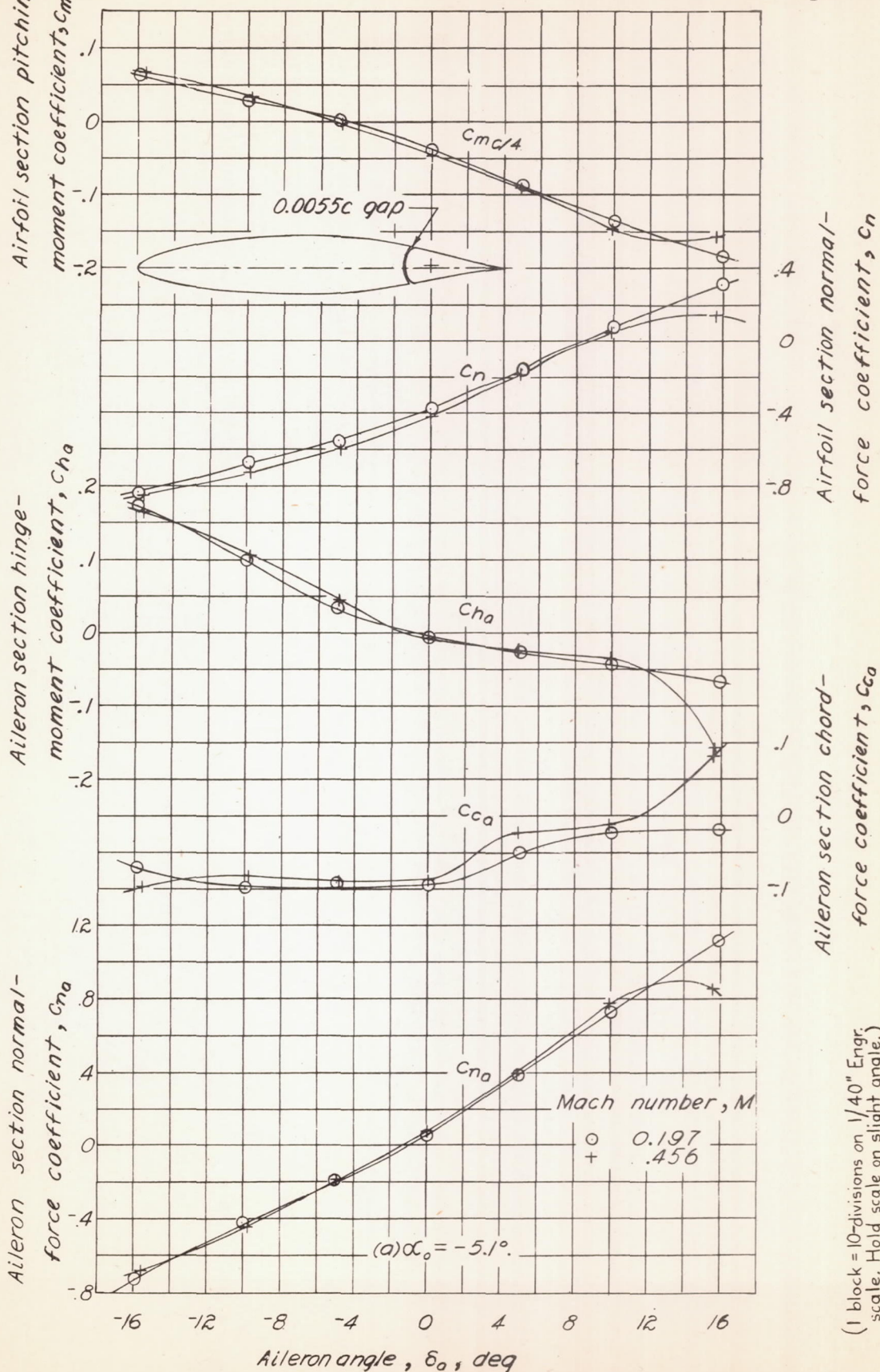
Figure 12.—Section characteristics of the NACA 66,2-216 airfoil with a 0.20c aileron having a blunt-nose balance of 0.35c a and 0.02c balance-nose radii.
