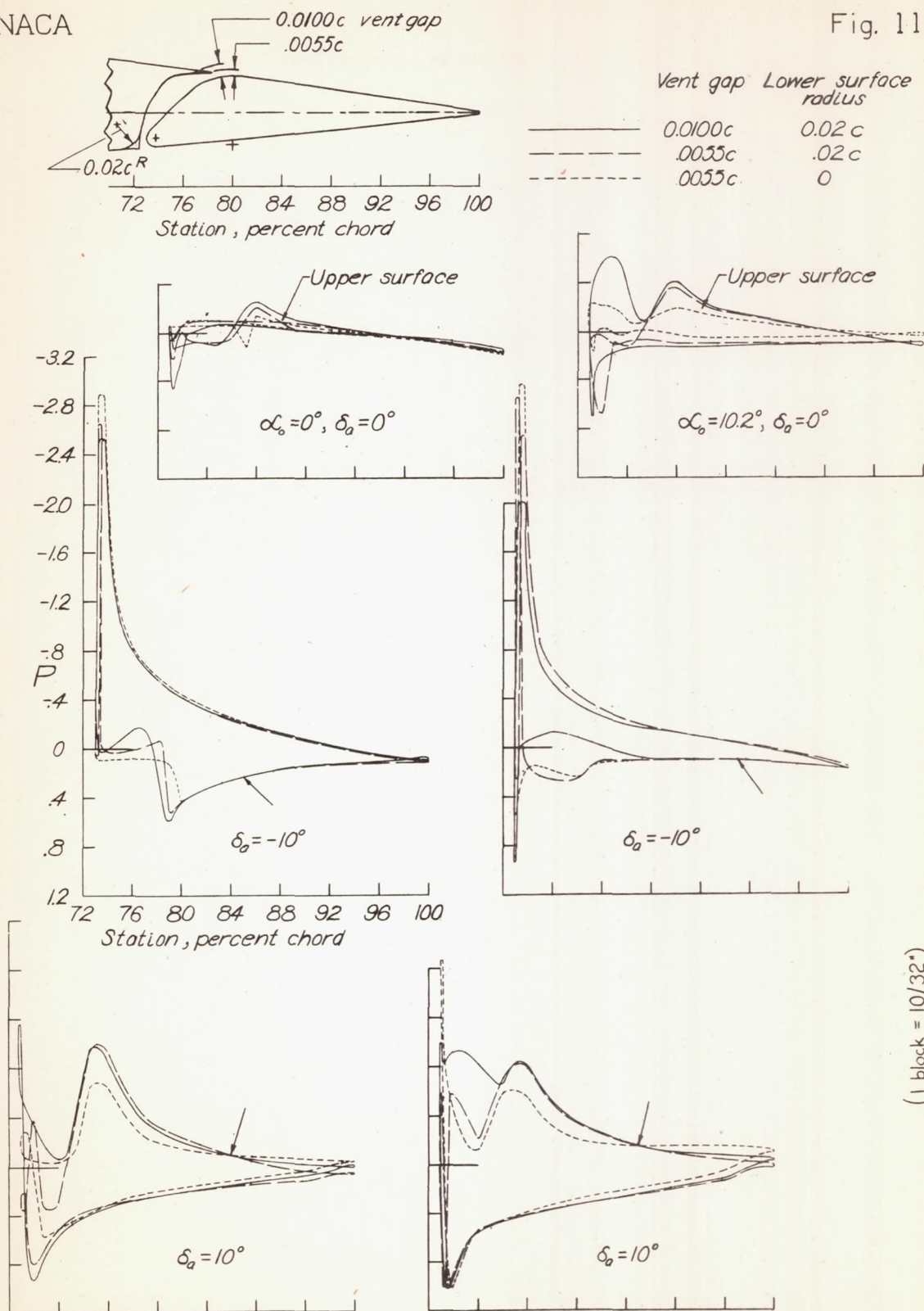
(b) Effect of vent gap and lower-surface radius. Balance-nose radius = 0.008c. Figure 11. — Concluded.
