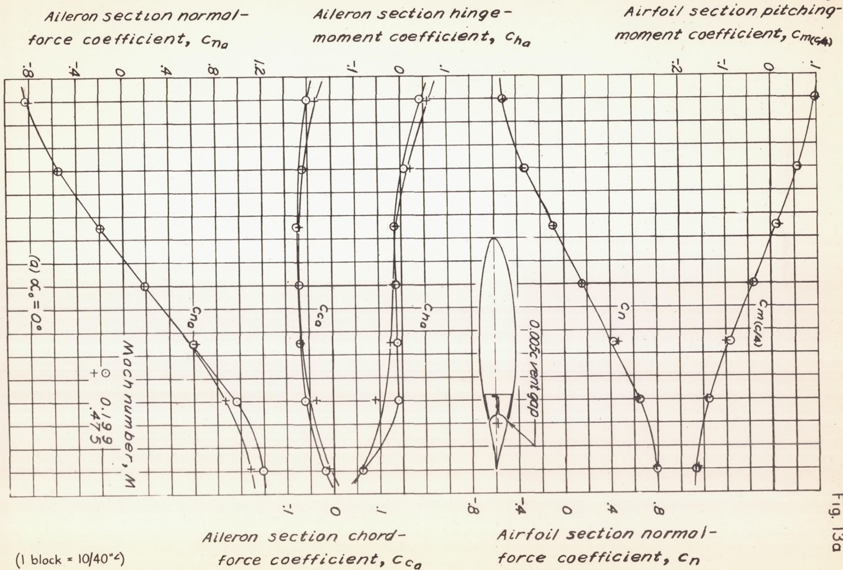
Figure 13. — Section characteristics of the NACA 66,2-216 airfoil with a 0.020c aileron having an internal balance of 0.60 C_o .
