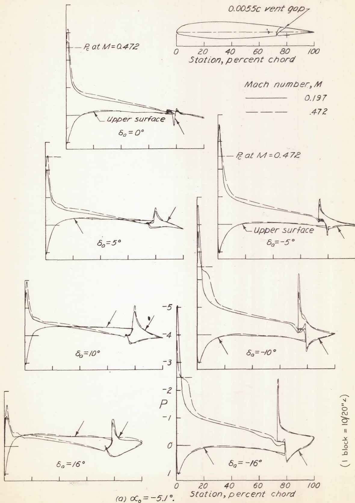
Figure 6. — Pressure distribution of the NACA 23012 airfoil with a 0.20c aileron having a Frise type balance of 0.35c a and a 0.008c nose radius.
