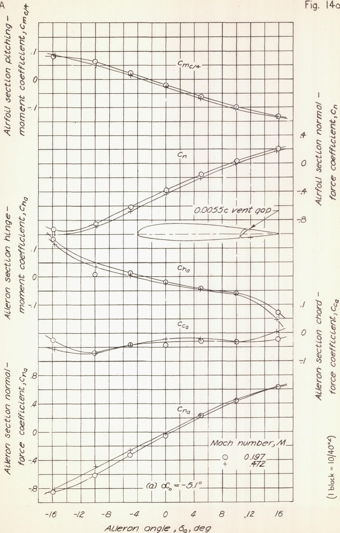
Figure 14. - Section characteristics of the NACA 23012 airfoil with a 0.20c aileron having a Frise type balance of 0.35c a and a 0.008c nose radius.
