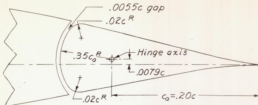
(a) Blunt-nose-balance aileron on the NACA 66,2-216, \alpha = 1.0 airfoil.
