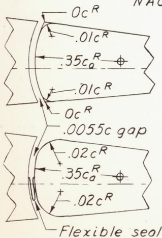
Figure 2. — Sketch of ailerons. All ailerons are of true contour. c = 24.00 inches.
