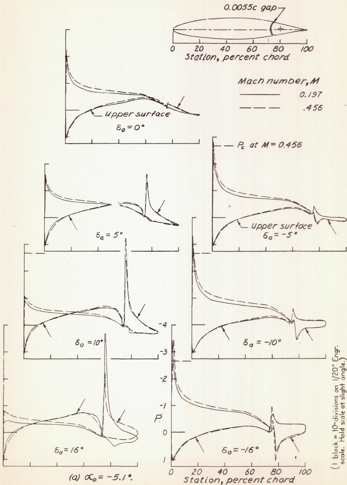
Figure 4. — Pressure distribution of the NACA 66, 2-216 airfoil with a 0.20c gileron having a blunt-nose balance of 0.35c a and 0.02c balance-nose radii.
