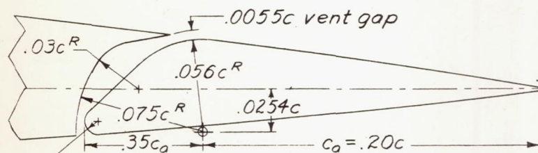
(c) Frise aileron on the NACA 23012 airfoil.
