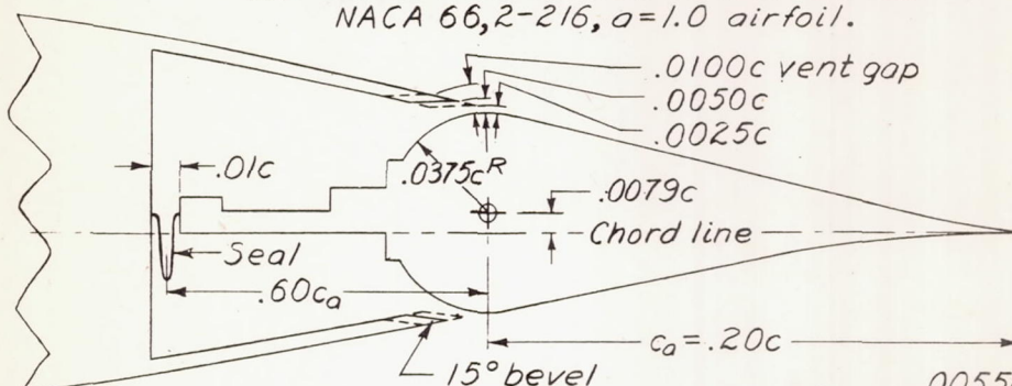
(b) Sealed-internal-balance aileron on the NACA 66,2-216 airfoil.
