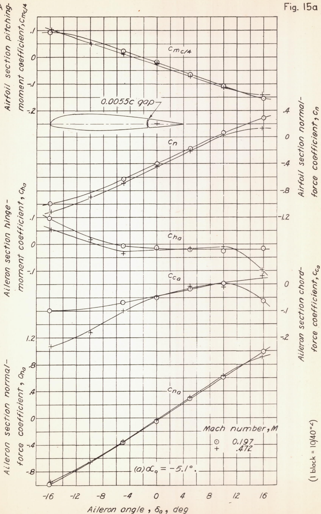
Figure 15. — Section characteristics of the NACA 23012 airfoil with a 0.20c aileron having a blunt nose balance of 0.35c and 0.02c balance-nose radii.
