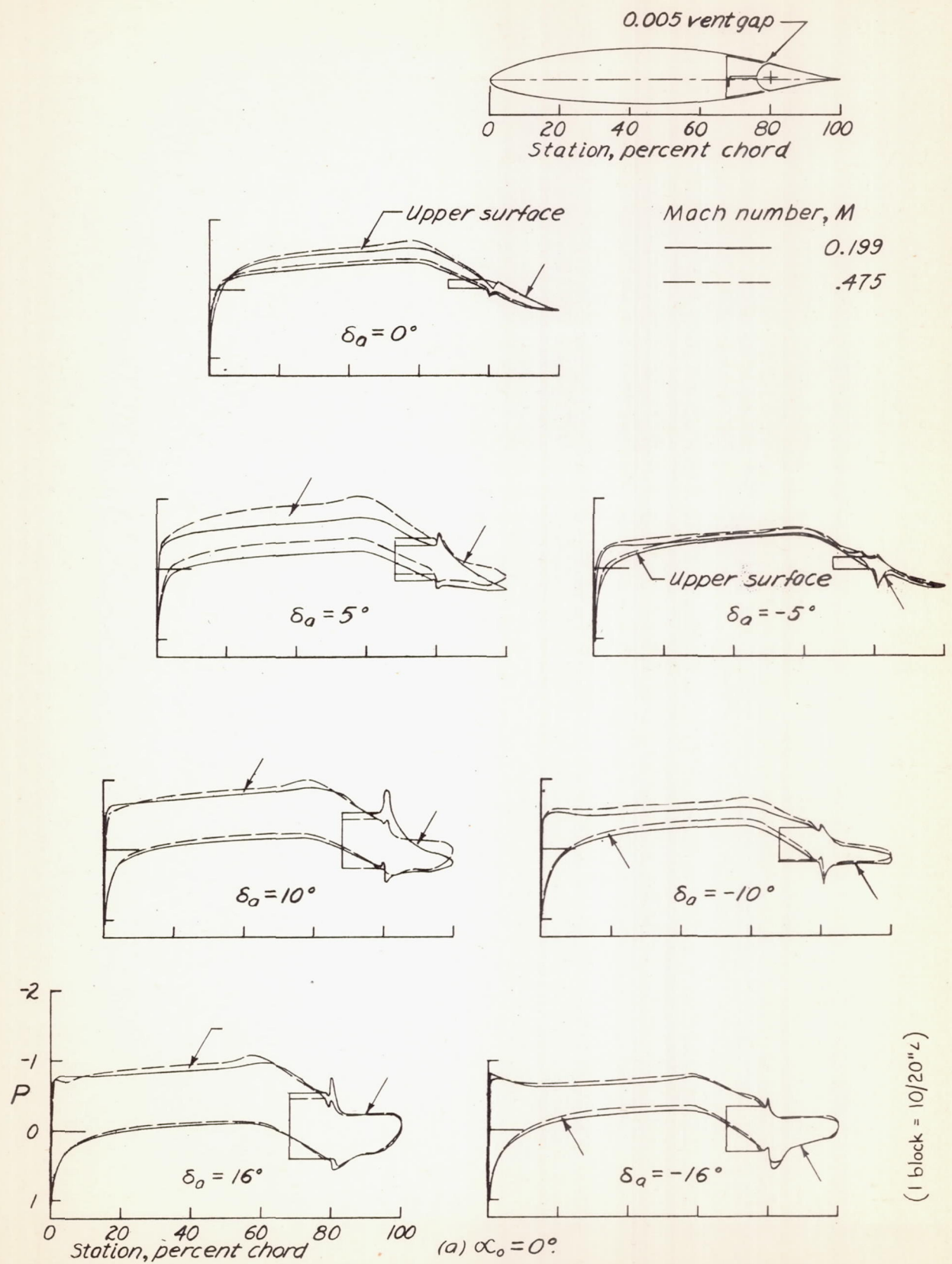
Figure 5. —Pressure distribution of the NACA 66,2-216 airfoil with a 0.20c aileron having an internal balance of 0.60 c_a .
