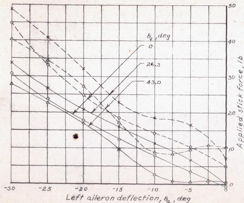
Figure 16. - Stick forces required to deflect the left aileron with the flap in various positions. Approximate test speed 58 miles per hour.
