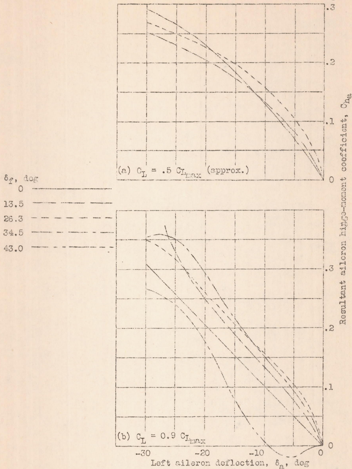
Figure 15.- Comparison of the resultant aerodynamic hinge-moment coefficients for the aileron at various flap positions. Approximate test speed, 58 miles per hour.
