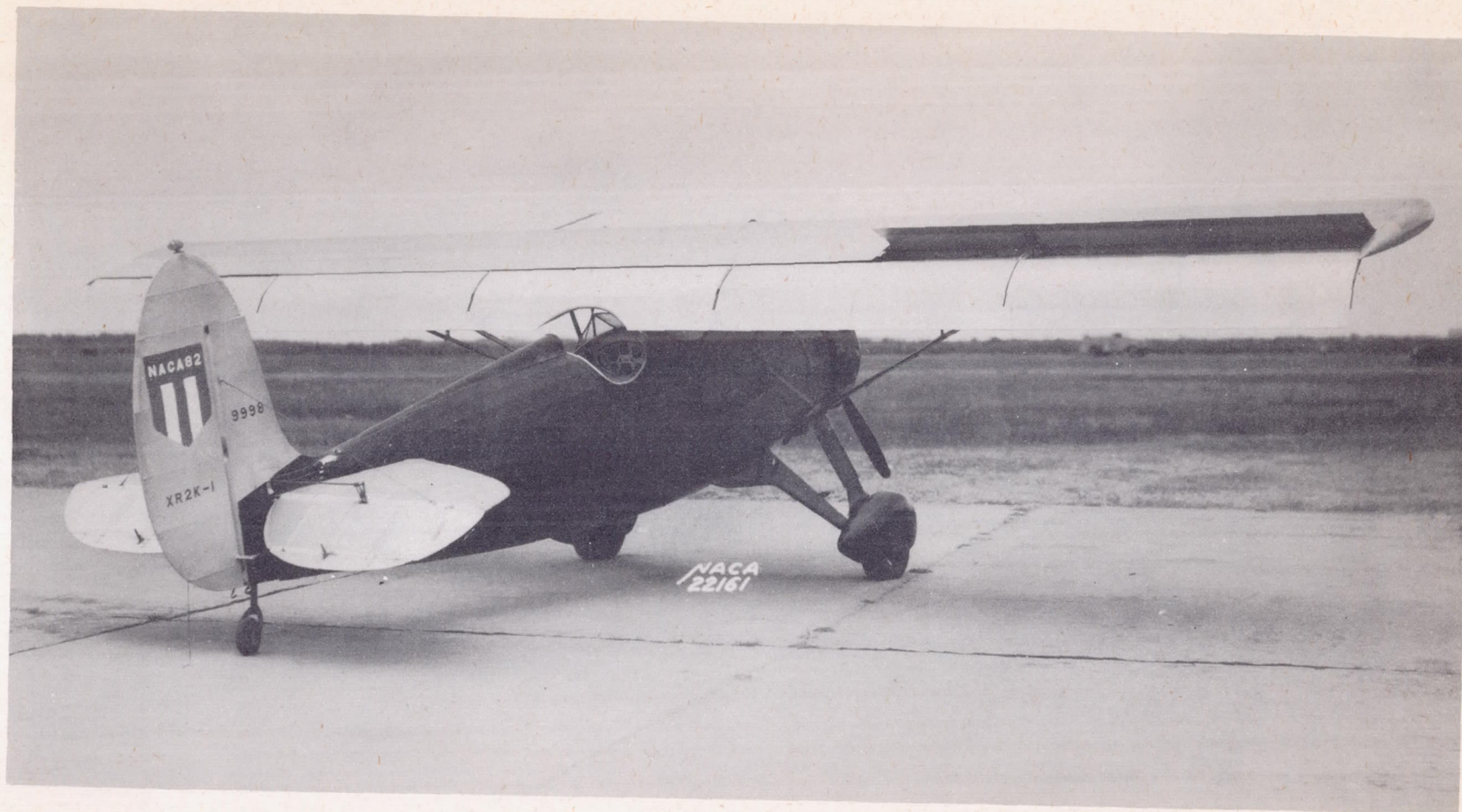
Figure 3.- Fairchild XR2K-1 airplane with Zap flap fully extended and right aileron raised.
