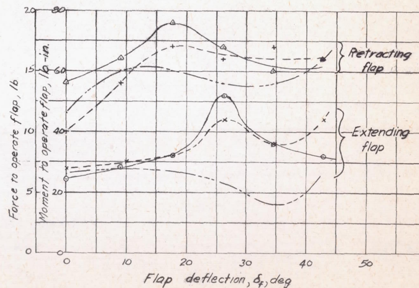
Figure 17. - Control forces required for extending and retracting the Zap flap.
