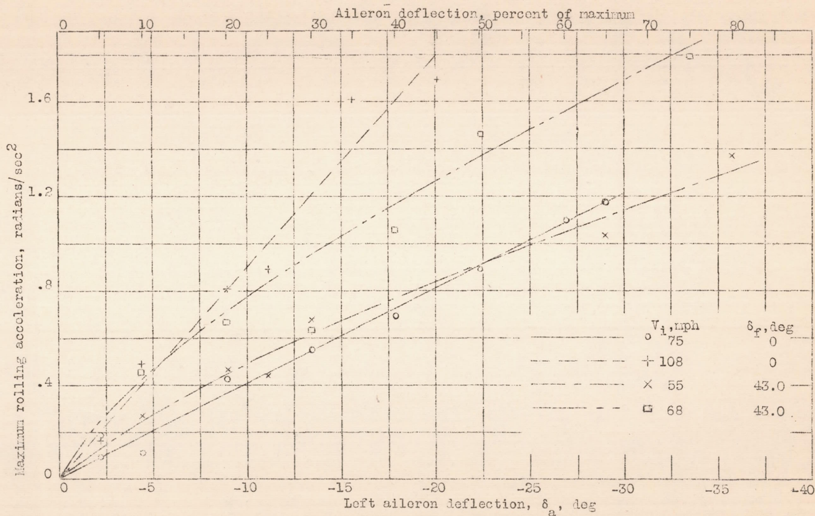
Figure 22.- Variation of the maximum rolling acceleration with aileron deflection for several indicated airspeeds and flap settings in abrupt aileron rolls. Fairchild XR2K-1 airplane with Zap-flap wing installation. Power on.
