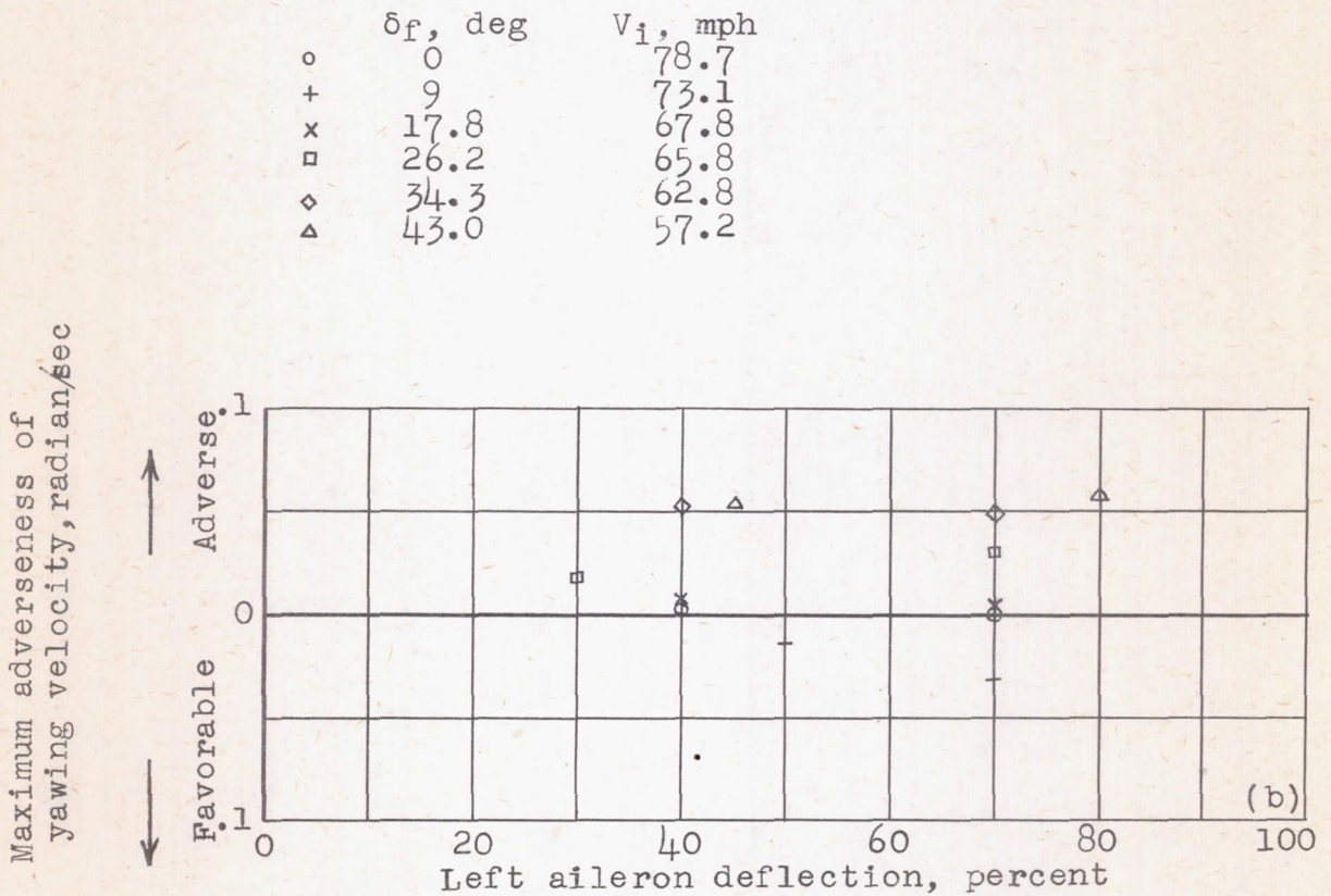
Figure 24.- Summary of aileron yawing characteristics on the Fairchild XR2K-1 airplane with Zap-flap wing installation.
