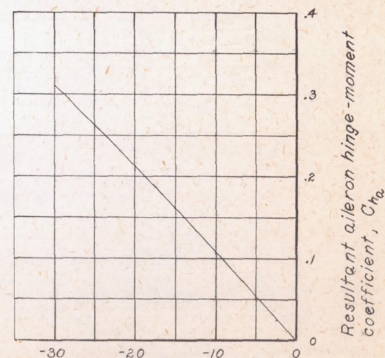
Figure 12. - Aileron rolling- and yawing-moment coefficients about the wind axes and resultant aileron hinge-moment coefficients of the Fairchild XR2K-1 airplane with the Zap-flap wing installation. Approximate test speed, 58 miles per hour; rolling velocity, zero; flap deflection, 0^\circ .
