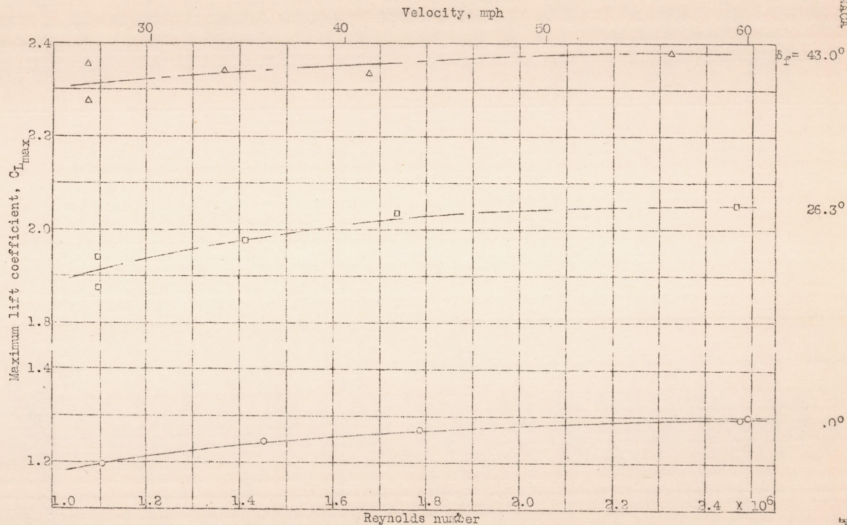
Figure 8.- Scale effect on the maximum lift coefficient with the Zap flap in three positions. Approximate range of test speeds from 28 to 60 miles per hour.
