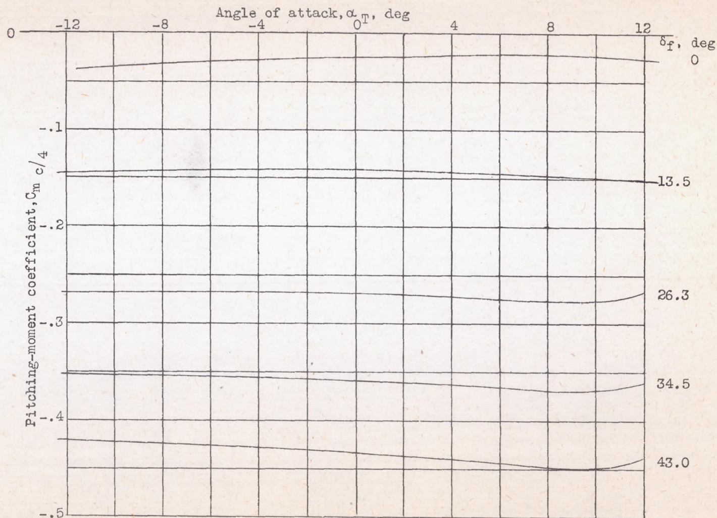
Figure 9.- Pitching-moment coefficients about the quarter-chord point for various flap deflections of the Fairchild XR2K-1 airplane with the Zap-flap wing installation. Approximate test speed, 58 miles per hour.
