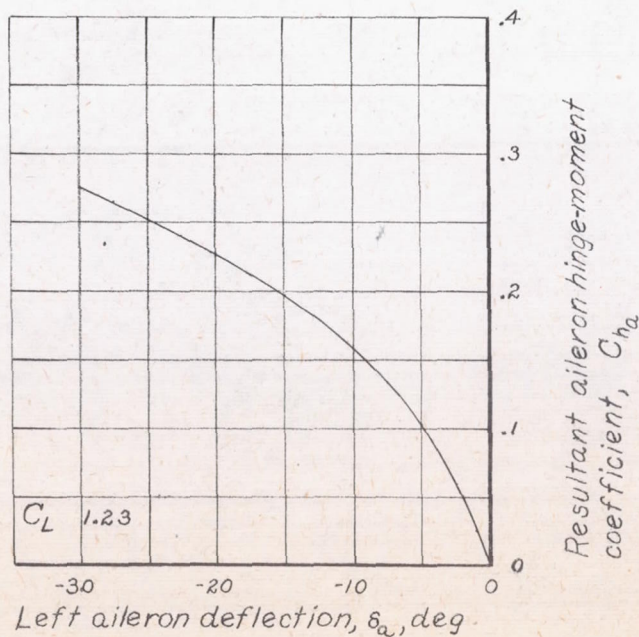
(a) C_L = 1.23 .
