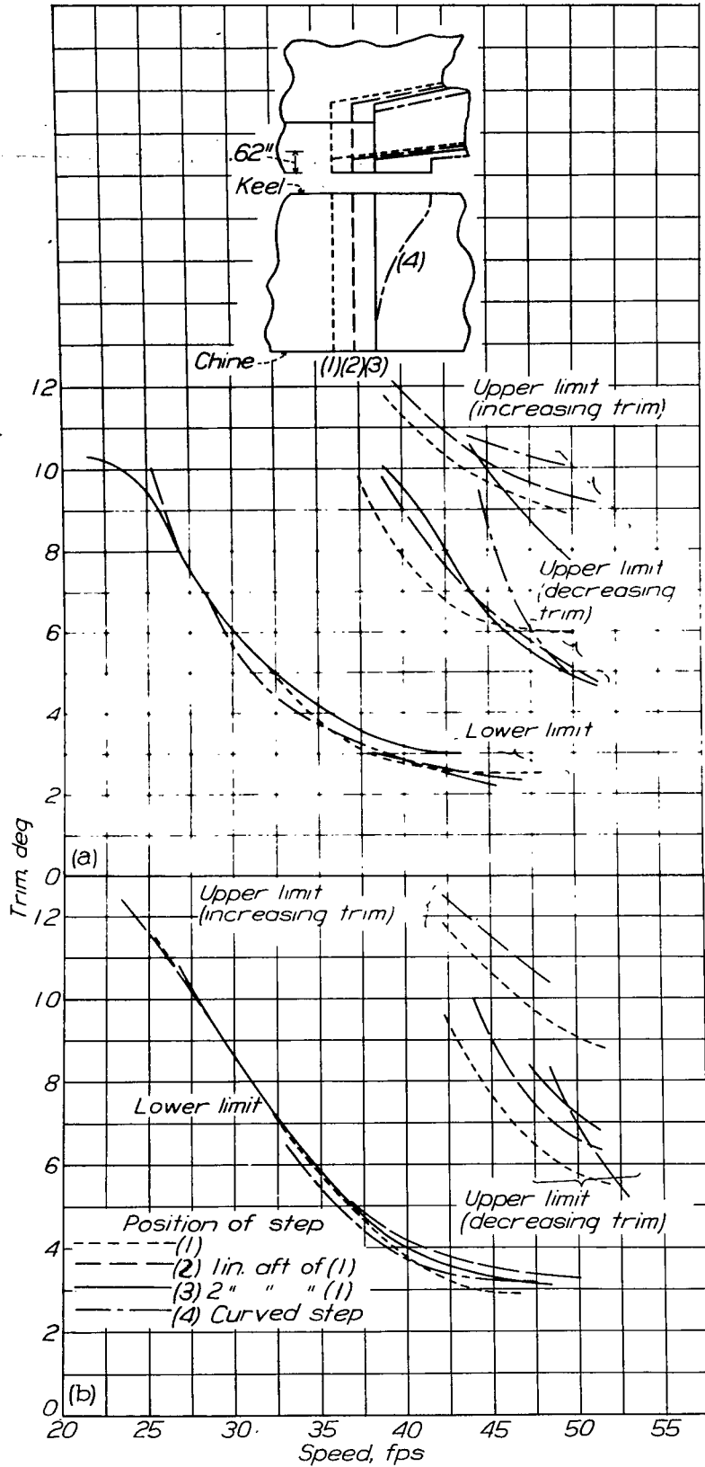
Figure 9.- Effect of position and plan form of step on trim limits of stability. Model 2, 1/8 full- size.
