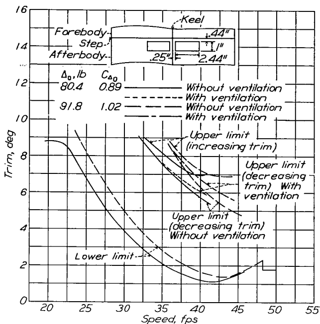
Figure 15.- Effect of ventilation on upper trim limits of stability. Model 1. 1/12 full-size
