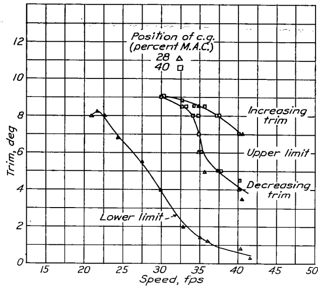
Figure 6.- Effect of position of the center of gravity on trim limits of stability. Model 7. \Delta_0 , 91.9 lb; C_{\Delta_0} , 0.86. Scale, 1/12 full size.
