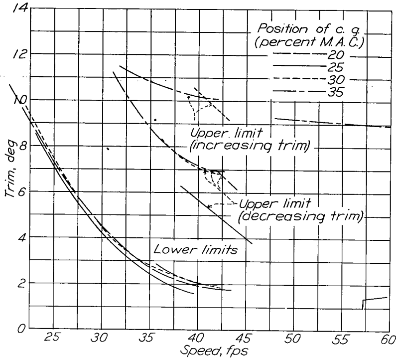
Figure 5.- Effect of position of the center of gravity on the trim limits of stability. Model 5, 1/10 full-size. \Delta_0 , 61.5 lb; C_{\Delta_0} , 0.86.
