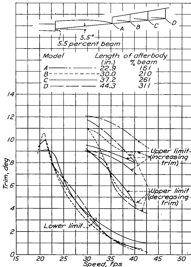
Figure 16.- Effect of afterbody length on trim limits of stability. Model 3. \Delta_0 , 91.9 lb; C_{\Delta_0} , 0.86 Scale, 1/12 full-size.
