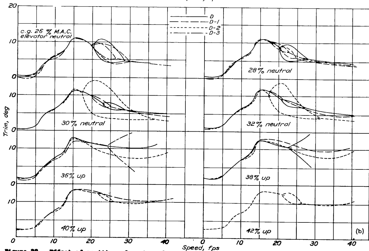
Figure 28.- Effect of position of center of gravity and location of step on trim. Model 11, 1/8 full-size. For sketch see figure 26-b. (a) \Delta_0 , 58.8; C_{A_0} , .44. (b) \Delta_0 , 77.5; C_{A_0} , .59.
