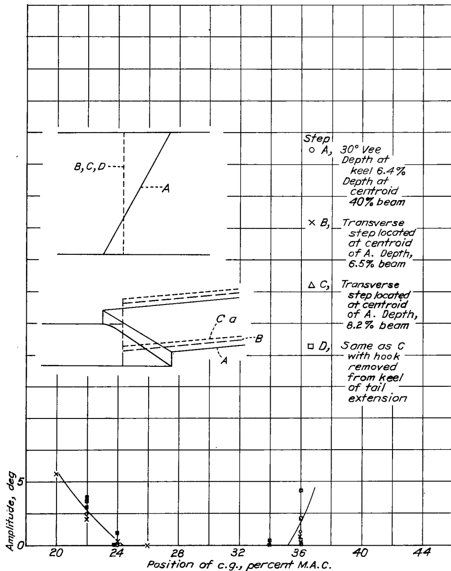
Figure 27.- Effect of plan form and depth of step on the maximum amplitude of porpoising. Model 16.
