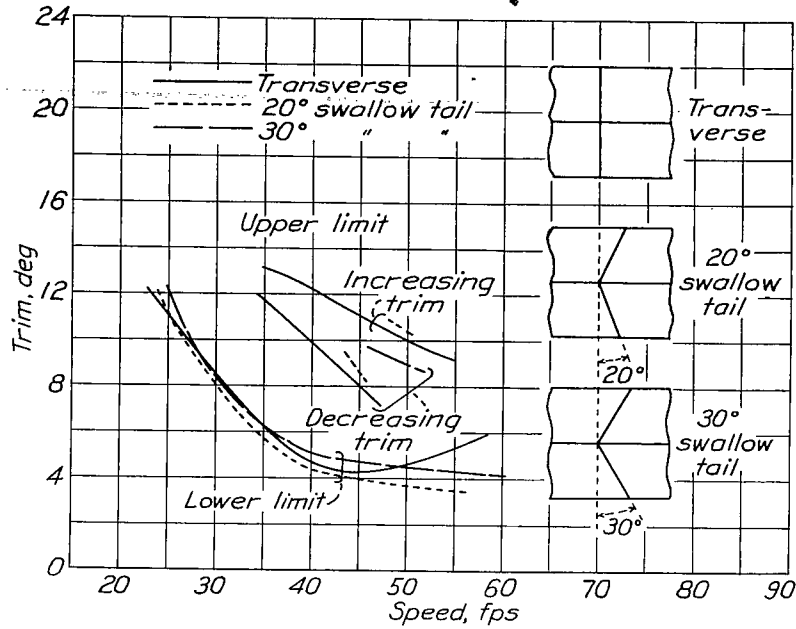
Figure 11.- Effect of plan form of step on trim limits of stability. Model 6, 1/5 full-size. \Delta_0 , 63.4 lb; C_{\Delta_0} , 1.01.
