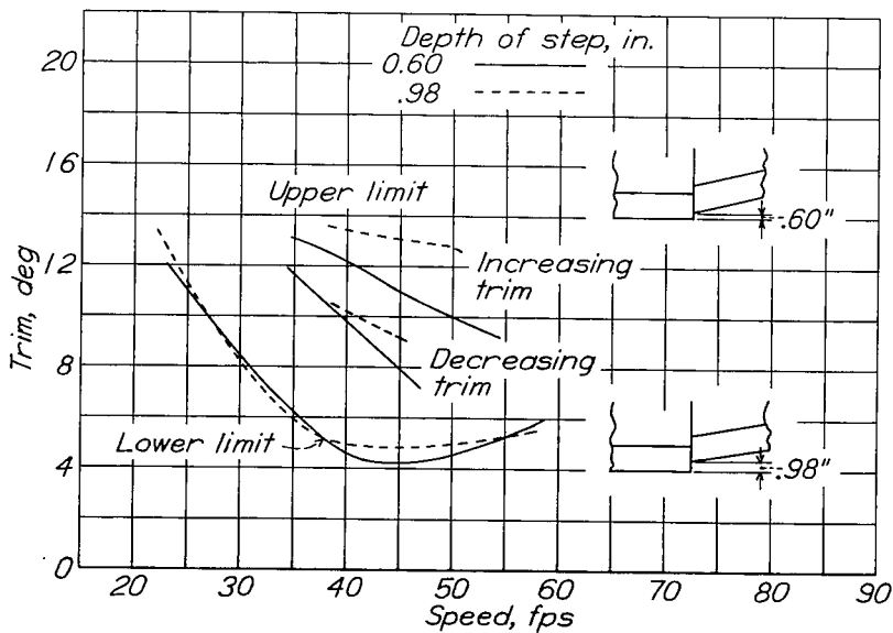
Figure 7.- Effect of depth of step on trim limits of stability. Model 6, 1/5 full-size. \Delta_0 , 63.4 lb; C_{\Delta_0} , 1.01.
