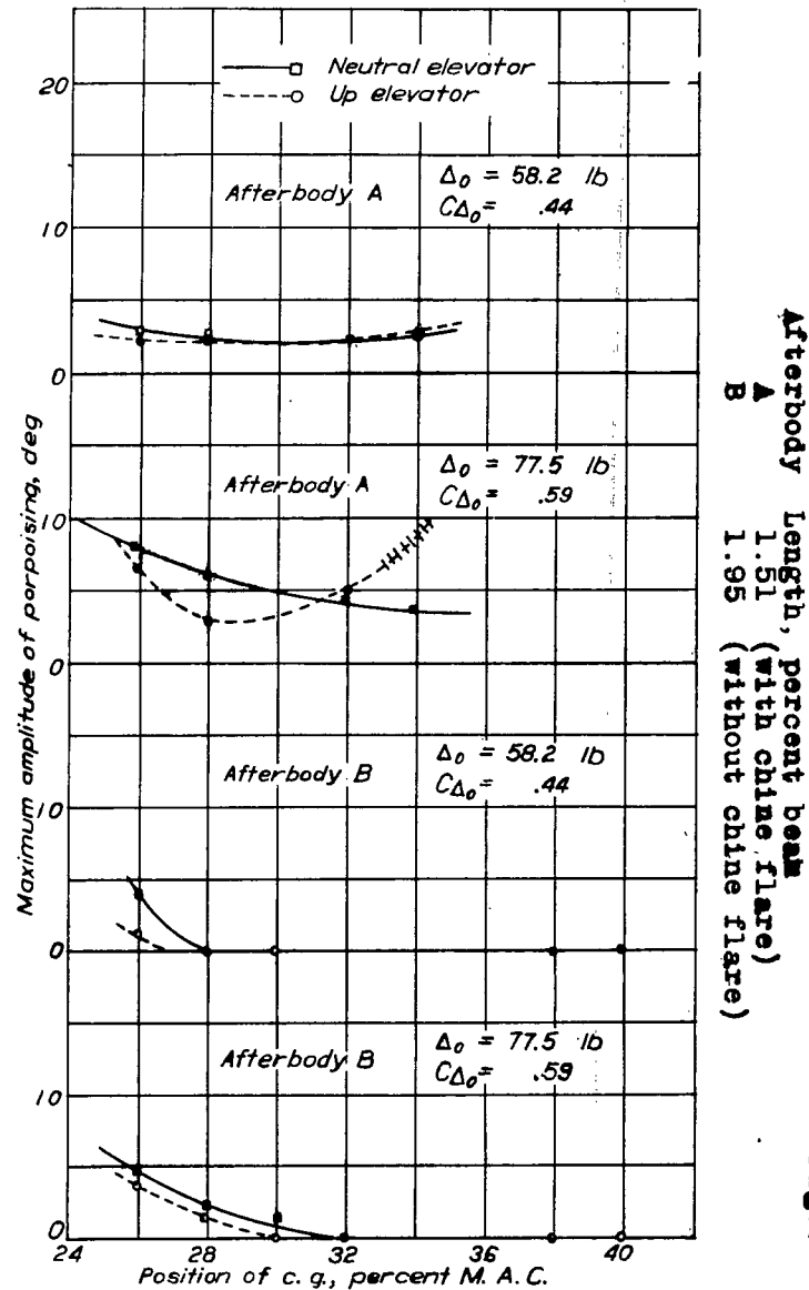
Figure 28.- Effect of length of afterbody on the maximum amplitude of porpoising. Model 17, 1/8 full-size.
