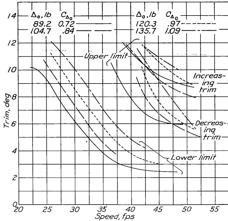
Figure 2.- Effect of gross weight on trim limits of stability. Model 2, 1/8 full-size.
