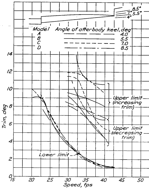
Figure 18.- Effect of increasing the angle of afterbody keel on trim limits of stability. Model 3. \Delta_0 , 91.9 lb; C_{\Delta_0} , 0.86. Length of afterbody beam = 2.61. Scale, 1/12 full size.
