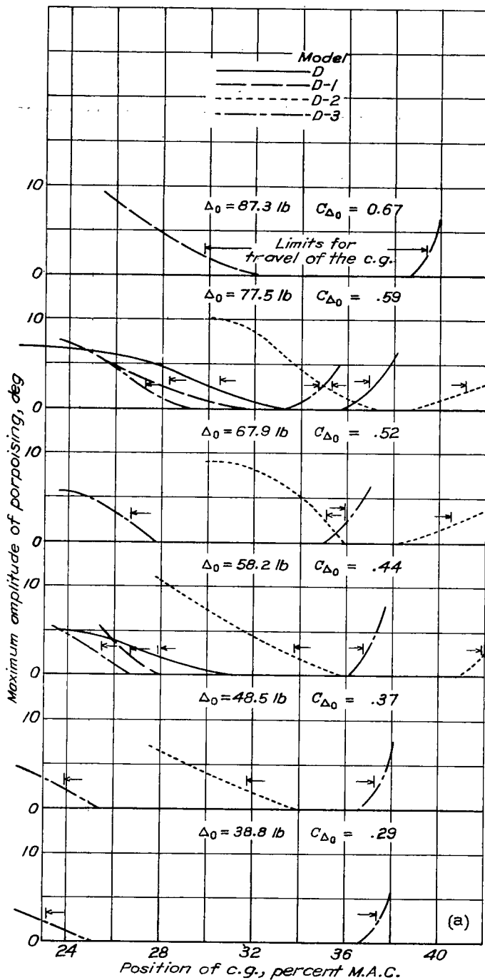
(a) On maximum amplitude of porpoising. Elevators neutral at forward positions of c.g. Elevators up at after positions of c.g.
