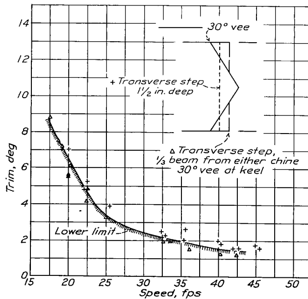
Figure 13.- Effect of plan form on lower limit of stability. Model 8. \Delta_0 , 53.8 lb; C_{\Delta_0} , 0.41. Scale, 1/8 full-size.
