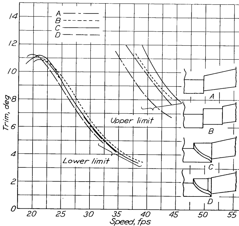
Figure 12.- Effect of plan form of step on trim limits of stability. Model 7, 1/8 full-size. \Delta_0 , 76.2 lb; C_{\Delta_0} , 1.0.
