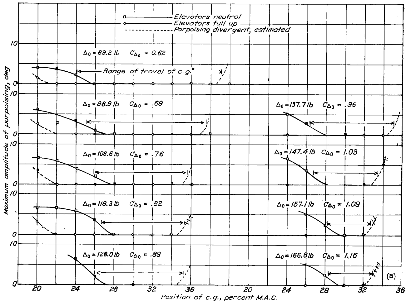
(a) On amplitude of porpoising. Model 13. Scale, 1/8 full-size.
