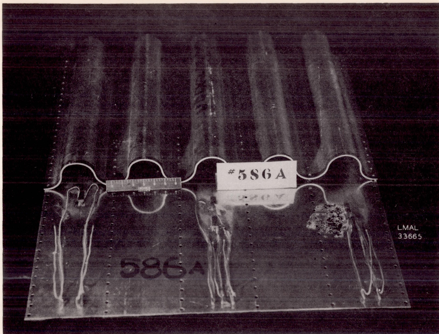
Figure 4.- Location of wire-resistance-type strain gages under the corrugated sheet.
