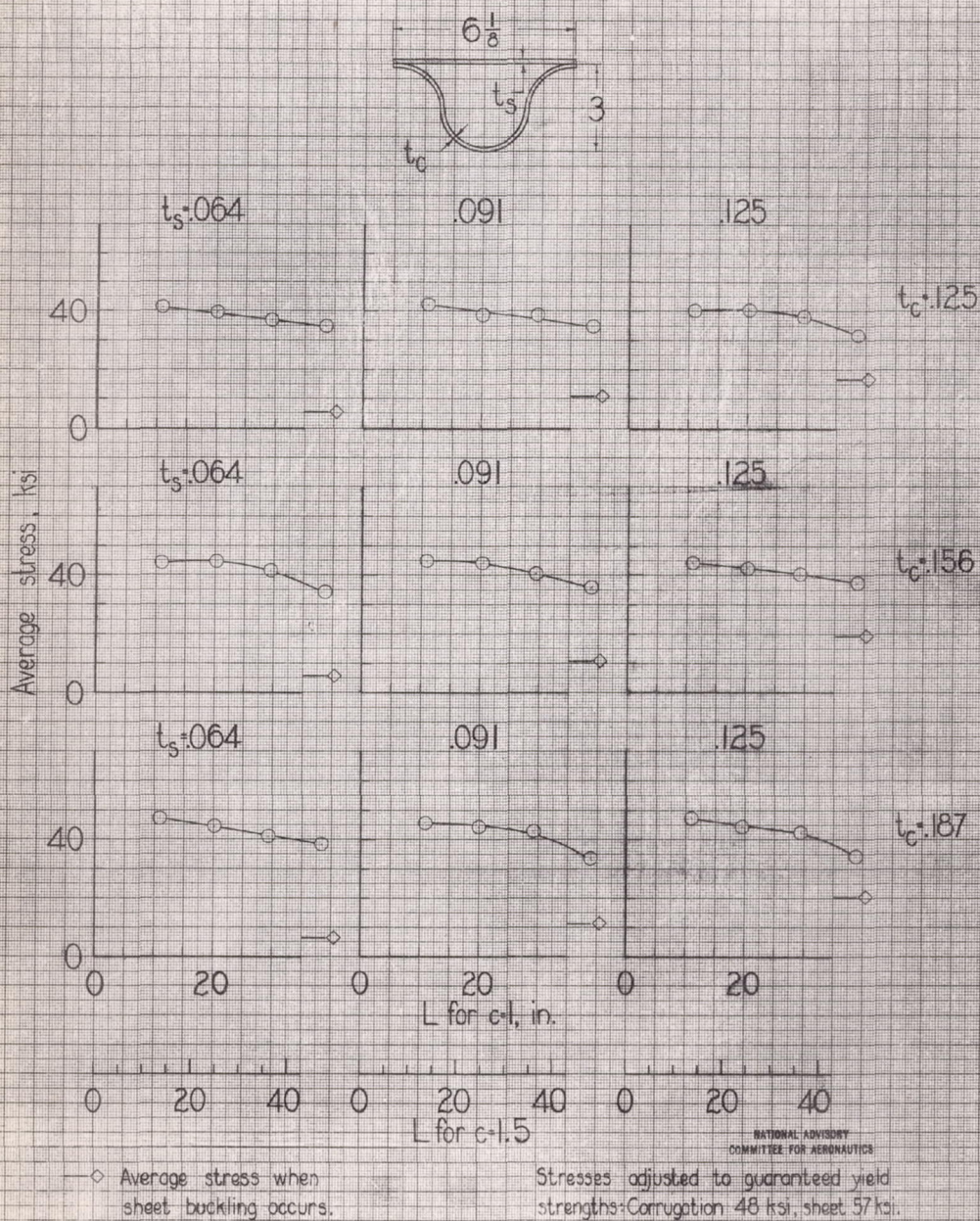
Figure 6.-Strength of panels stiffened with corrugated sheet. b_c = 3 in. b_r = 6\frac{1}{8} in.
