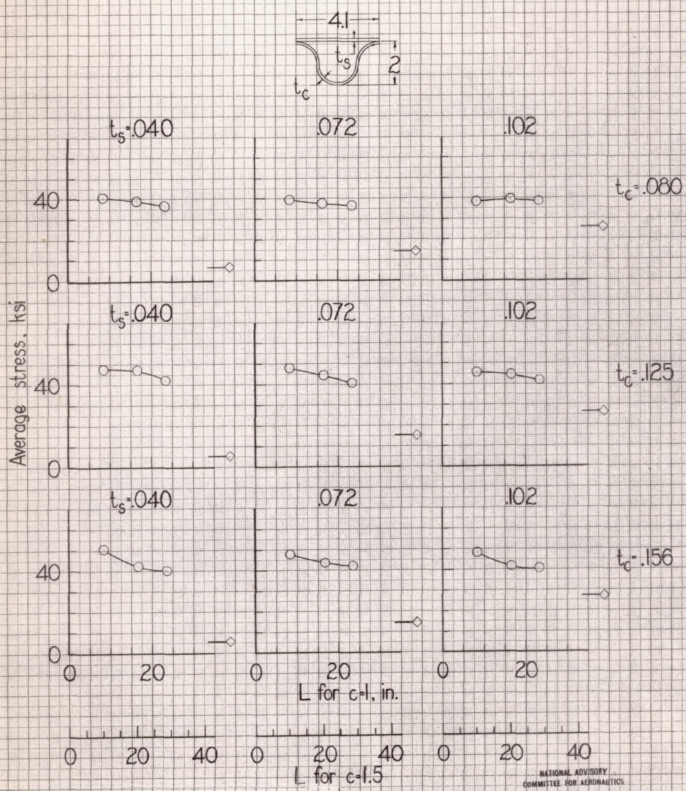
Figure 5.-Strength of panels stiffened with corrugated sheet. b_c = 2 in. b_r = 4.1 in.
