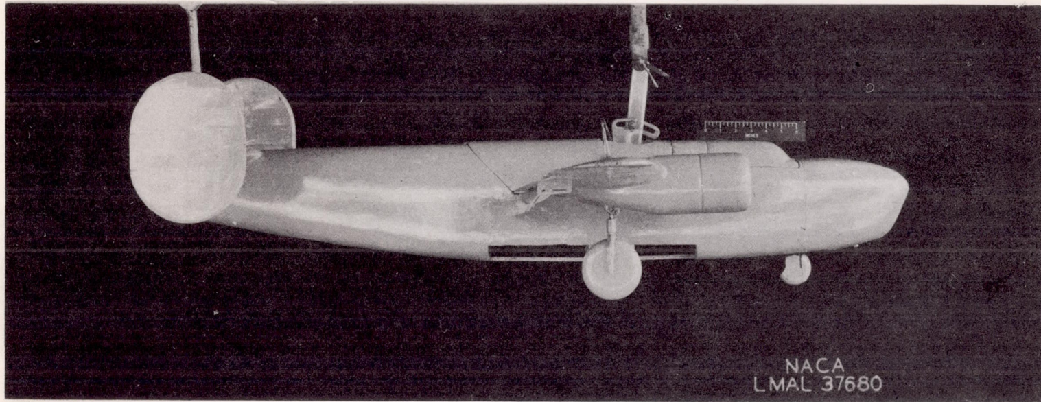
(b) Side view. The nose wheel is notched so that it can fall back partially into the open wheel compartment.
