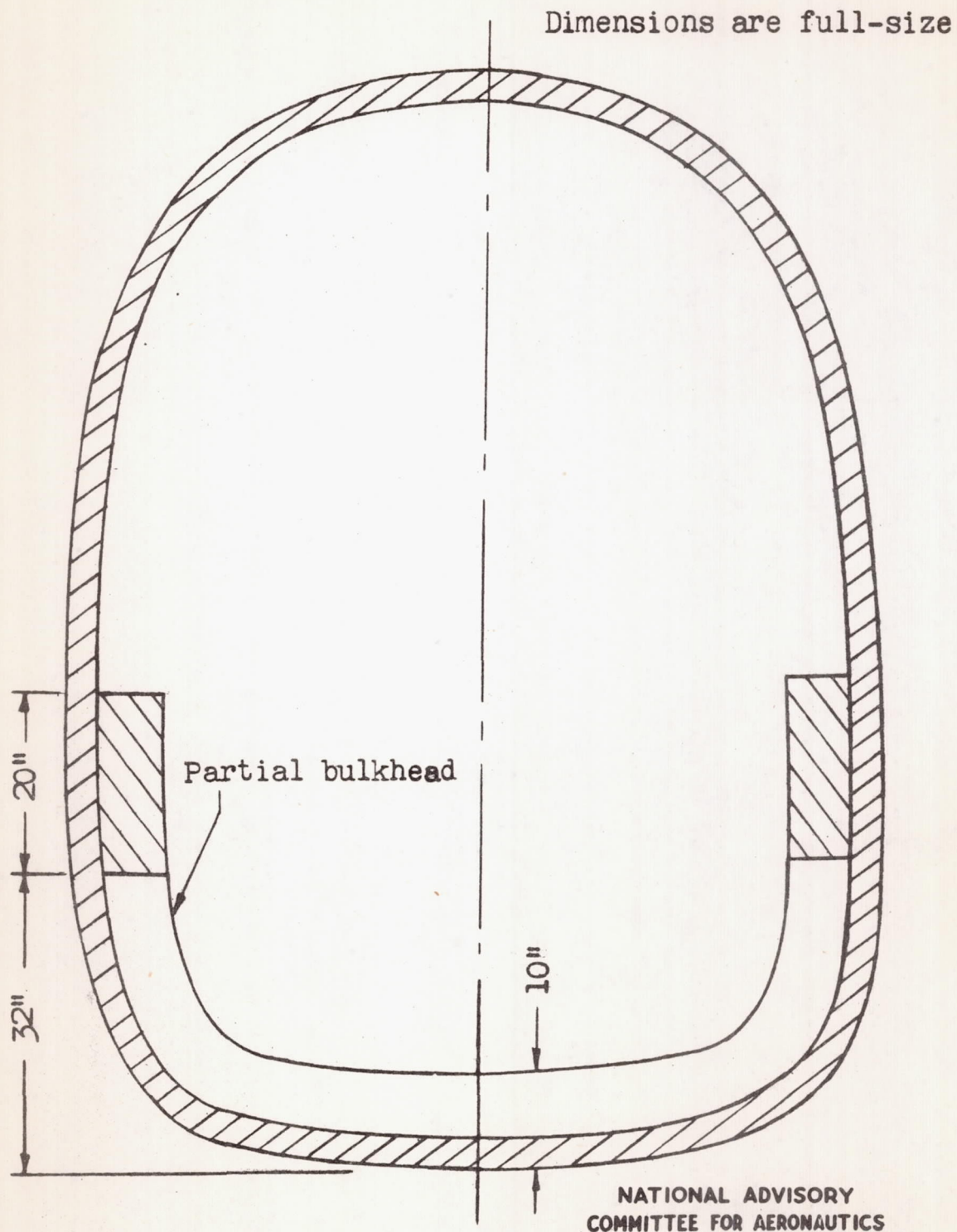
Figure 7.- Drawing showing partial bulkhead in fuselage just aft of bomb-bays on a model of an Army B-24 airplane.
