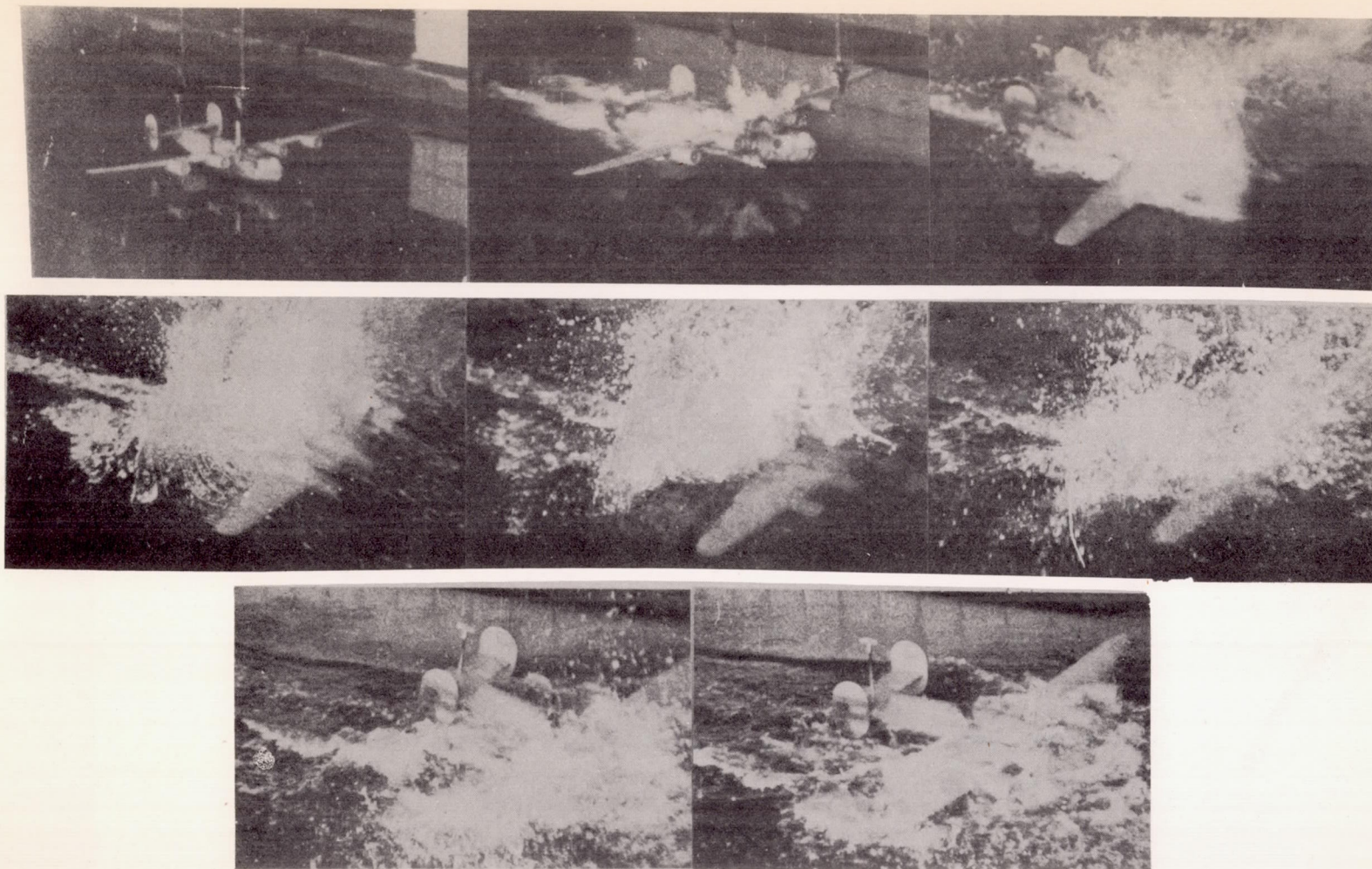
Figure 13.- Photographs at 1-second intervals, full-scale, of a ditching of a \frac{1}{16} -size model of an Army B-24 airplane. Attitude of thrust line is 1^\circ at contact; flaps down 40^\circ ; speed 120 miles per hour, full-scale. Model with bomb-bay doors removed.
