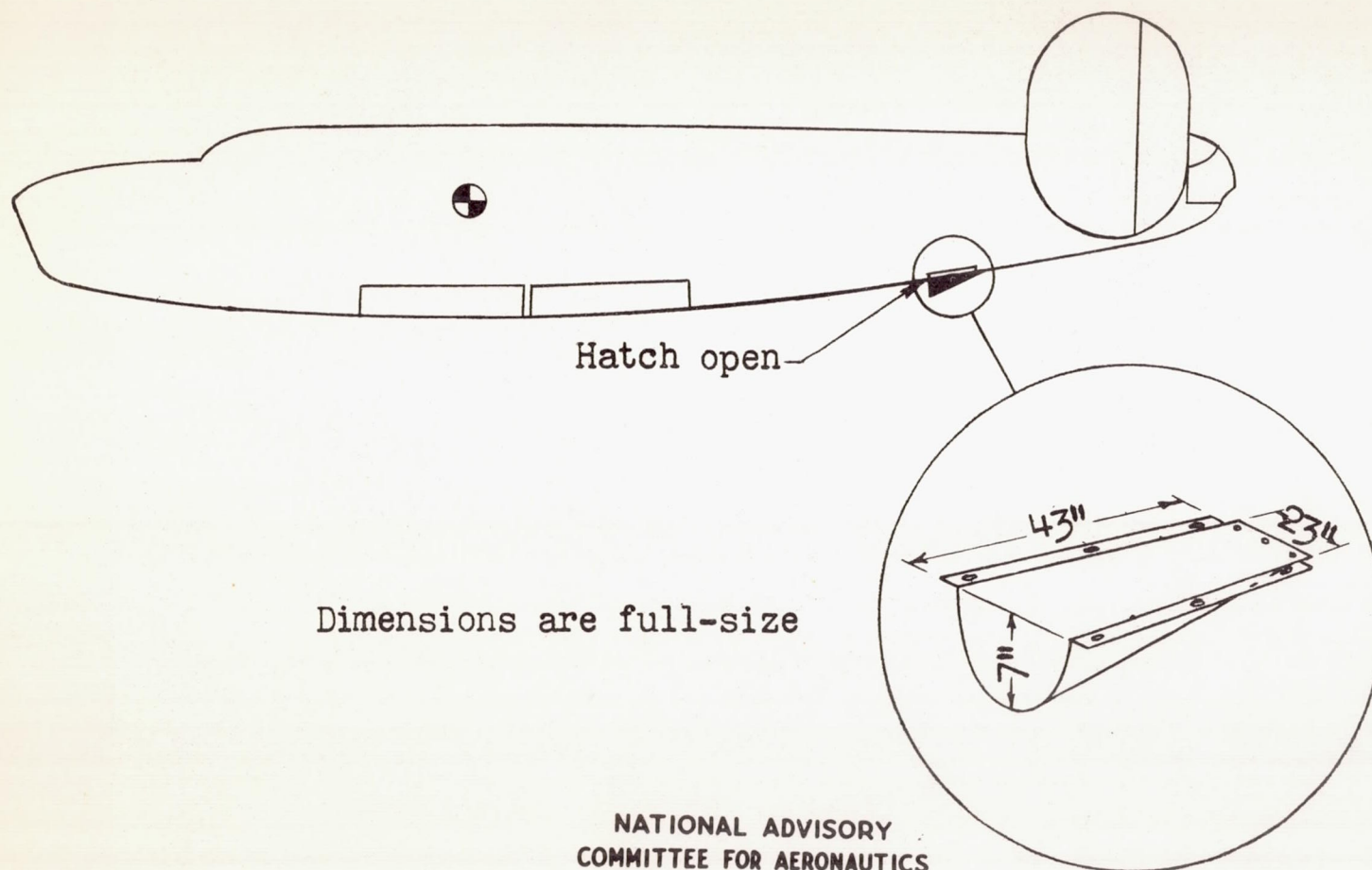
Figure 10- Drawing showing a water scoop and its location on a model of an Army B-24 airplane.
