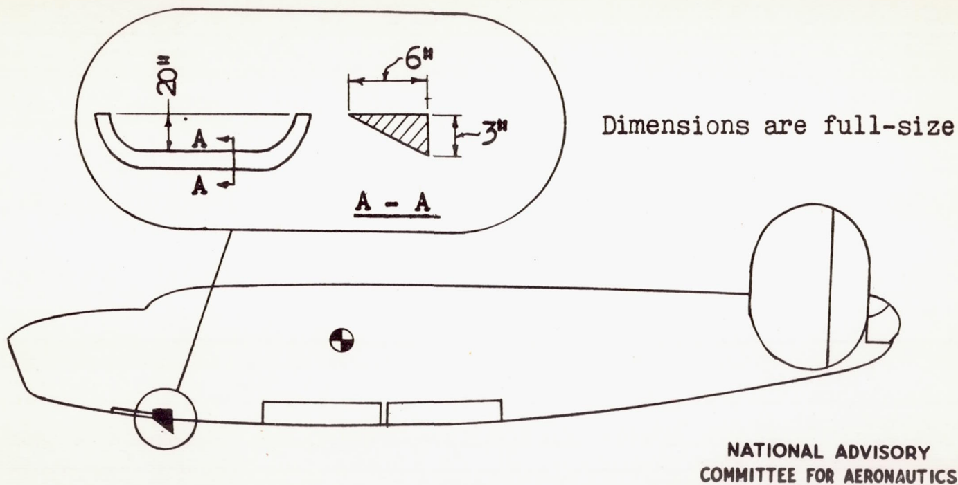
Figure 9.- Drawing showing a triangular hydrospoiler and its location on a model of an Army B-24 airplane.
