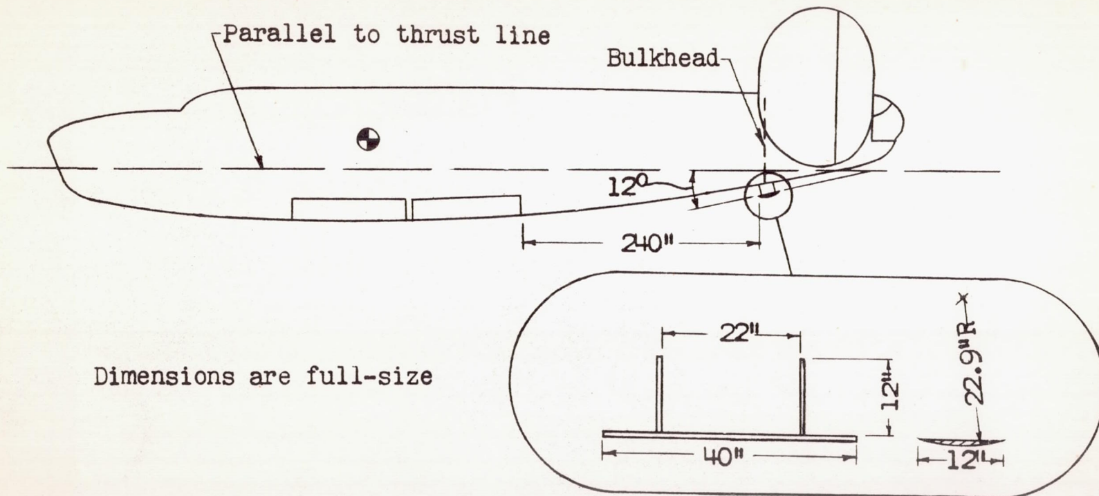
(a) 40-inch hydrofoil
