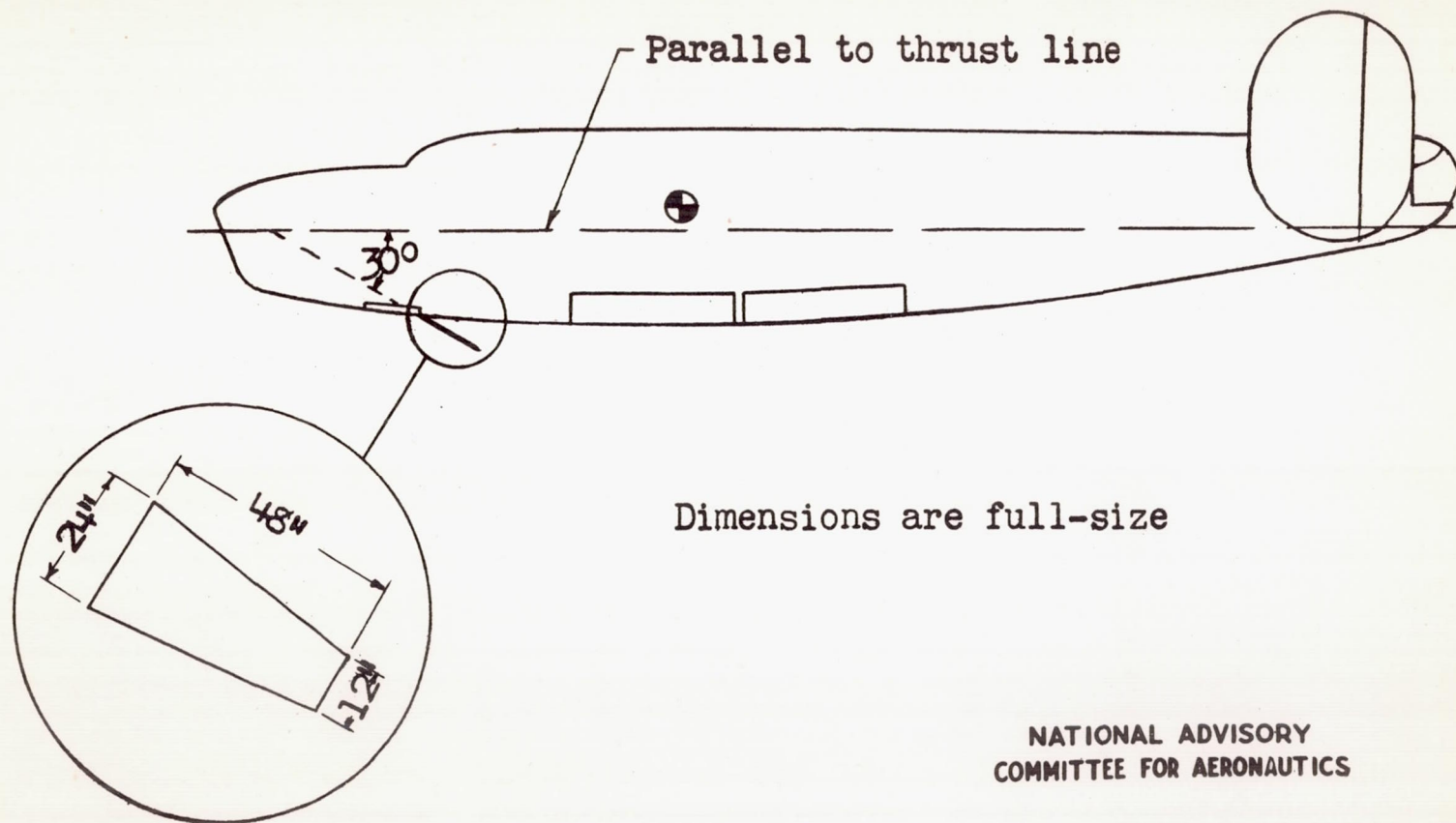
Figure 8.- Drawing showing a trapezoidal hydroflap and its location on a model of an Army B-24 airplane.
