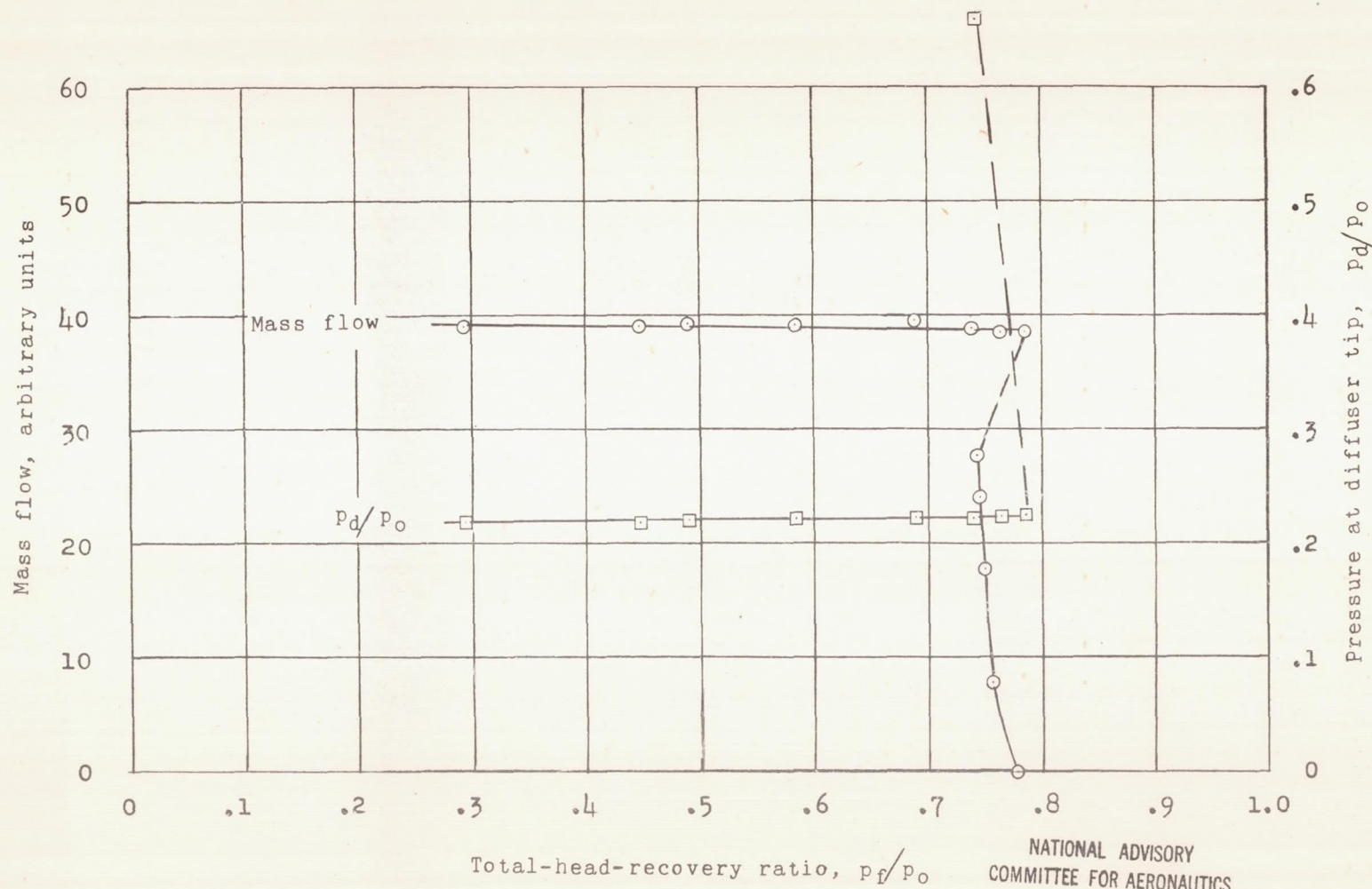
Figure 7.- Performance of a supersonic diffuser during typical test.
