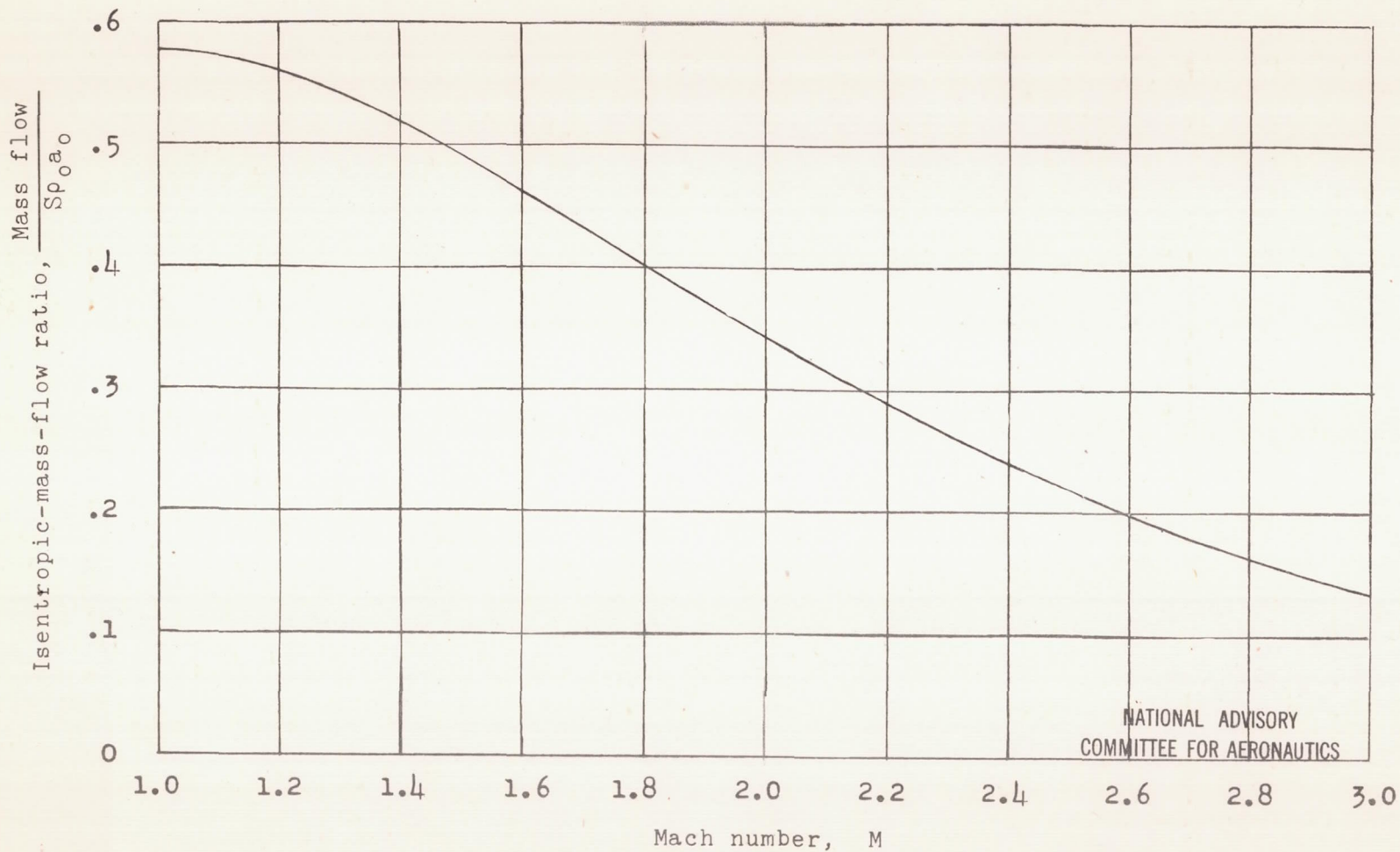
Figure 1.- Isentropic-mass-flow ratio as a function of Mach number. Mass flow measured through area S at Mach number M ; \rho_0 , density; a_0 , speed of sound at initial stagnation conditions.
