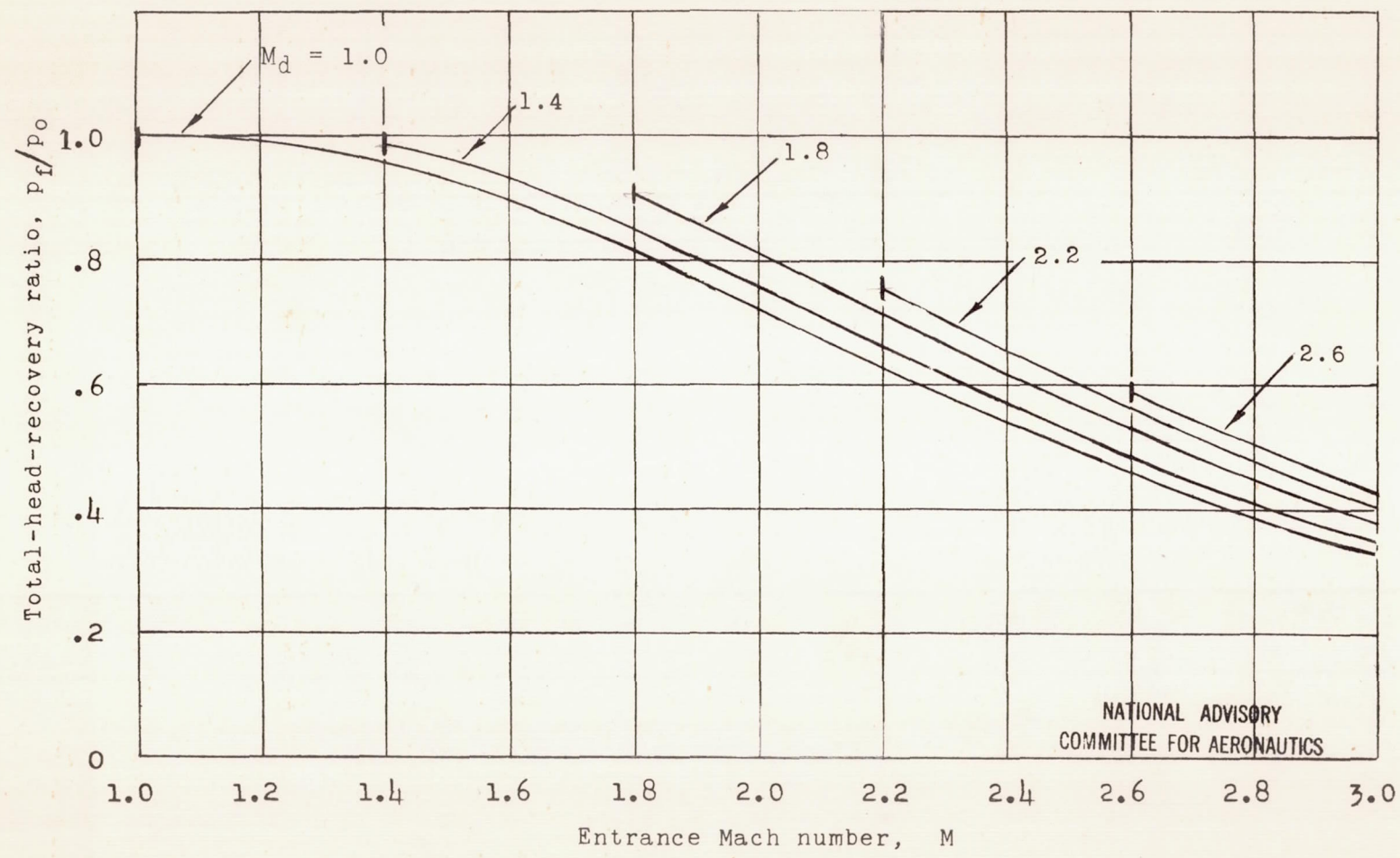
Figure 4.- Theoretical performance by approximate method of five supersonic diffusers with maximum theoretical contraction ratios corresponding to minimum starting or design Mach numbers of 1.0, 1.4, 1.8, 2.2, and 2.6. Vertical lines indicate design Mach numbers.
