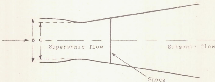
(b) Stable supersonic diffuser flow. (For circular diffuser \frac{b^2}{c^2} = C_R , where C_R is contraction ratio.)
