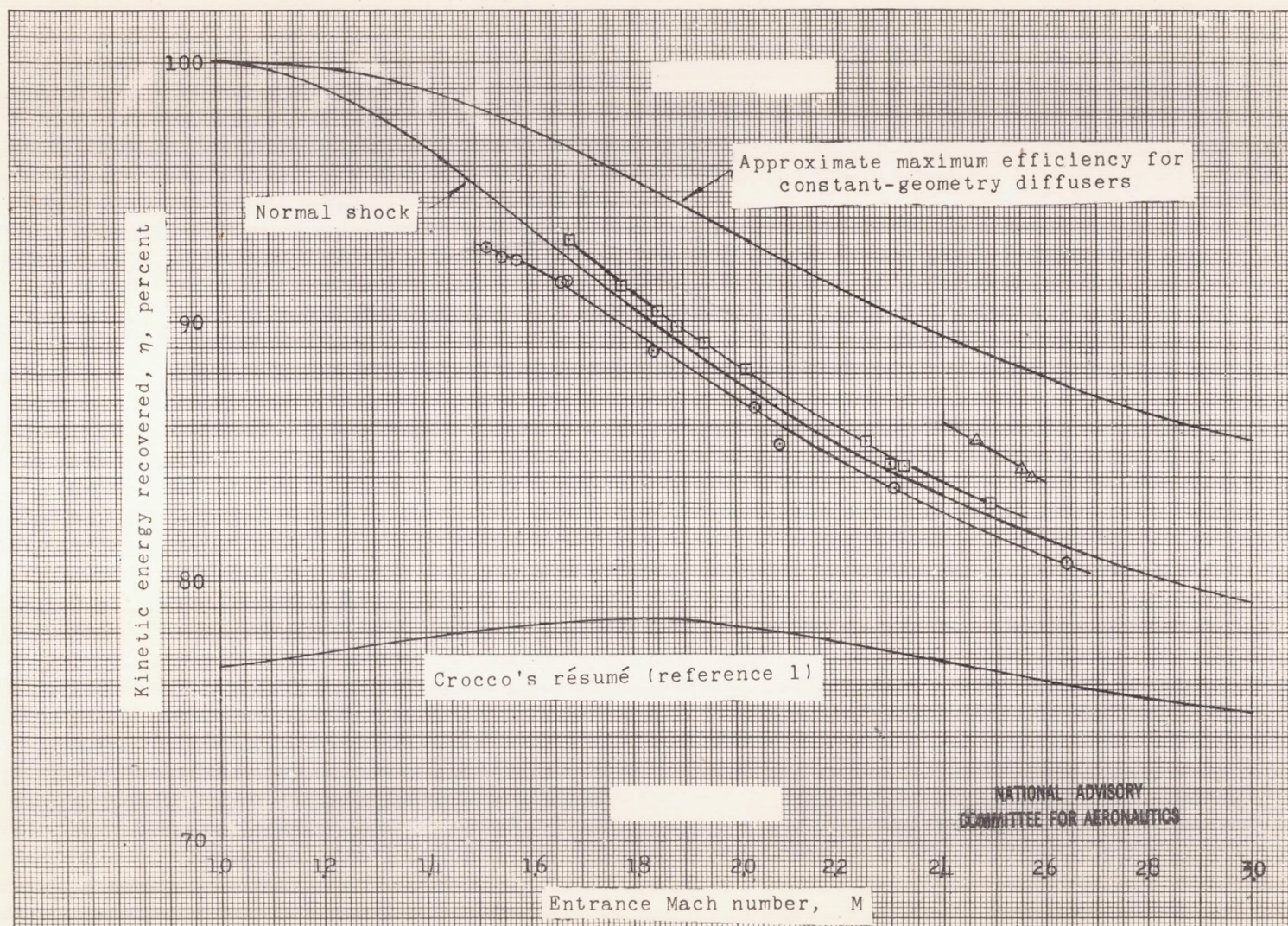
Figure 10.- Comparison on an energy basis of diffusers tested with theoretical results and with results of former experiments. Experimental points are from same tests as those shown in figure 8.
