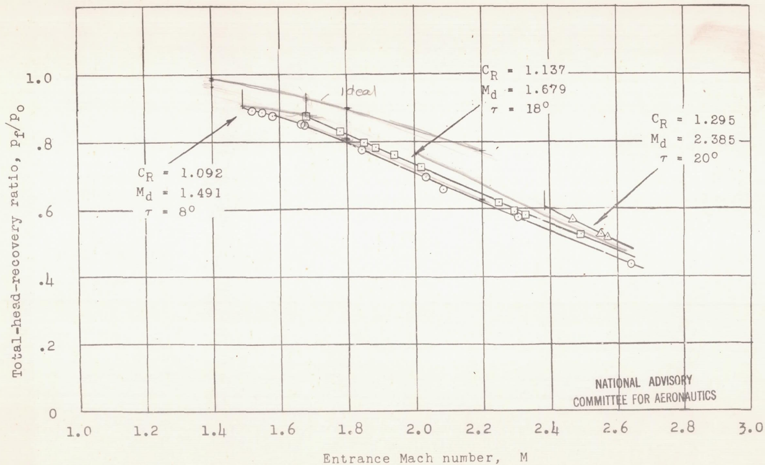
Figure 8.- Performance of the three diffusers shown in figure 6 with exit-cone angles of 3^\circ . \tau , entrance-cone angle.
