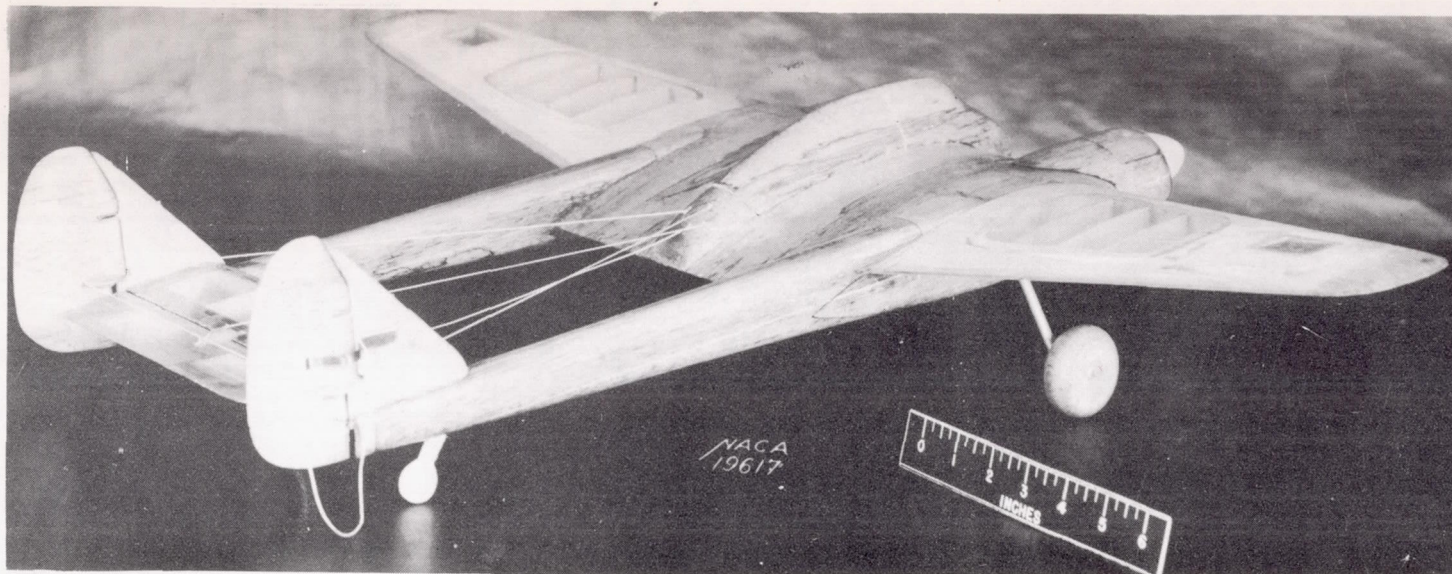
Figure 4.- Three-quarter rear view of 1/25-scale model of Burnelli XB-AB-3 airplane.
