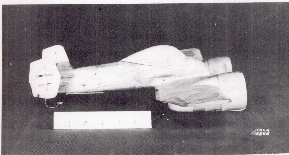
Figure 3.- Side view of 1/22-scale model of Grumman XF5F-1 airplane.
