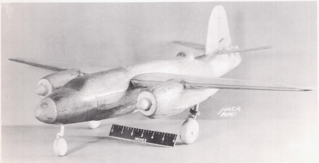
Figure 6.- Three-quarter front view of 1/25-scale model of Grumman XP-50 airplane.
