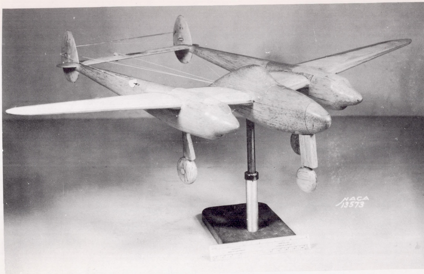
Figure 1.- Three-quarter front view of 1/20-scale model of Lockheed YP-38 airplane.
