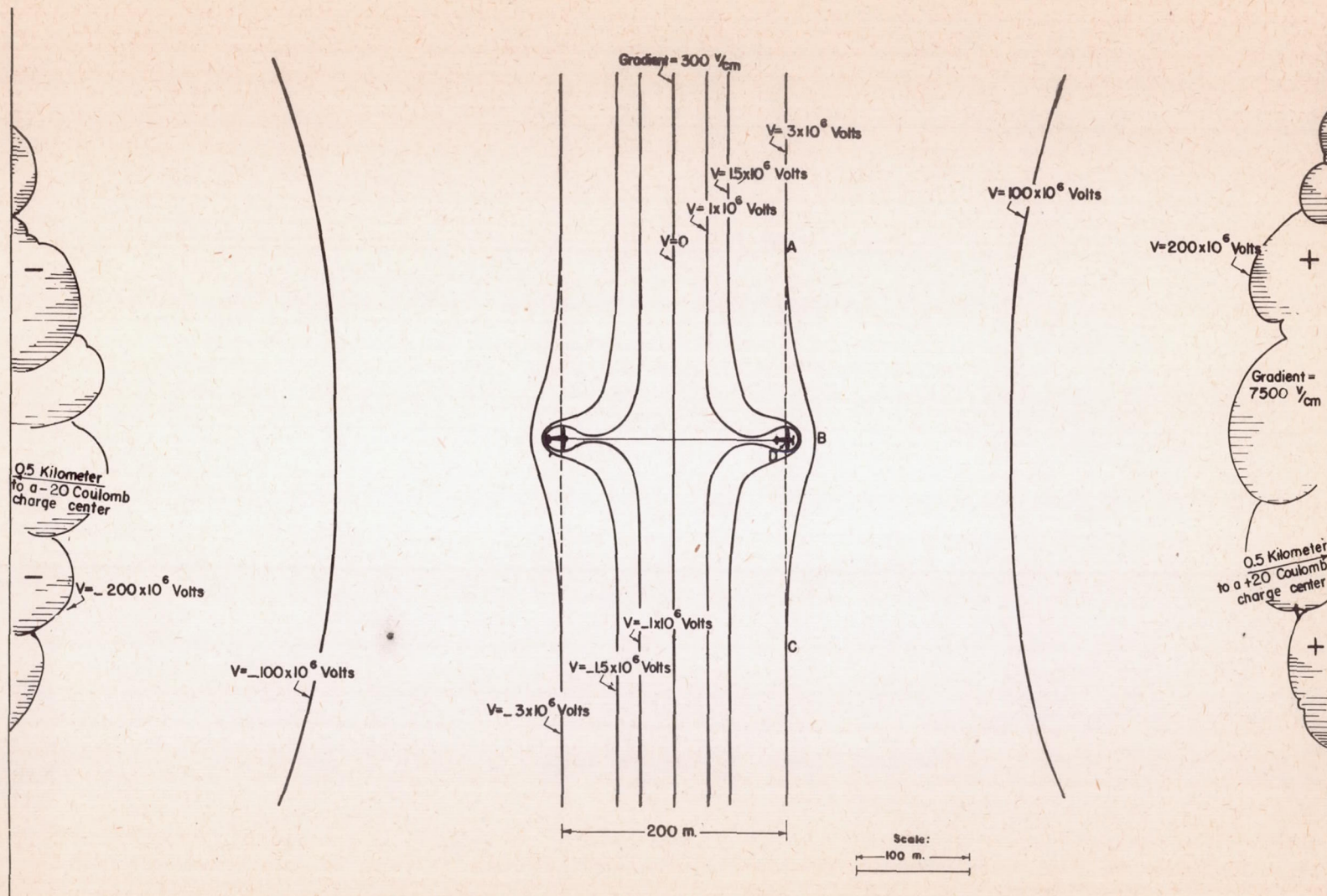
FIGURE 17.-DISTORTION OF ELECTRIC FIELD OF CLOUDS BY GLIDER TOW
