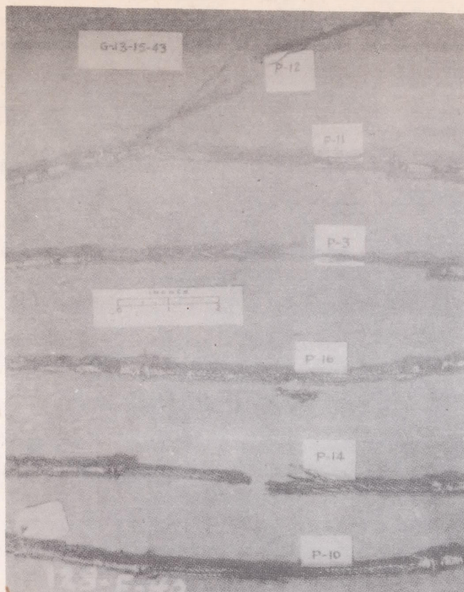
Figure 12.- Steel aircraft cable samples after test with 1000-ampere surge followed by 30-coulomb arc while under mechanical tension. Unprotected samples P-12, P-3, and P-14, respectively 1/16" , 3/32" , and 1/8" in diameter, all failed though tension applied was only 100 pounds. Samples P-11, P-16 and P-10 of same diameter respectively as the others and subjected to 600 pounds tension did not fail because protected by metal braid and thin layer of insulation.
