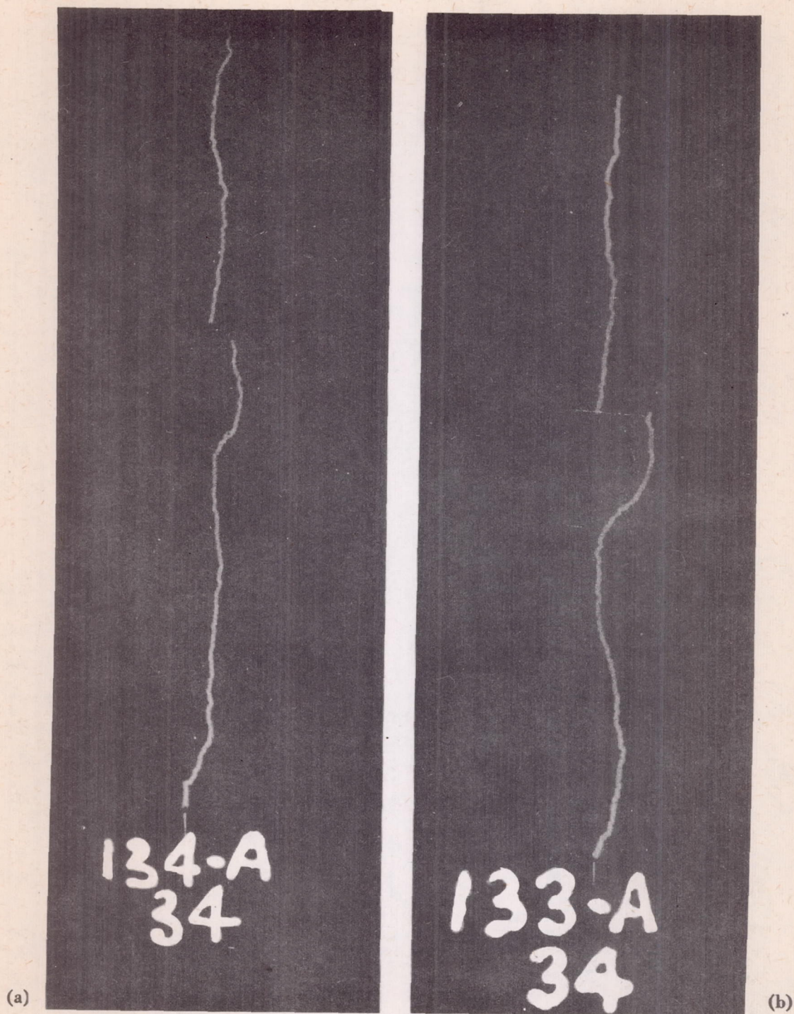
FIGURE 11.—Surge discharge to model of tow. (a) EAST CAMERA. (b) NORTH CAMERA. This discharge strikes from the upper rod electrode to the metal towline and leaves by left wing tip of the towing plane to continue to the lower electrode. Distance between electrodes, 8 feet. The thin lines are the paraffined threads which supported the model.
