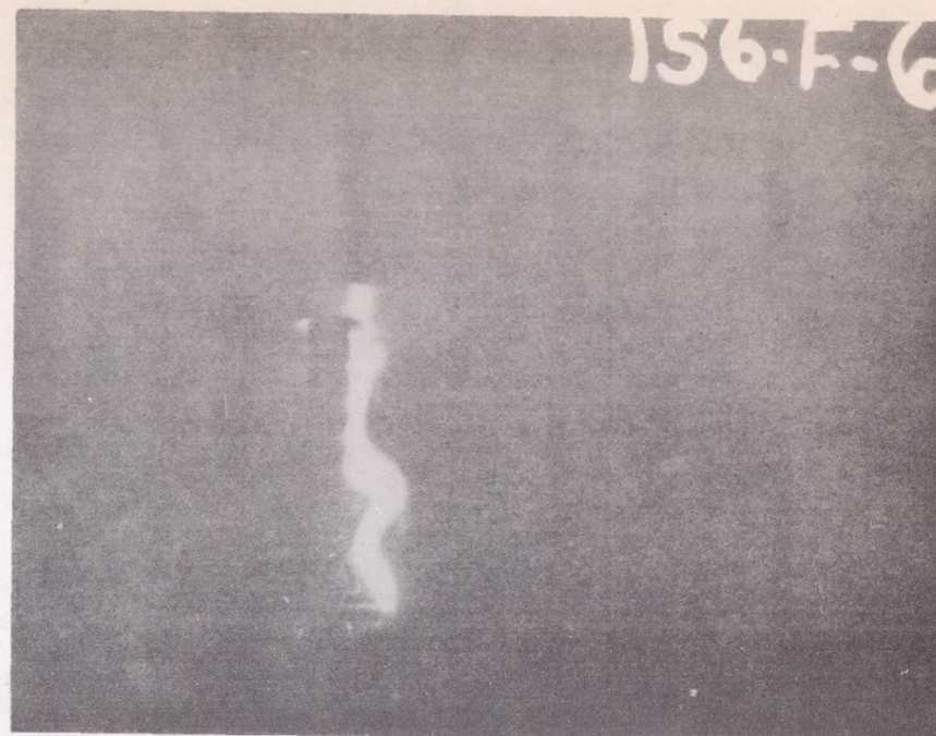
Figure 10.- Sixty-cycle, 3-ampere arc along aquadag-treated 13/16-inch nylon rope, showing action of metal arcing ring in keeping discharge away from rope at lower end.
