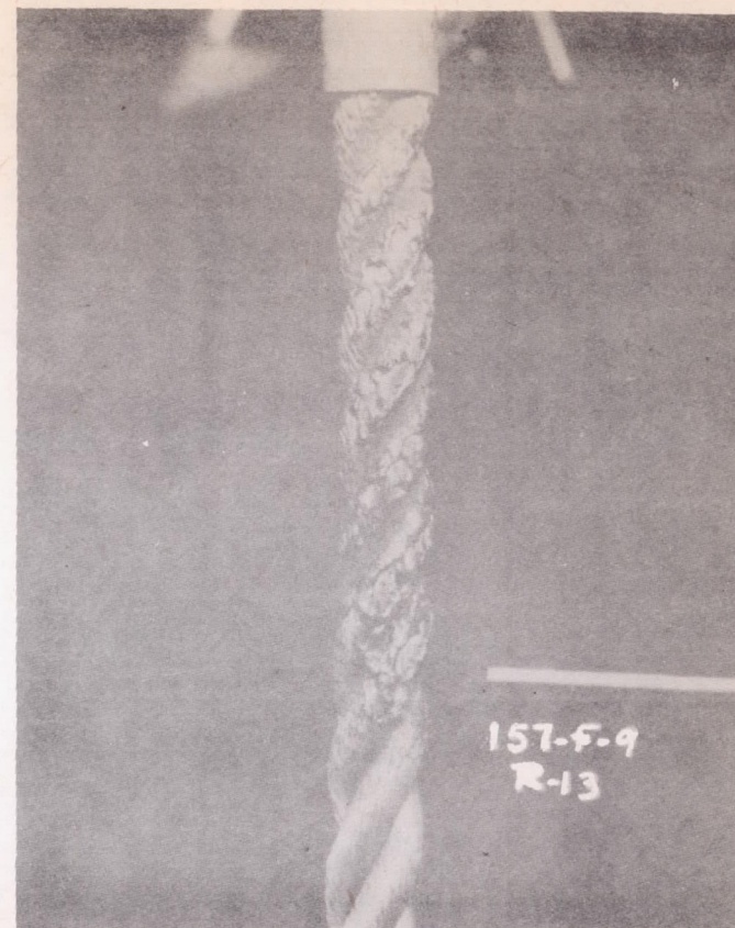
Figure 15.- Damage produced on 13/16-inch nylon rope, treated with aquadag so as to have 200 ohms per cm, after a 3-ampere a-c arc had struck and restructured over its surface 5 times from the rod electrode to the upper metal sleeve during a total exposure of 15 seconds.
