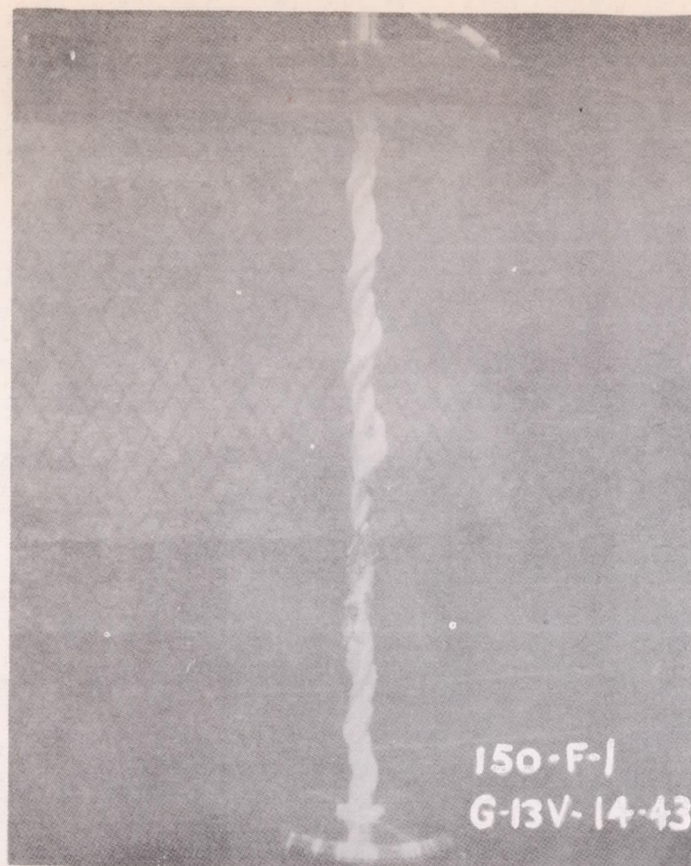
Figure 36.- Condition of 13/16-inch nylon rope initially soaked in distilled water, after 30 ma had passed for 100 seconds. Load = 650 pounds.
