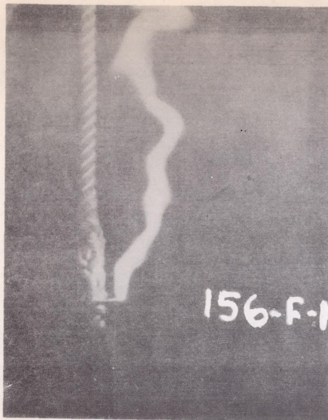
Figure 9.- Sixty-cycle, 4-ampere arc rising along dry, untreated 13/16-inch nylon rope; showing action of metal arcing ring in keeping discharge away from textile. No visible damage resulted.
