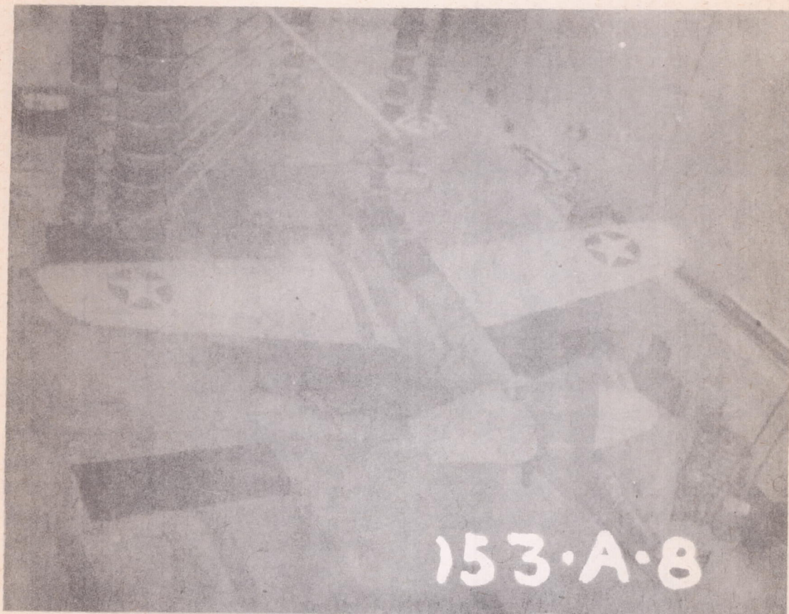
Figure 27.- Fairchild PT-19-A airplane suspended in High-Voltage Laboratory for corona measurements. The total corona current from the airplane was measured by a milliammeter enclosed in the cylindrical shield visible between the two toroidal shields
