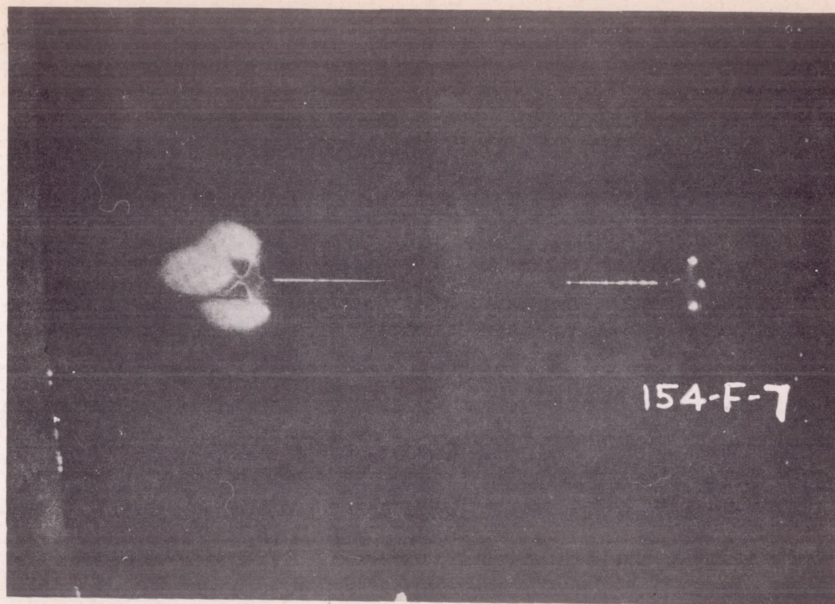
FIGURE 41.—Photograph of model tow showing, qualitatively, corona discharges from aircraft and towline. Wing span of metal models 2 inches, towline 0.005-inch diameter, 16 inches long; metal plates simulating clouds were charged to +70,000 volts (at right) and -70,000 volts (at left) relative to ground.
