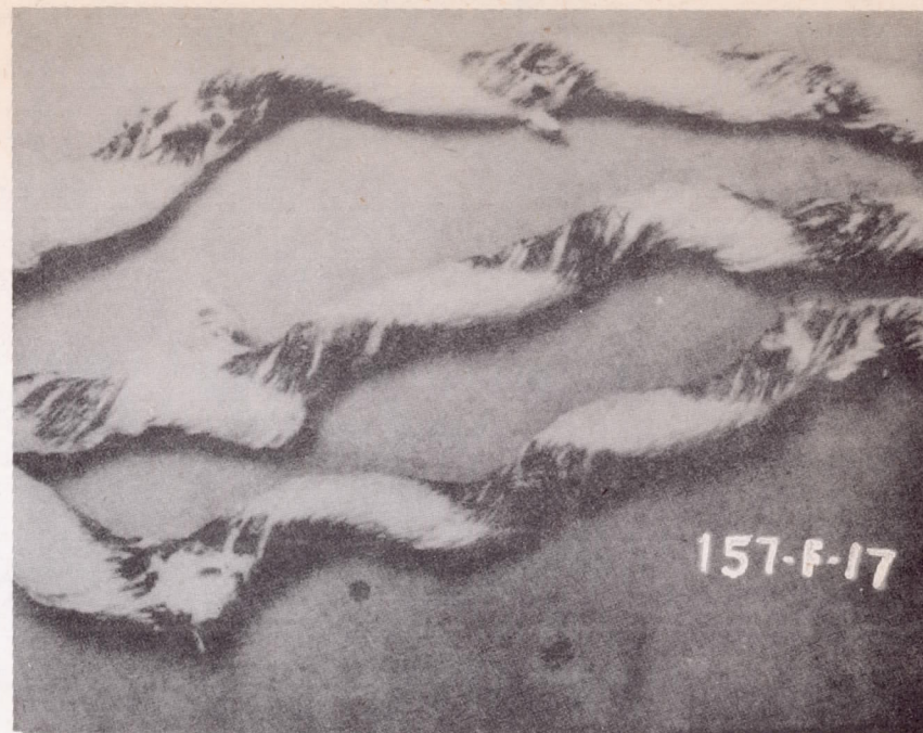
Figure 35.- Condition of 13/16-inch nylon rope after high-current discharge (25,000 amperes) had volatilized the metal helix embedded in center of rope. Strands have been untwisted to show scorching of inner fibers and presence of nodules of metal.
