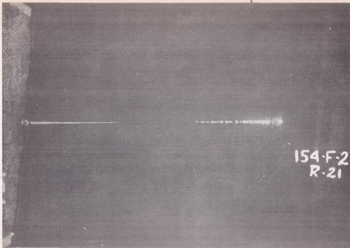
FIGURE 29.—Corona discharge from fine (No. 36) wire stretched between two 1.6-cm. spheres and placed in electric field between two large metal plates perpendicular to the wire. Plates were charged to +70,000 volts at the right and -70,000 volts at the left. Note beaded character of corona from induced negatively charged end, and the smooth positive glow. Exposure 15 minutes at f4.5 Eastman Tri X Pan.
