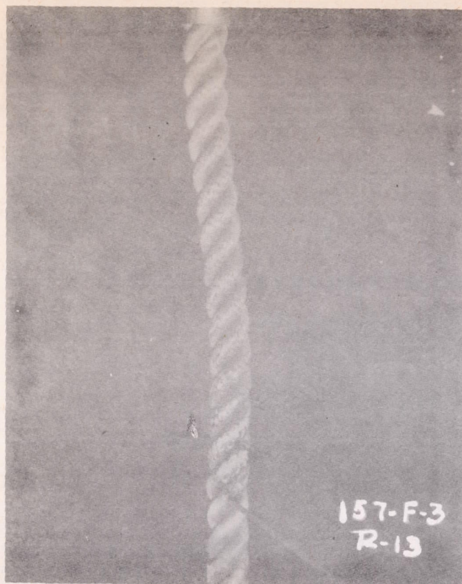
Figure 14.- Damage resulting from arc shown in figure 13, after arc had ceased and restructured three times for a total application of 14 seconds. The scorching and melting of the surface is confined to a thin layer and is not concentrated opposite the rod electrode.
