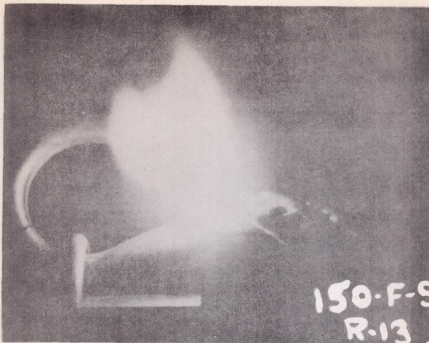
Figure 7.- 30-ampere d-c arc concentrated for 1 second between thimble and #10 copper wire. Camera shutter open during full duration of arc.
