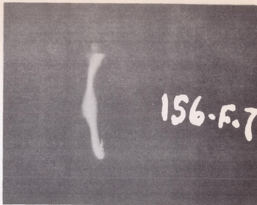
Figure 4.- Sixty-cycle, 3-ampere arc along the surface of 13/16-inch nylon rope which had been treated with aquadag to give a resistance of 2000 ohms per cm. Length of specimen 15 cm. Exposure 0.01 sec.
