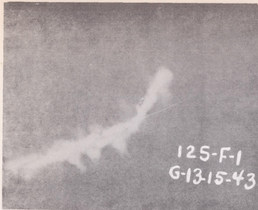
Figure 1.- A transient discharge striking and following along a wet, 1/4-inch cotton sash cord, 2 feet long. Crest current 25,000 amperes, duration about 40 microseconds. The cord showed no damage after the stroke.
