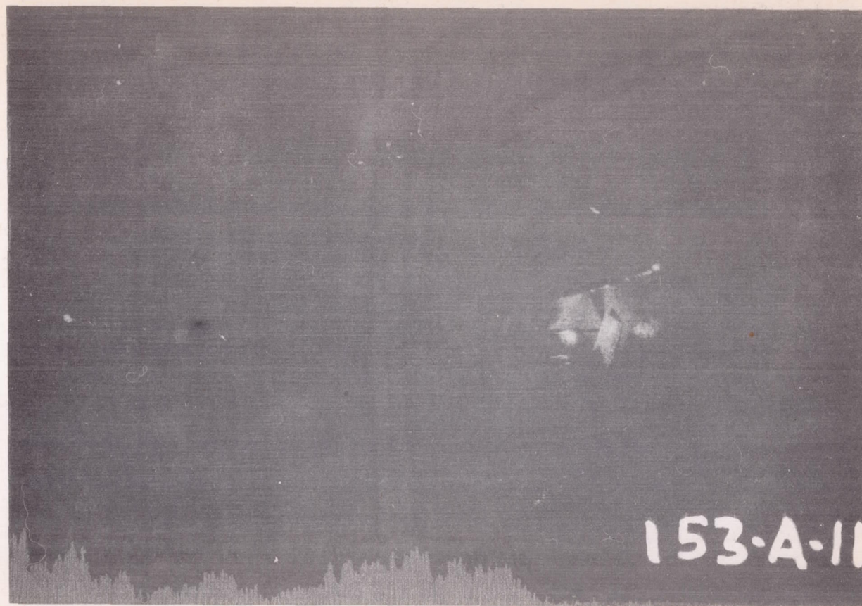
FIGURE 28.—Corona discharge from Fairchild PT-19-A airplane when charged to -1,200,000 volts. The spreading of the spots is the result of a slight swinging of the craft by air currents during the course of the 10-minute exposure.
