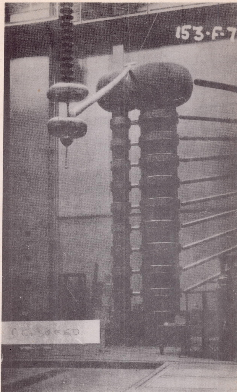
Figure 25.- The string of suspension insulators at the top of the photograph supports the two toroidal shields and the cylindrical shield below, which encloses the microammeter. The tube hanging down from this carries the polished 5-cm sphere from which the discharge point protrudes. The metal floor is the plane electrode. The lead, 6-inches in diameter and 42-feet long, connects the toroid with the 1.4-million volt X-ray generator. This lead is much foreshortened in the photograph.
