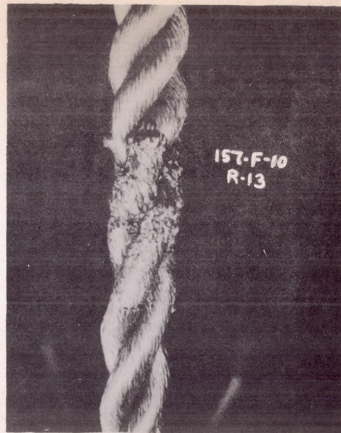
Figure 40.- Detail of part of specimen B after test up to 240 ma. In spite of this local melting under the electrode, the specimen could hold the load of 3500 pounds.
