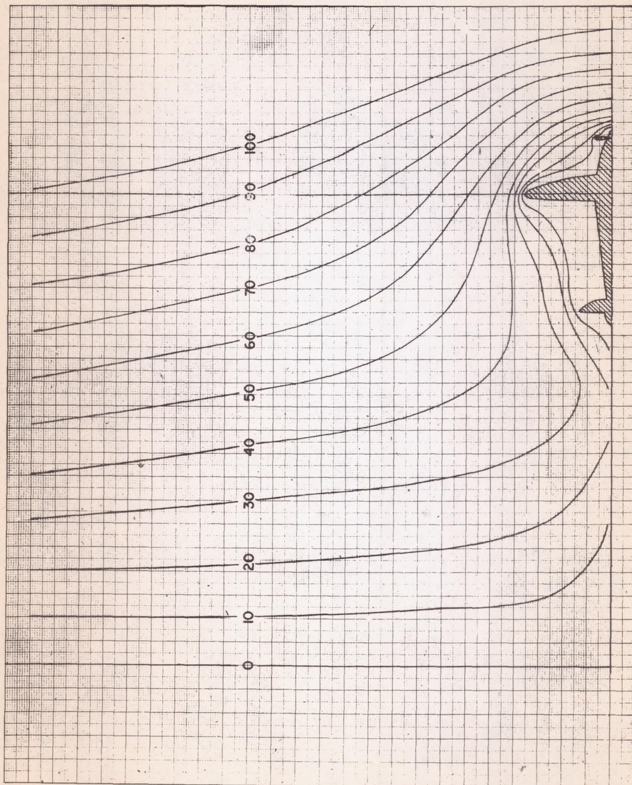
FIGURE 18.-ELECTRIC FIELD AROUND TOW PLANE
