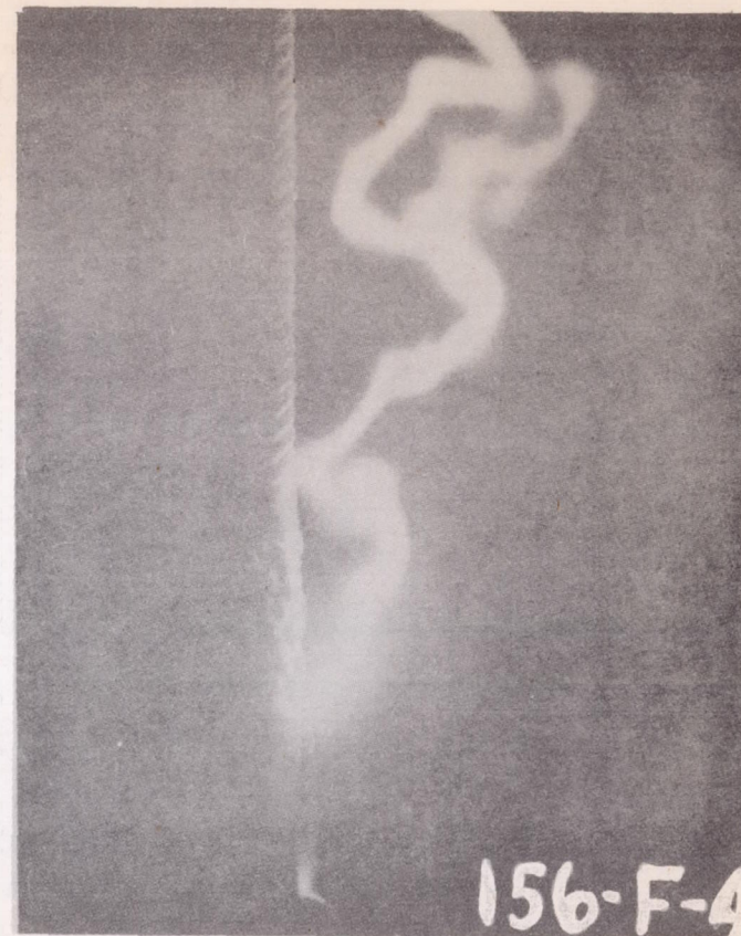
Figure 2.- Sixty-cycle, 4-ampere arc rising along a dry, untreated nylon rope, 13/16-inch diam. Exposure of 0.01 second shows illumination during parts of two half-cycles.
