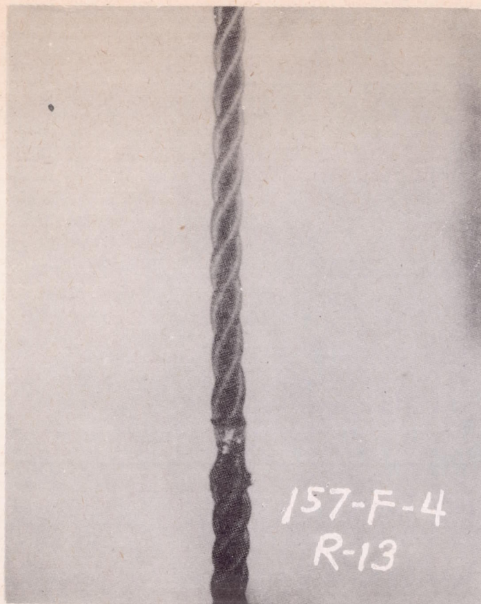
Figure 39.- Specimen "B" of 13/16-inch nylon treated with 3 dips of 1.3 dilution aquadag after being tested up to 240 ma.
