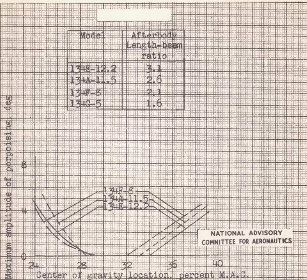
Figure 6.- Comparison of maximum amplitude of porpoising at several center of gravity locations showing the effect of changing the afterbody length-beam ratio. Each afterbody used with a depth of step which results in adequate landing stability.
