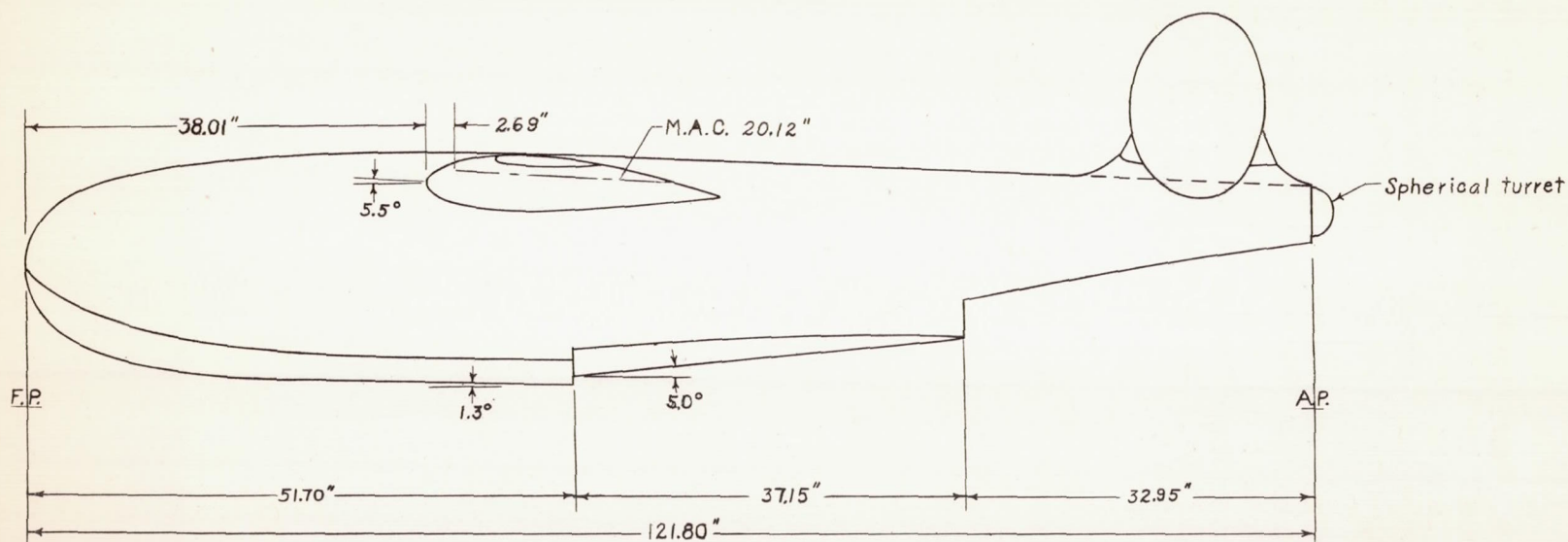
Figure 1.—Profile of Model 134A
