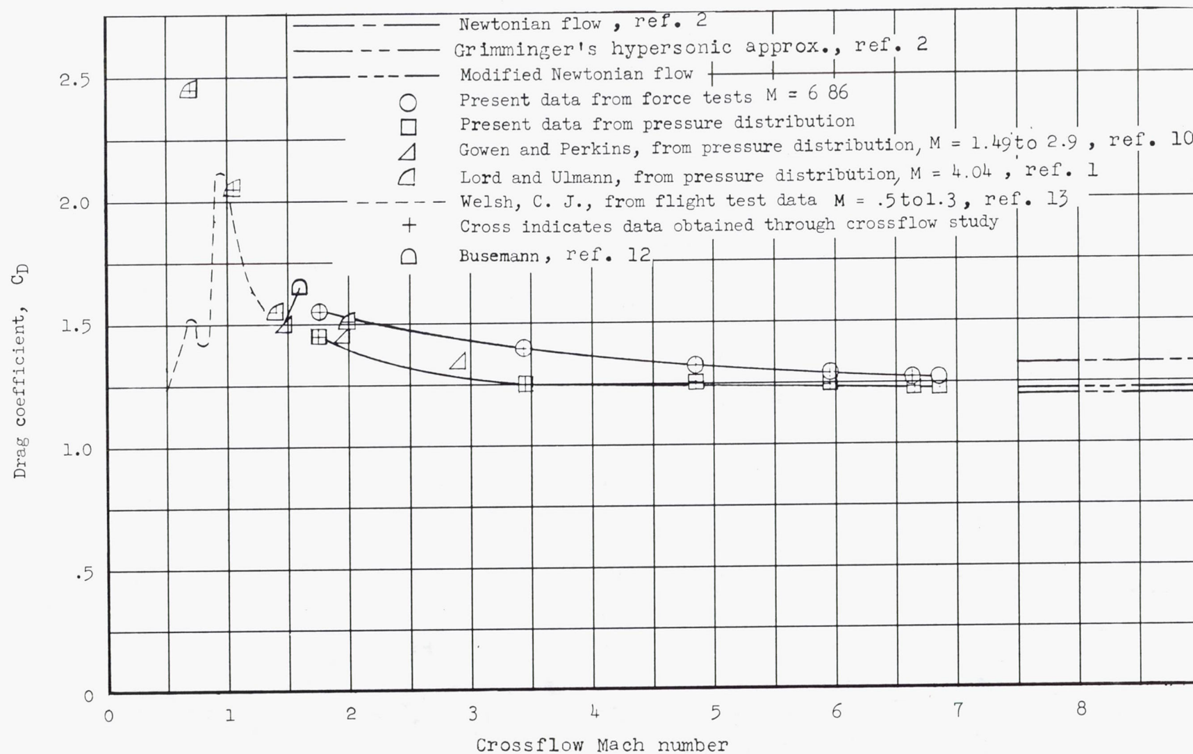
Figure 15.- Variation with crossflow Mach number of the drag coefficient of a circular cylinder.
