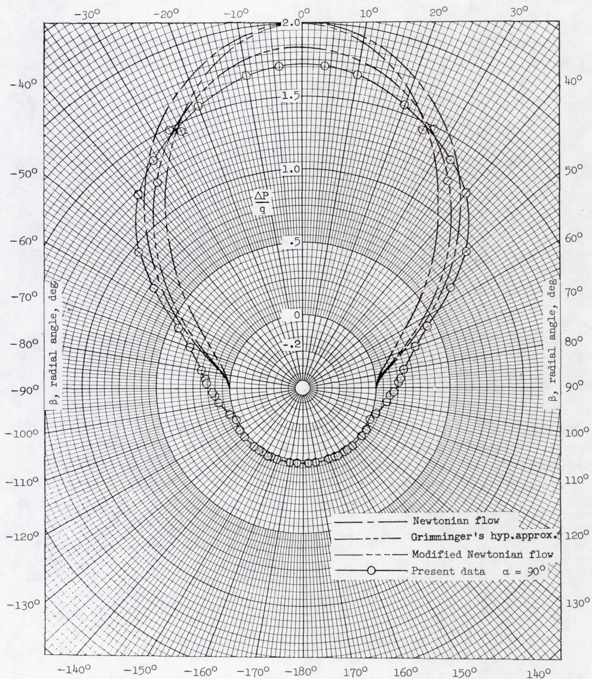
Figure 6.- Pressure distribution around a circular cylinder at \alpha = 90^\circ , M = 6.86 .
