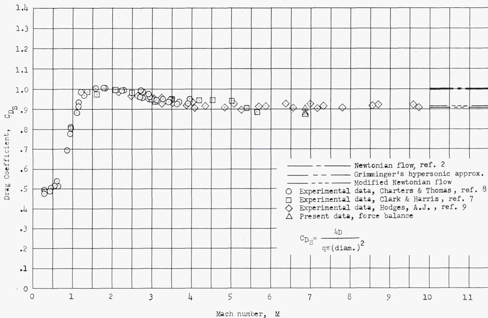
Figure 9.- Variation with Mach number of drag coefficient of a sphere.
