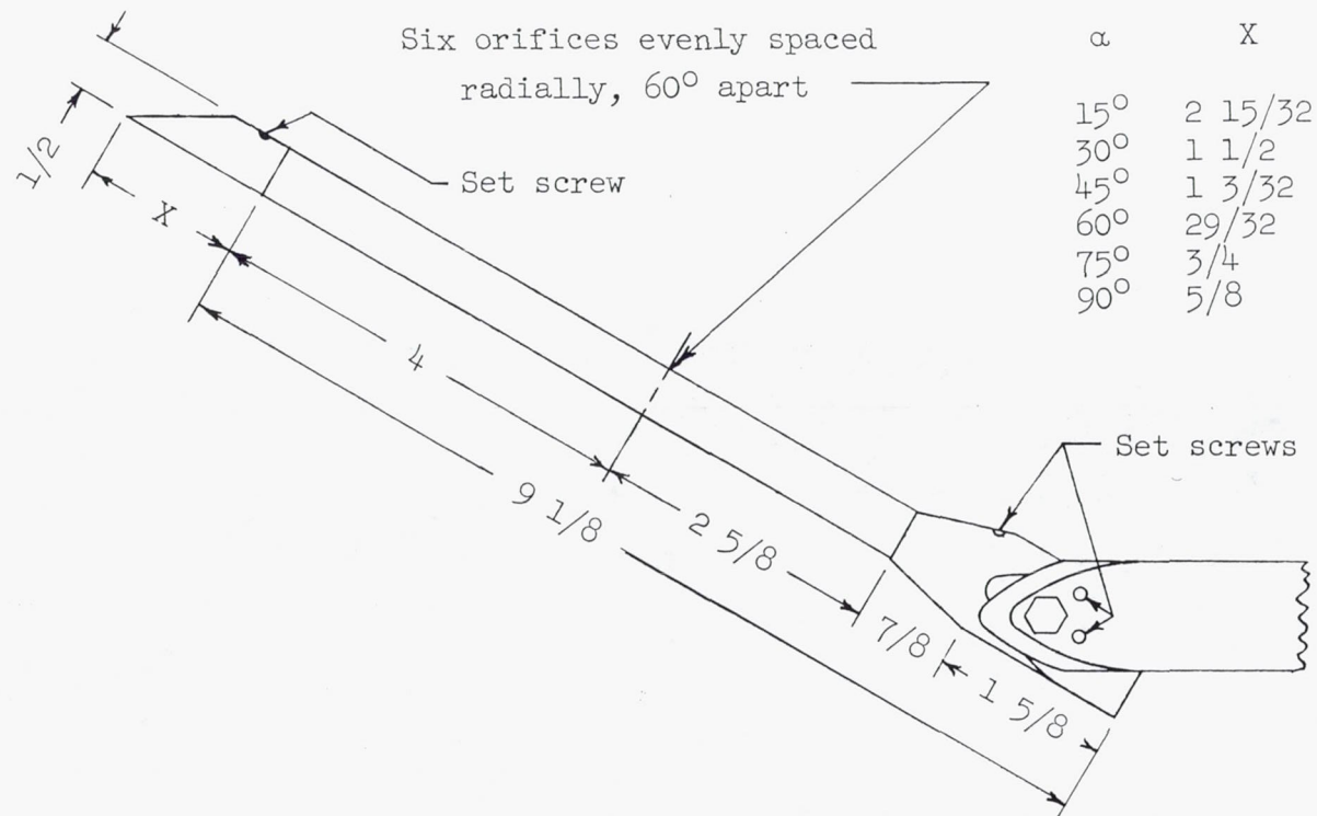
Figure 4.- Pressure model. Dimensions are in inches.
