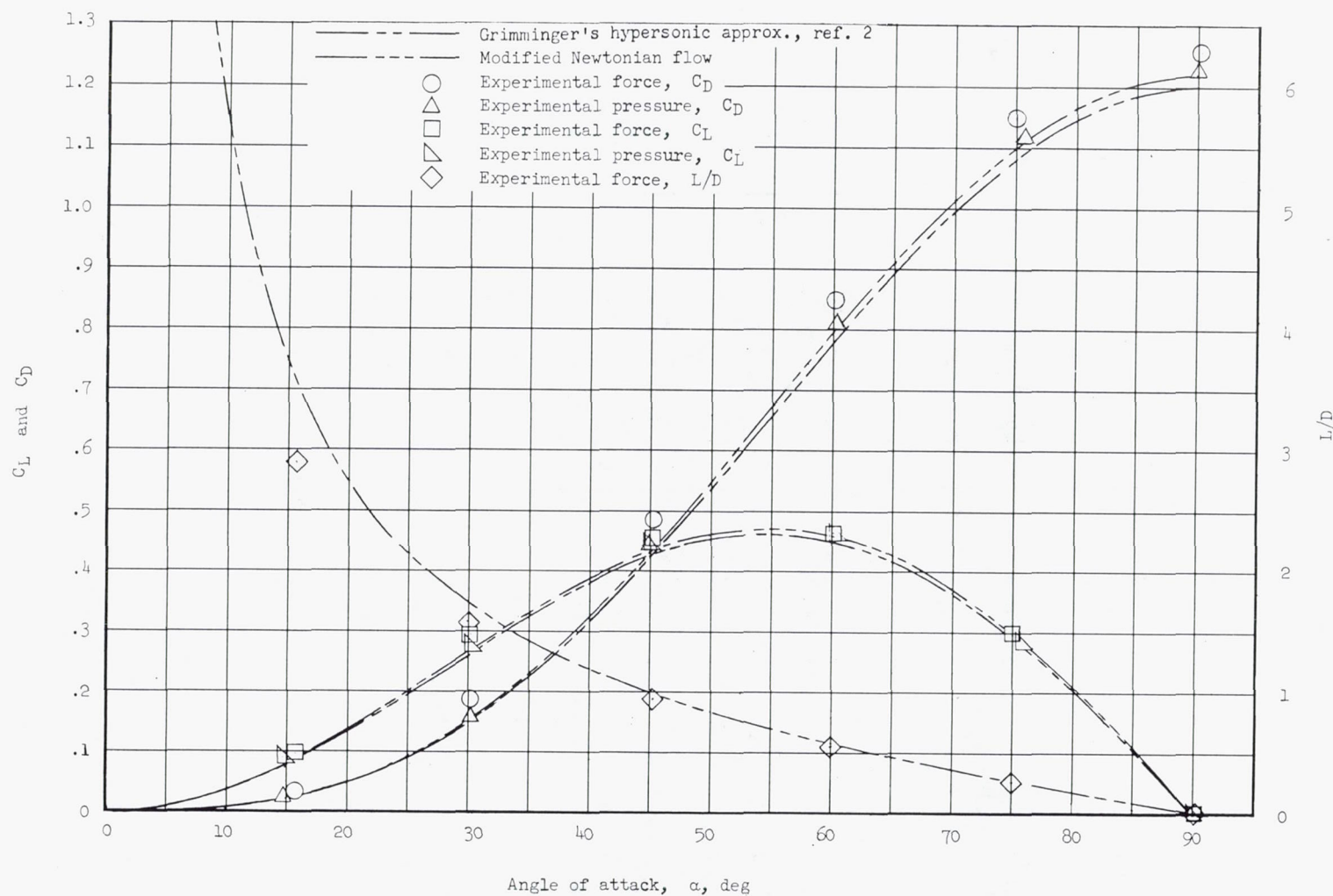
Figure 11.- Variation with angle of attack of the lift and drag coefficients of a circular cylinder. M = 6.86 .
