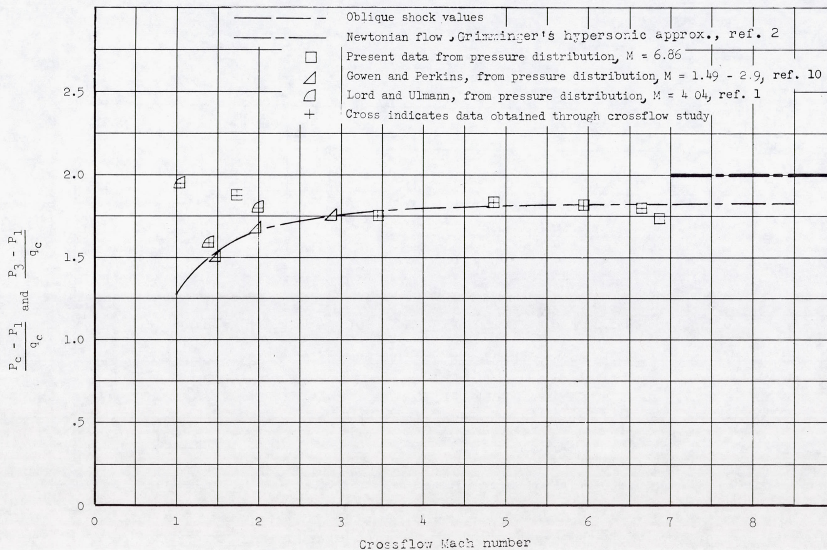
Figure 14.- Variation with crossflow Mach number of the stagnation pressure coefficient of a circular cylinder.
