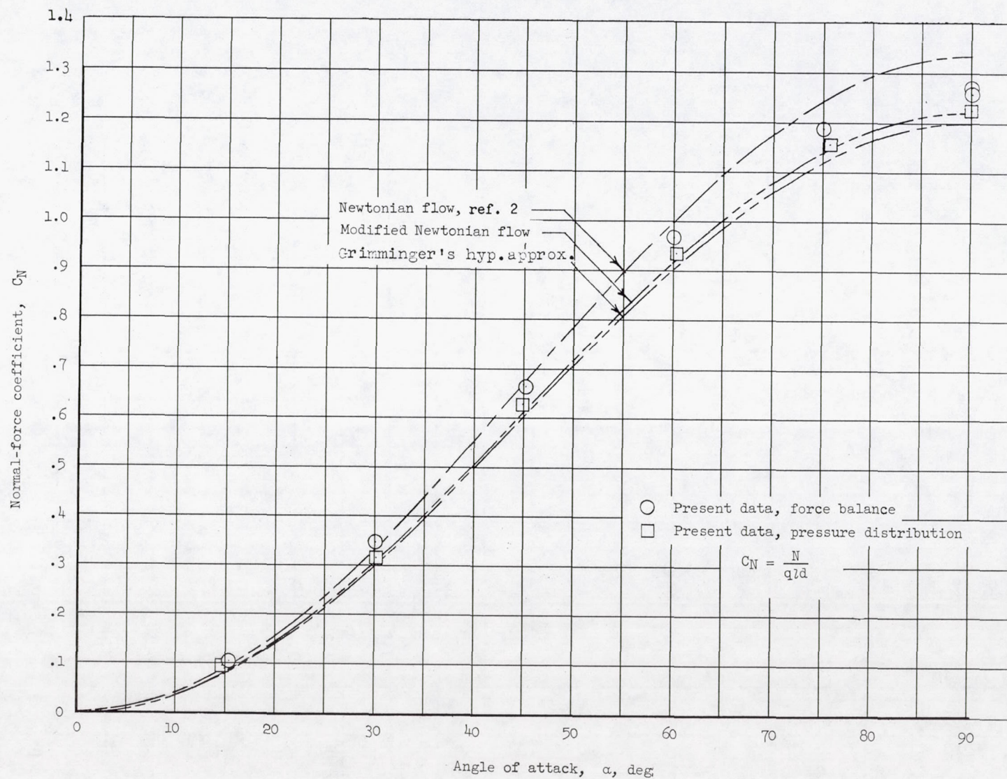
Figure 8.- Variation with angle of attack of the normal-force coefficient of a circular cylinder, M = 6.86 .
