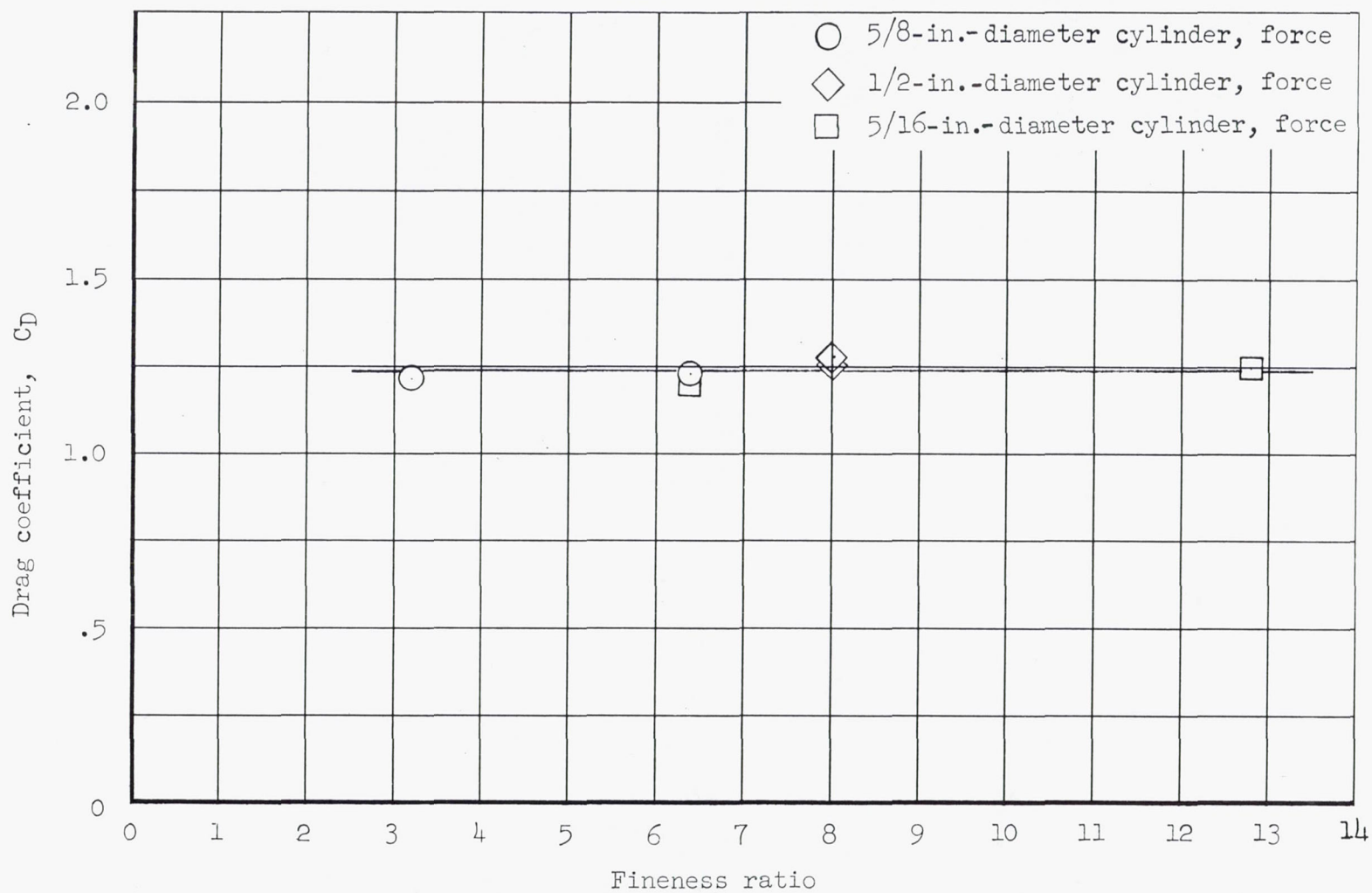
Figure 13.- Variation with fineness ratio of the drag coefficient of a circular cylinder normal to the flow. M = 6.86 ; Reynolds number = 257,000/inch.
