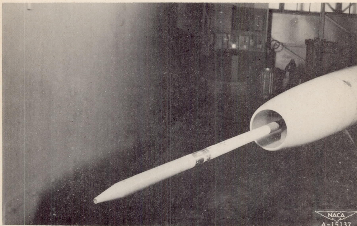
Figure 6.- Nose inlet and airspeed boom installation.
