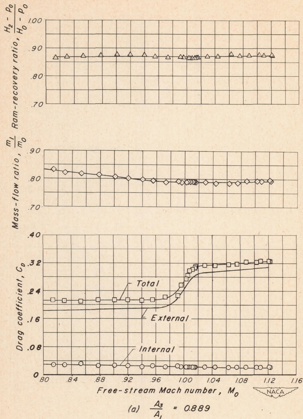
Figure 13. - Variation of drag coefficients, pressure recovery, and mass-flow ratio with free-stream Mach number for submerged inlet model.
