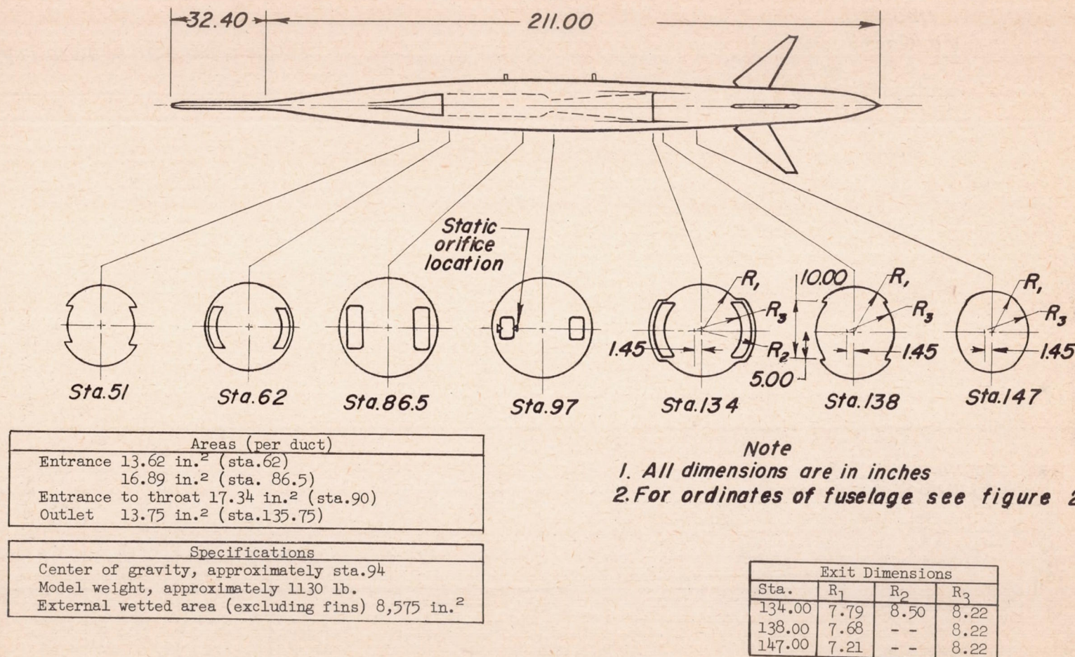
Figure 3— Details of submerged inlet model.
