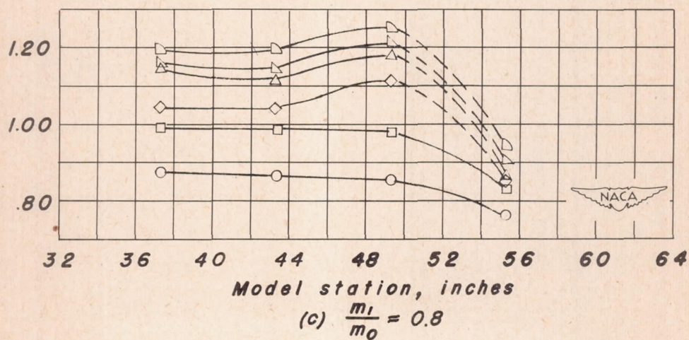
Figure 15. — Mach number distribution along ramp of submerged inlet at mass-flow ratios of about 0.4, 0.6, and 0.8.
