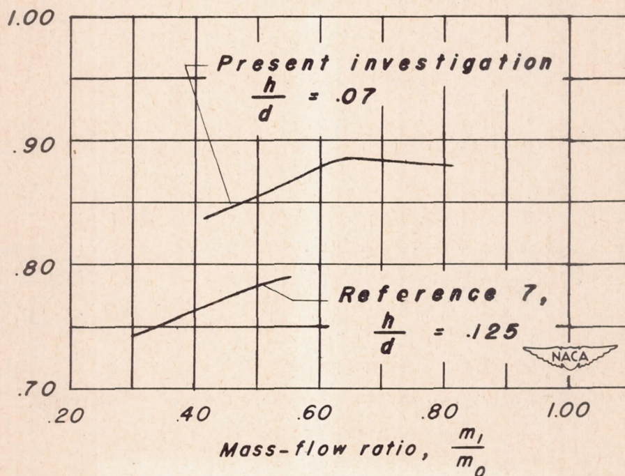
Figure 23. — Comparison of variation of ram-recovery ratio with mass-flow ratio of submerged-inlet model with previous data.
