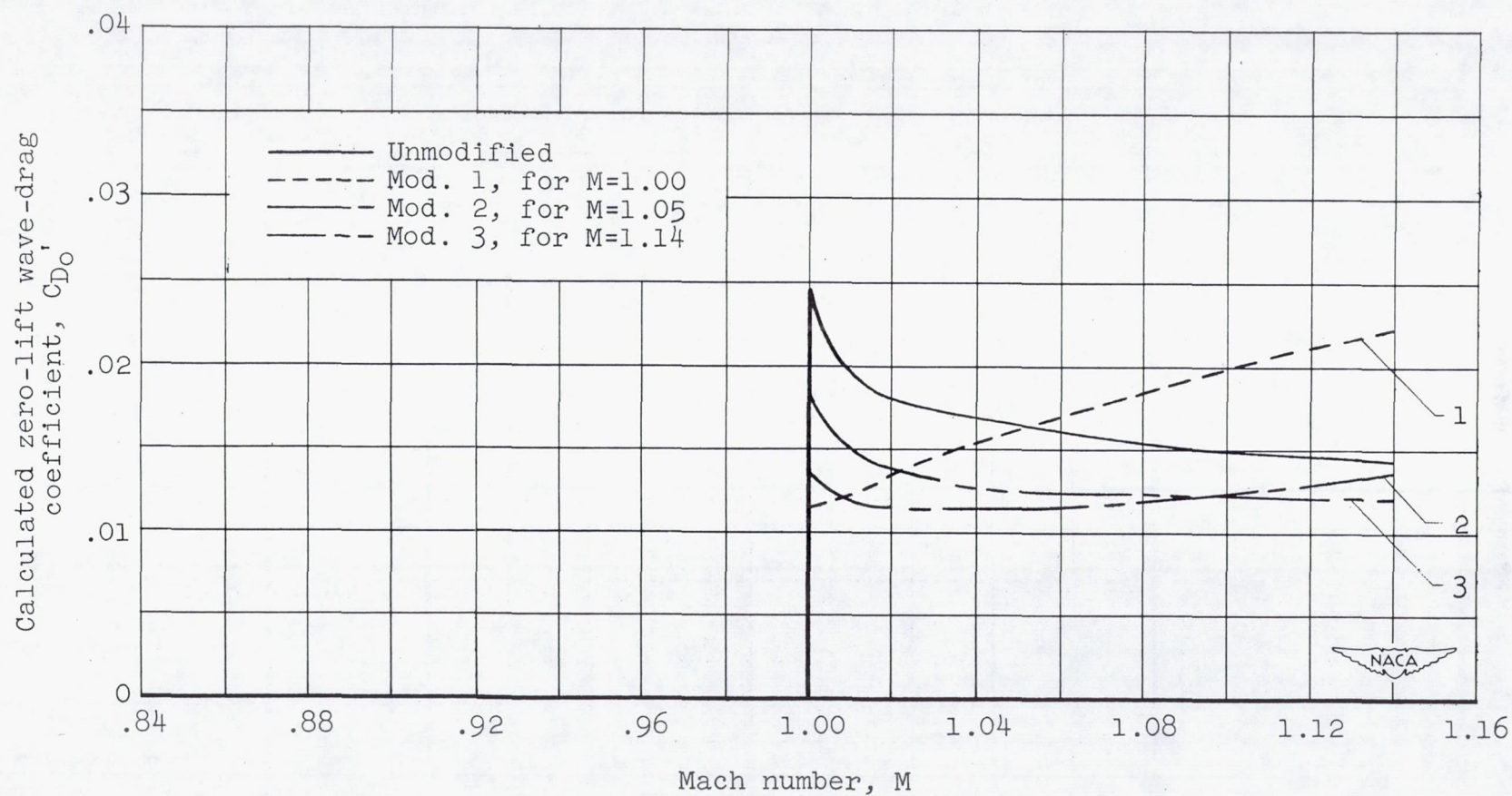
Figure 11.- Theoretical computations from reference 2.
