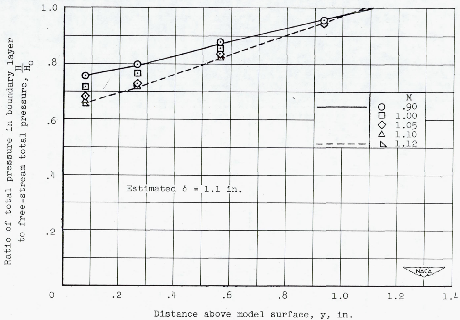
Figure 12.- Total pressure distribution in the boundary layer measured at fuselage station 100.
