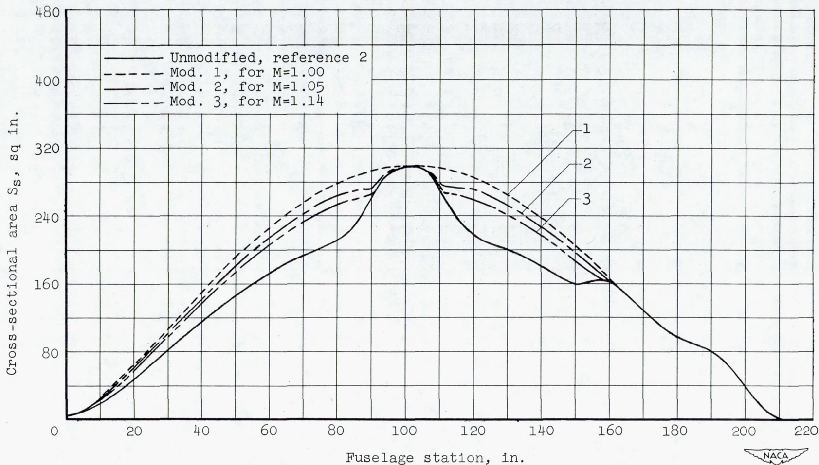
Figure 2.- The axial distributions of cross-sectional area normal to the longitudinal axis for the basic model and for the three modifications.
