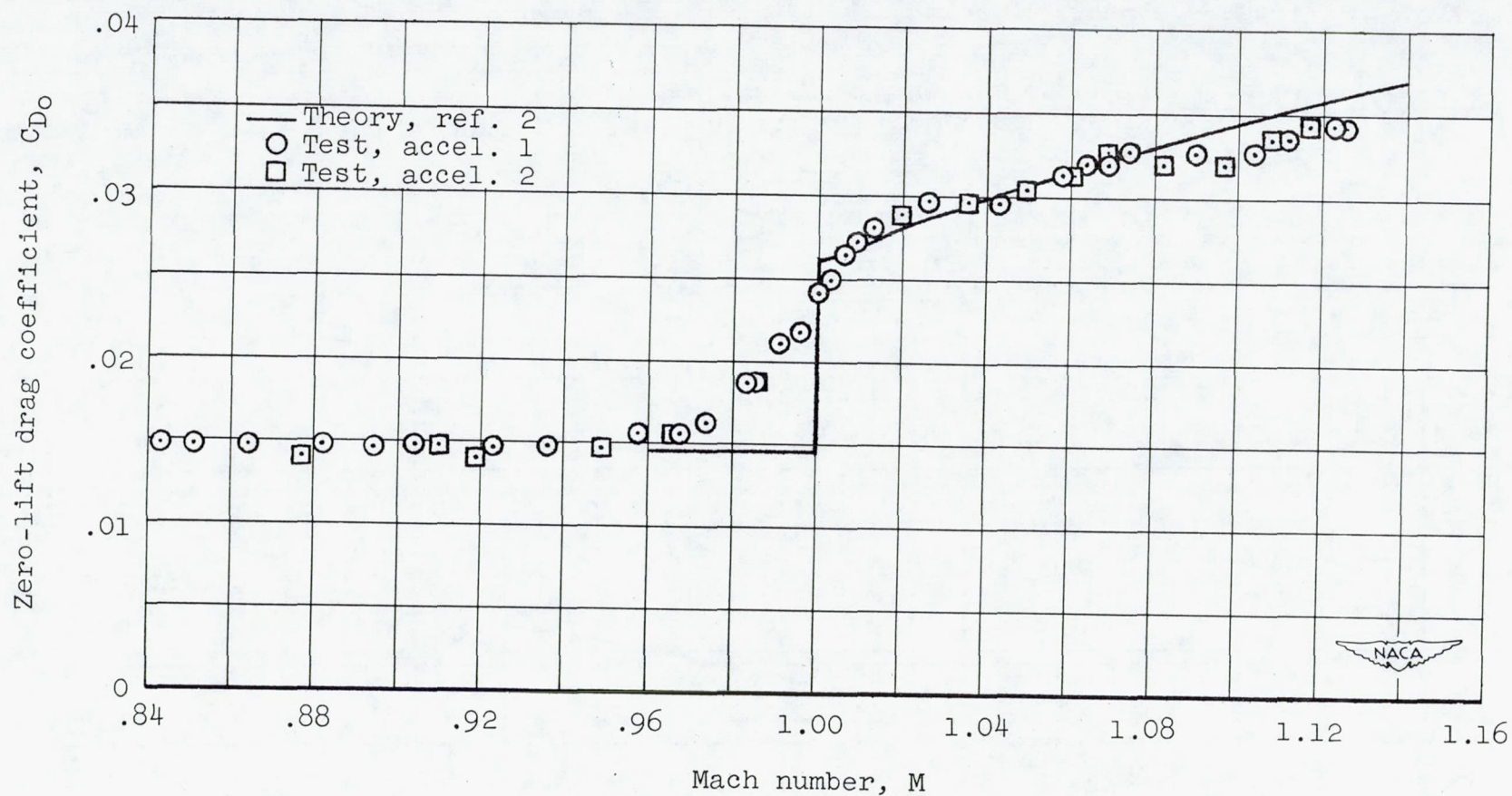
(a) Modification 1, for M=1.00 .
