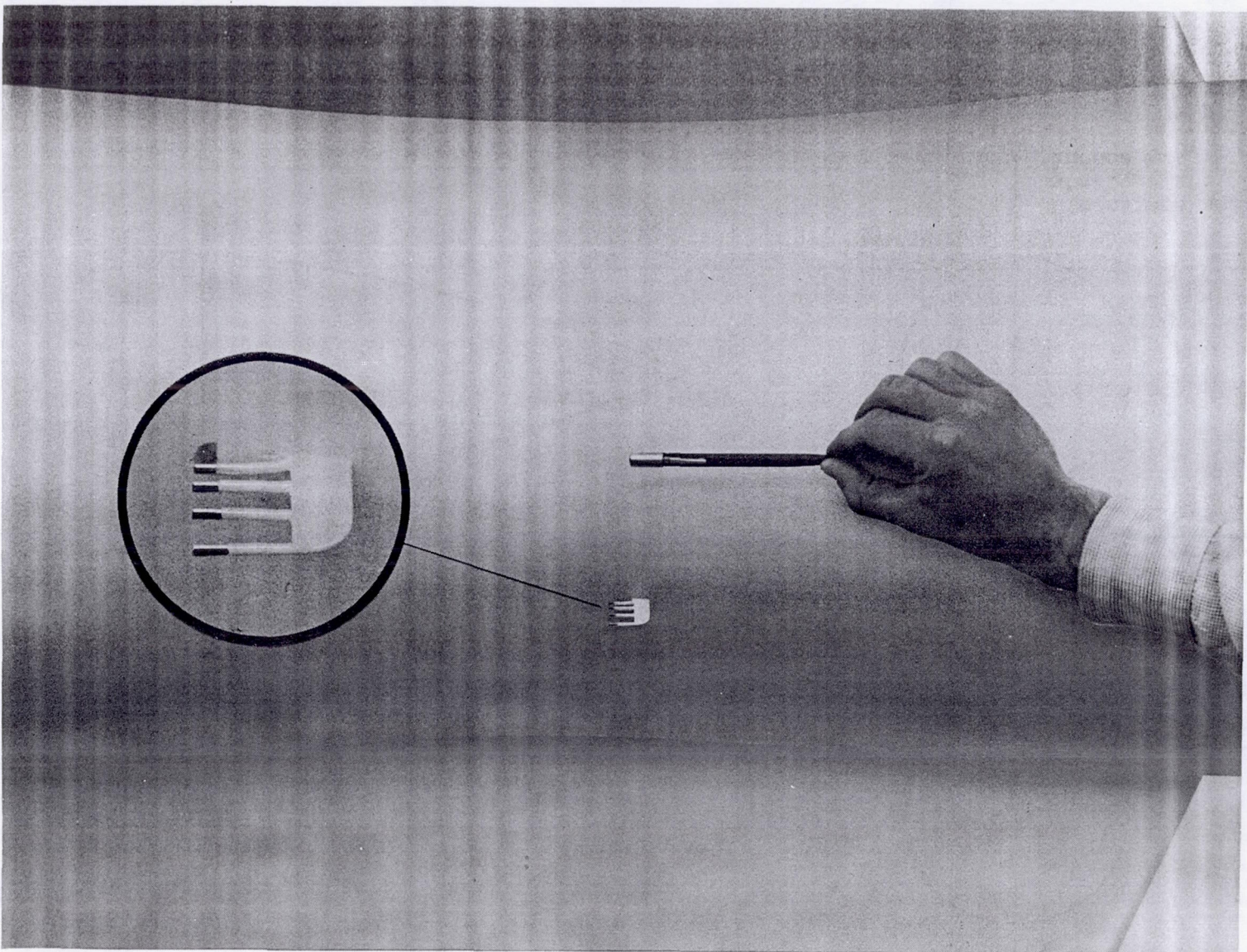
Figure 5.- Four-tube pitot-pressure rake located at fuselage station 100.
