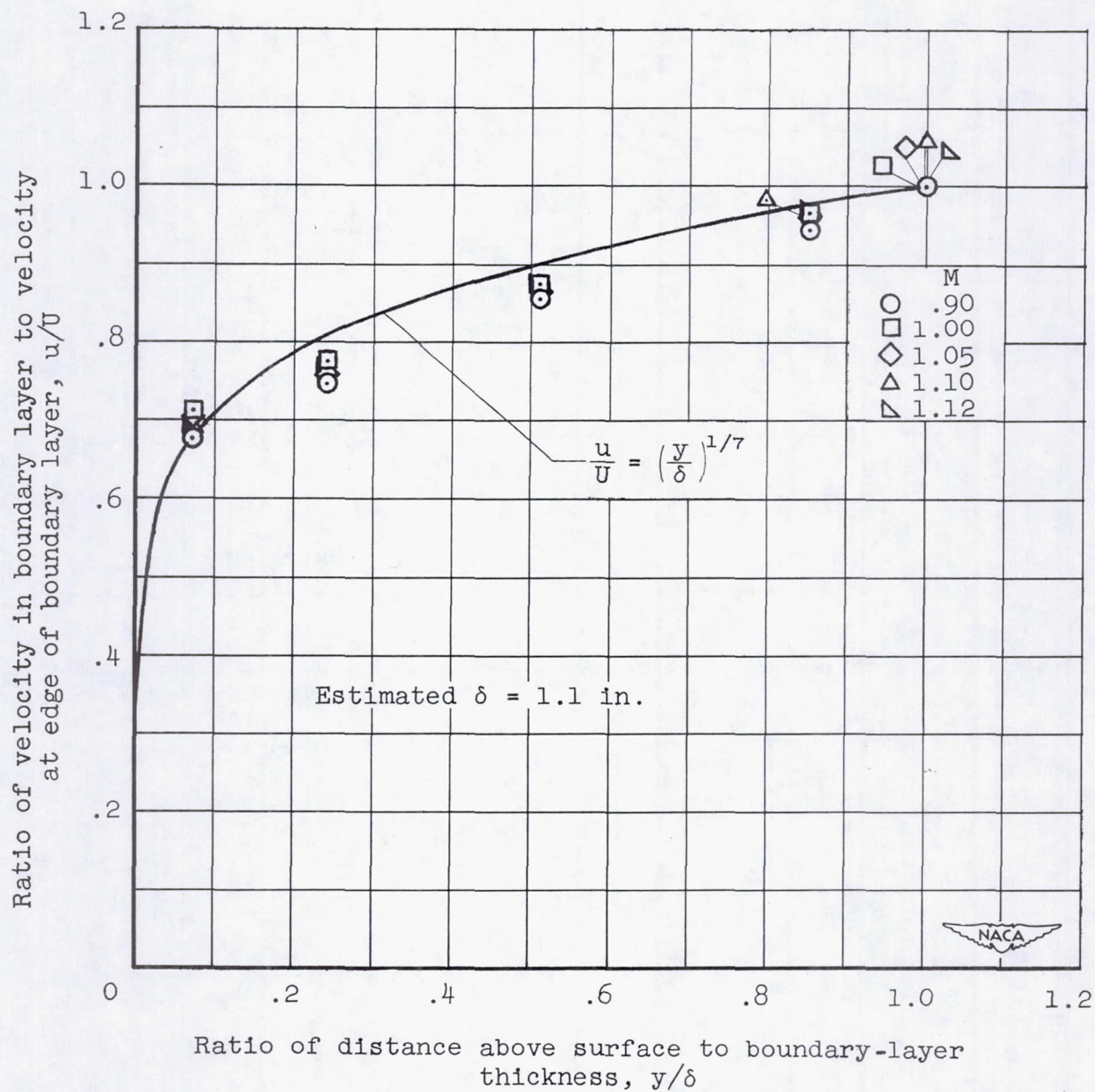
Figure 15.- Velocity profile data points in the turbulent boundary layer at fuselage station 100.
