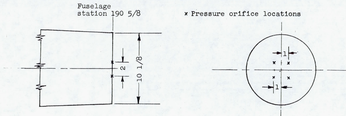
(a) M=1.05 modification with blunted tail.
