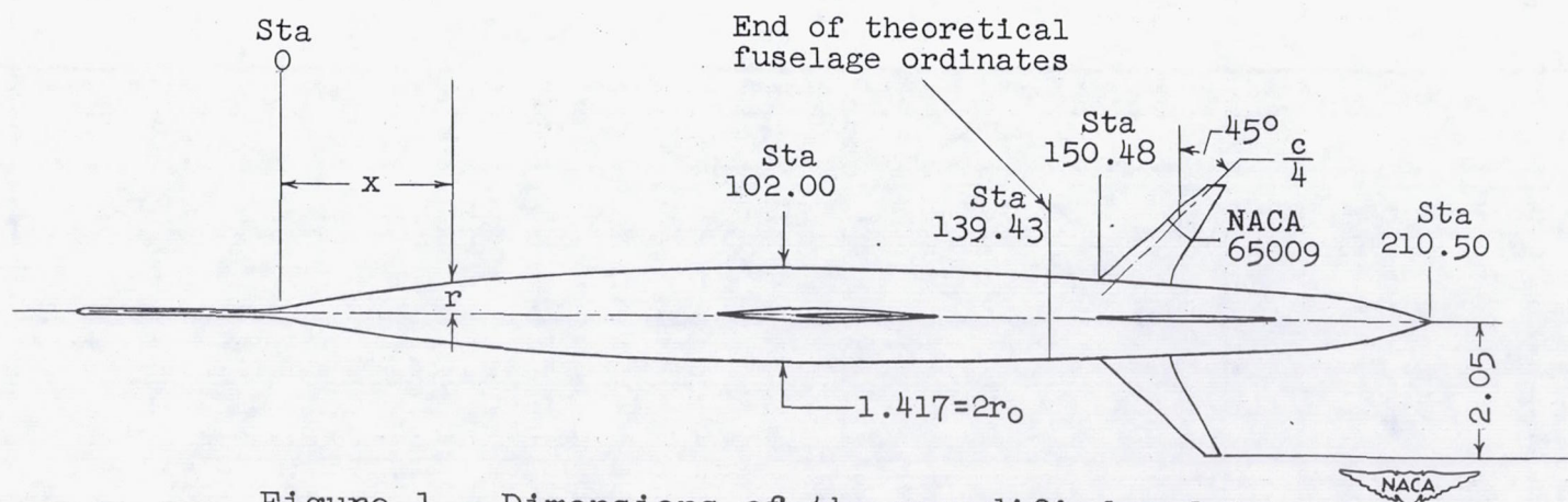
Figure 1.- Dimensions of the unmodified model.
