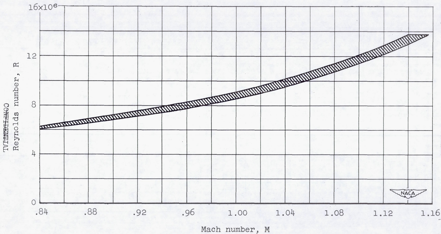
Figure 7.- Reynolds number variation with Mach number for the tests of the modified configurations.
