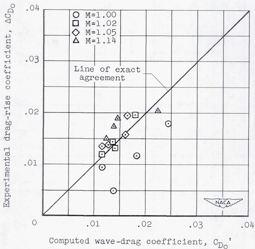
Figure 13.- Comparison between computed zero-lift wave-drag coefficients and experimental zero-lift drag-rise coefficients (see table II).
