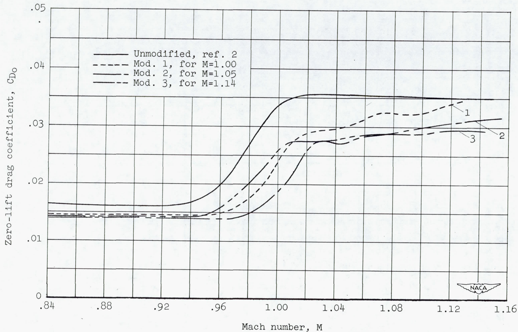
Figure 10.- Comparison of the experimental zero-lift drag coefficients for the various modifications with the unmodified configuration.
