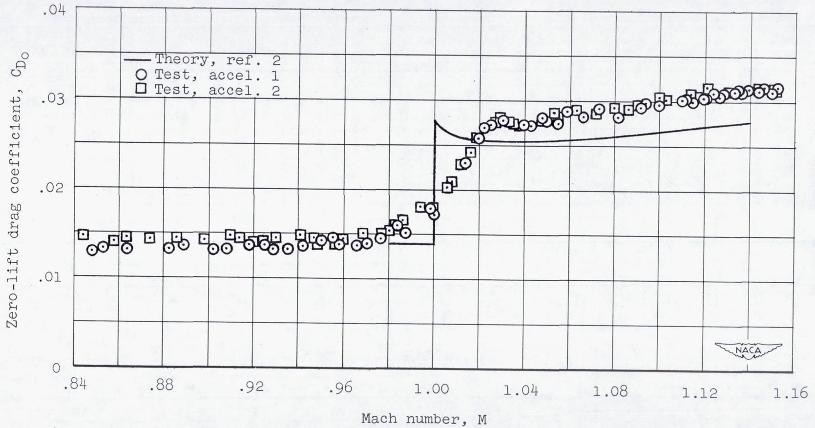
(b) Modification 2, for M=1.05 .
