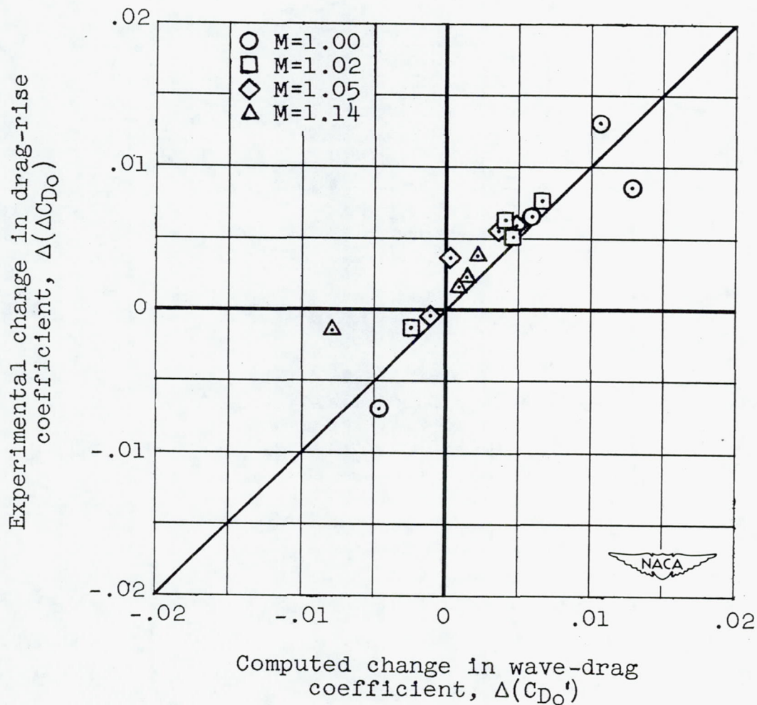
Figure 14.- Comparison between changes in computed zero-lift wave-drag coefficients and changes in experimental zero-lift drag-rise coefficients due to modifications (see table III).
