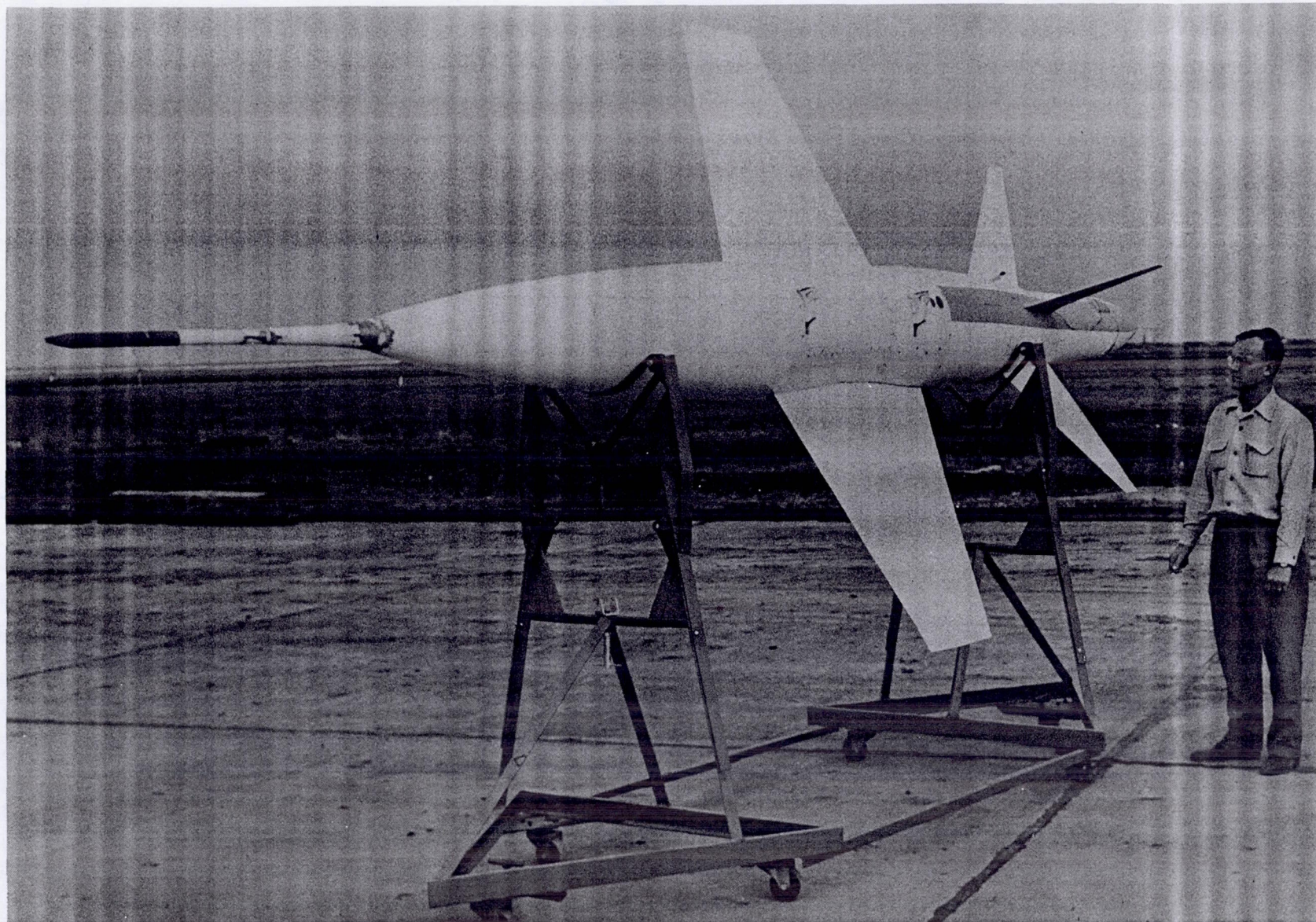
Figure 3.- Model modified for M=1.00 . The airplane attachment brackets were retracted to form a flush surface during free-fall flight.
