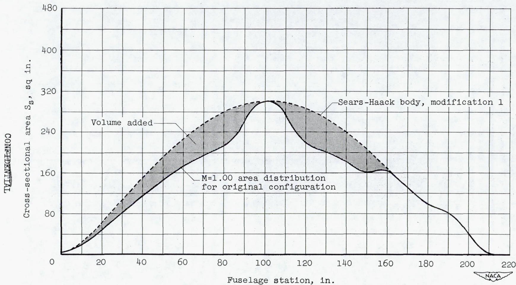
(a) Modification 1, for M=1.00 .
