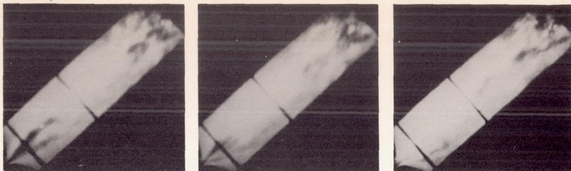
1 2 3 (a) Run 17: interval between frames, 0.42 millisecond; thrust, 73 pounds.
