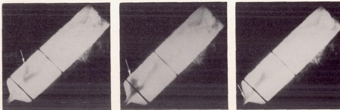
Figure 8. - Combustion of liquid oxygen and gasoline in transparent-sided rocket engine using single-intersecting jets and showing motion of nonluminous pocket. Run 1; interval between frames, 0.333 millisecond; thrust, 75 pounds.
