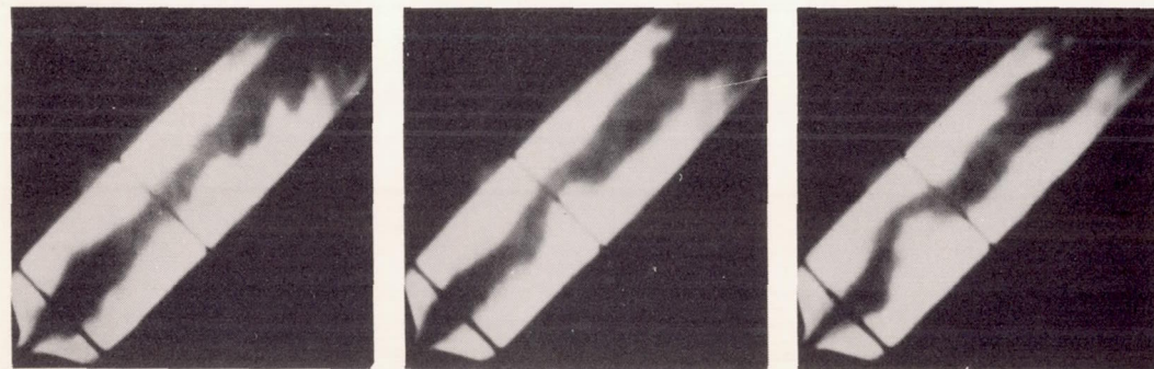
1 2 3 (a) Run 17: interval between frames, 0.42 millisecond; thrust, 73 pounds.
