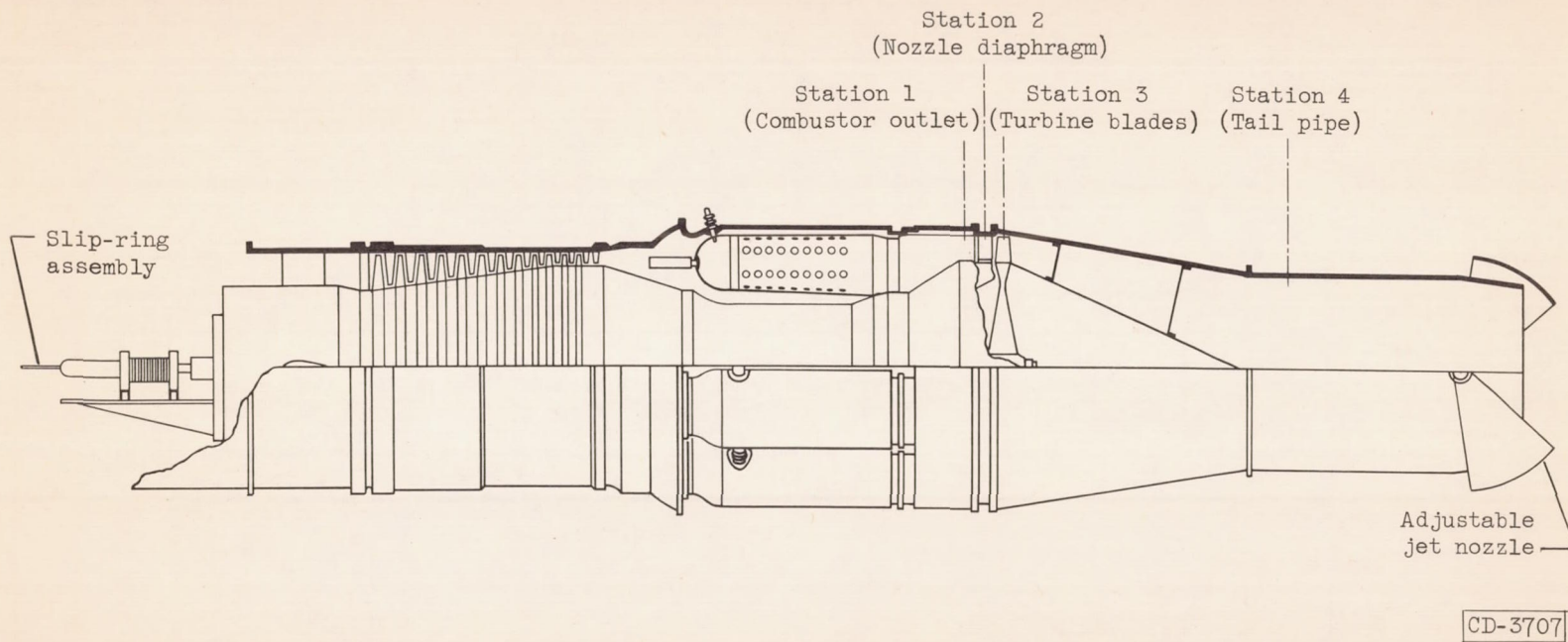
Figure 1. - J47-25 engine instrumentation.
