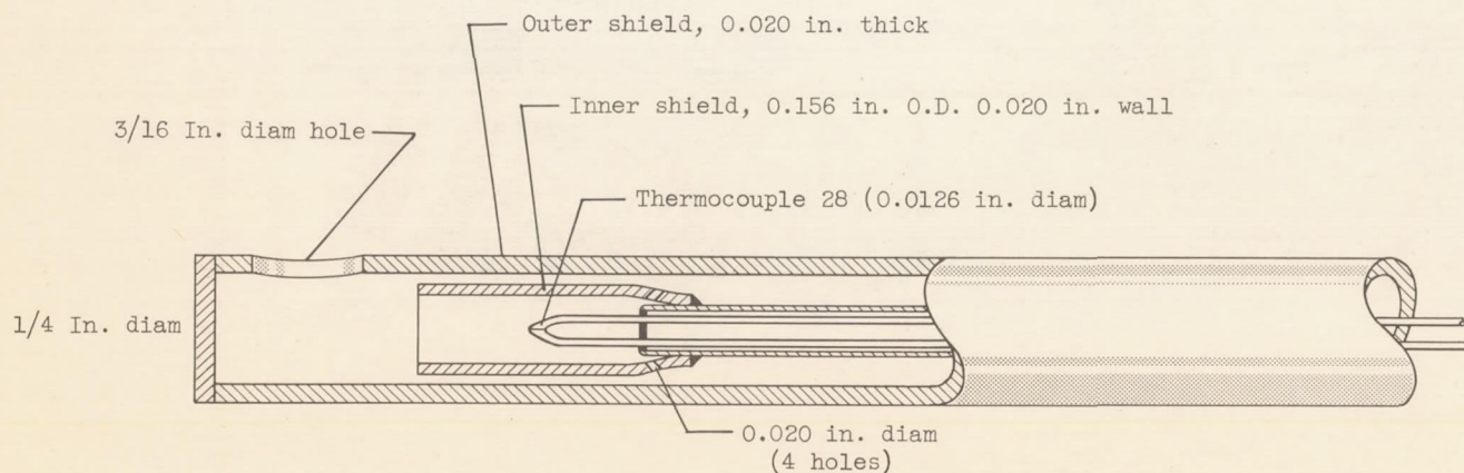
Figure 2. - Double-shielded aspirated thermocouple probe.
