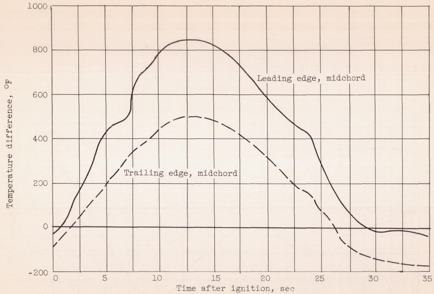
Figure 19. - Concluded. Turbine-blade temperature difference during transient runs.
