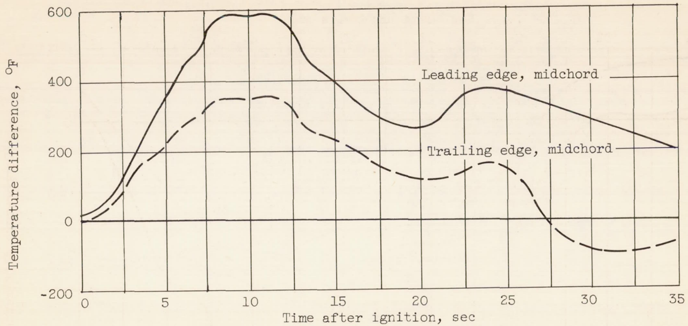
Figure 19. - Continued. Turbine-blade temperature difference during transient runs.
