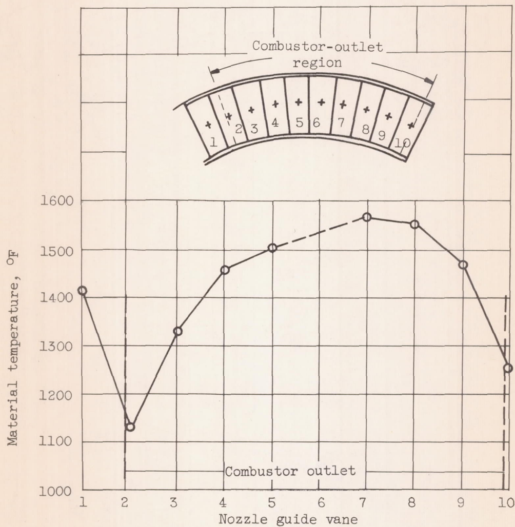
(a) Nozzle guide vane. Combustor-outlet survey.
