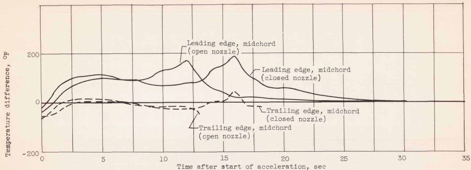
Figure 19. - Turbine-blade temperature difference during transient runs.
