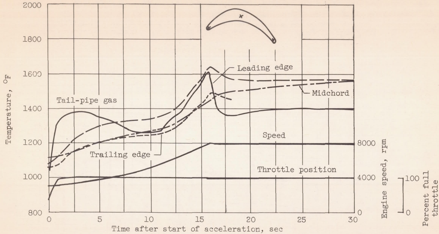
(a) Turbine blade.
