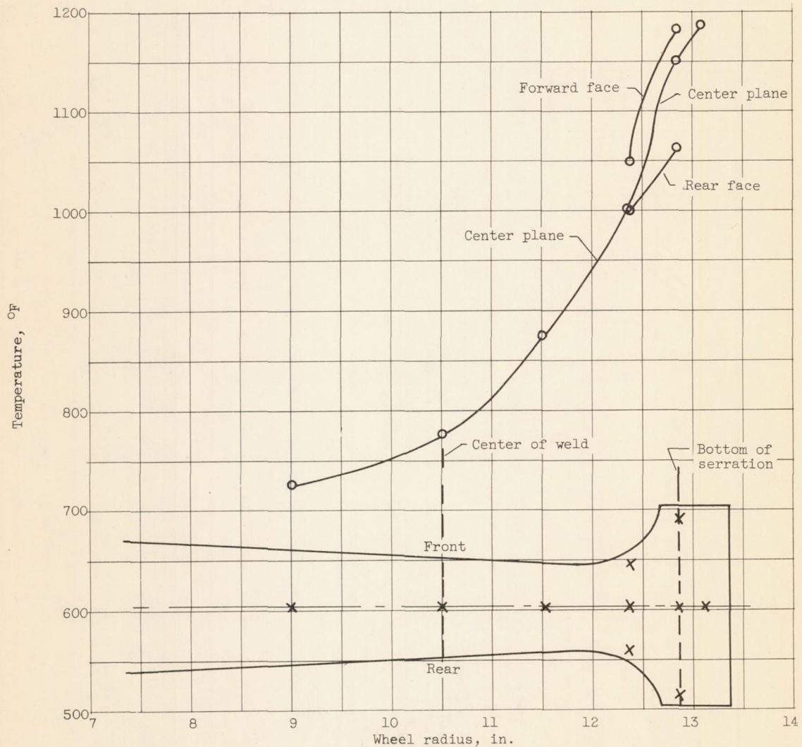
Figure 14. - Equilibrium temperatures in turbine disk. Engine speed, 7950 rpm; tail-pipe gas temperature 1275° F.
