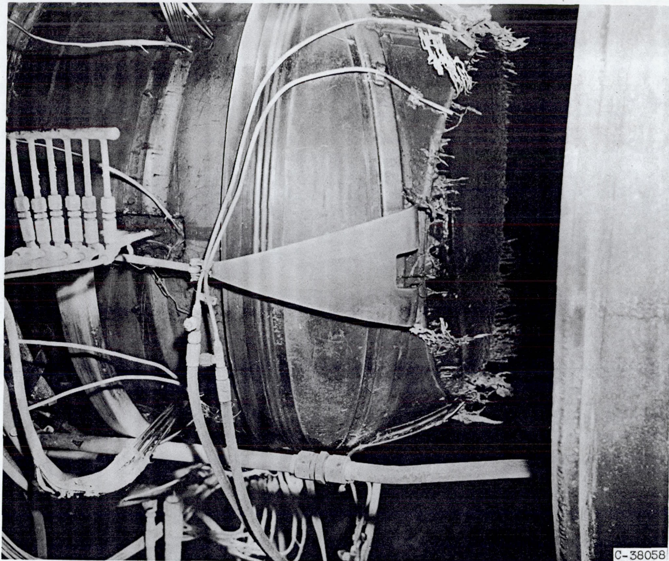
(g) Exhaust nozzle.
