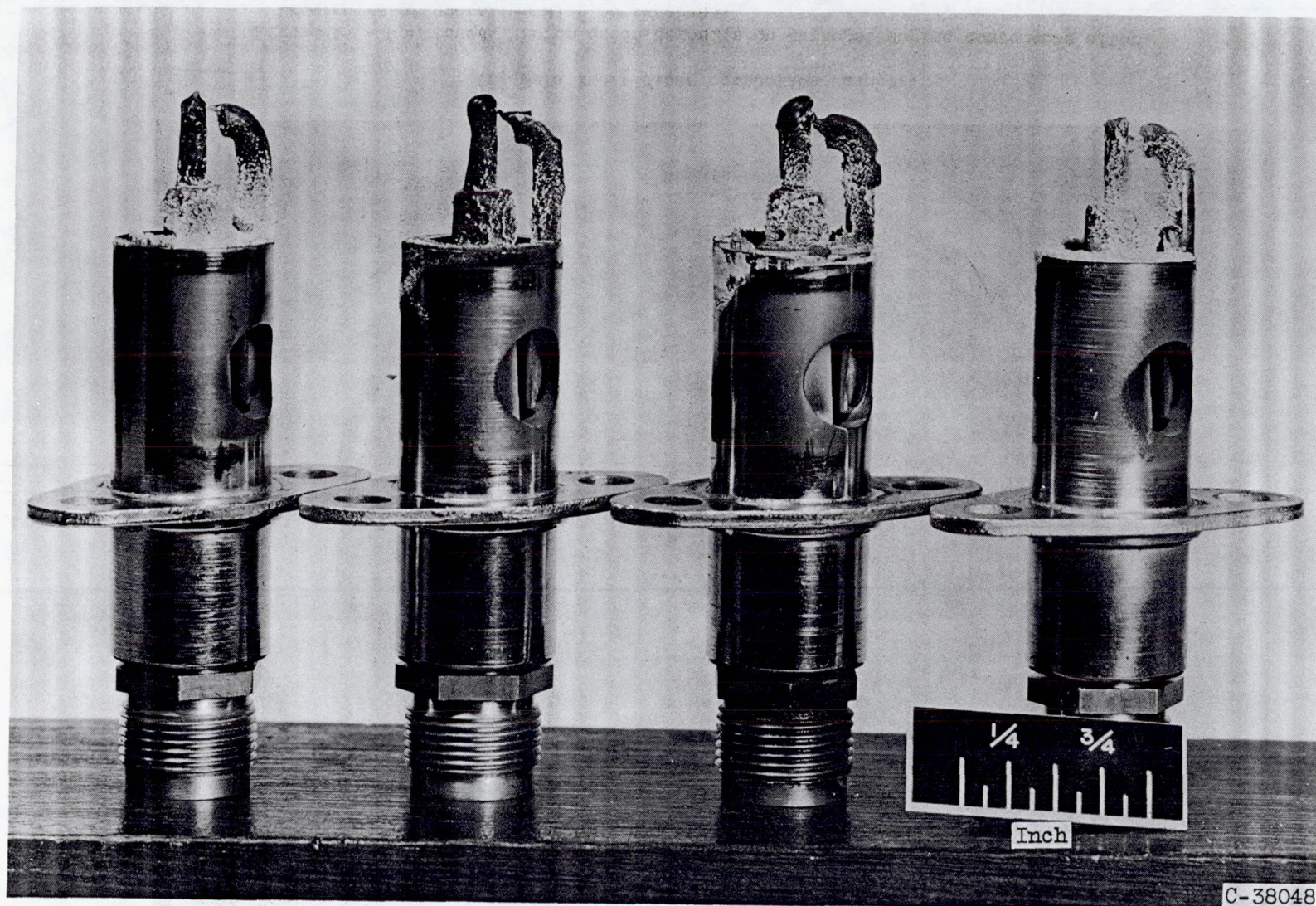
(c) Engine spark plugs.
