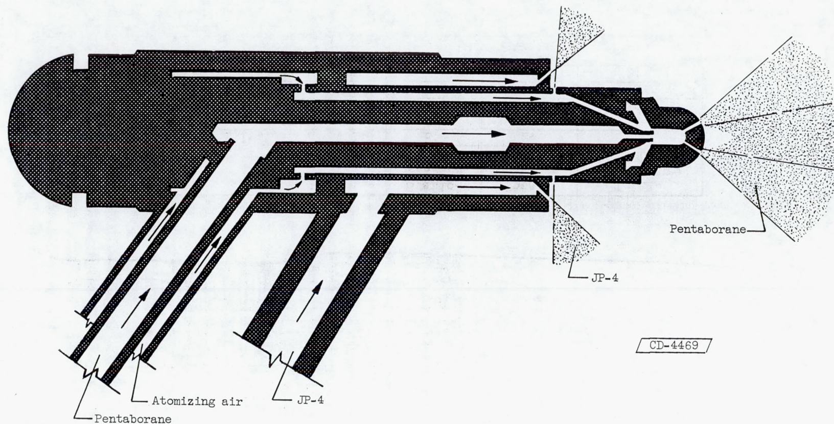
Figure 2. - Air-atomizing fuel nozzle used during pentaborane fuel test in full-scale turbojet engine. Nozzle also provided for use of JP-4 fuel.
