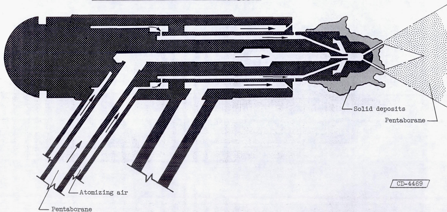
Figure 3. - Boron oxide deposits on turbojet-engine fuel nozzle after 22 minutes of operation with pentaborane.
