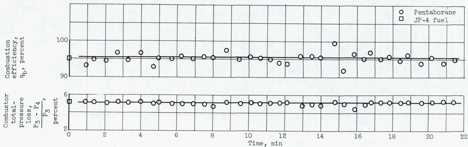
Figure 6. - Effect of operation with pentaborane fuel on combustor performance. Altitude, 50,000 feet; flight Mach number, 0.8.
