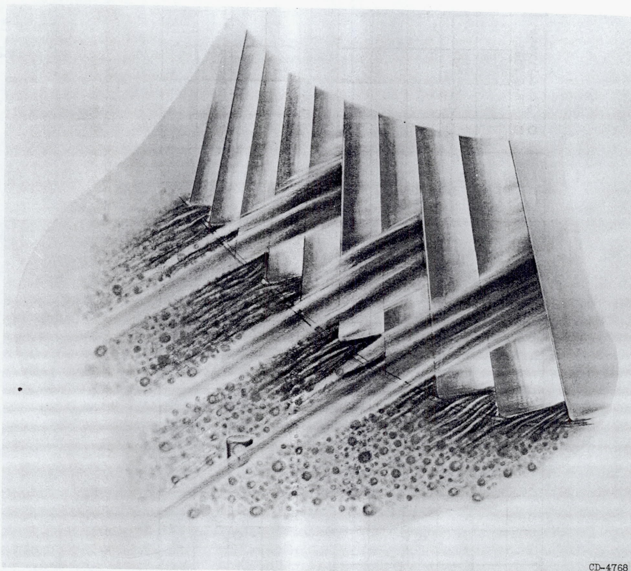
Figure 8. - Boron oxide flowing through turbine rotor section into turbojet-engine tailpipe.
