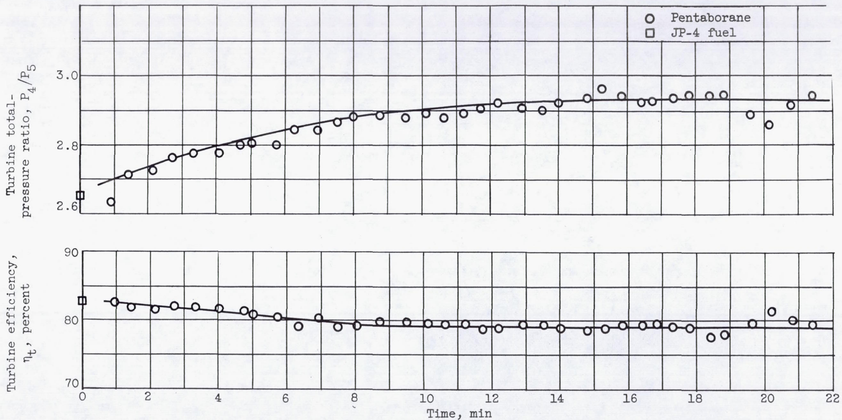
Figure 7. - Effect of operation with pentaborane fuel on turbine performance. Altitude, 50,000 feet; flight Mach number, 0.8.
