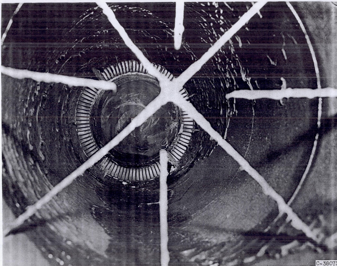
(f) Tailpipe (looking upstream).
