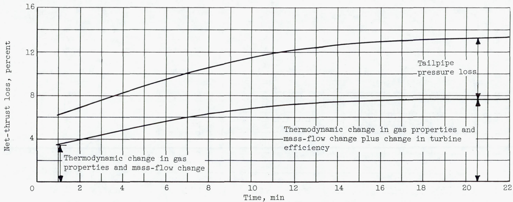
Figure 12. - Net-thrust loss encountered with use of pentaborane fuel. Altitude, 50,000 feet; flight Mach number, 0.8.
