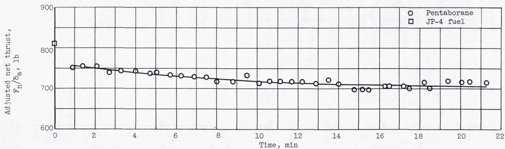
Figure 11. - Effect of operation with pentaborane fuel on net thrust. Altitude, 50,000 feet; flight Mach number, 0.8.
