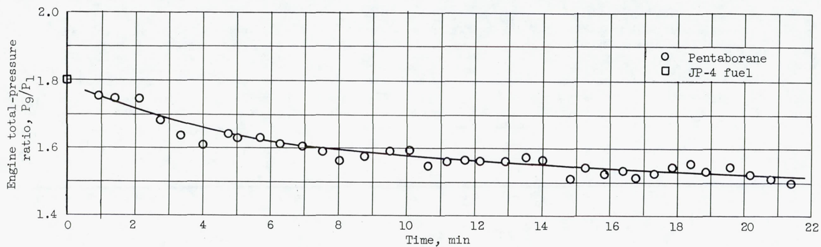
Figure 10. - Effect of operation with pentaborane fuel on engine total-pressure ratio. Altitude, 50,000 feet; flight Mach number, 0.8; engine total-temperature ratio, 3.3.
