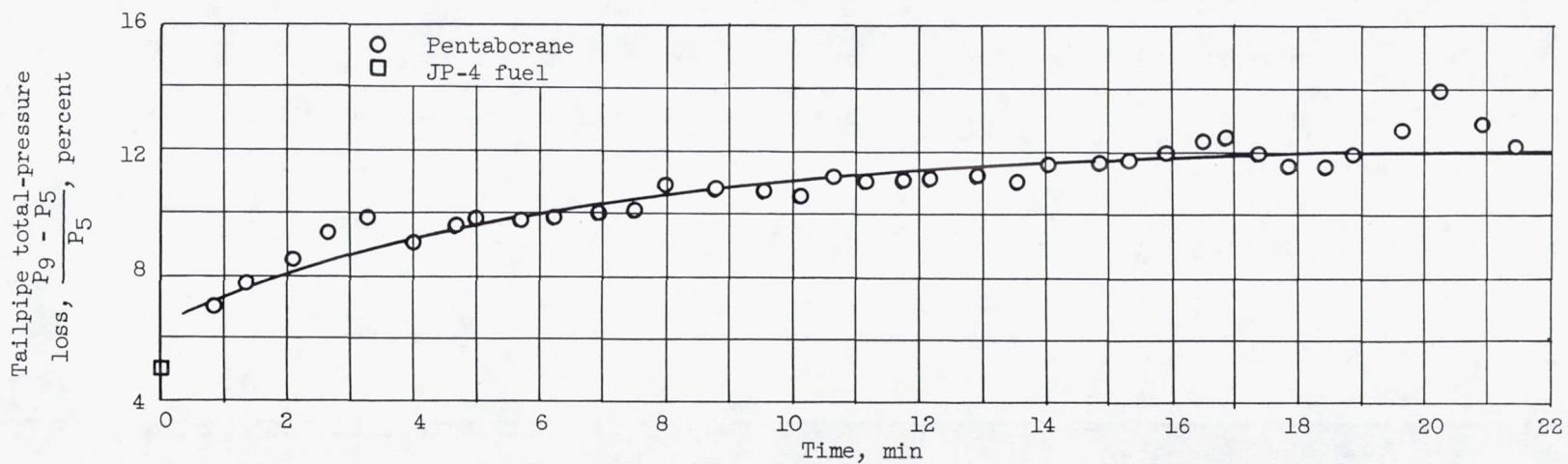
Figure 9. - Variation of tailpipe total-pressure loss with extended operation with pentaborane fuel. Altitude, 50,000 feet; flight Mach number, 0.8.
