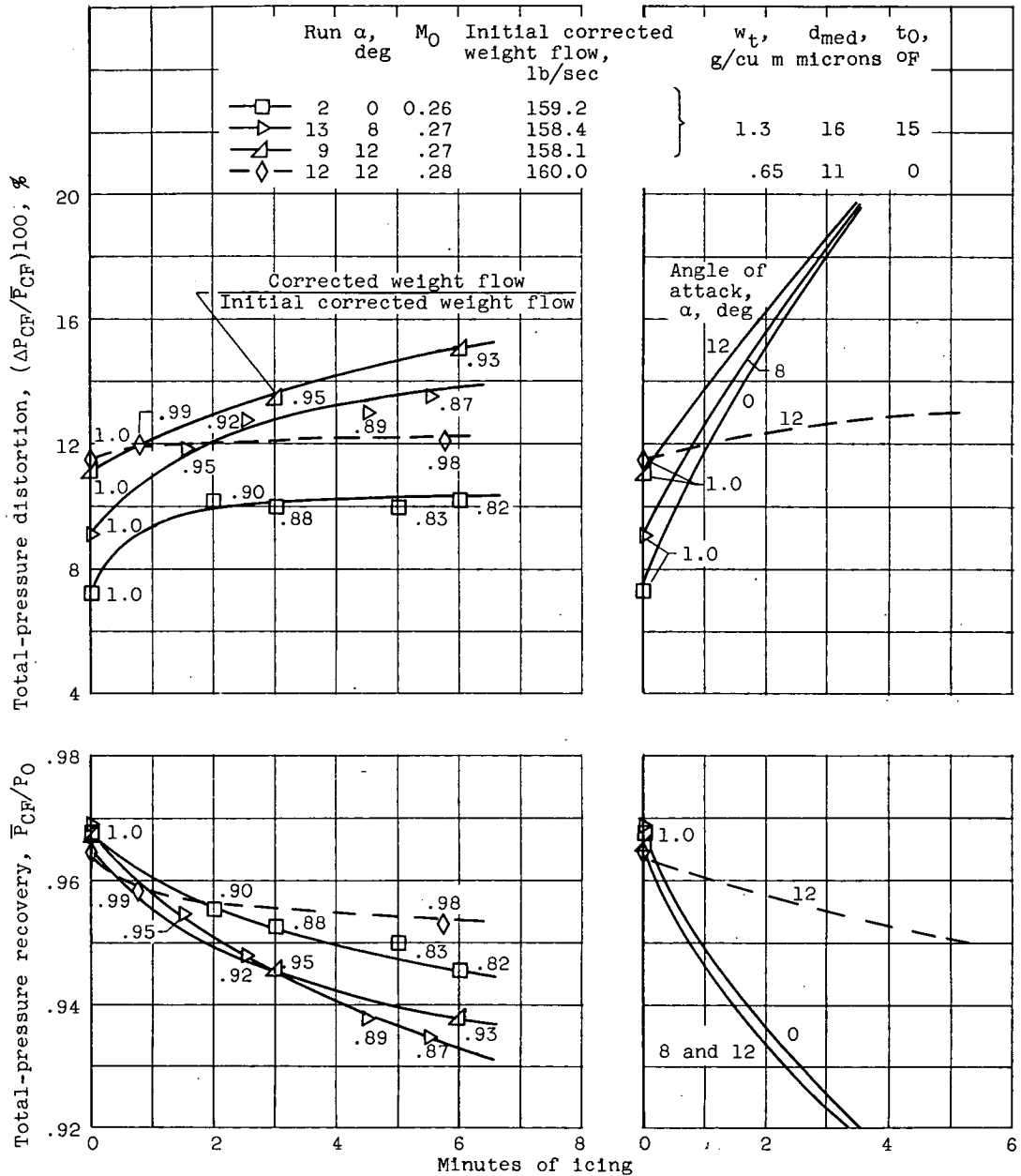
Figure 12. - Effect of icing time and intensity on total-pressure distortion and recovery at diffuser exit (compressor face) of supersonic nose inlet at 12°, 8°, and 0° angle of attack.
