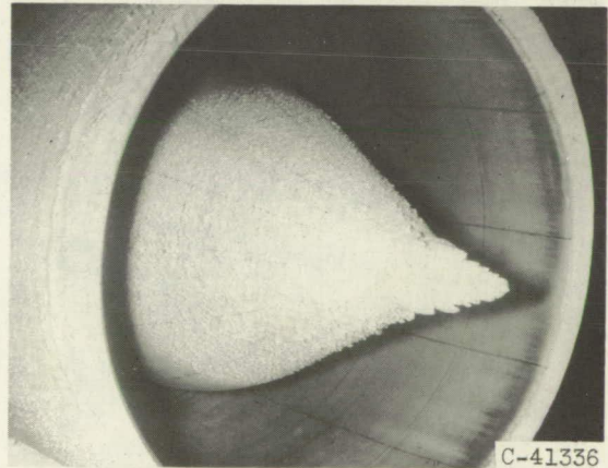
Photographs after 10 3/4 minutes of icing
