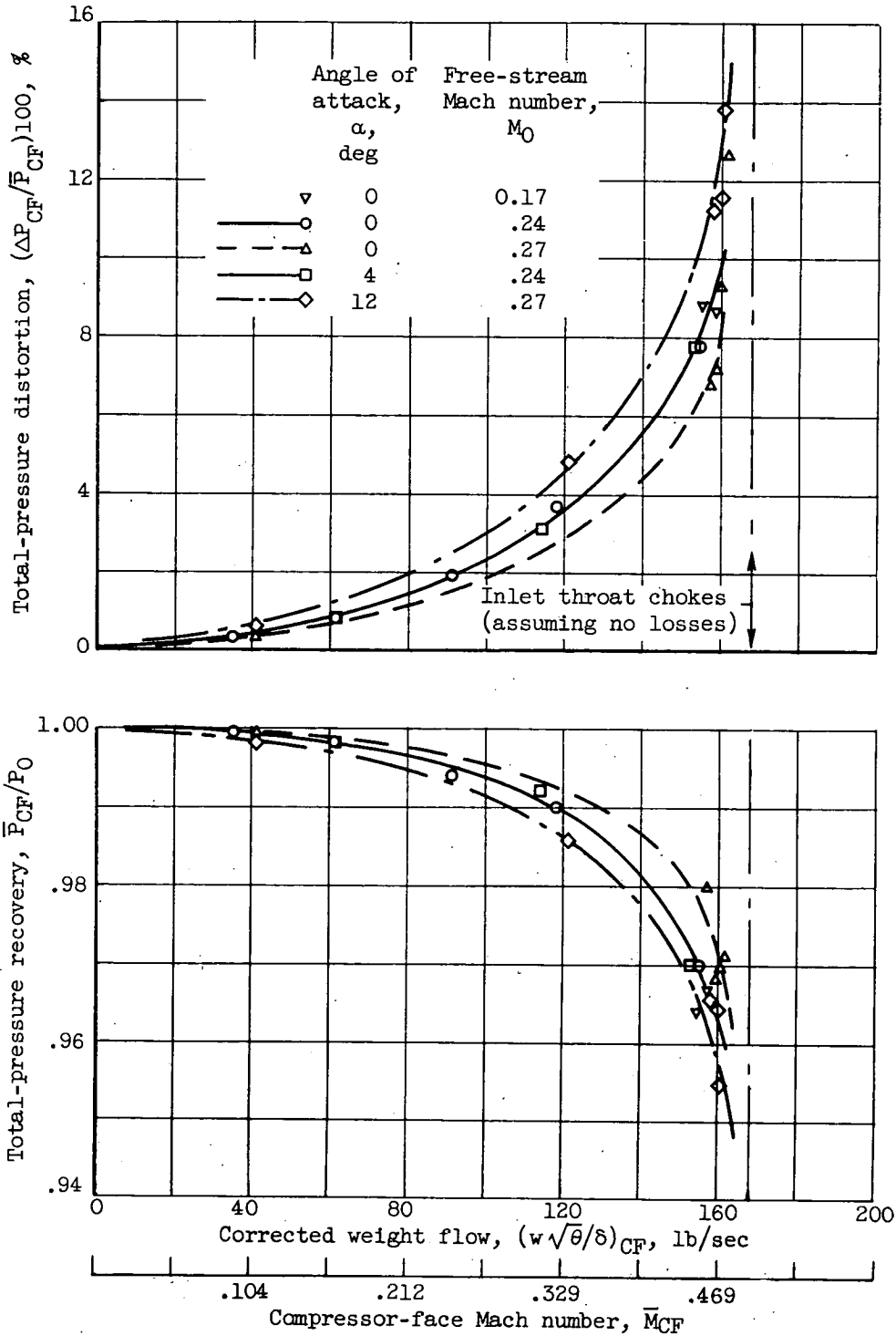
Figure 6. - Total-pressure distortion and recovery at diffuser exit (compressor face) of supersonic nose inlet in subsonic clear air.
