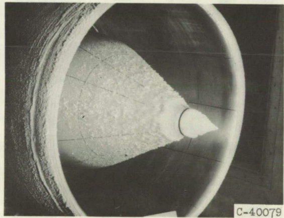
Photographs after 6\frac{3}{4} minutes of icing
