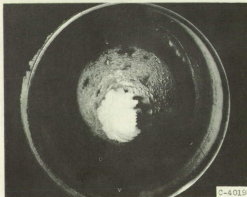
Photographs after 10\frac{1}{2} minutes of icing
