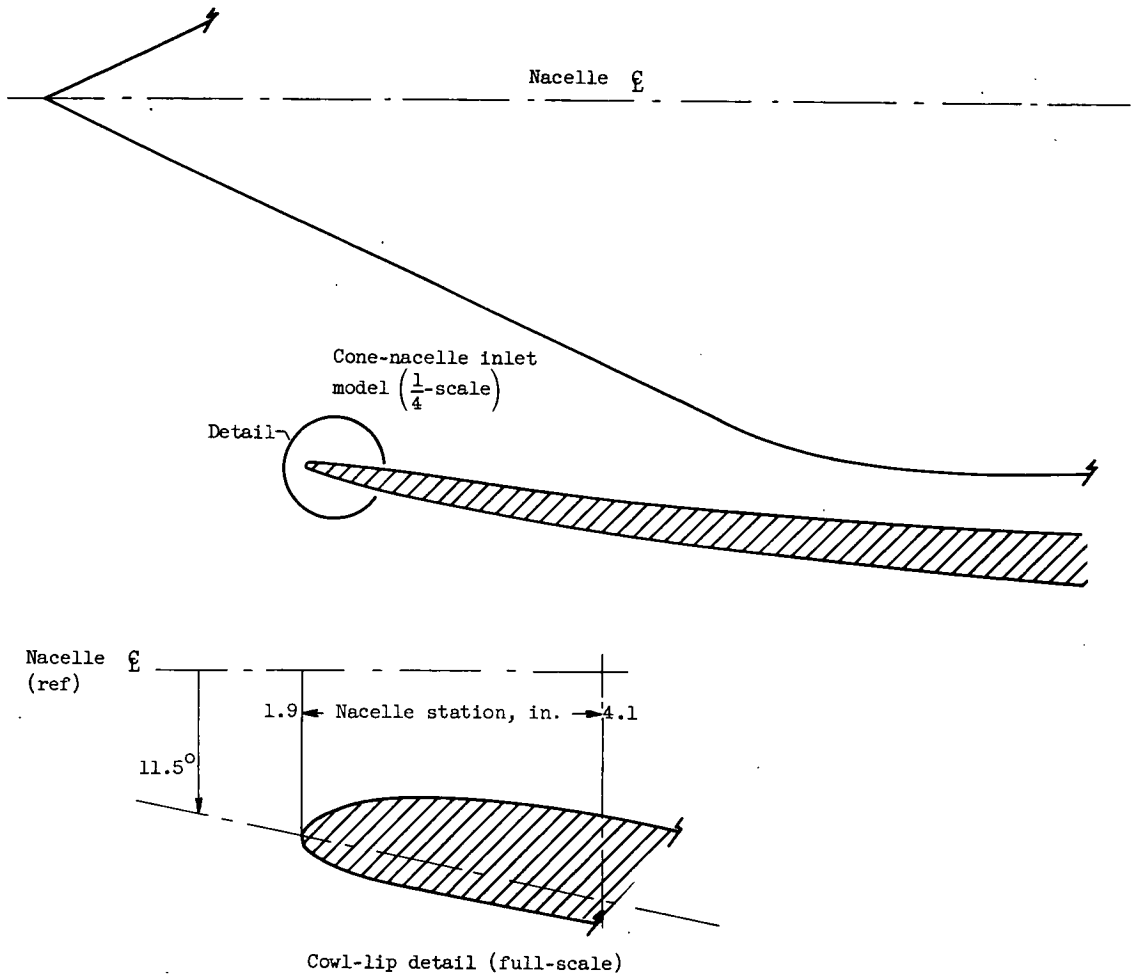
(d) Schematic drawing of centerbody and cowl-lip detail.
