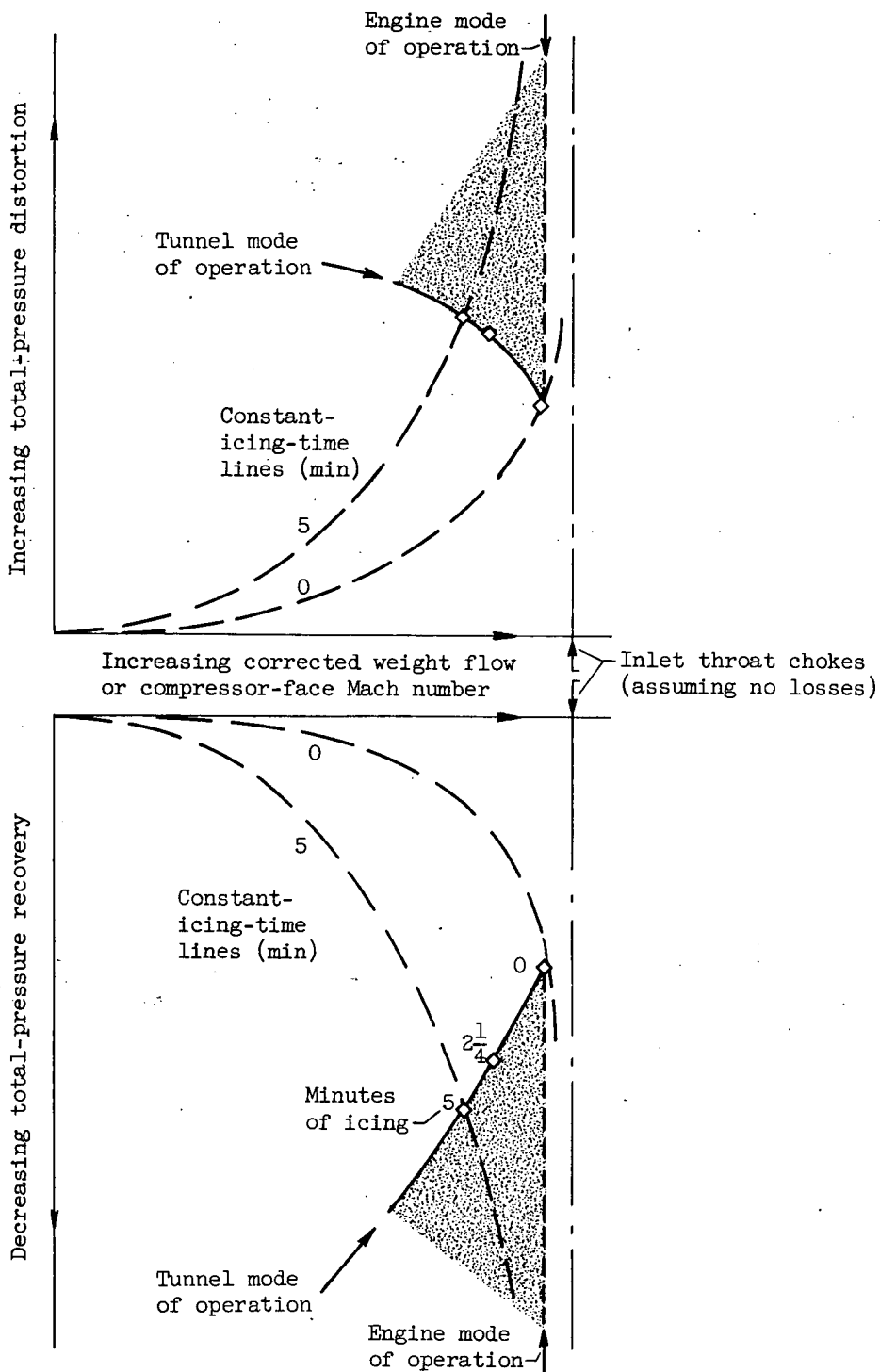
Figure 4. - Schematic drawing showing typical presentation of total-pressure distortion and recovery at diffuser exit (compressor face) of a supersonic nose inlet in subsonic flight and the effect of icing and mode of operation.
