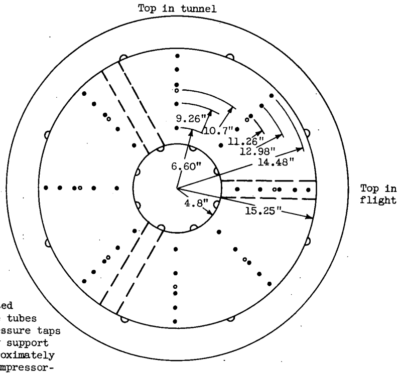
(b) Schematic cross section looking downstream at nacelle station 85 (compressor face) showing location of pressure tubes and taps.
