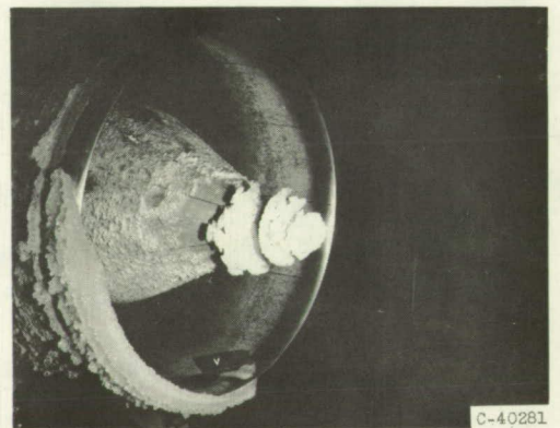
Photographs after 10\frac{1}{2} minutes of icing
