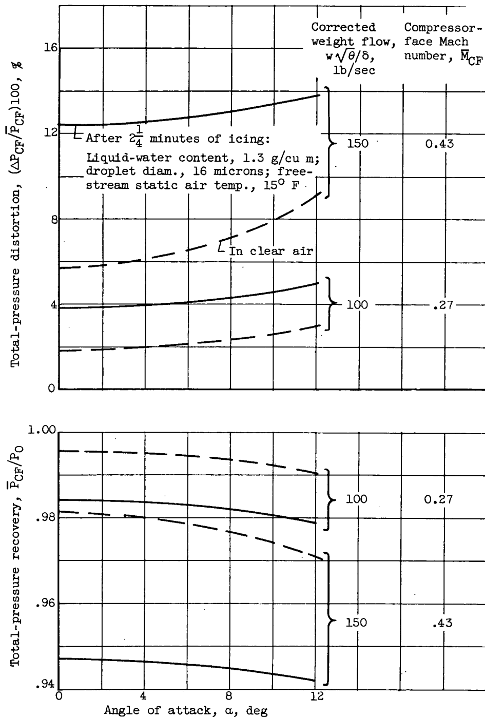
Figure 13. - Effect of angle of attack on total-pressure distortion and recovery at diffuser exit (compressor face) of supersonic nose inlet with constant corrected weight flow (engine mode of operation). Free-stream Mach number, 0.27.
