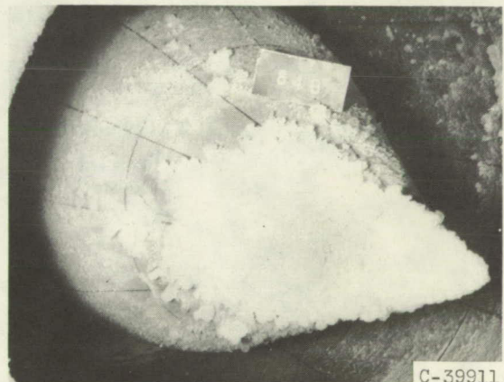
Photographs after 5 minutes of icing
