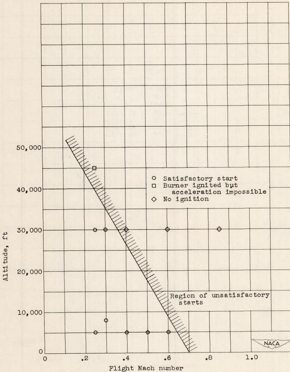
Figure 9. - Windmilling-starting characteristics.
