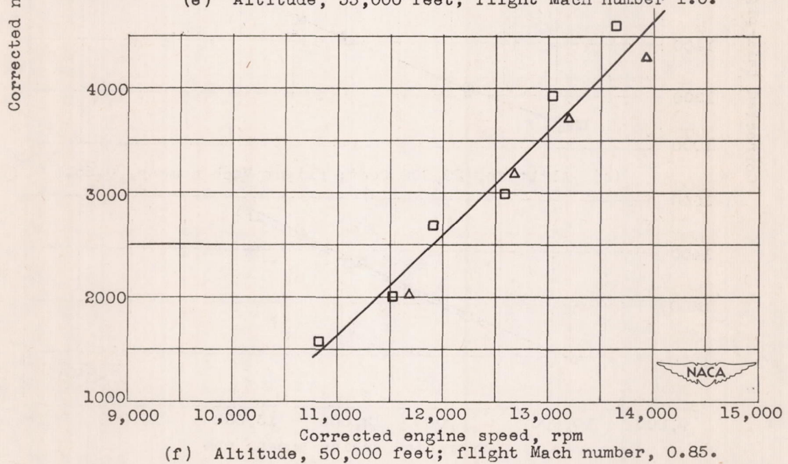
Figure 4. - Concluded. Comparison of corrected net thrust for AN-F-58 fuel and gasoline at various altitudes and flight Mach numbers.
