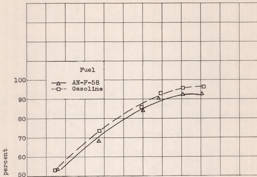
(c) Altitude, 20,000 feet; flight Mach number, 0.85.
