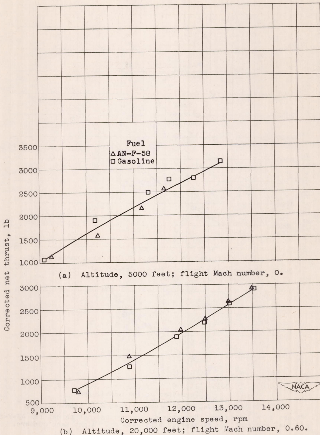
Figure 4. - Comparison of corrected net thrust for AN-F-58 fuel and gasoline at various altitudes and flight Mach numbers.
