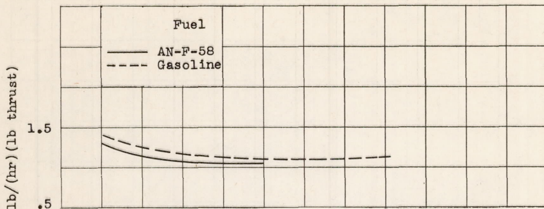
(a) Altitude, 5000 feet; flight Mach number, 0.
