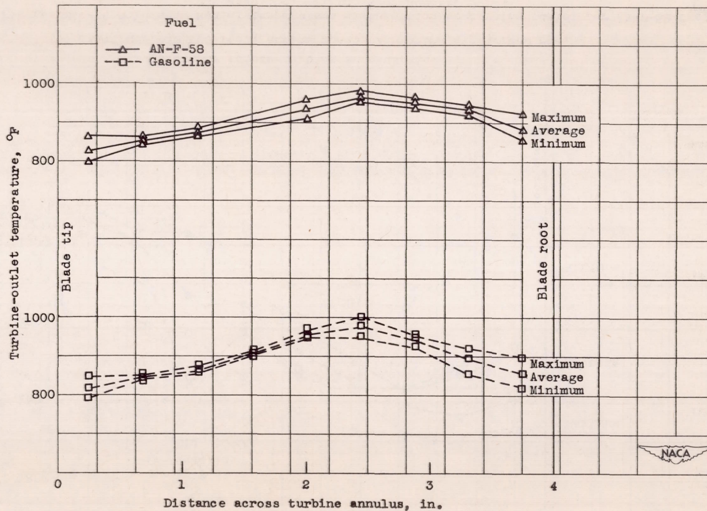
Figure 10. - Radial temperature distribution at turbine outlet for AN-F-58 fuel and gasoline. Flight Mach number, 0.85.
