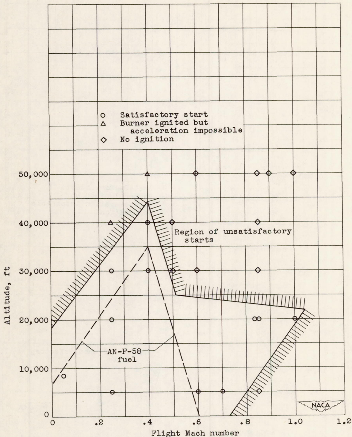
Figure 9. - Concluded. Windmilling-starting characteristics.
