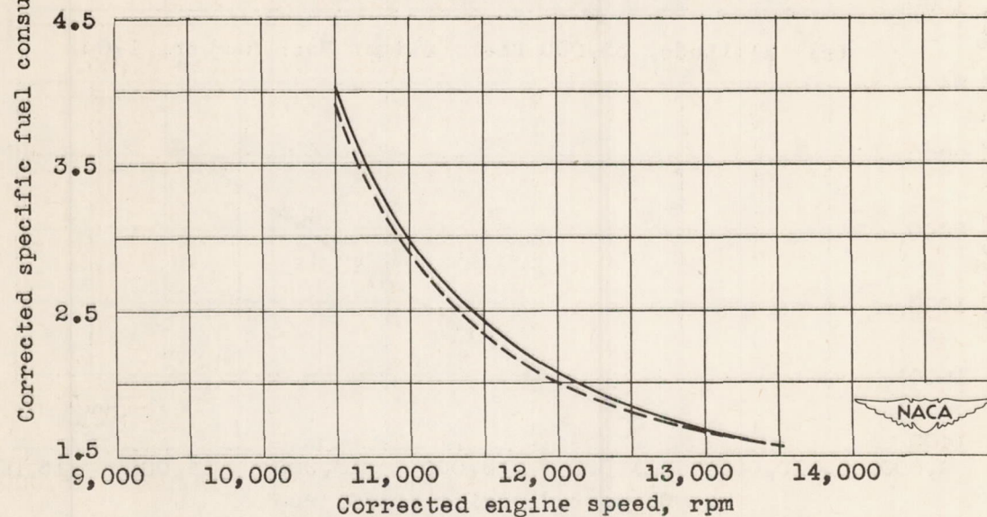
(c) Altitude, 20,000 feet; flight Mach number, 0.85.
