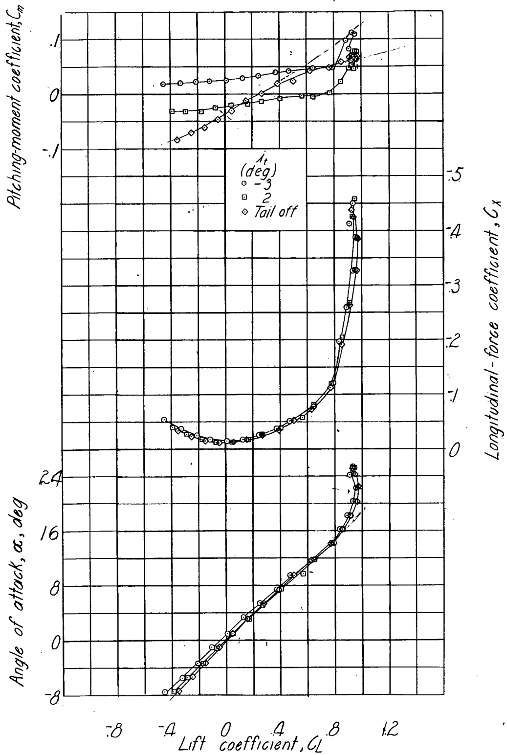
Figure 11.- Effect of stabilizer on the aerodynamic characteristics in pitch of a model with a 45.1 - 2.50 - .42 wing. \delta_f = 0^\circ ; \psi = 0^\circ ; r = 0^\circ ; test c.g. at 35.9 percent M.A.C.
