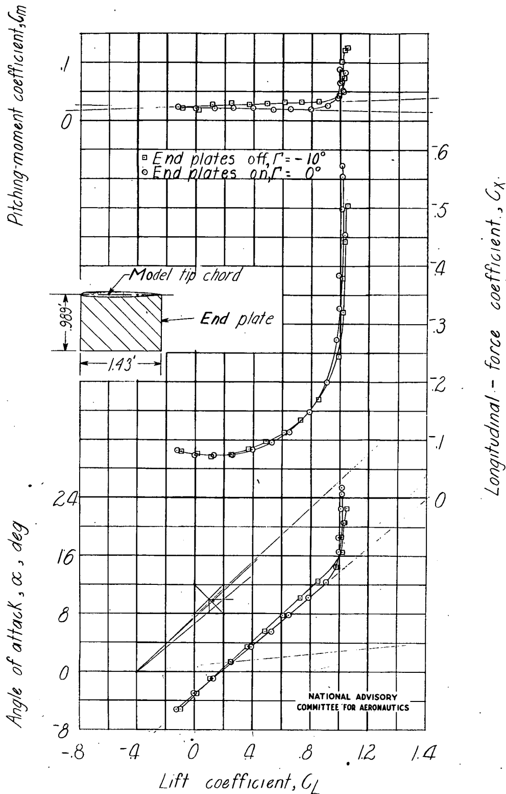
Figure 21.- Effect of end plates on the aerodynamic characteristics in pitch of a model with a 45.1 - 2.50 - .42 wing. \delta_f = 50^\circ ; \psi = 0^\circ ; test c.g. at 35.9 percent \bar{M}.A.C.
