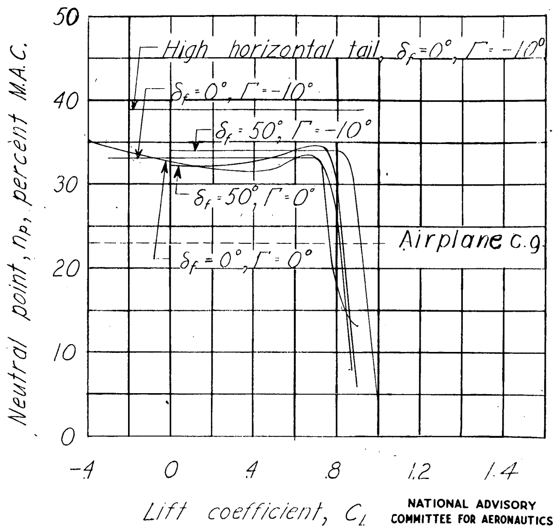
Figure 19.- Neutral points for a model with a 45.1 - 2.50 - .42 wing.
