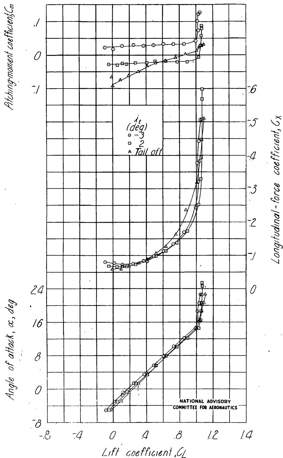
Figure 14.- Effect of stabilizer on the aerodynamic characteristics in pitch of a model with a 45.1 - 2.50 - .42 wing. \delta_f = 50^\circ ; \psi = 0^\circ ; r = -10^\circ ; test c.g. at 35.9 percent M.A.C.
