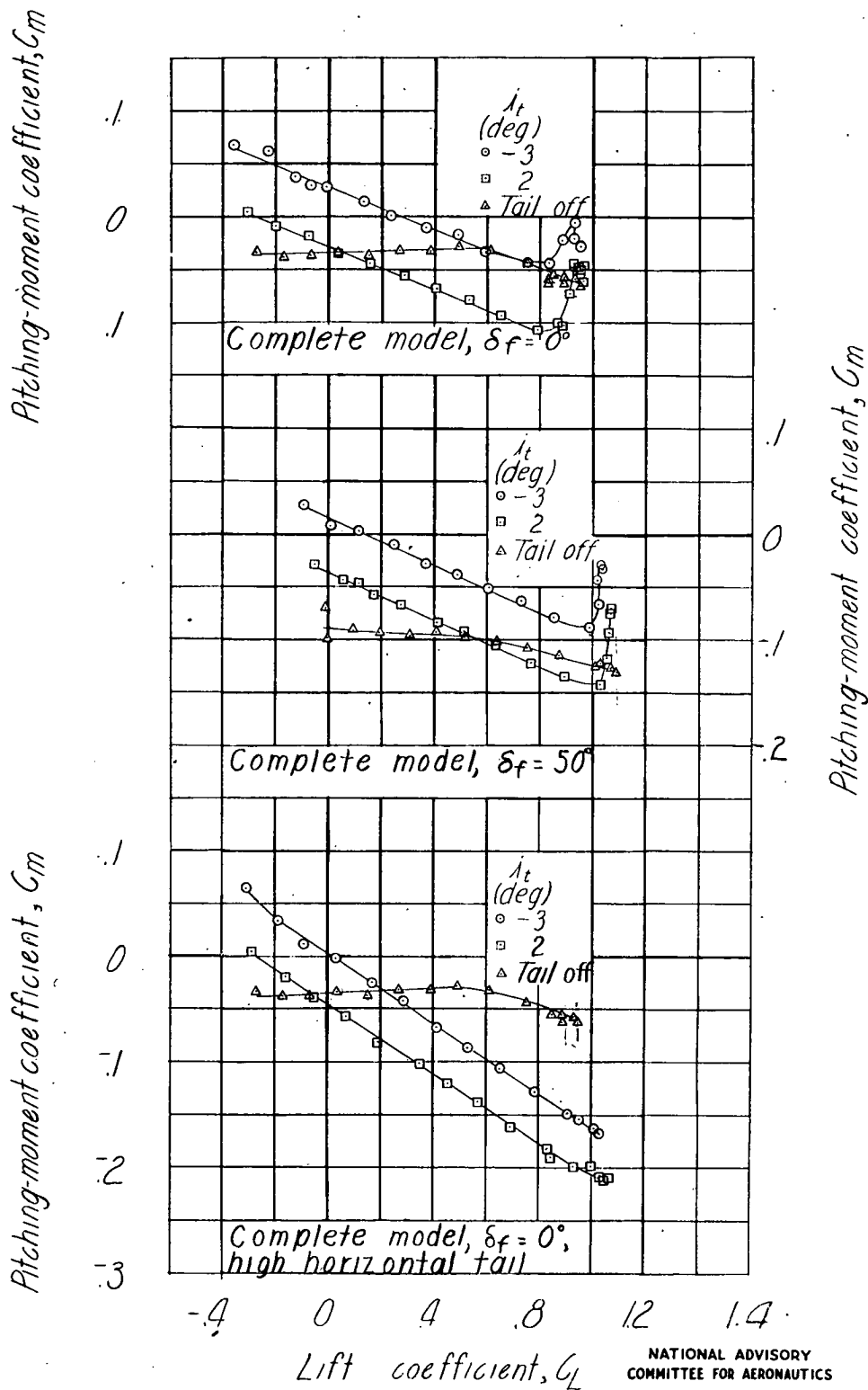
Figure 17.- Effect of stabilizer on the aerodynamic characteristics in pitch of a model with a 45.1 - 2.50 - .42 wing. \psi = 0^\circ ; \Gamma = -10^\circ ; center of gravity transferred to 23.0 percent M.A.C.
