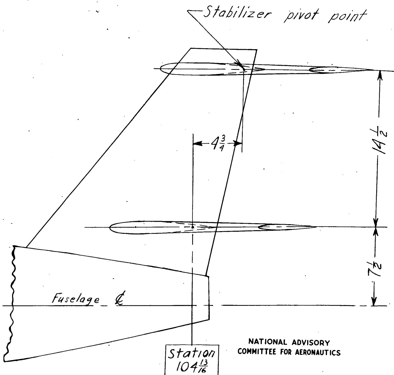
Figure 5.- Horizontal tail locations of model with a 45.1 - 2.50 - .42 wing. All dimensions are in inches.
