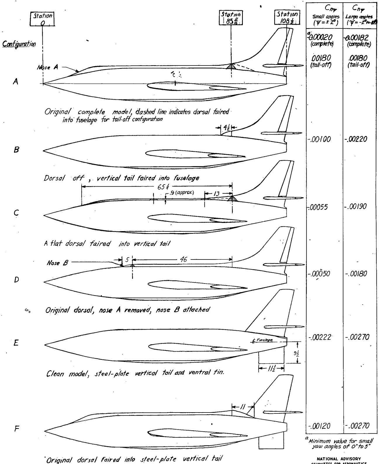
Figure 7.- Effect of dorsal and vertical-tail modifications on the directional stability of a model with a 45.1 - 2.50 - .42 wing.
