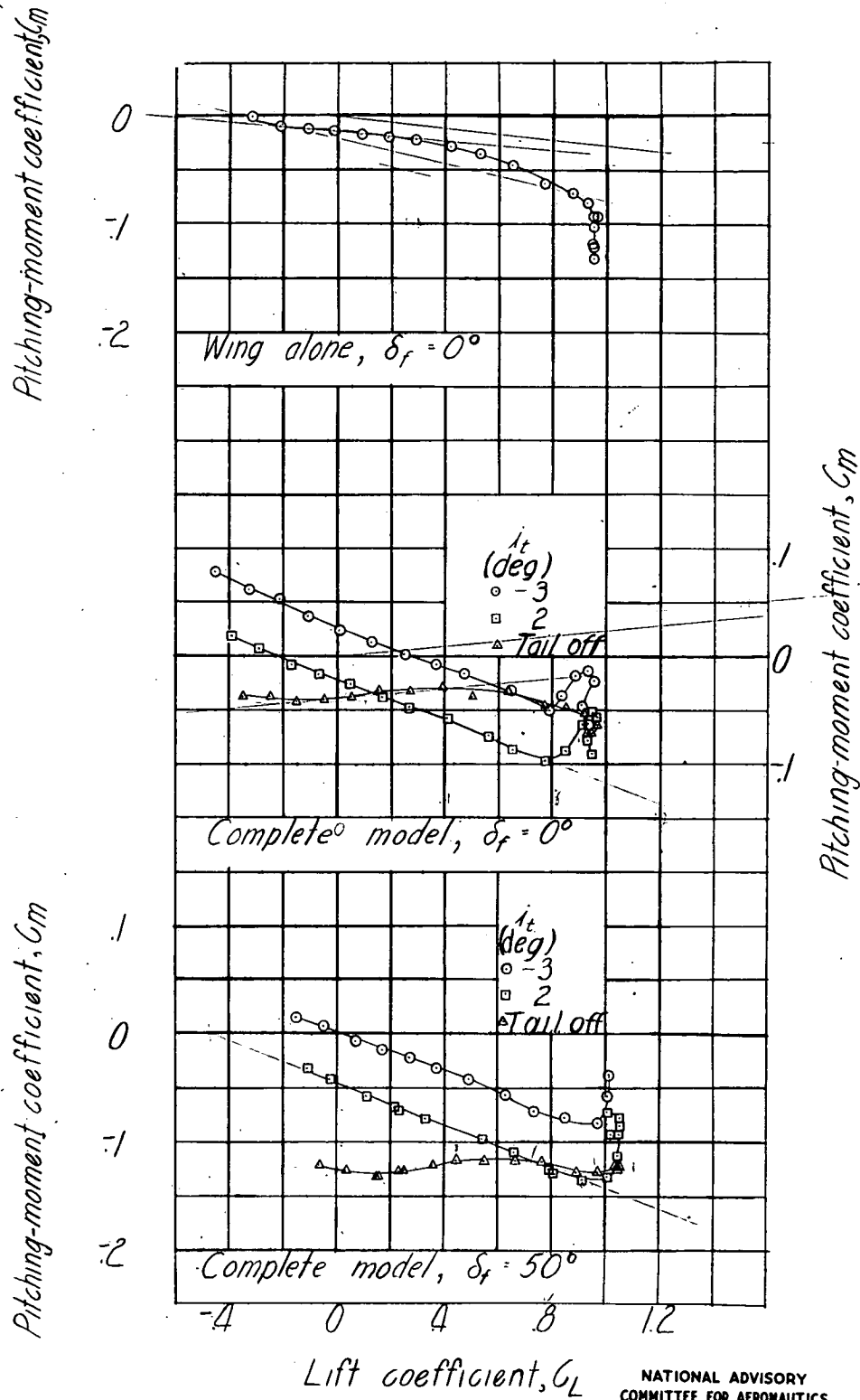
Figure 16.- Effect of stabilizer on the aerodynamic characteristics in pitch of a model with a 45.1 - 2.50 - .42 wing. \psi = 0^\circ ; \Gamma = 0^\circ ; center of gravity transferred to 23.0 percent M.A.C.
