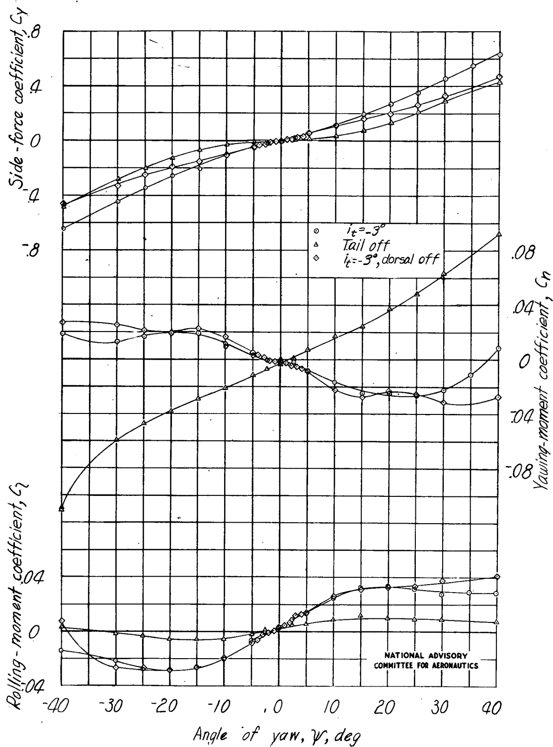
Figure 25.- Variation of the aerodynamic characteristics with angle of yaw for a model with a 45.1 - 2.50 - .42 wing. Original wing; r = 0^\circ .
