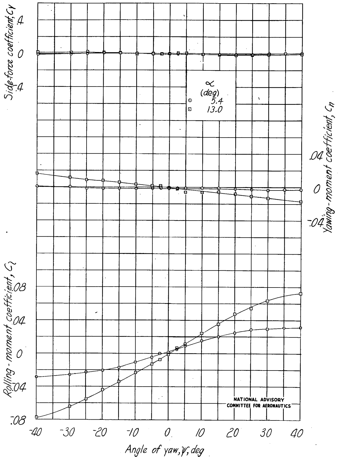
Figure 26.- The wing-alone aerodynamic characteristics in yaw of a model with a 45.1 - 2.50 - .42 wing. r = 0^\circ .
