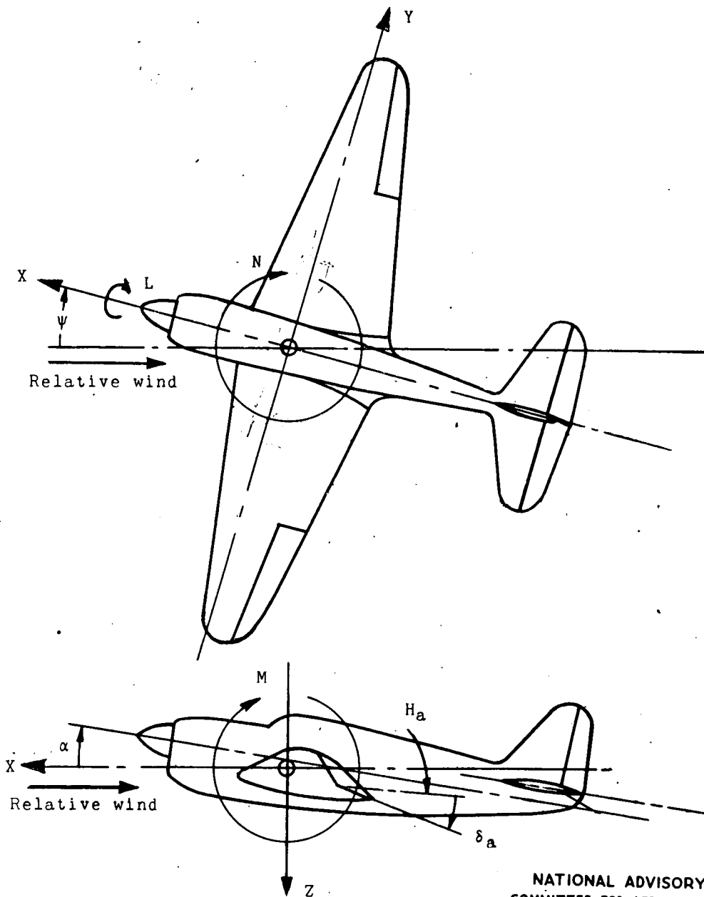
Figure 2.- System of axes and control-surface hinge moments and deflections. Positive values of forces, moments, and angles are indicated by arrows. Positive values of tab hinge moments and deflections are in the same directions as the positive values for the control surfaces to which the tabs are attached.
