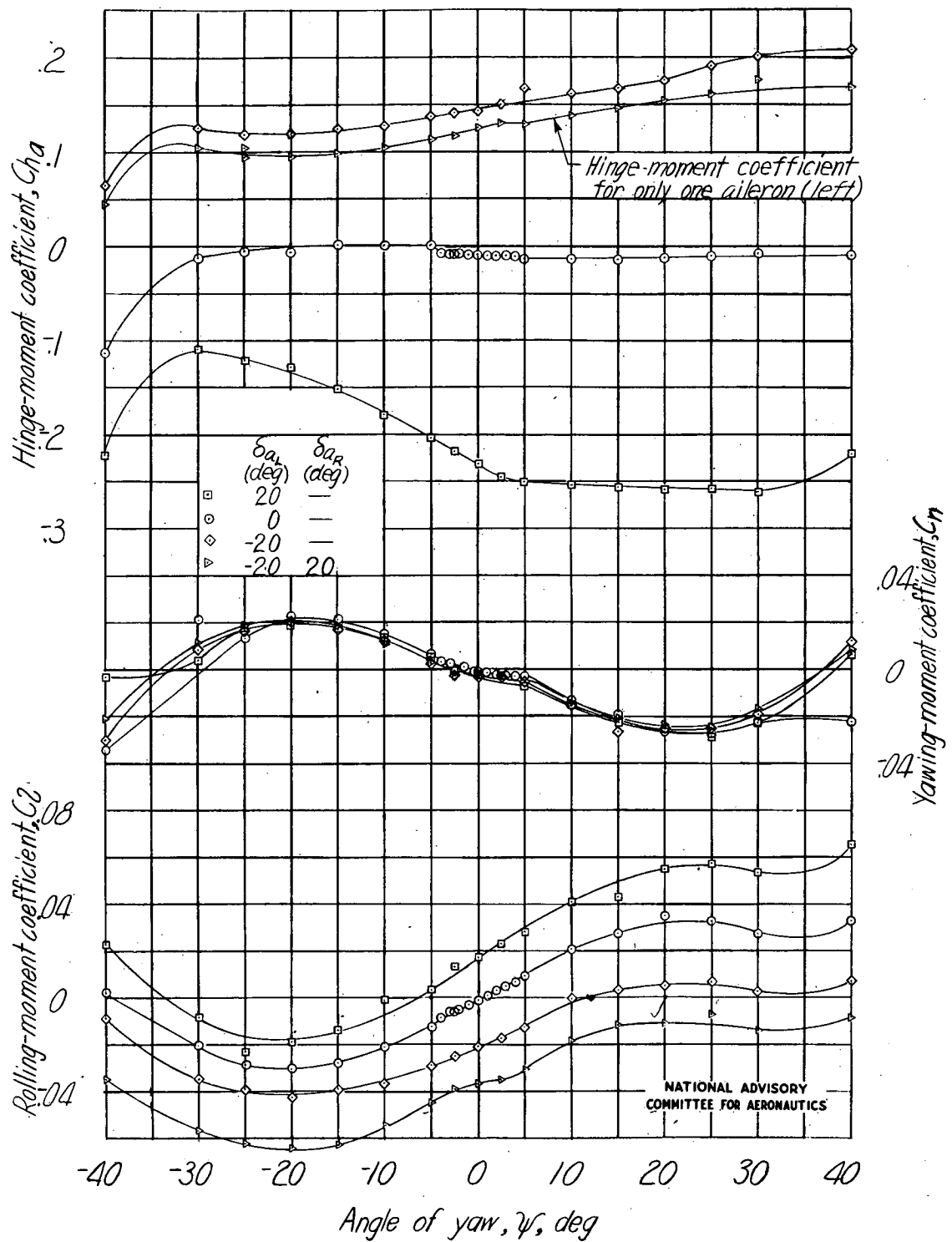
Figure 31.- Effect of aileron deflection on the aerodynamic characteristics in yaw of a model with a 45.1 - 2.50 - .42 wing. \Gamma = 0^\circ .
