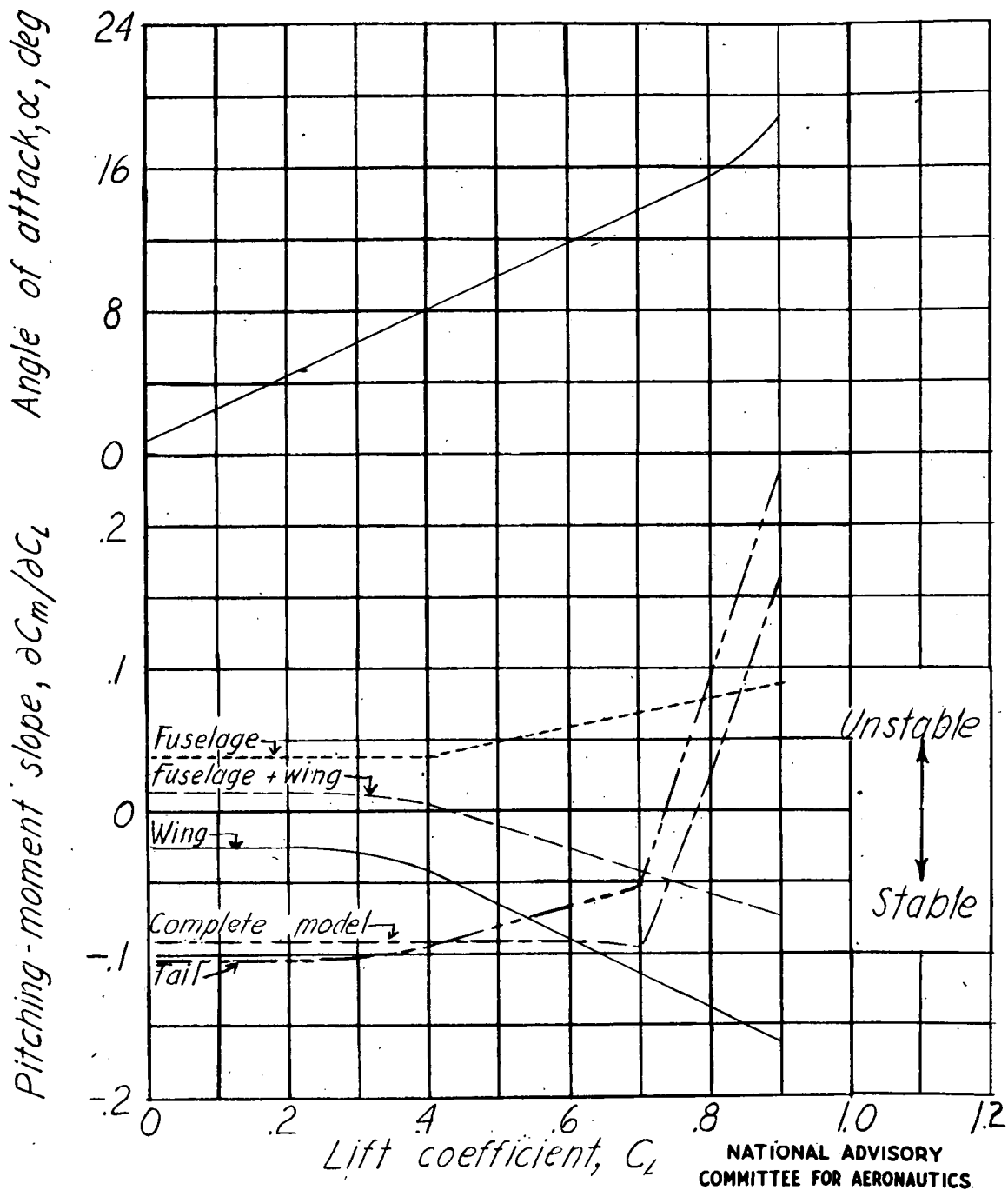
Figure 22.- Contribution of the various components to longitudinal stability of a model with a 45.1 - 2.50 - .42 wing. \delta_f = 0^\circ ; r = 0^\circ ; c.g. = 23 percent M.A.C.
