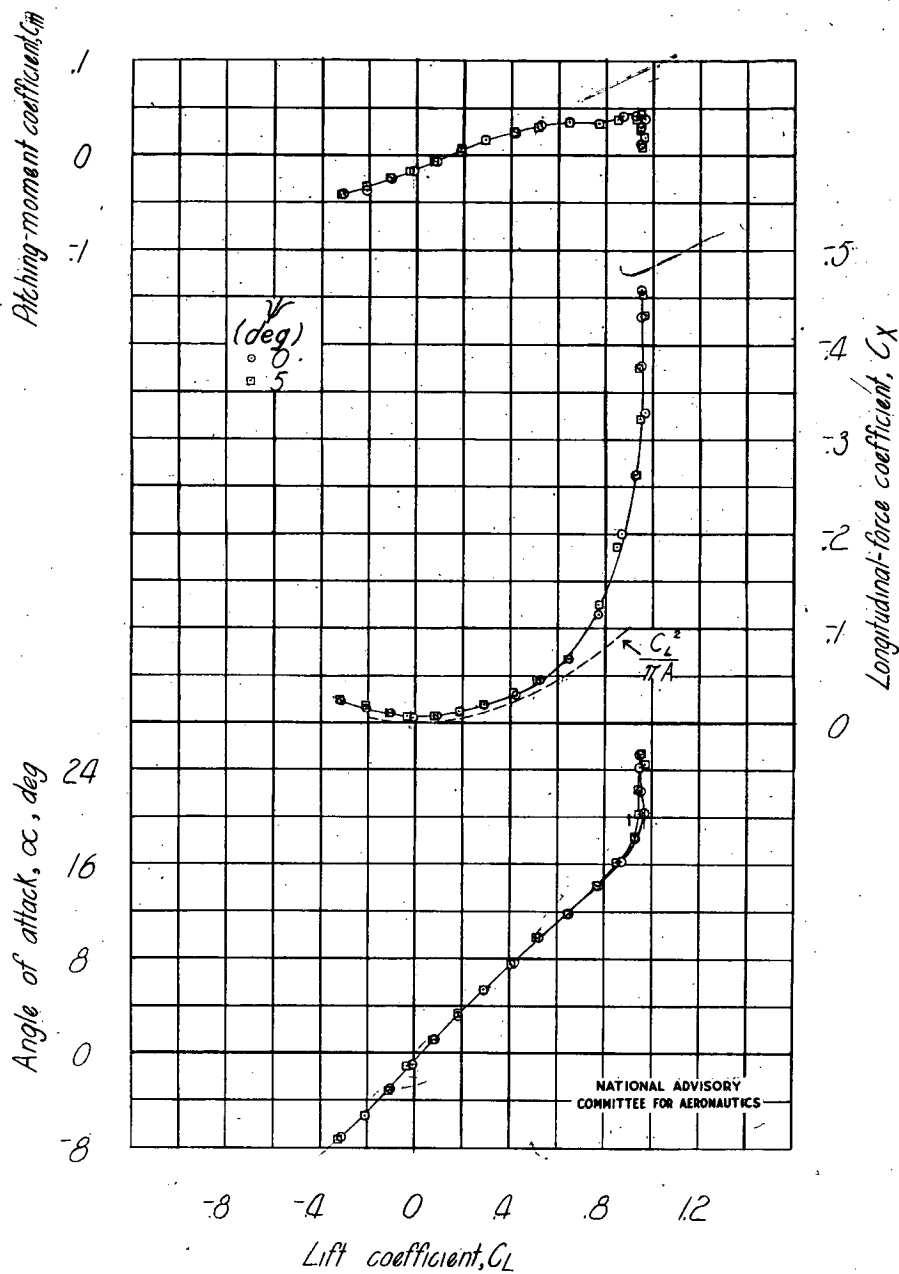
Figure 10.- Wing-alone characteristics in pitch of a model with a 45.1 - 2.50 - .42 wing. \delta_f = 0^\circ ; r = 0^\circ ; test c.g. at 35.9 percent M.A.C.
