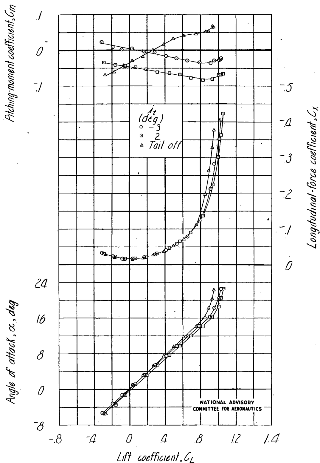
Figure 15.- Effect of stabilizer on the aerodynamic characteristics in pitch of a model with a 45.1 - 2.50 - .42 wing. \delta_f = 0^\circ ; \psi = 0^\circ ; \Gamma = -10^\circ ; test c.g. at 35.9 percent M.A.C.
