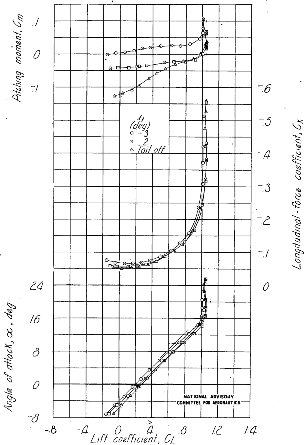
Figure 12.- Effect of stabilizer on the aerodynamic characteristics in pitch of a model with a 45.1 - 2.50 - .42 wing. \delta_f = 50^\circ ; \psi = 0^\circ ; \Gamma = 0^\circ ; test c.g. at 35.9 percent M.A.C.
