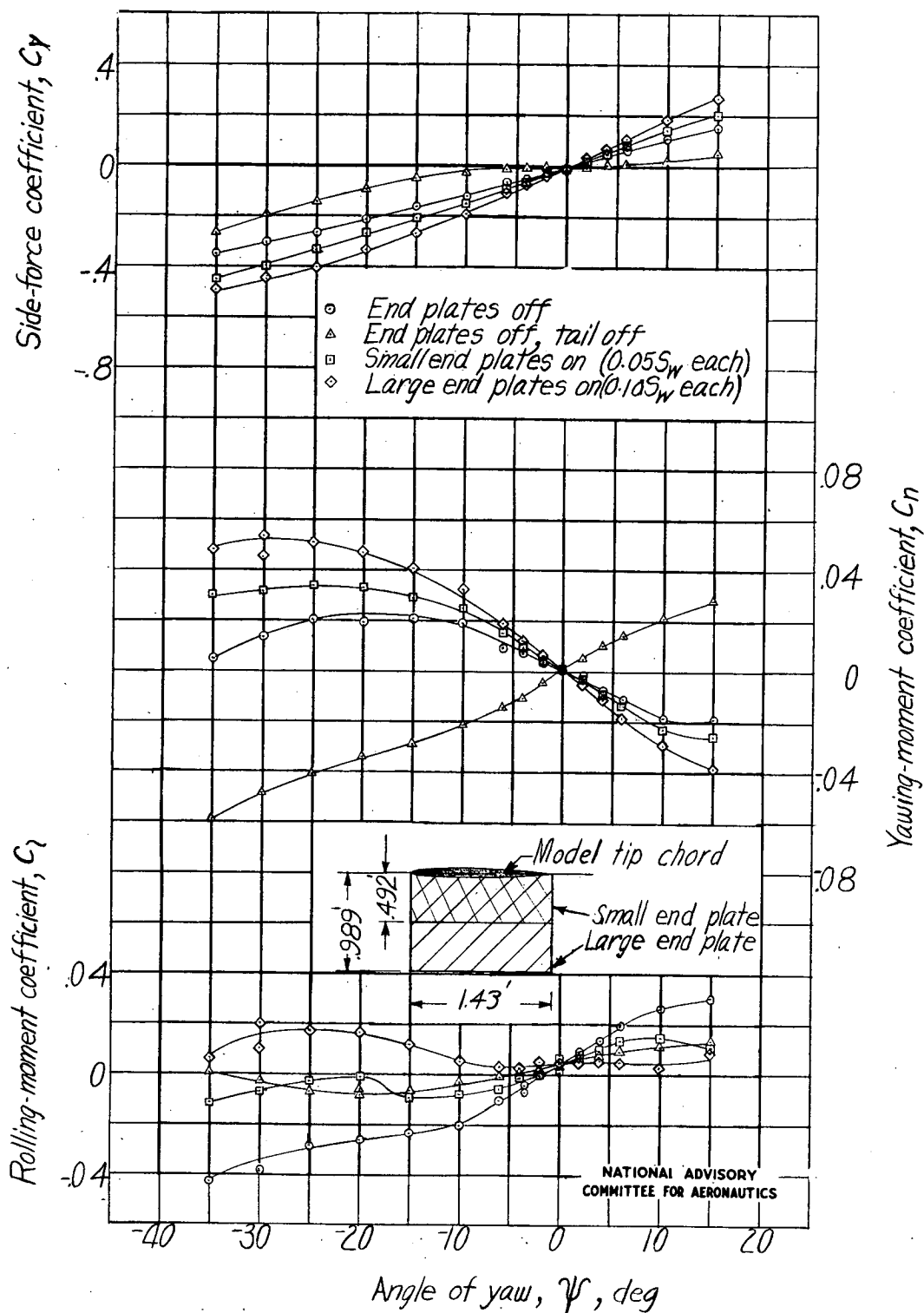
Figure 29.- Effect of end plates on the aerodynamic characteristics i yaw of a model with a 45.1 - 2.50 - .42 wing. r = 0^\circ .
