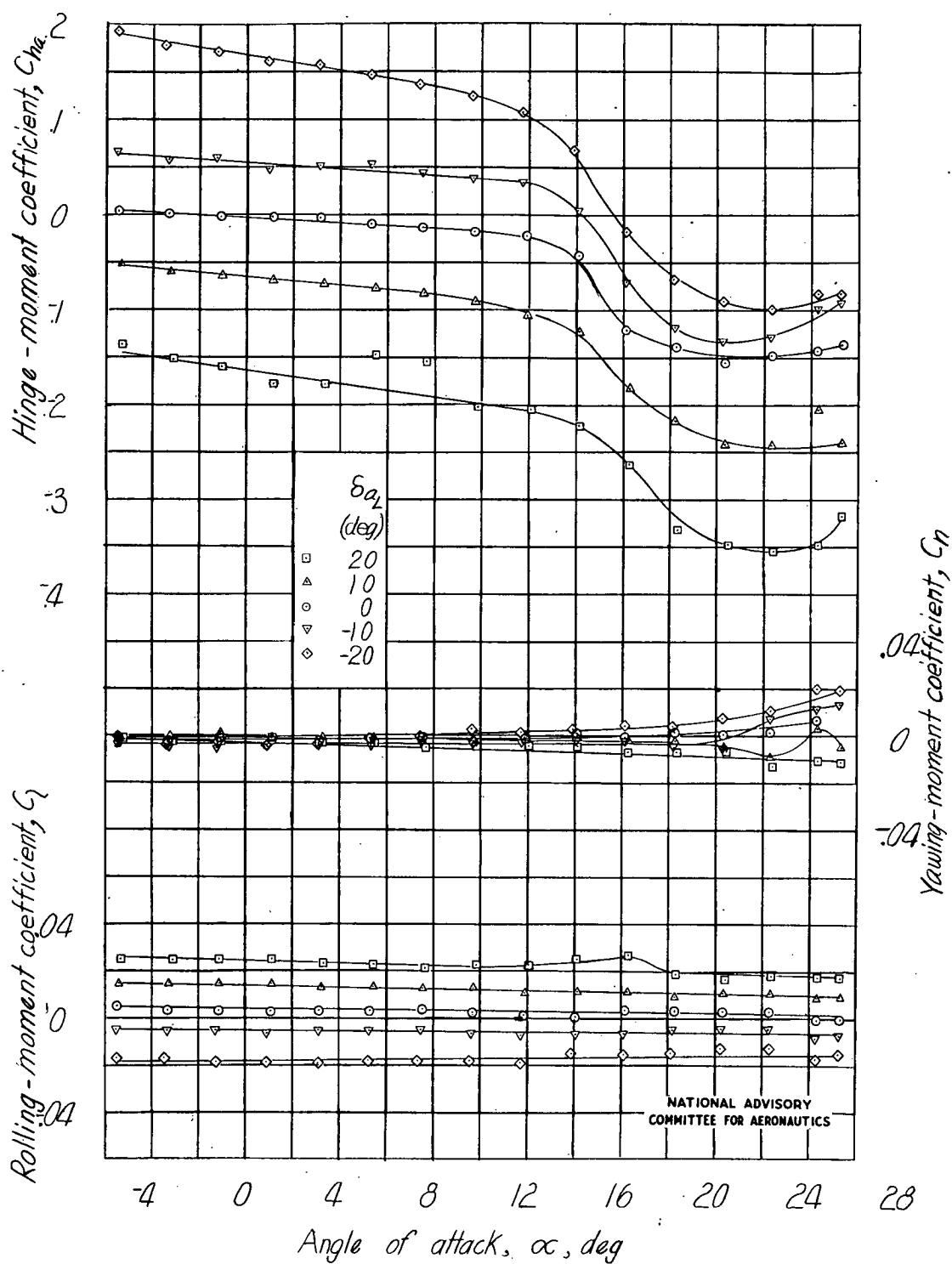
Figure 30.- Effect of aileron deflection on the aerodynamic characteristics in pitch at various angles of attack of a model with a 45.1 - 2.50 - .42 wing. \Gamma = 0^\circ .
