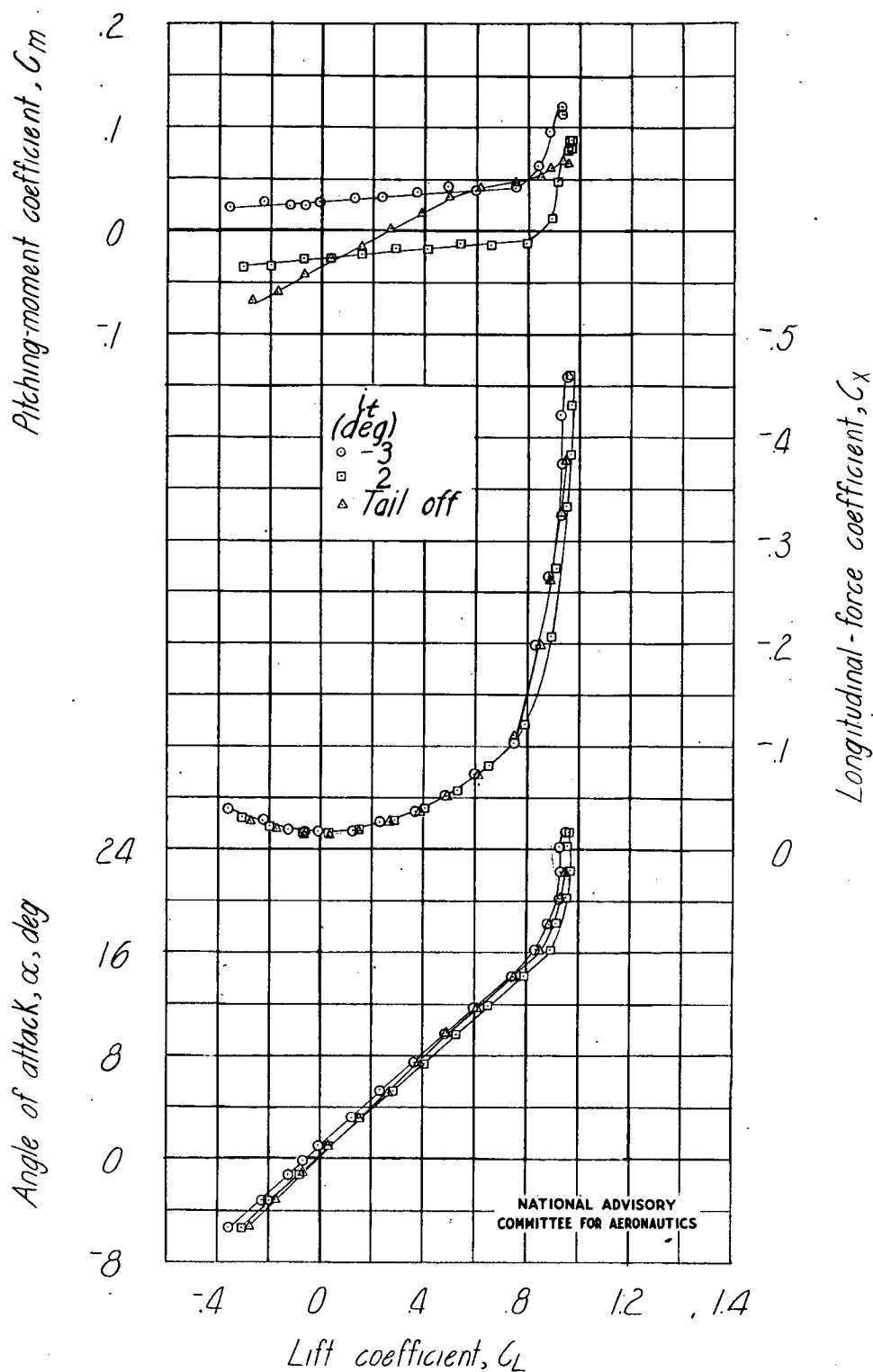
Figure 13.- Effect of stabilizer on the aerodynamic characteristics in pitch of a model with a 45.1 - 2.50 - .42 wing. \delta_f = 0^\circ ; \psi = 0^\circ ; r = -10^\circ ; test c.g. at 35.9 percent M.A.C.
