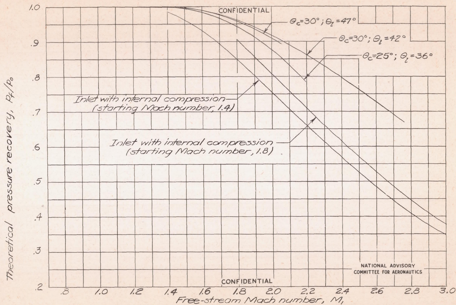
Figure 5.- Theoretical supersonic pressure recovery as a function of the free-stream Mach number. (Curves for inlet with internal compression from reference 2.)
