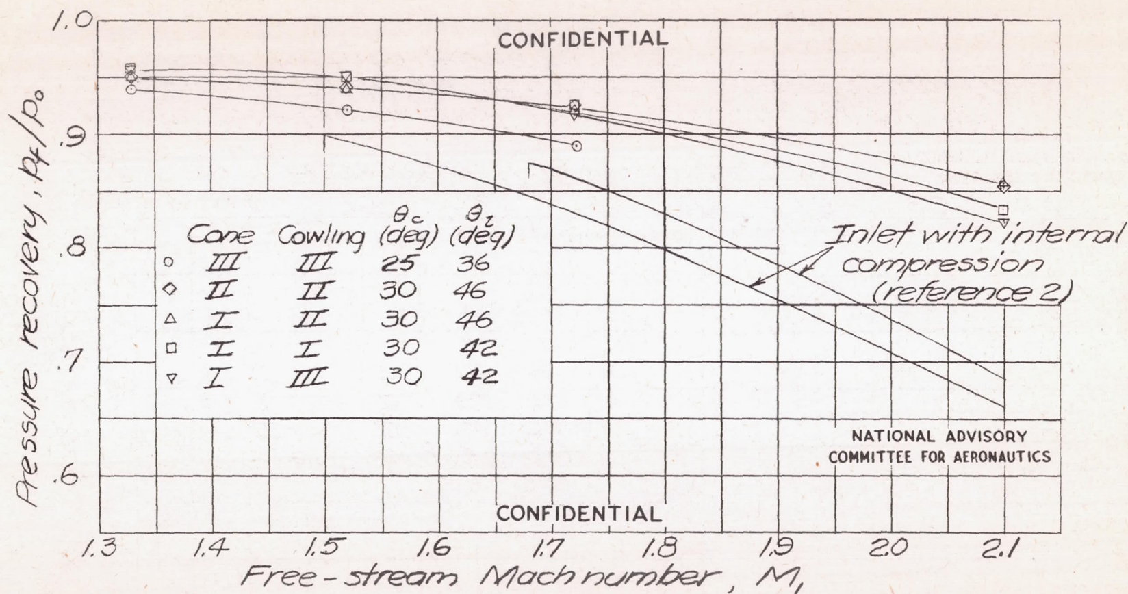
Figure 15. - Experimental values of pressure recovery for the optimum conditions as a function of free-stream Mach number for fixed-geometry inlet.
