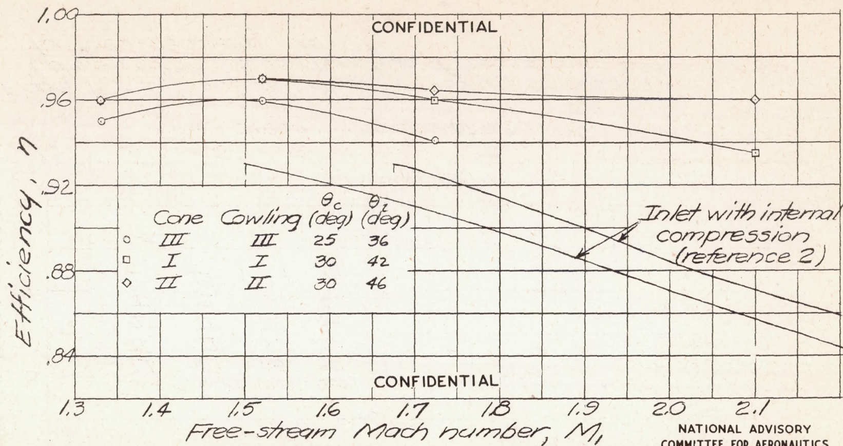
Figure 16. - Experimental values of efficiency for the optimum conditions as a function of free-stream Mach number for fixed-geometry inlet.
