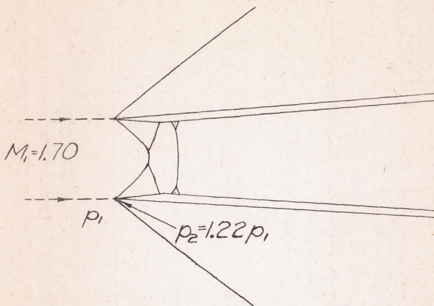
(a) Mass flow corresponding to design condition.
