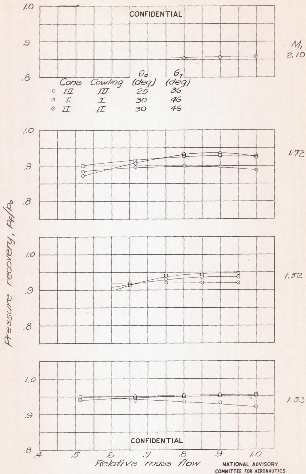
Figure 17.— Variation of pressure recovery with the relative mass flow.
