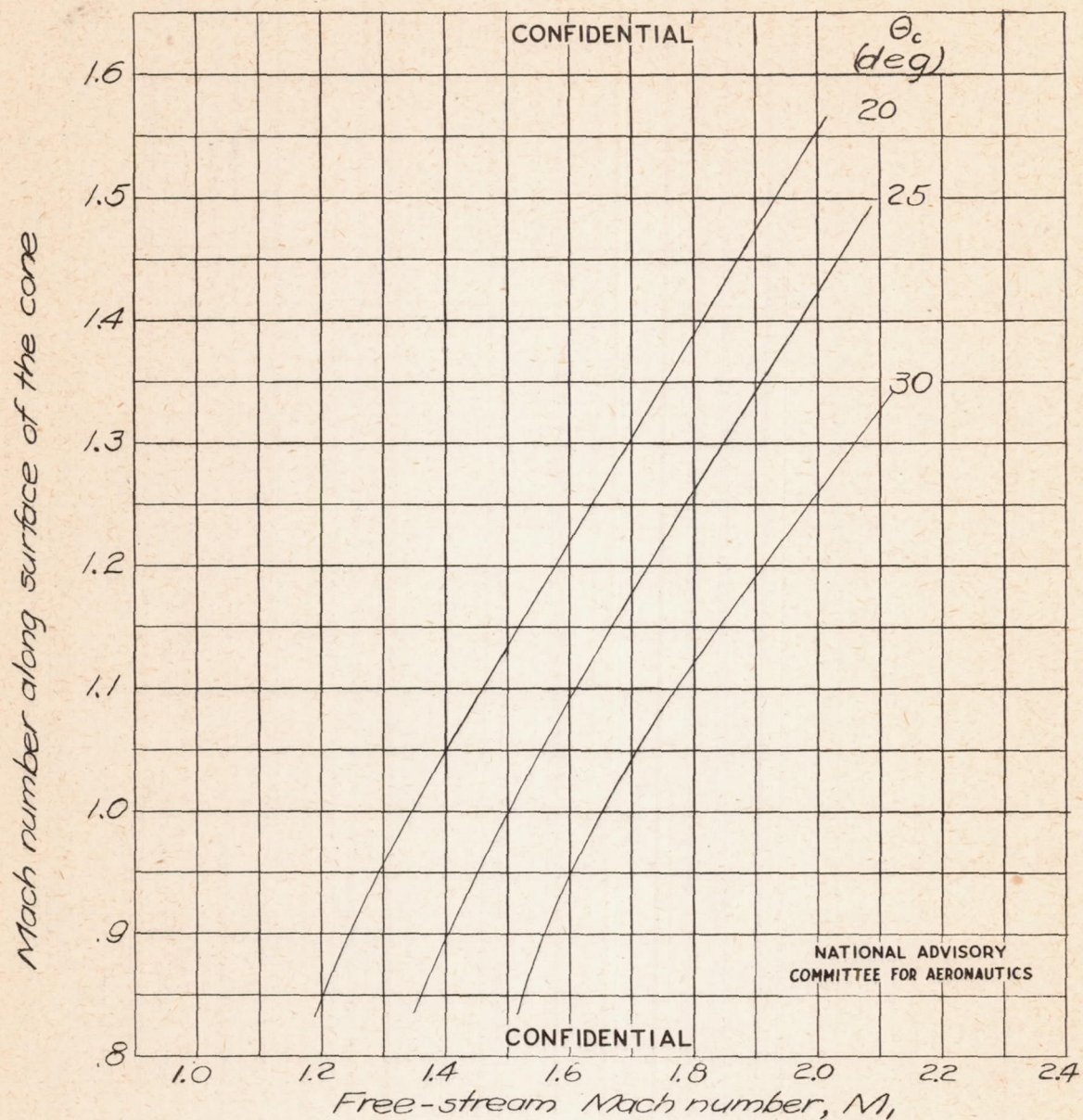
Figure 6.- Mach number along surface of the cone as a function of the free-stream Mach number.
