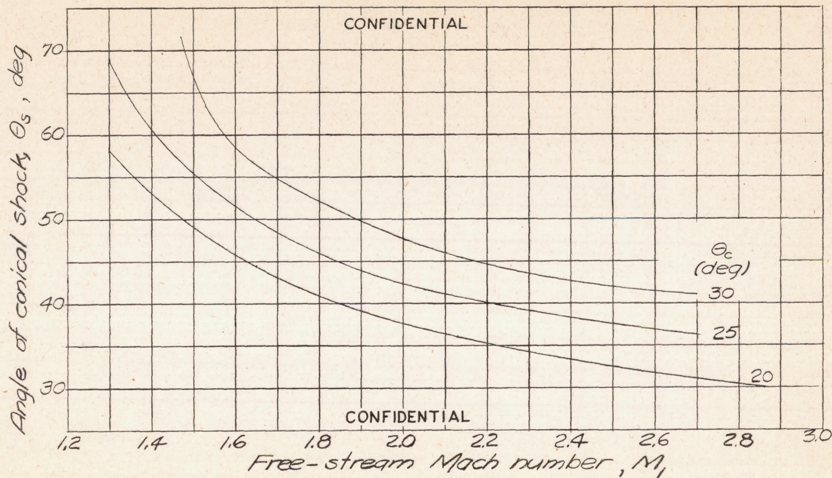
Figure 4 . - Angle of conical shock as a function of the free-stream Mach number.
