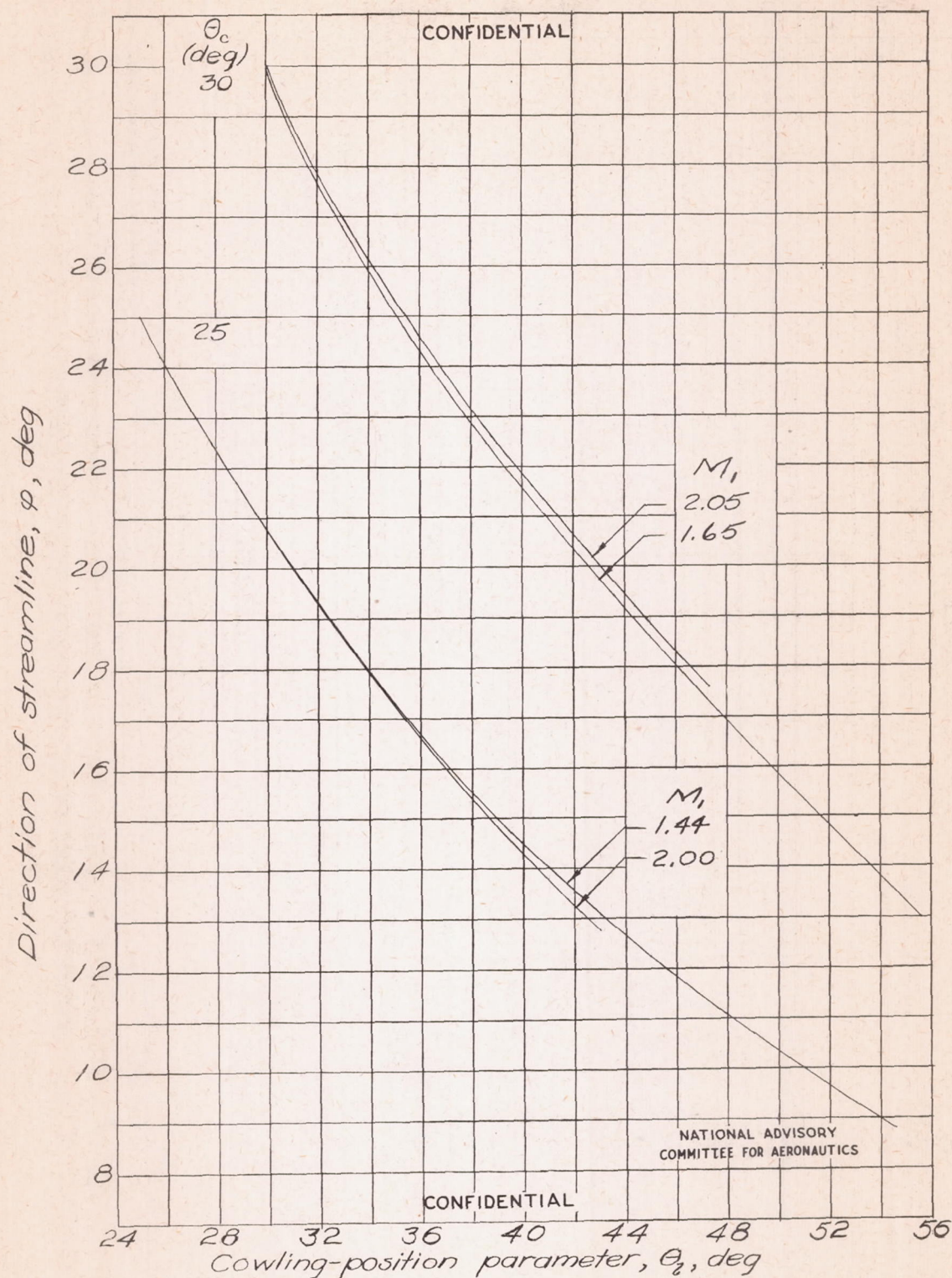
Figure 7.—Direction of the streamline for different Mach numbers and cone angles as a function of cowling-position parameter.
