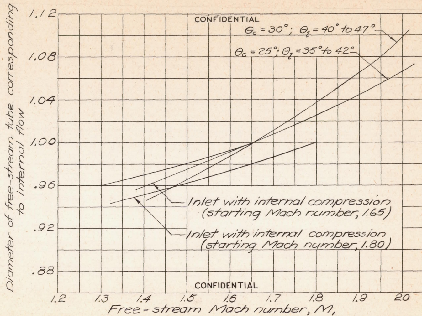
Figure 8.- Diameter of the free-stream tube of the internal flow as a function of the free-stream Mach number.
