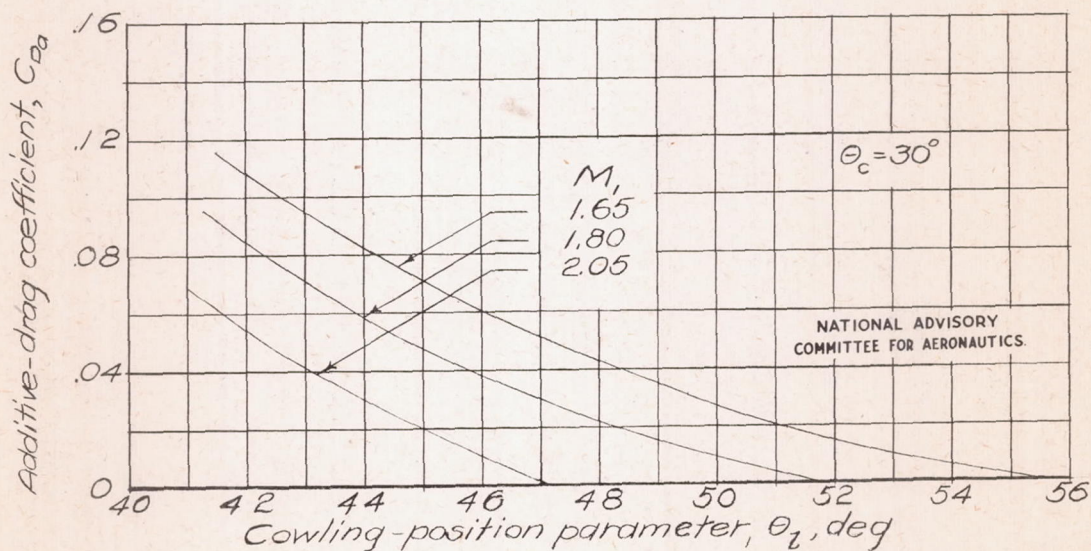
Figure 3.- Additive-drag coefficient as a function of cowling-position parameter.
