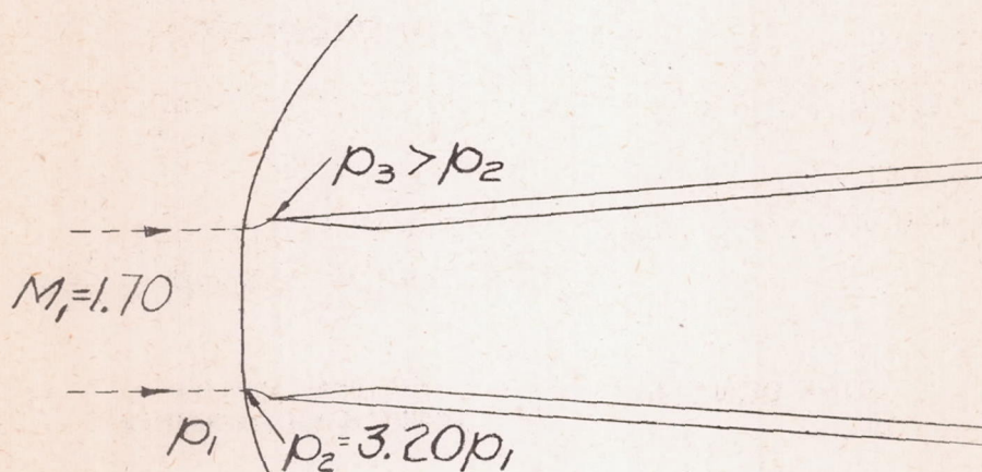
(b) Mass flow lower than value for design condition.
