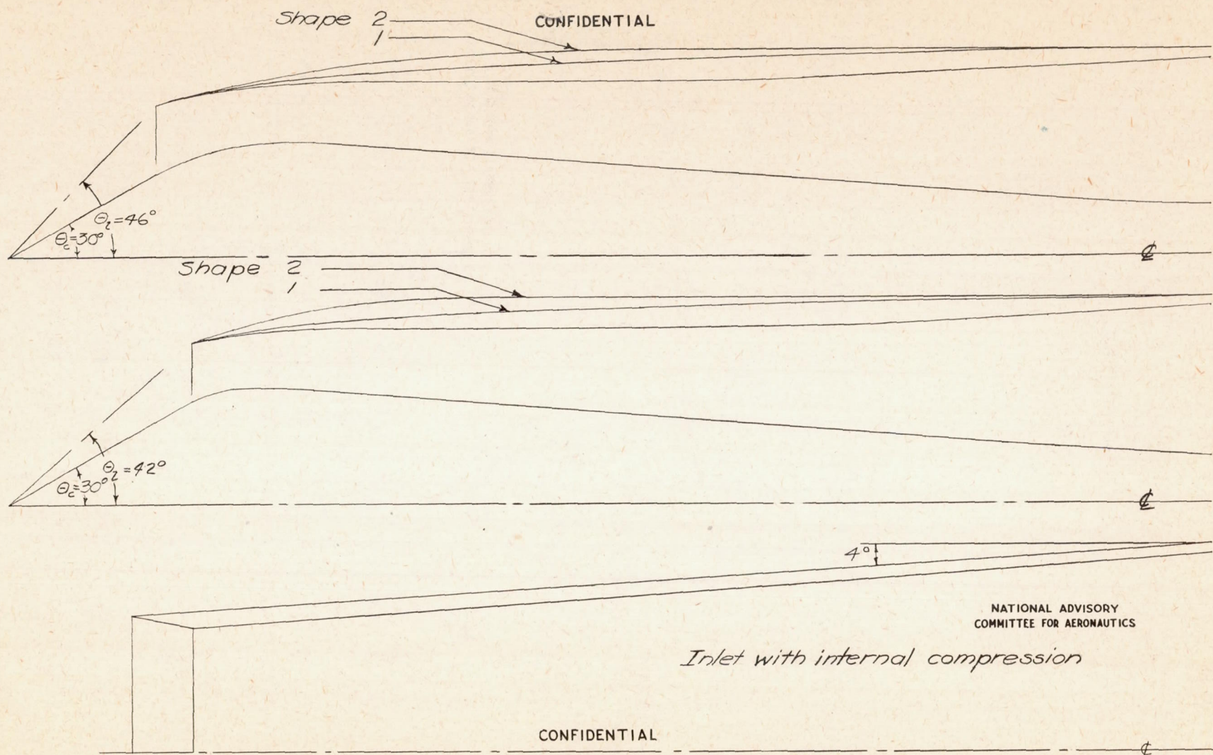
Figure 10.- The external shapes of the inlets with external compression and the inlet with internal compression used to determine the external drag.
