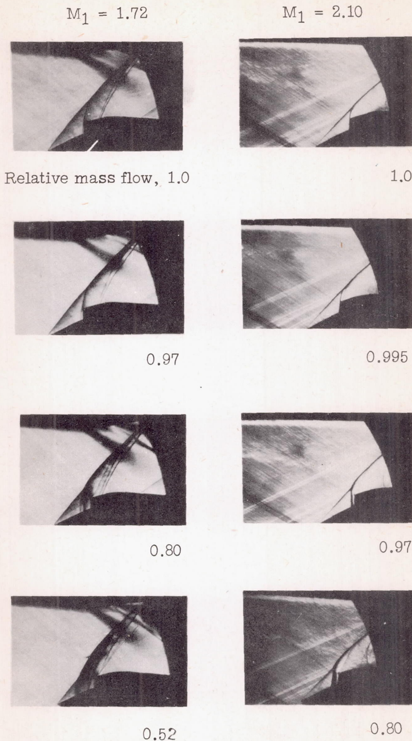
Figure 14.- Schlieren photographs for the inlet with internal compression for different values of relative mass flow. \theta_c = 30^\circ , \theta_l = 42^\circ .
