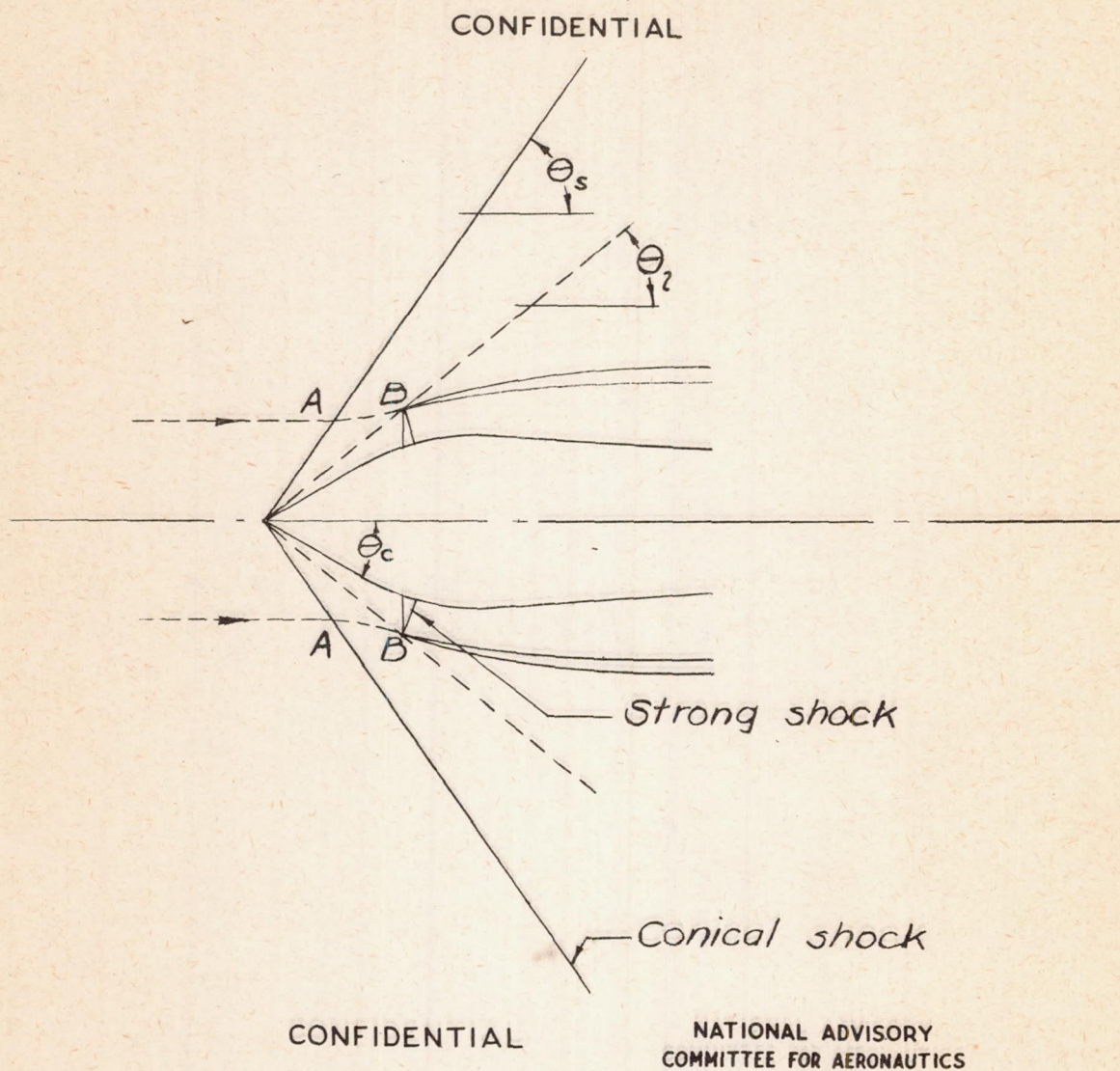
Figure 2. - Arrangement of the inlet considered.
