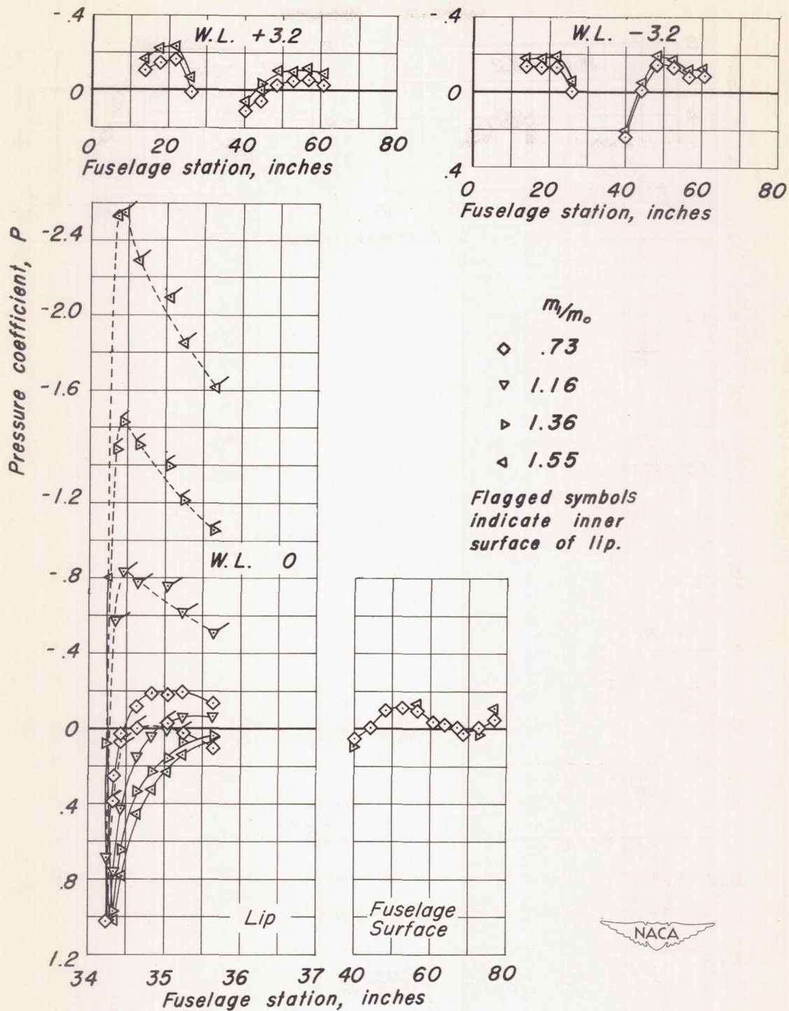
Figure 13.- Pressure distribution on inner and outer surface of lip and on fuselage surface adjacent to ramp.
