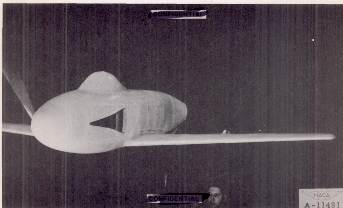
Figure 1.— Model with the inlets at fuselage station 34.25.
