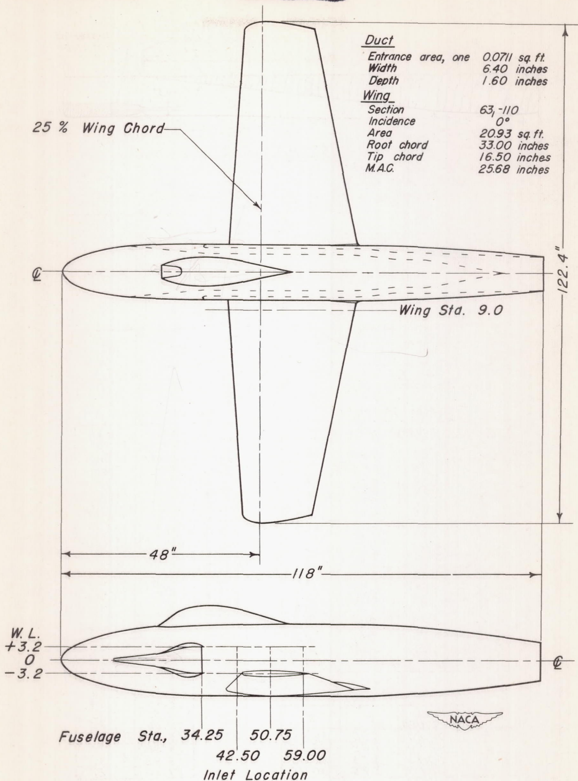
Figure 2. — Submerged-inlet model.
