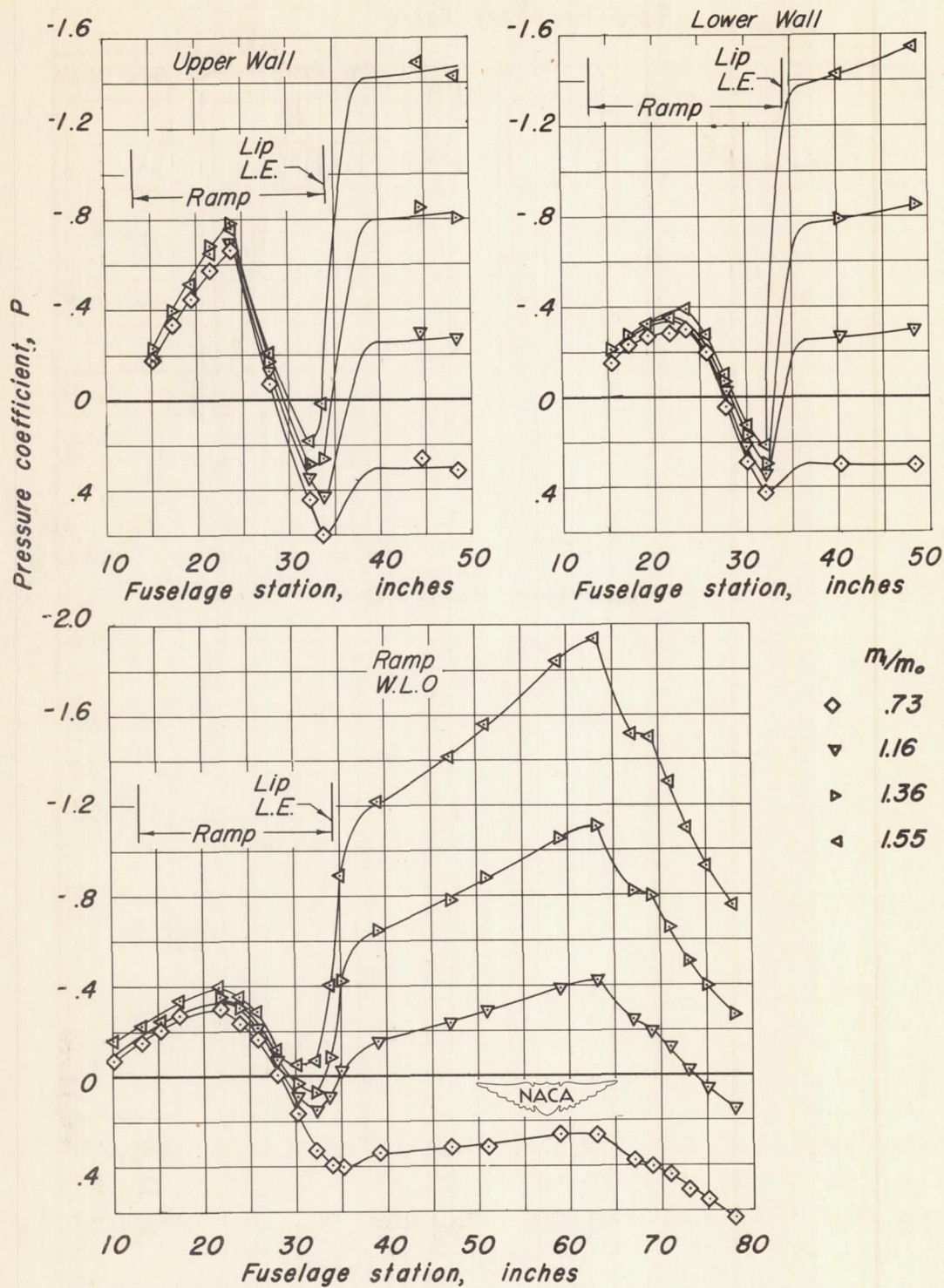
Figure 12.- Pressure distribution along the ramp and inside the duct.
