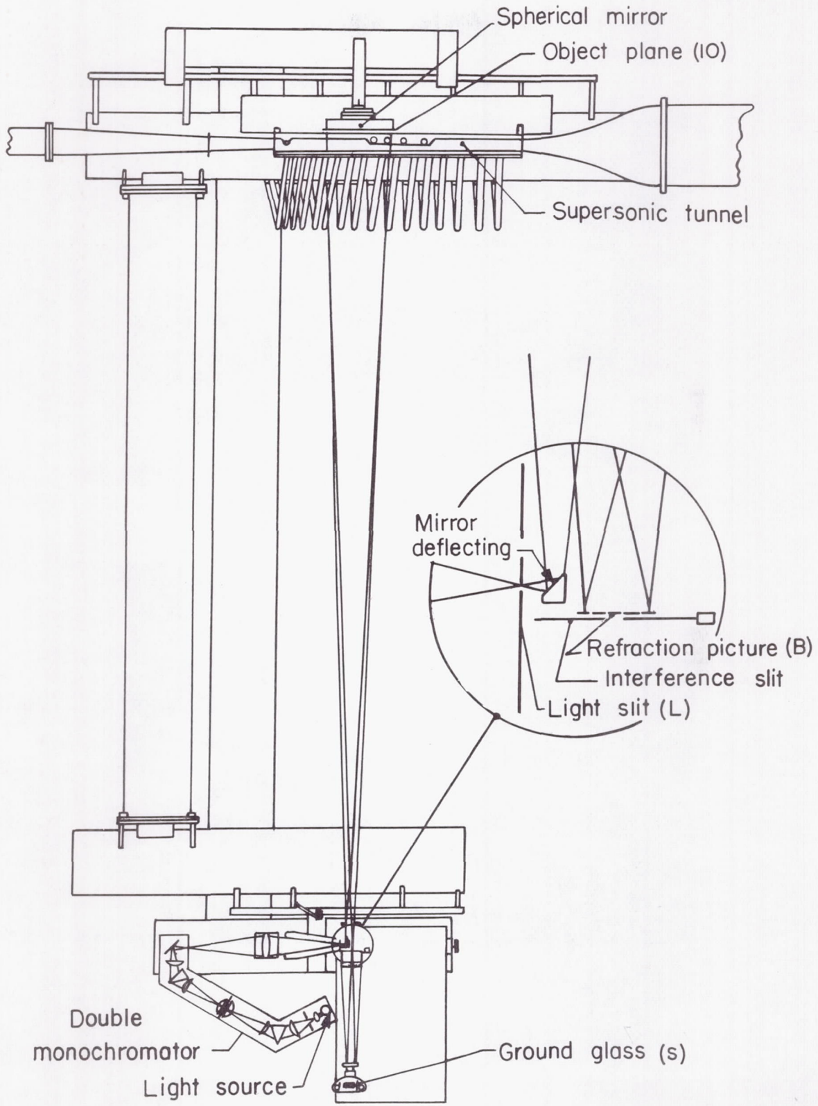
Figure 29.- Experimental setup.
