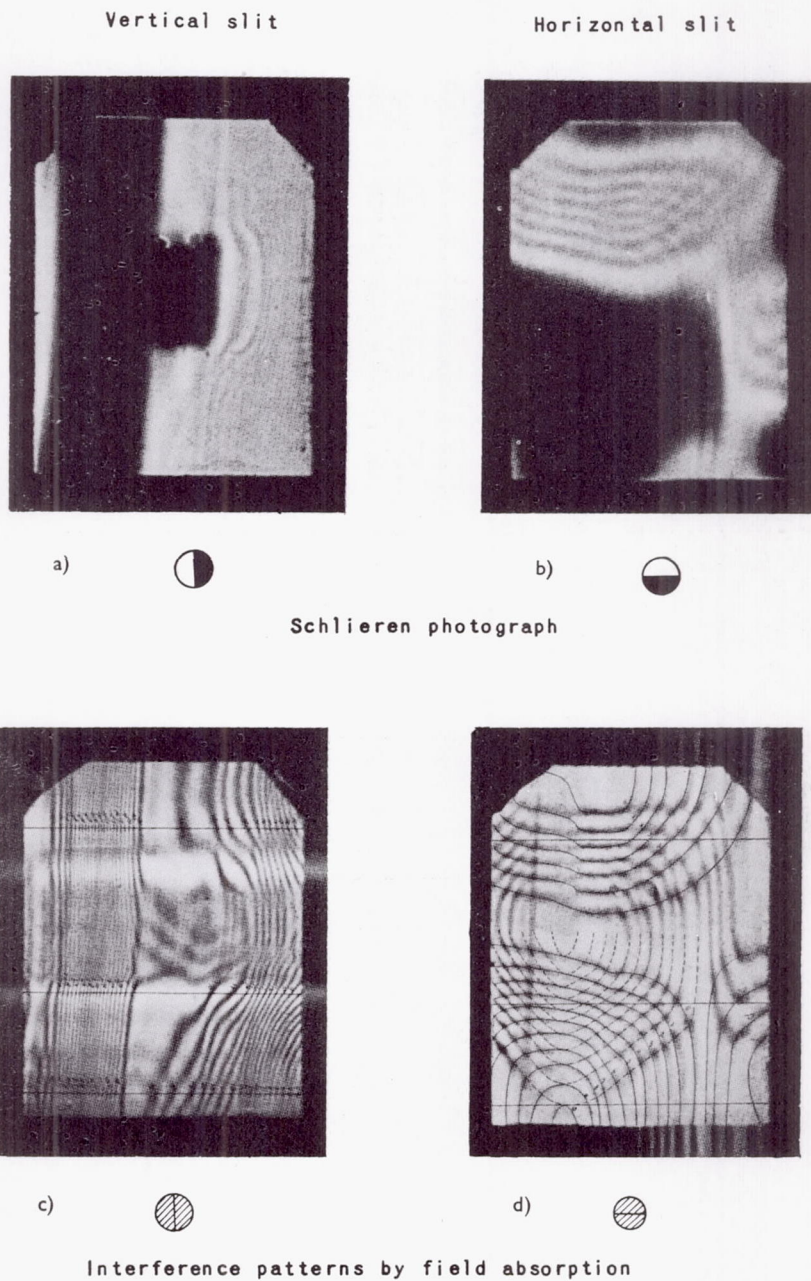
Figure 21.- Interference photographs by field absorption, small object glass.
