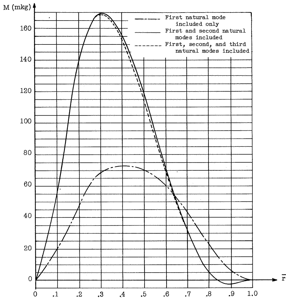
Figure 9.- N.C.2001 blade - blade bending moments for \psi = 0 .
