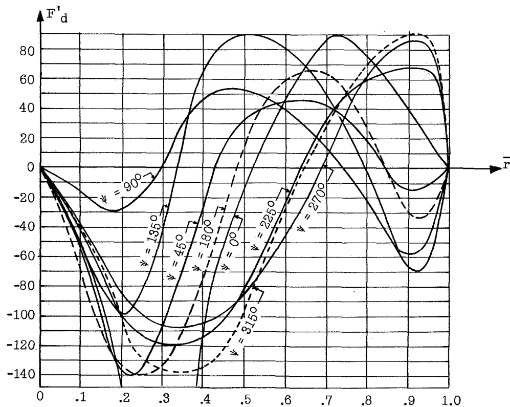
Figure 8.- N.C.2001 blade - total forces F'_d distributed over the rigid blade.
