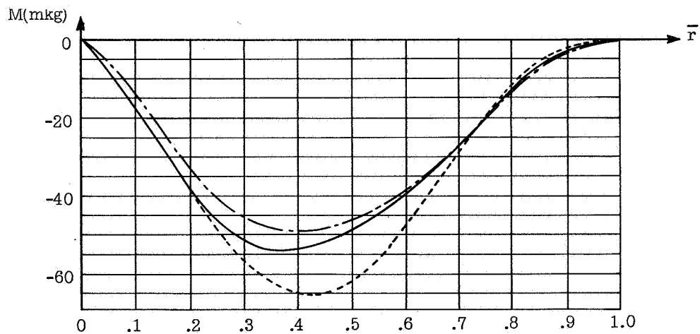
Figure 10.- N.C.2001 blade - blade bending moments for \psi = 90^\circ .
