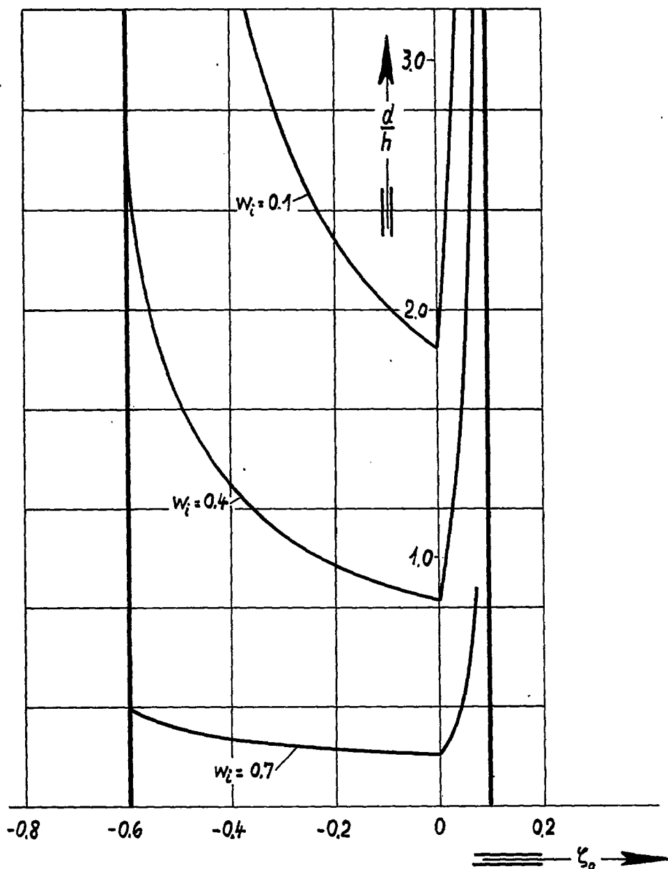
Figure 11.- The ratio of the wall thickness to the half opening height for the generalized symmetrical inlet with external compression as a function of \xi_0 for a constant w_{\max}/w_\infty = 1.2 for w_i/w_\infty = 0.1, 0.4, 0.7 . For the hodograph of the simplest symmetrical inlet with external compression of sections III and IV, \xi_0 equals zero, and d/h is a minimum.
