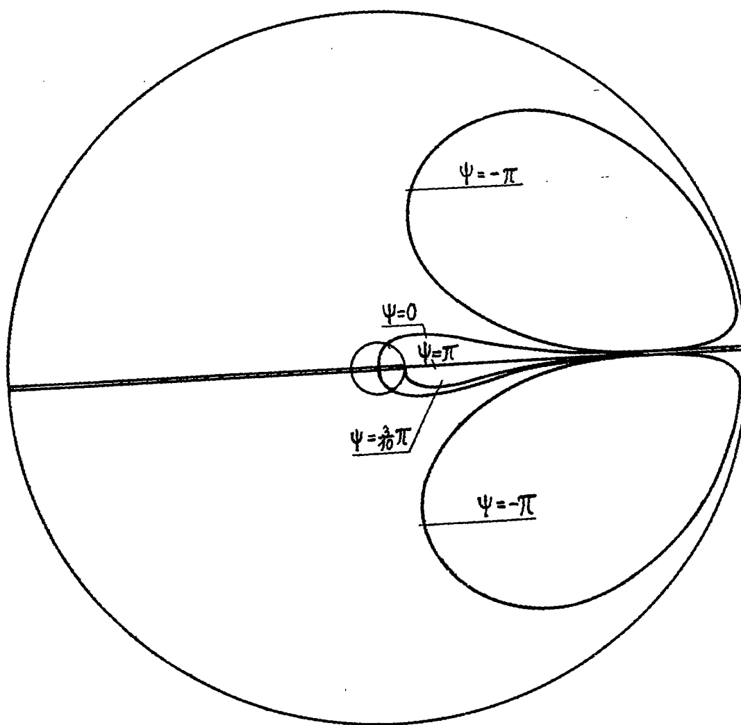
Figure 24.- In the hodograph for w_i/w_\infty = 0.1 , w_{\max}/w_\infty = 1.4 , the stream line \psi = 3\pi/10 barely satisfies the condition that it must lie outside of a circle of the radius w_i/w_\infty around the zero point.
