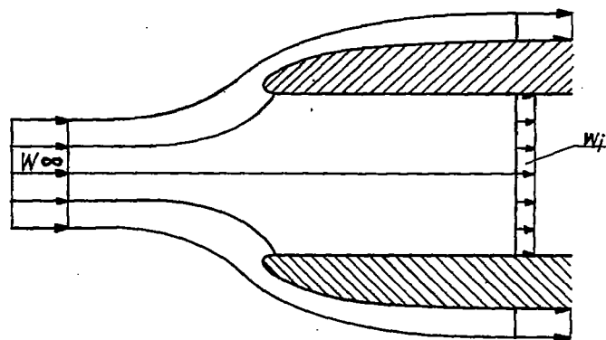
Figure 2.- External-compression inlet.
