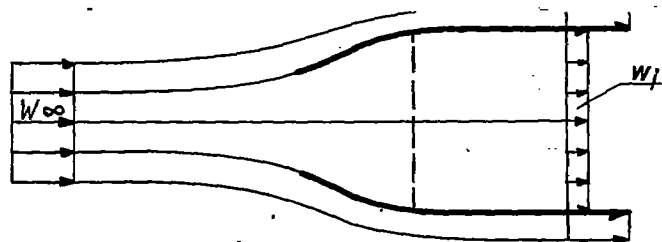
Figure 1.- Internal-compression inlet.
