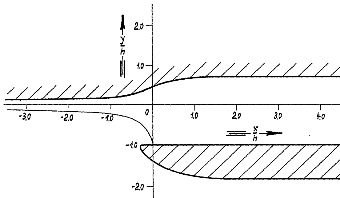
Figure 25.- If the stream line \psi = 3\pi/10 (see fig. 24) is made the solid wall, the pressure increases along this wall continuously and monotonically up to its end value p_i . ( w_i/w_\infty = 0.1 , w_{\max}/w_\infty = 1.4 ).
