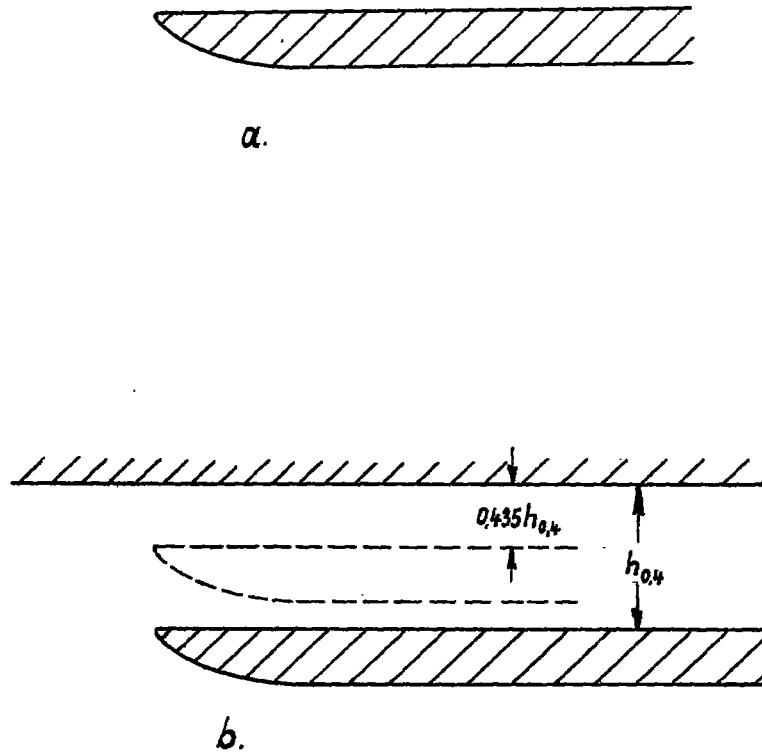
Figure 22.- Retractable inlet with external compression. In (a) the contour of the external-compression inlet for w_i/w_\infty = 0.4 , w_{\max}/w_\infty = 1.4 and the contour of the external-compression inlet for w_i/w_\infty = 0.1 and w_{\max}/w_\infty = 1.4 scaled to the same wall thickness are plotted on top of each other. A difference can no longer be represented. In (b) the positions of the retractable lower wall are represented for w_i/w_\infty = 0.4 (solid line) and for w_i/w_\infty = 0.1 (dashed line).
