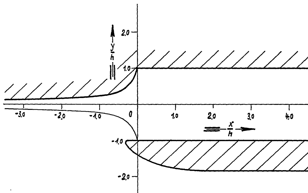
Figure 23.- With the stagnation-point stream line assumed as solid boundary, one obtains the most unsymmetrical external-compression inlet to be derived from the symmetrical one. ( w_1/w_\infty = 0.1 , w_{\max}/w_\infty = 1.4 ).
