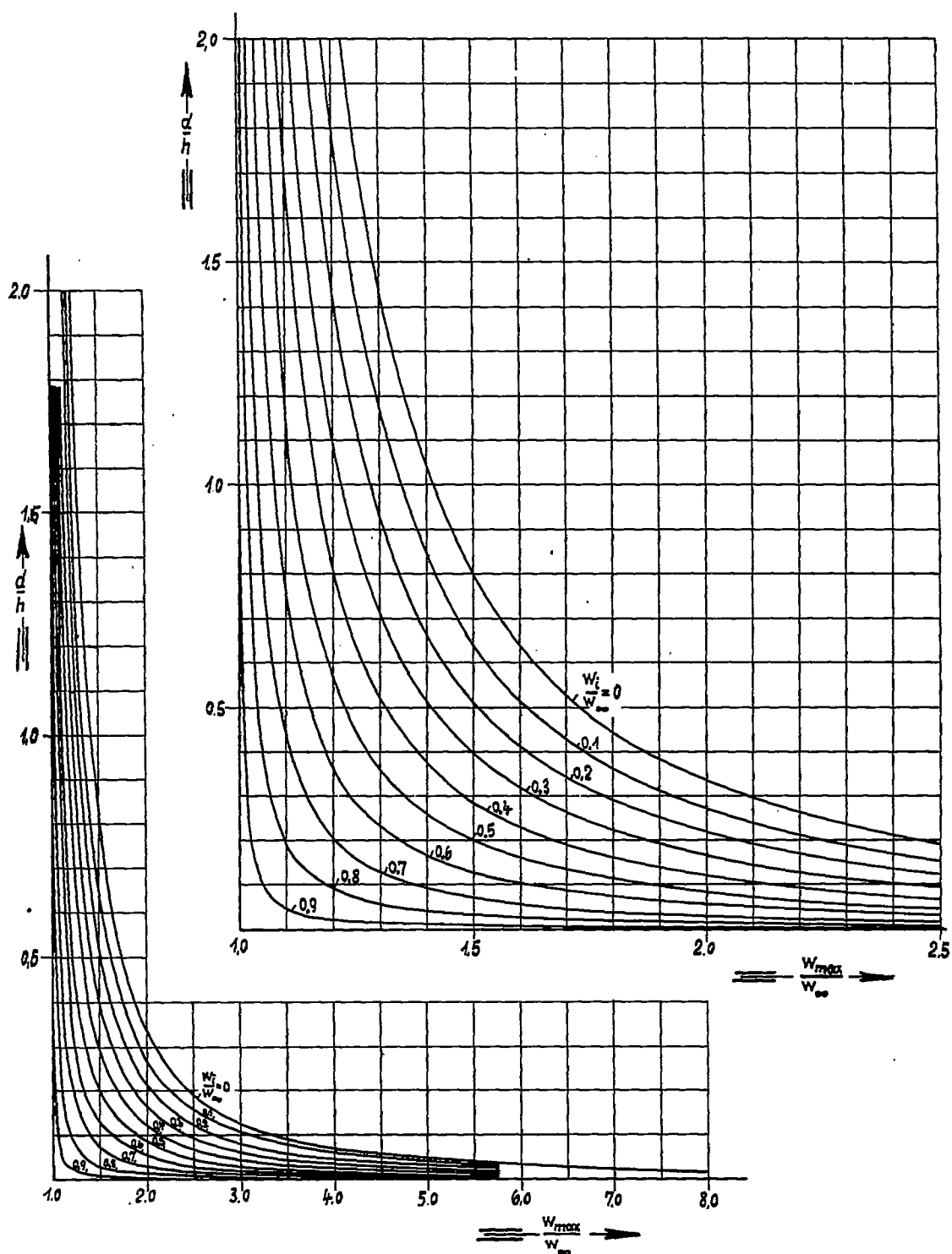
Figure 14.- The ratio d/h for the simplest symmetrical inlet with external compression as a function of w_{max}/w_{\infty} and w_i/w_{\infty} .
